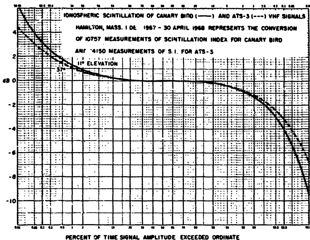
Figure 3-11a. Percent of Time Signal Amplitude Exceeded Ordinate
