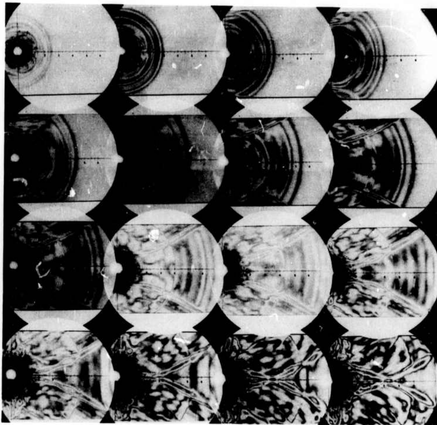
Fig. 6 ISOCHROMATIC FRINGE PATTERNS IN SPECIMEN NO. 8 ( \frac{1}{4} in. Thick Plexiglas; 100 mg PETN Charge; Camera Speed 180,000 in./sec)
