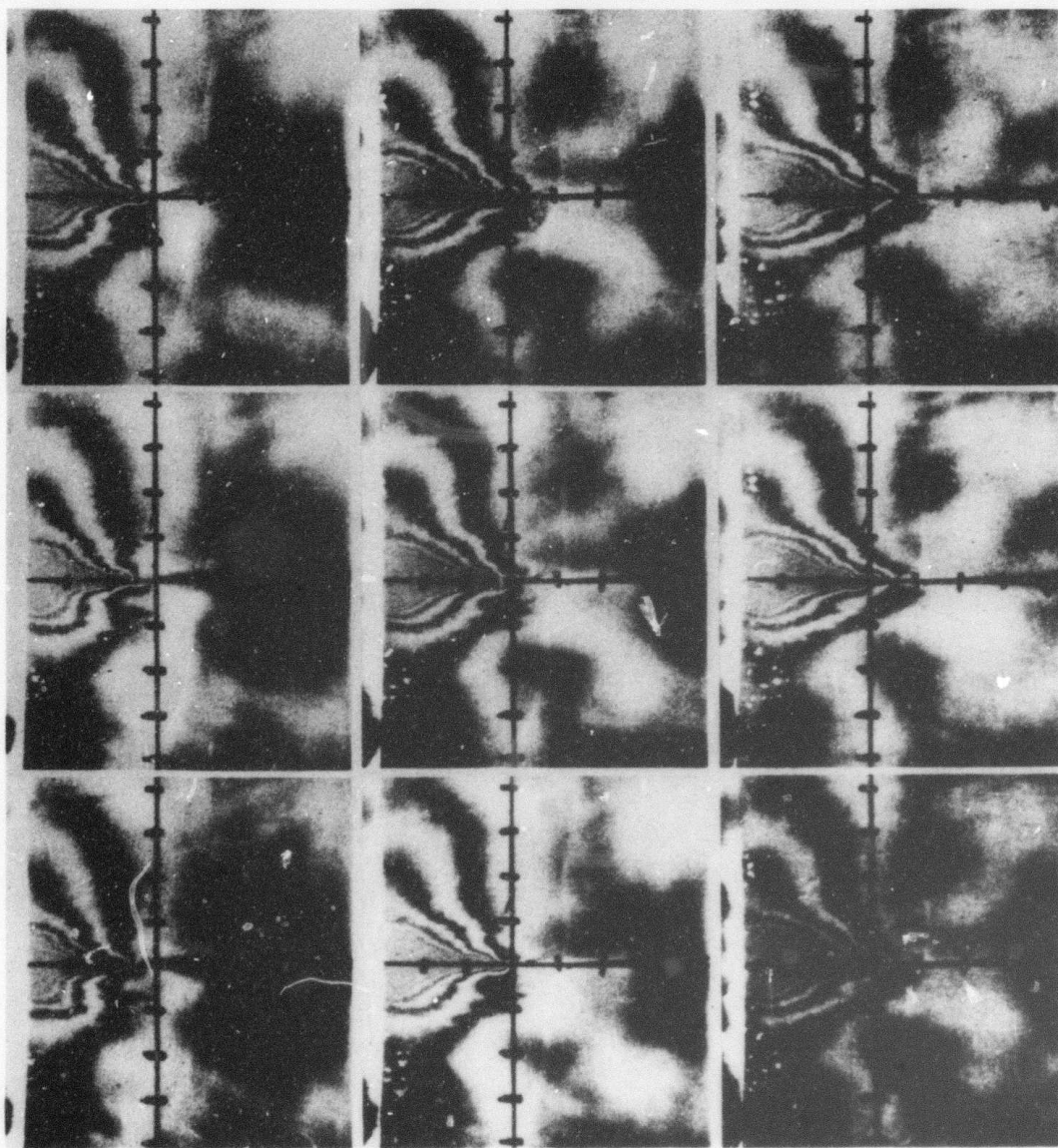
Fig. 37 CRACK PROPAGATION IN MARBLE PLATE LOADED EXPLOSIVELY THROUGH METAL WEDGE IN NOTCH (FRAMES SHOWN AT 4 \mu SEC INTERVALS; SPECIMEN 31573-3)
