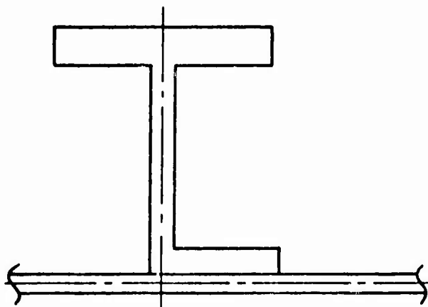
Fig. 2-1 Typical Stiffener
