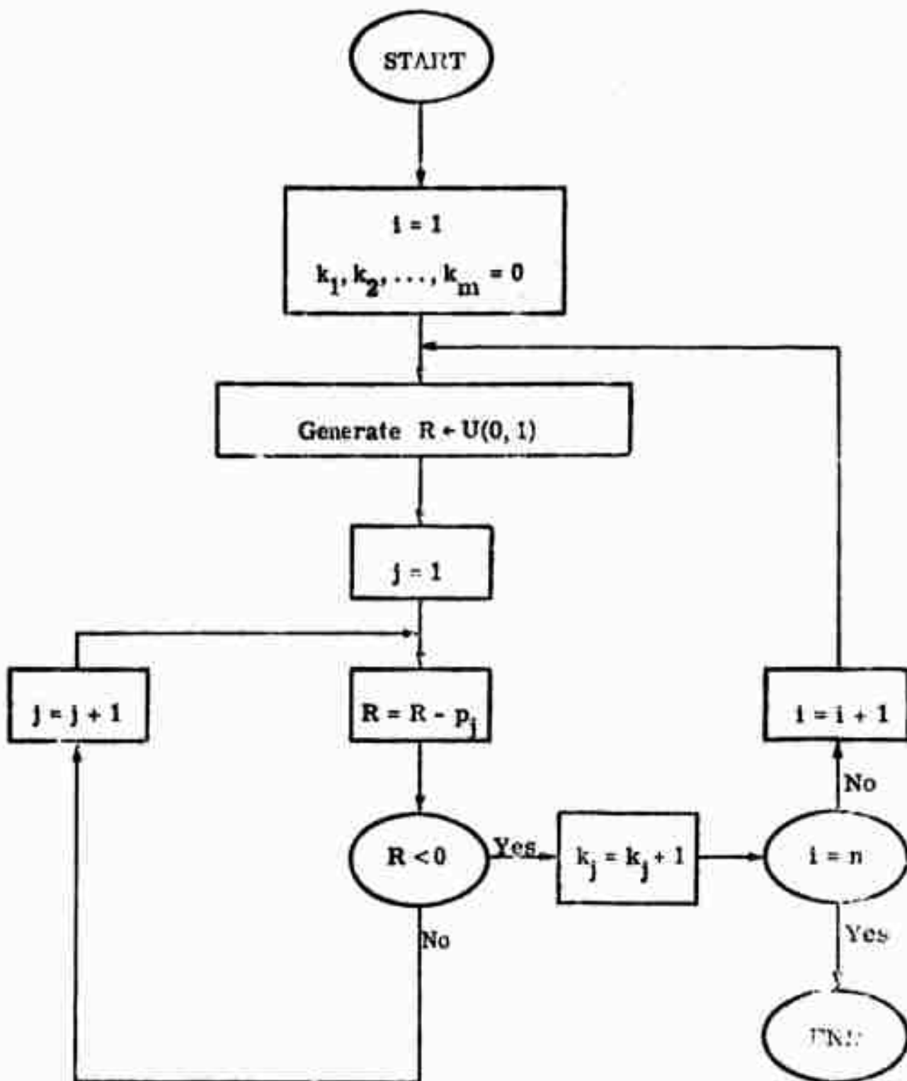
Figure 3-6. Random number generation algorithm for multinomial distribution
