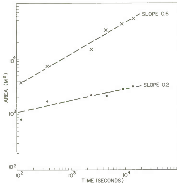
Fig. 4 — Area of the inner thick region (dots) and the total area of the visible slick (crosses) measured from the photography of the oil spill represented in Fig. 3 is plotted versus the time the picture was taken. The dashed lines are possible representations of the measurements.
