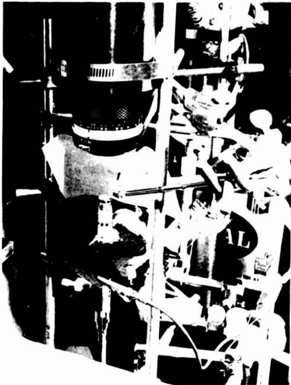
FIG. 9 CLOSE-UP OF DISK SHOWING TACHOMETER LIGHT REFLECTING OFF ITS SURFACE TO DENTAL MIRROR; X-Y-Z- POSITIONER MICROMETERS VISIBLE IN BACKGROUND
