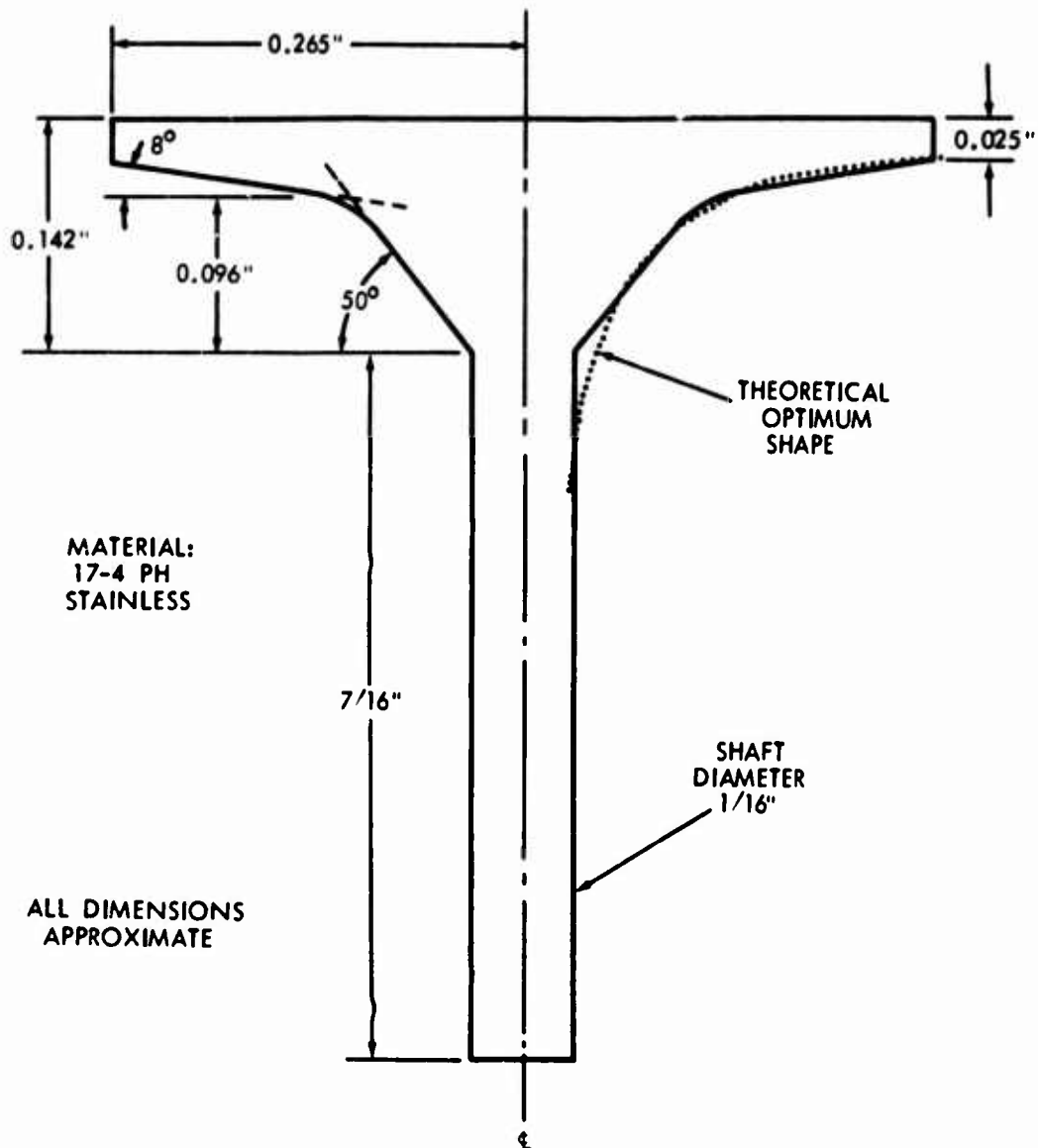
FIG. 3 HIGH-SPEED ROTOR CROSS-SECTION
