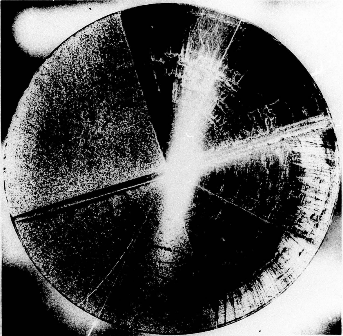
FIG. 7 FLASH PHOTOGRAPH OF DISK IN MOTION AT 6116 RPS AFTER FOUR MONTHS OF CONTINUOUS ROTATION. ARROW INDICATES SAME LINE SO INDICATED IN FIG. 6. DASHED CURVE SHOWS RELATIVITY EFFECT THAT WOULD HAVE BEEN SEEN FOR \alpha = 1/2
