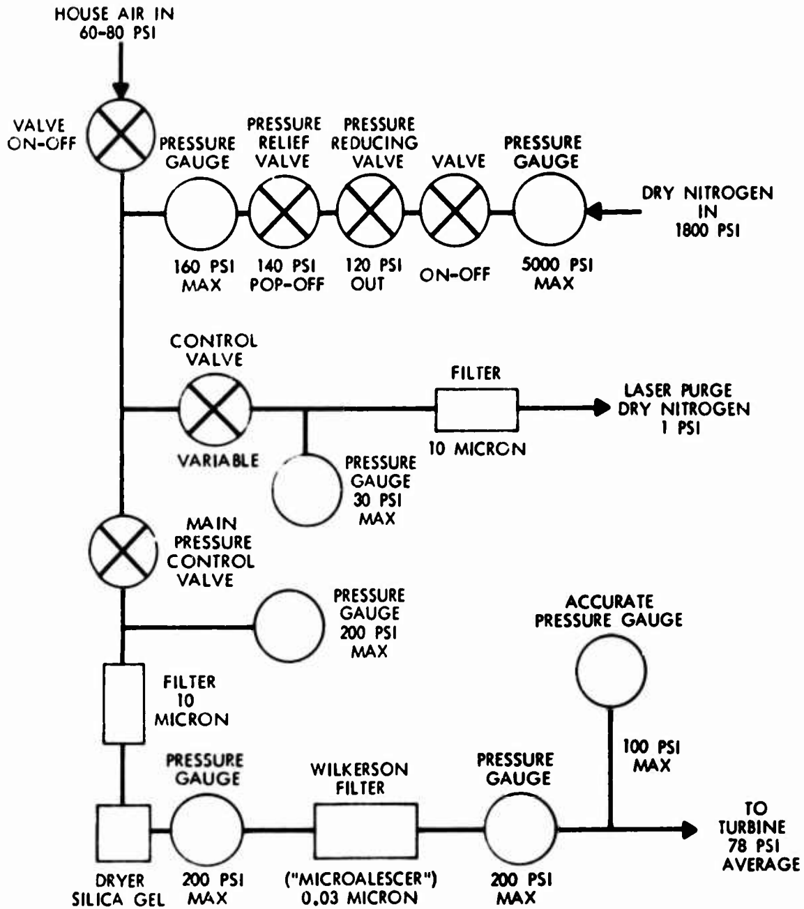
FIG. 4 SCHEMATIC OF PRESSURIZED GAS SUPPLY TO TURBINE
