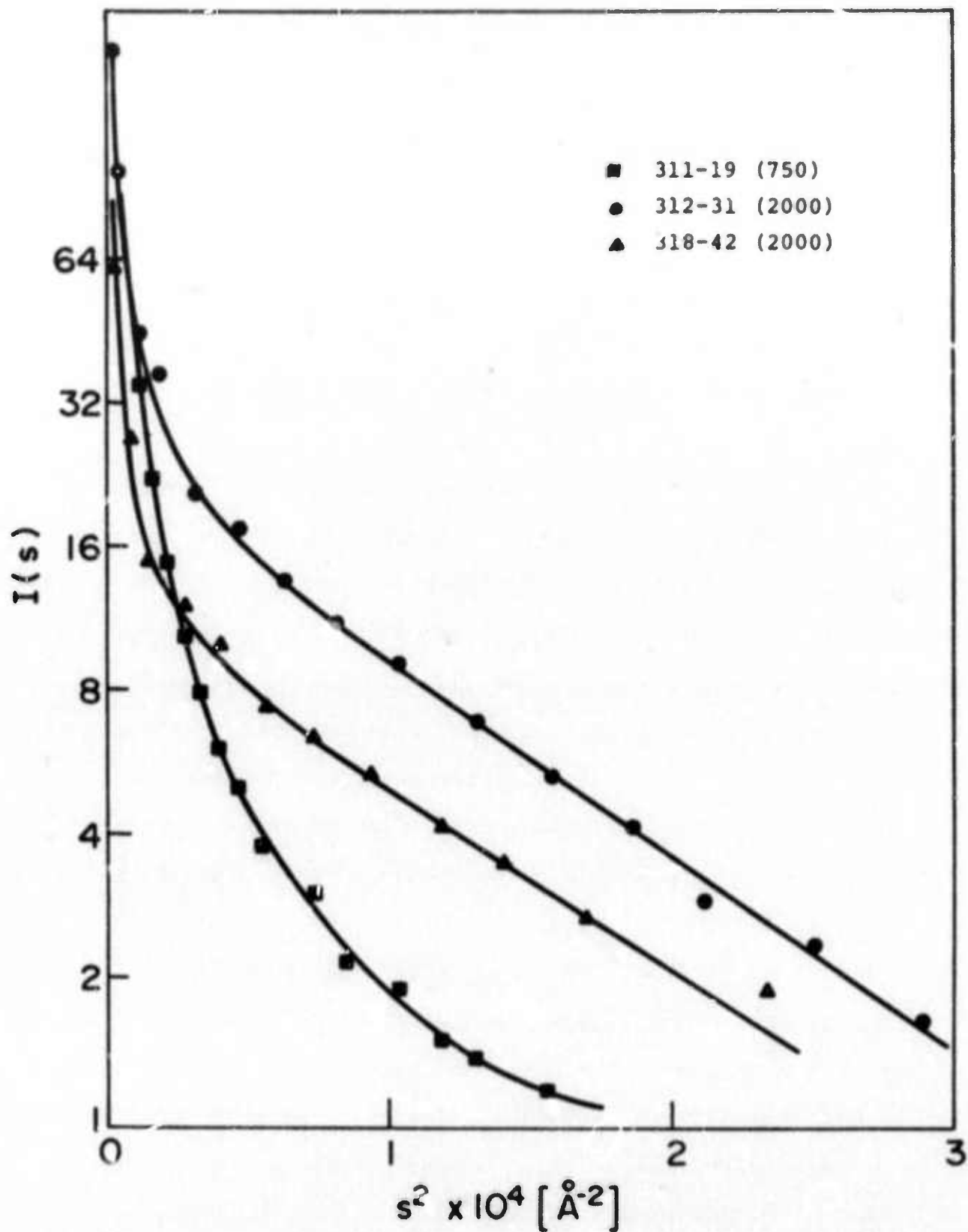
FIGURE 11. Guinier's plots for samples showing polydispersity.
