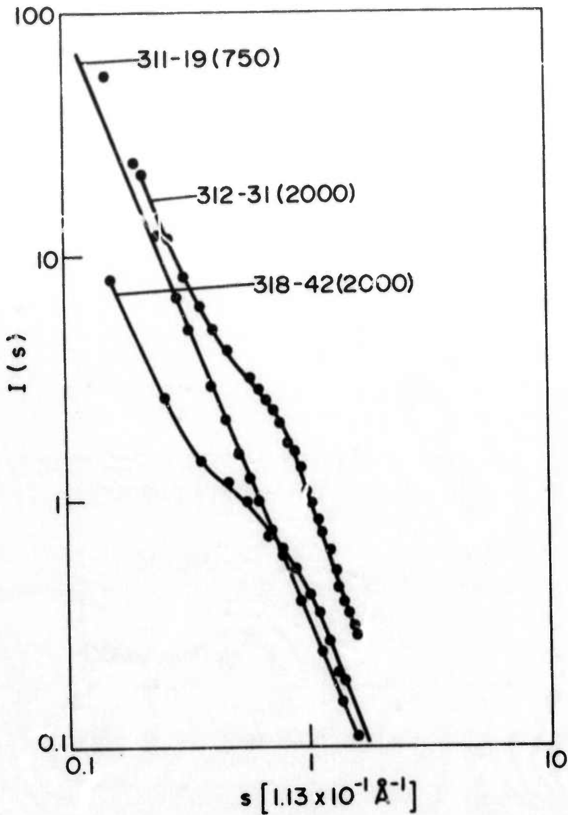
FIGURE 14. Porod's plots for samples showing polydispersity.
