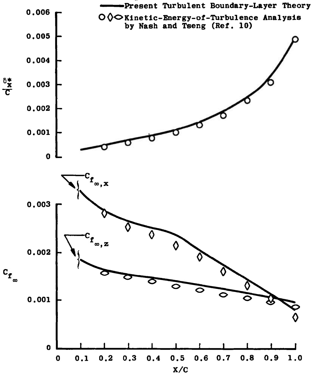
Fig. 9 Comparison of Turbulent Boundary-Layer Parameters with Infinite Yawed Wing Results of Nash and Tseng (Ref. 10)
