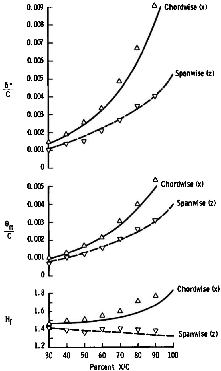
Fig. 19 Turbulent Boundary-Layer Parameters on a Lifting Infinite Yawed Airfoil
