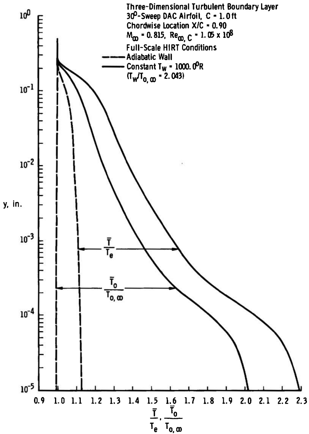
Fig. 34 Hot-Wall Effects on Turbulent Boundary-Layer Temperature Profiles
