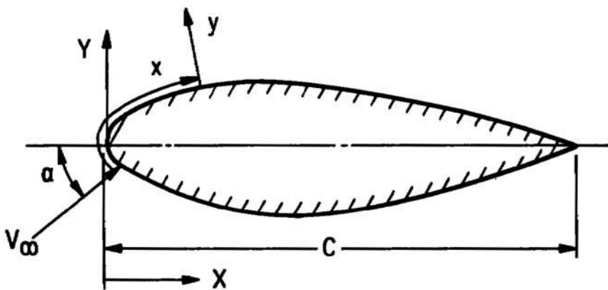
b. Chordwise Section of Wing Fig. 2 Infinite Yawed Wing Geometry and Nomenclature
