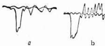
Fig. 2. a) oscillogram of cathode voltage (calibration signal 10 MHz) b) oscillogram of beam current (calibration signal 100 MHz).
