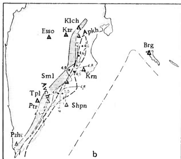
Fig. 5. Velocities V_P (a) and V_S (b) in the Mantle at a Depth of 120 Km.
