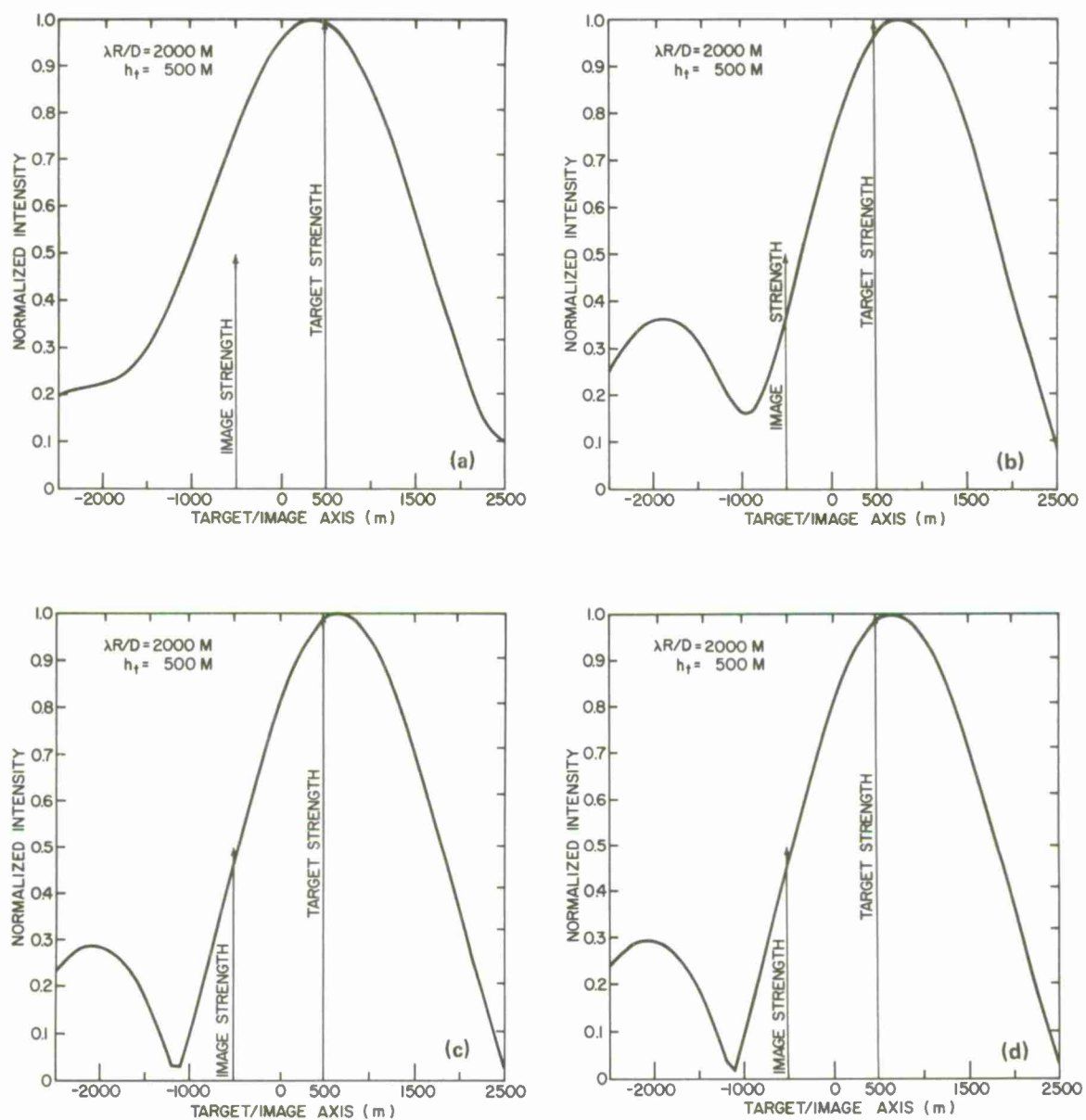
Fig. 4 — Pattern of a self-focusing antenna when the target/image spacing is half beam-width. (a) One iteration, (b) Two iterations, (c) Five iterations, (d) Ten iterations.
