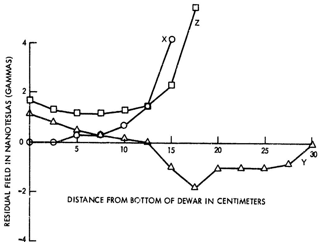
FIG. 8 MAGNETIC FIELD VALUES IN SMALL DEWAR AFTER 2ND BAG.
