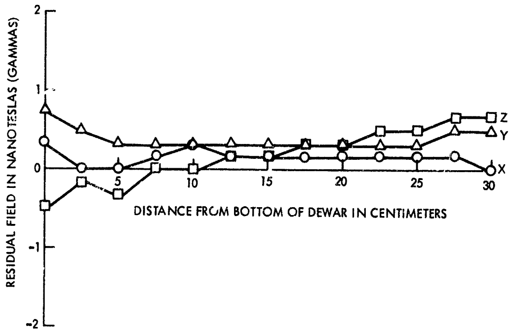
FIG. 9 MAGNETIC FIELD VALUES IN SMALL DEWAR AFTER 3RD BAG.
