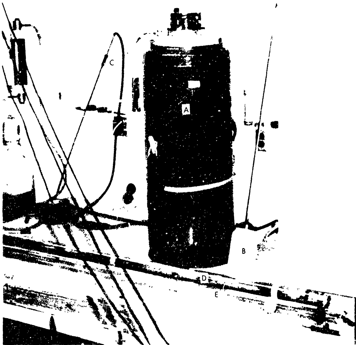
FIG. 1 SUPERCONDUCTING SHIELD ASSEMBLY BUILT BY THE NAVAL ORDNANCE LABORATORY FOR THE NASA AMES RESEARCH CENTER
