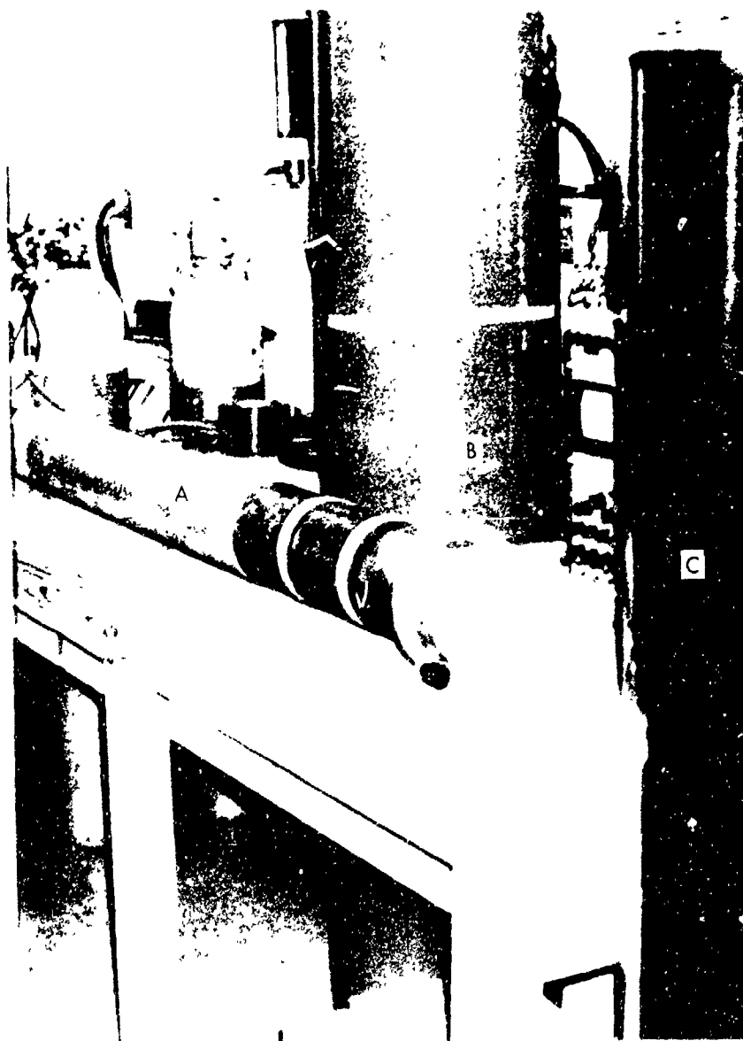
FIG. 2 DEWARS USED FOR SUPERCONDUCTING SHIELD A. ROOM TEMPERATURE ACCESS DEWAR B. LIQUID HELIUM FILLED OUTER DEWAR C. POT DEWAR FOR PRE-COOLING
