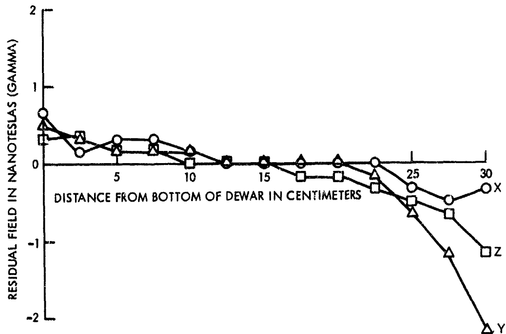
FIG. 7 MAGNETIC FIELD VALUES IN 10 CENTIMETER DEWAR AFTER 3RD BAG.
