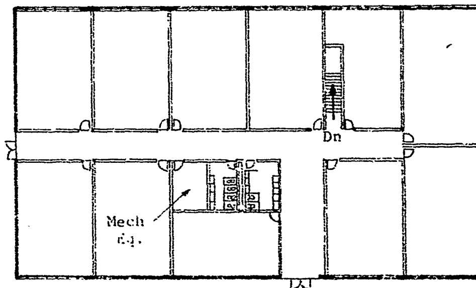
Fig. 4.2b Building with Blast Shelter Below Grade (Plan)
