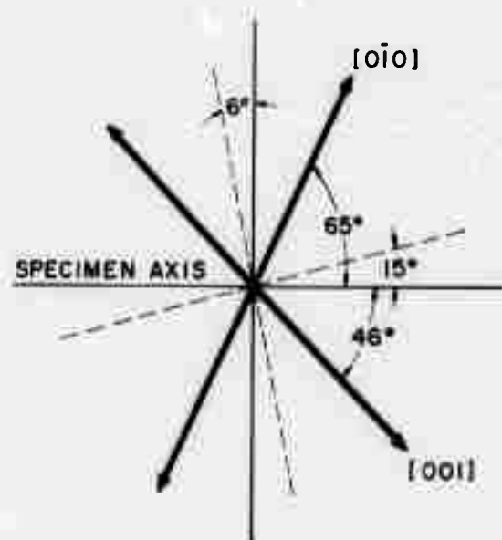
PROJECTION OF CRYSTAL AXES ON A PLANE NORMAL TO THE REFLECTED BEAM. ANGLE OF INCIDENCE = 47.5^\circ
