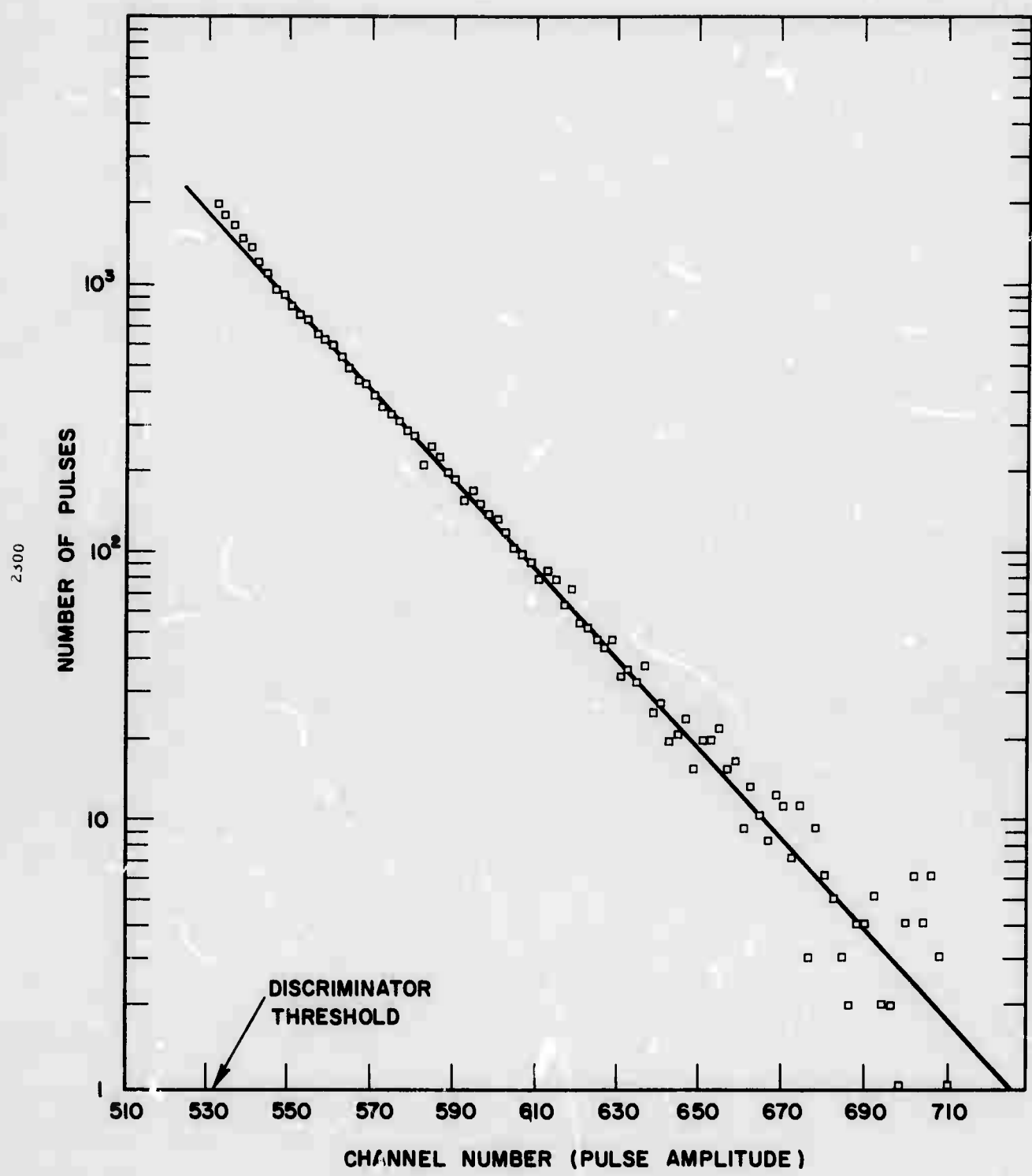
FIGURE 9. BARKHAUSEN PULSE HEIGHT DISTRIBUTION FOR ANNEALED POLYCRYSTALLINE Fe-3.2%Si SPECIMEN
