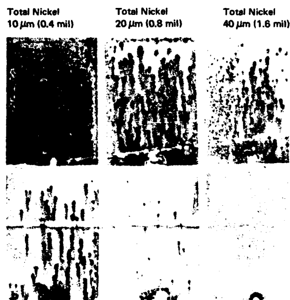
Figure 2 - Nickel plated steel panels (0.5 \mu\text{m} chromium topcoat) after 35 months' exposure to tropical open field environment. A-Single-layer nickel. B-Double-layer nickel.
