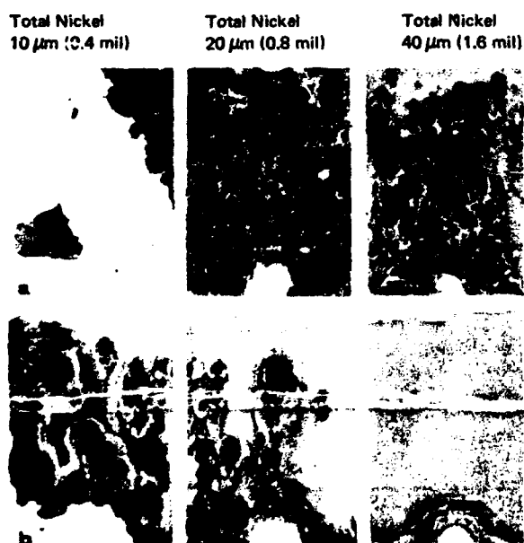
Figure 1 - Nickel plated steel panels (0.5 \mu\text{m} chromium topcoat) after 35 months' exposure to tropical marine environment. A-Single-layer nickel. B-Double-layer nickel.
