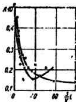
Fig. 35. Dependence of coefficient K on reduced dissolution time: ○ - solution in pure aluminum; × - solution in aluminum with 3 wt. % silicon added.
