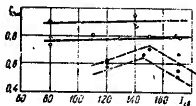
Fig. 38. Average value of the efficiency \eta_{бим} of the heating of a manufactured article by an arc: ○ - bead forming on the aluminum cladding; ● - bead forming on the steel base.
