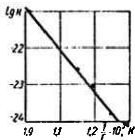
Fig. 20. Dependence of \ln k = f\left(\frac{1}{T}\right) for armco iron/aluminum bimetal.
