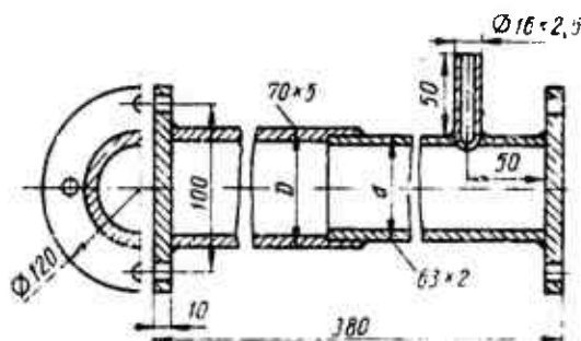
Fig. 88. Tubular steel/aluminum specimen manufactured for vibration testing.
