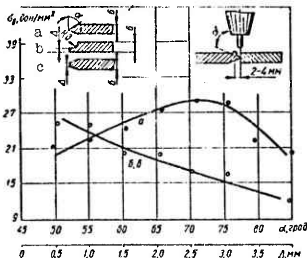
Fig. 76. Strength of a welded steel/aluminum joint as a function of the type of edge dressing on the steel plate (of edge bevel angle \alpha and shouldering of the edge, \Delta ).
