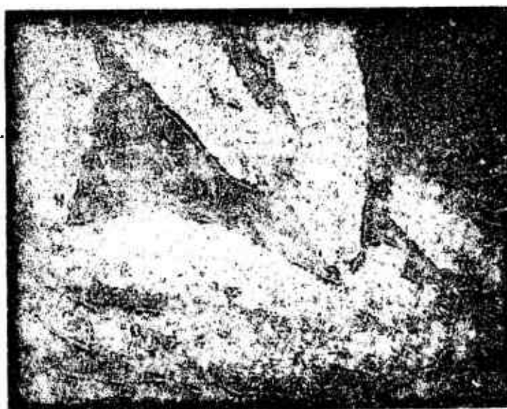
Fig. 14. Microstructure of weld metal during facing with a filler of aluminum AD1 on steel St. 3 ( \times 300 ).
