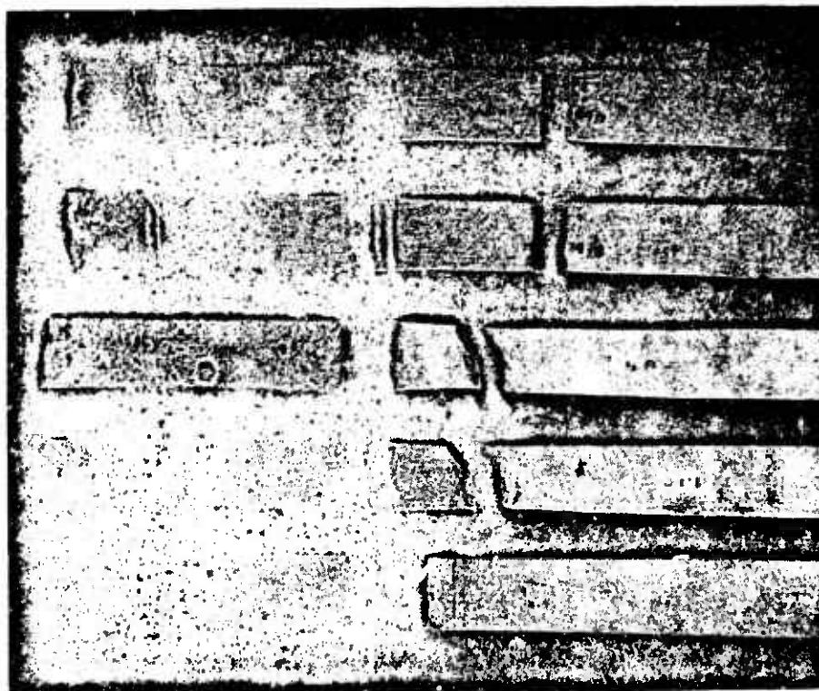
Fig. 79. Fracture specimens of a joint between steel 1Kh18N9T and alloy AMg6 (on the right) (width of diffusion zone 5 \mu m).
