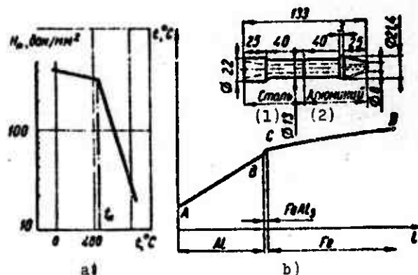
Fig. 8. Temperature dependence of hardness and heat conductivity of intermetallic phases: a) for FeAl_m ; b) for FeAl_3 (AB corresponds to the steel portion of the specimen and BC, to the compound FeAl_3 , and CD to the aluminum portion of the specimen [191]). The average thickness of the FeAl layer is \sim 0.12 mm. KEY: (1) Steel; (2) Aluminum.
