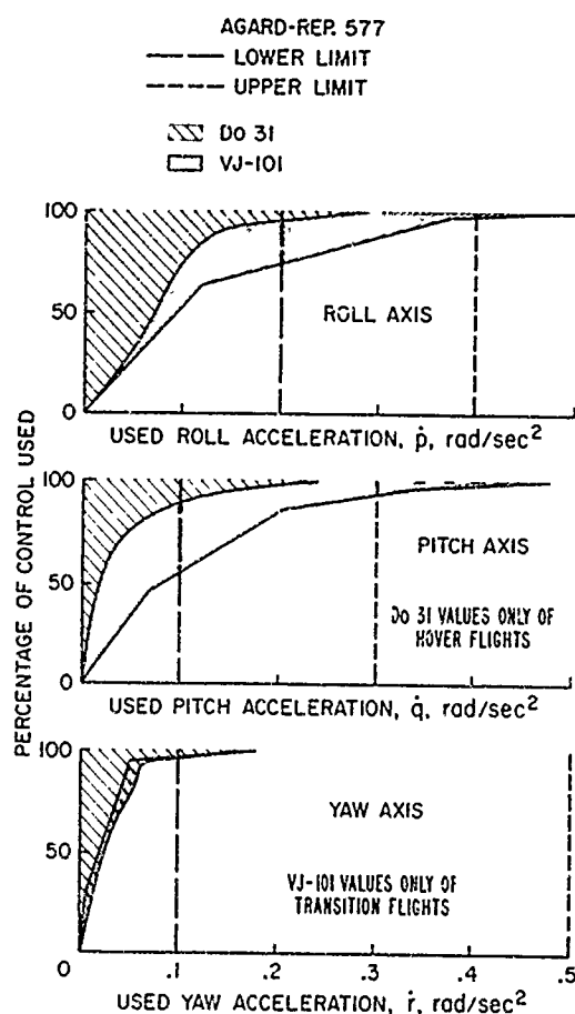
Figure 47. Envelope of Control Acceleration Used in Hover and Transition (Ref. 22).
