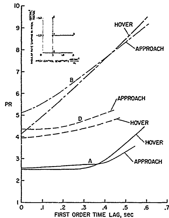
Figure 23. First-Order Time Lag Results.
