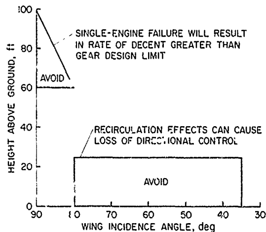
Figure 85. Single Engine Failure Boundaries for XC-142 Aircraft.
