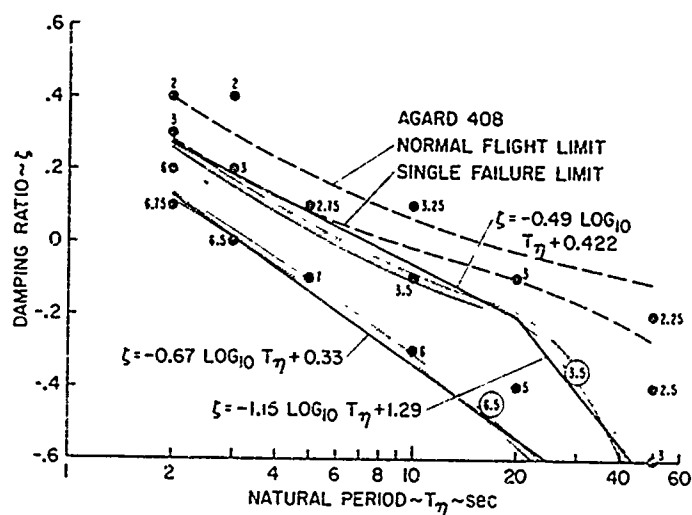
Figure 46. Longitudinal Damping - Period Characteristics for Hover Task.
