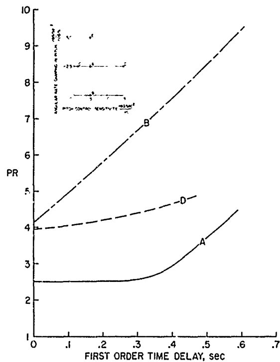
Figure 24. First-Order Time Delay Results - Hovering Task.
