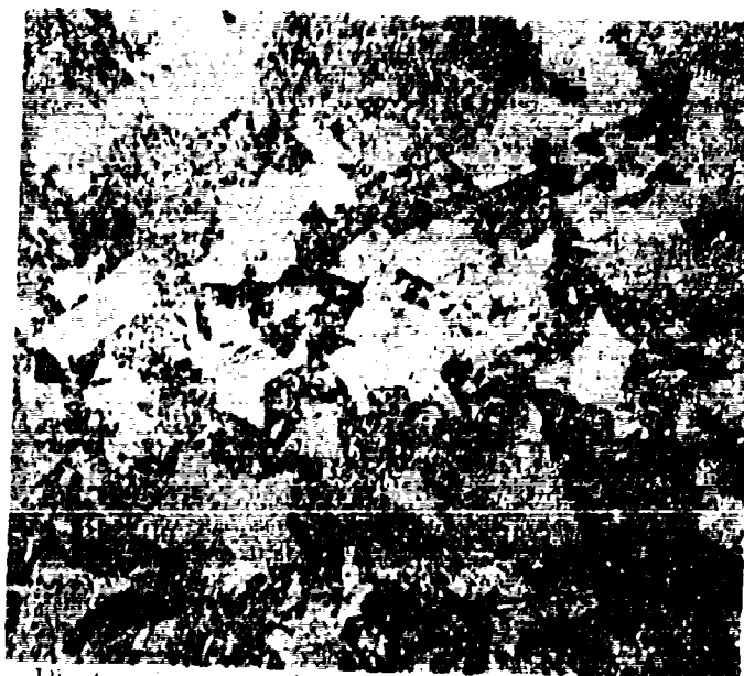
Figure 2-6. Photomicrograph showing secondary grain growth of boron suboxide. (250X)
