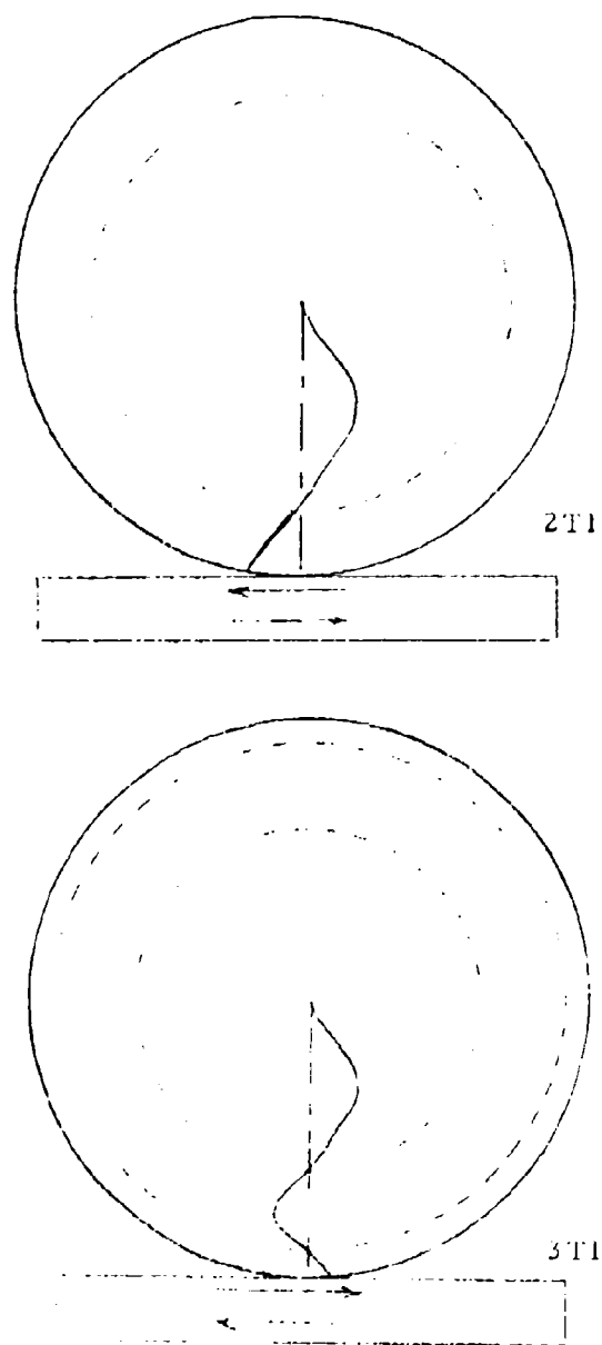
Figure A-1 Schematic Representation of Two Torsional Modes.
