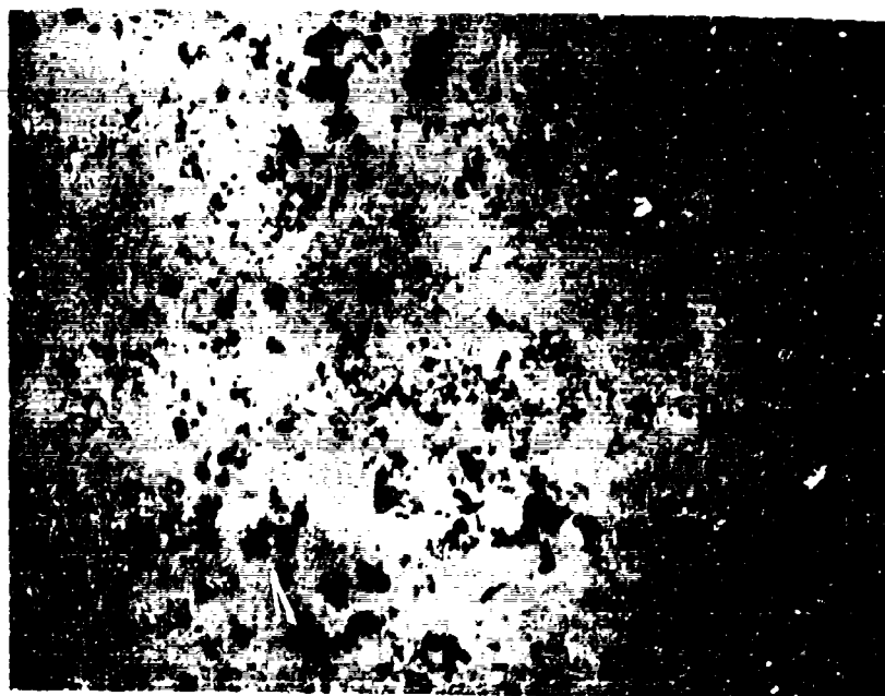
Figure 2-3. Photomicrograph of a 78 wt % boron specimen. (200X)
