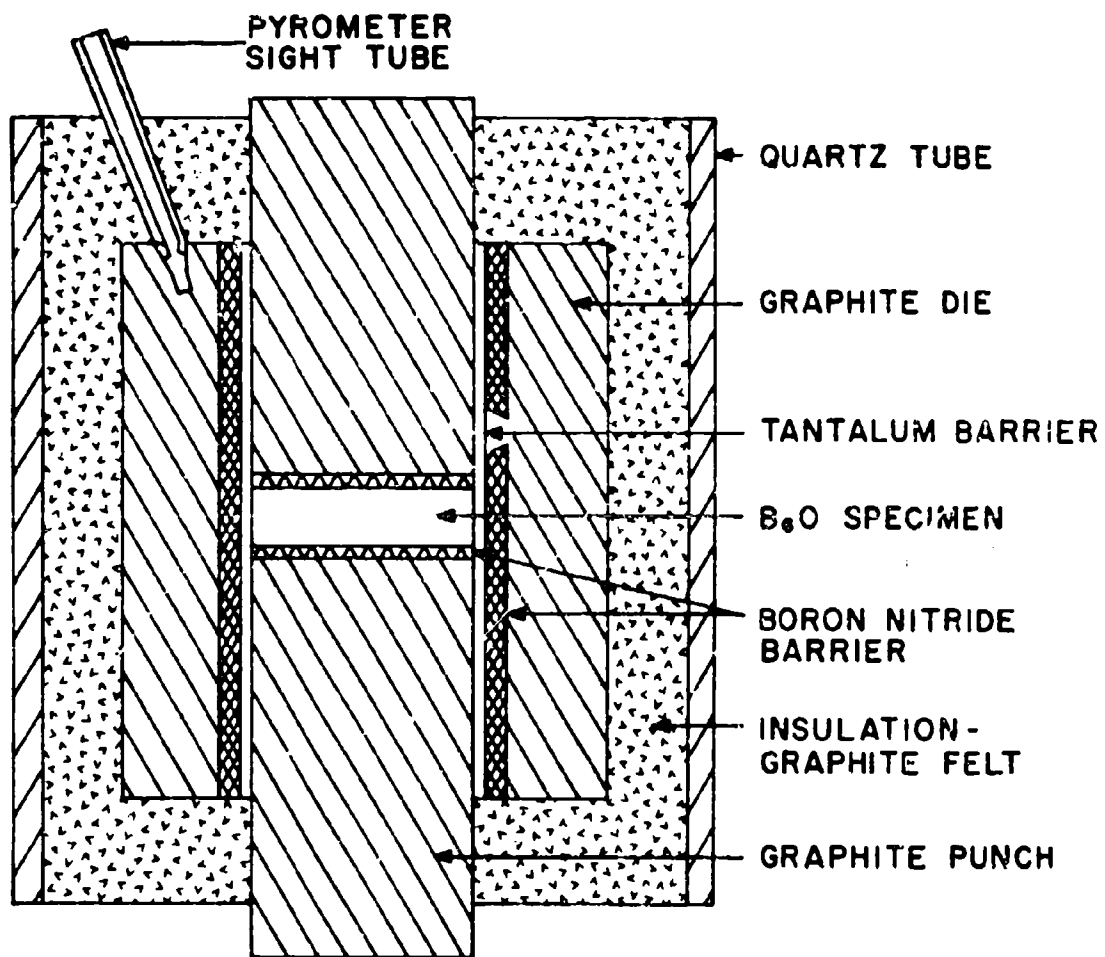
Figure 2-2. Furnace and die assembly for hot pressing boron suboxide
