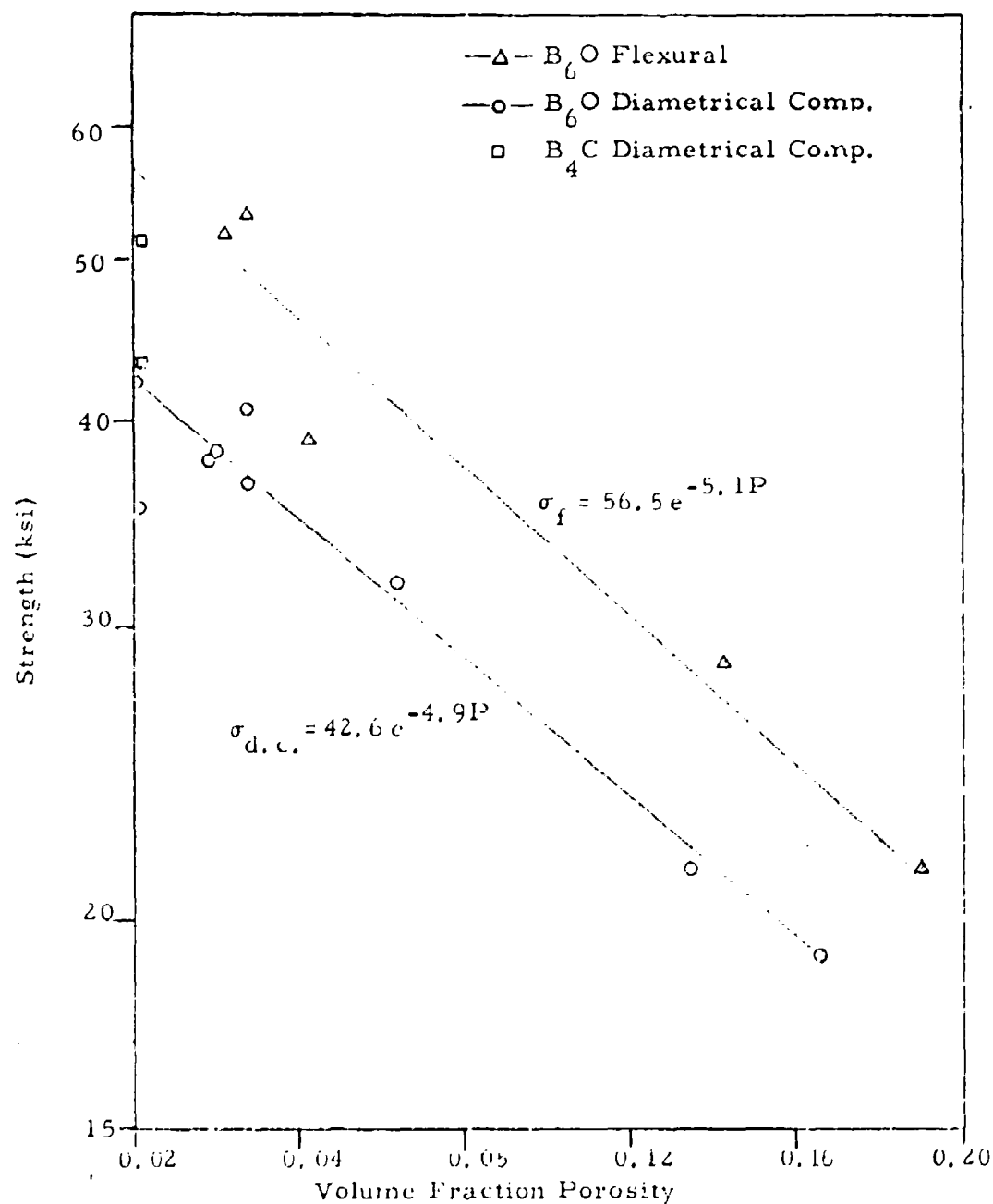
Figure 6-4. Diametrical Compression Strength of B_6O and B_4C versus Porosity and Flexural Strength of B_6O versus Porosity
