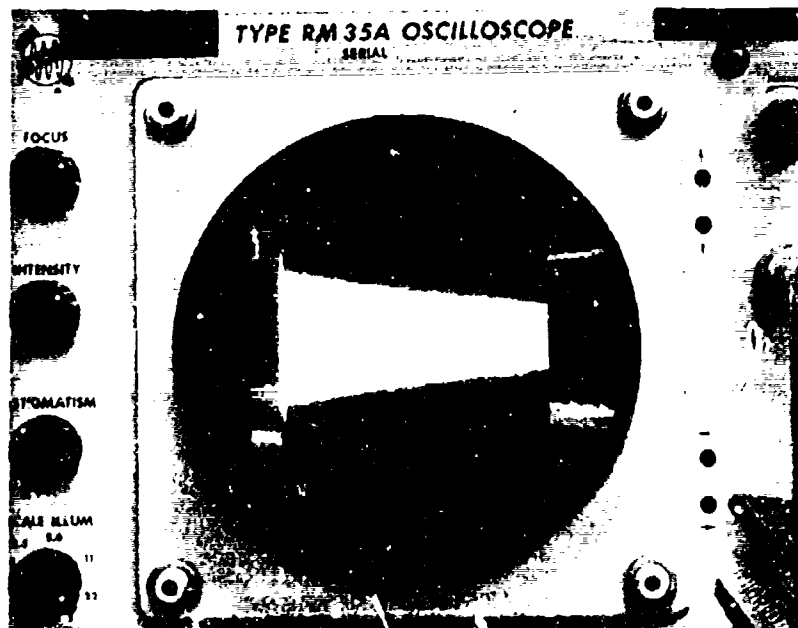
Figure A-4. Oscilloscope pattern showing resonant condition.
