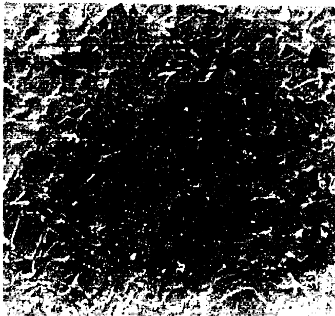
Figure 2-5. Electron micrograph of a 99% dense 80 wt % boron specimen. (Replication of a fractured and etched surface. 10,000X)
