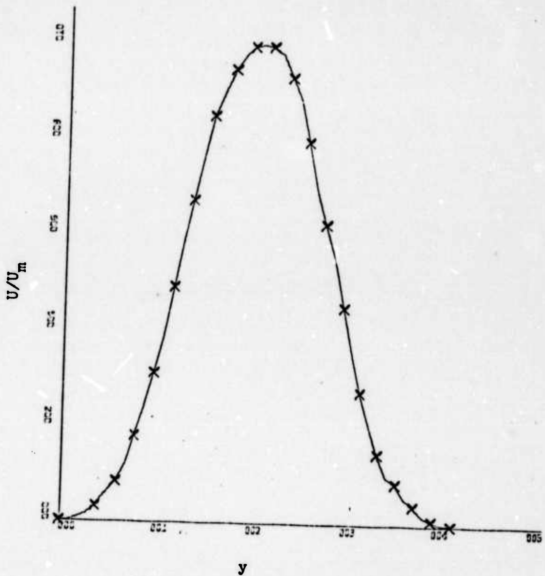
Figure 94. Velocity Profile at 9.58 Inches Downstream of Jet Exit for Jet Width of 1.31 Inches.
