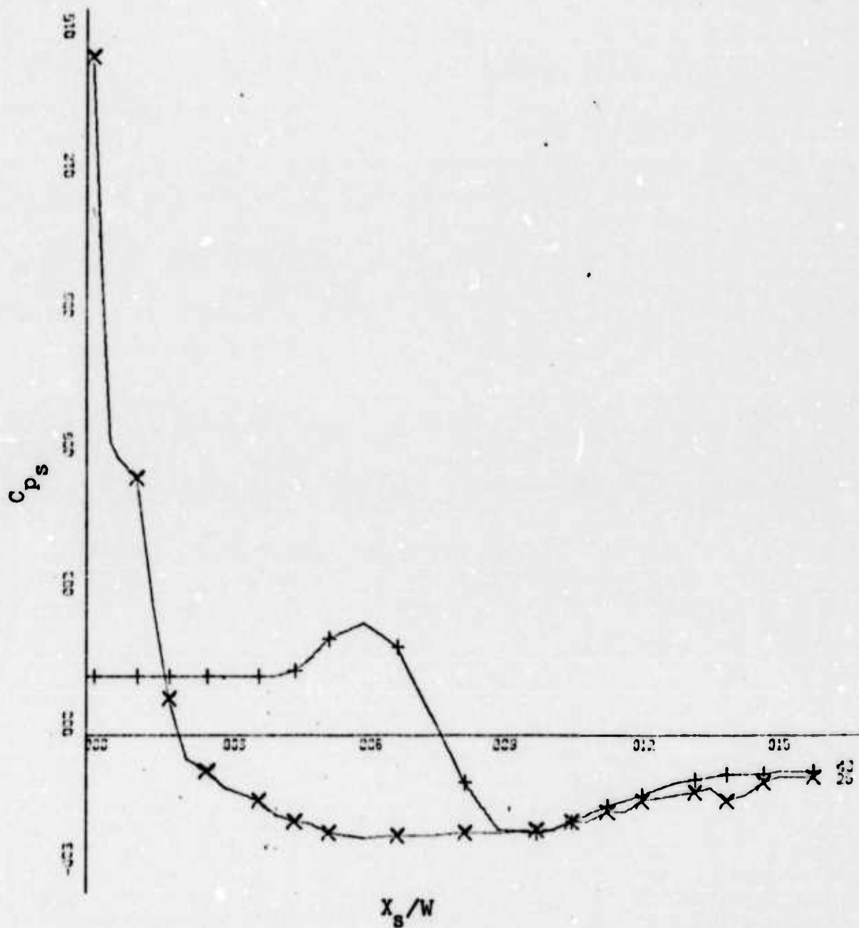
Figure 87. Surface Pressure Coefficient vs. Wall Position for Concave Wall at Various Deflection Angles and Offset Distance ( D/W ) of 0.18, Jet Width of 2.62 Inches, Re = 2.05 \times 10^5 , \alpha = 25, 40 degrees.
