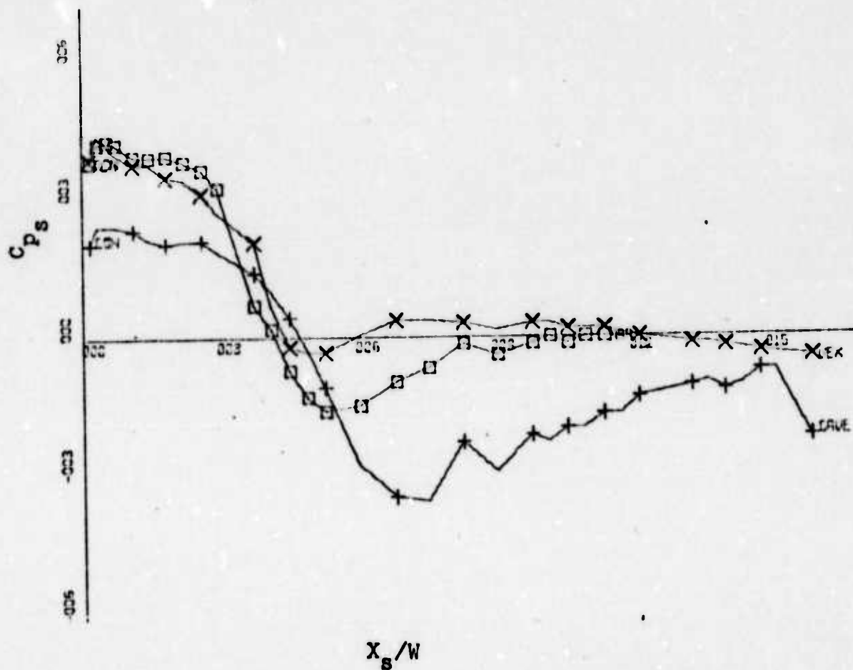
Figure 88. Surface Pressure Coefficient vs. Wall Position for Planar, Concave, and Convex Walls, for 30 Degrees Deflection Angle and Offset Distance (D/W) of 0.0, Jet Width of 2.62 Inches, Re = 2.05 \times 10^5 .
