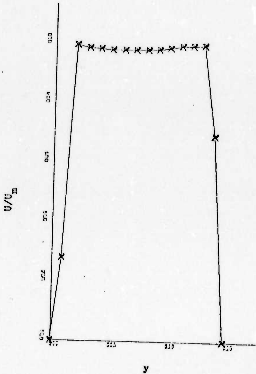
Figure 89. Velocity Profile at 0.5 Inches Downstream of Jet Exit for Jet Width of 1.31 Inches.
