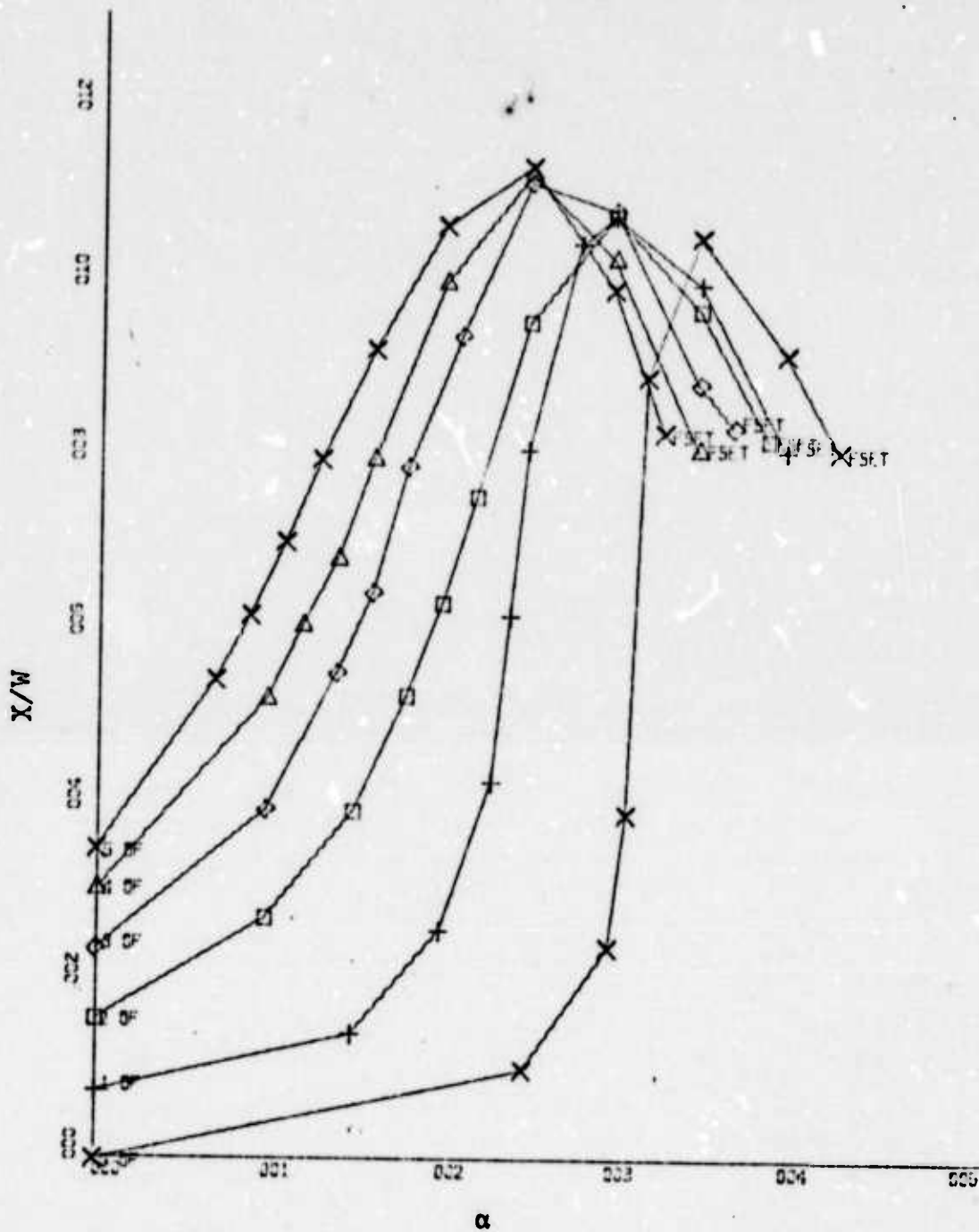
Figure 48. Attachment Distance vs. Deflection Angle for Various Offset Distances, Jet Width of 2.62 inches, Concave Wall, Re = 2.05 \times 10^5 , D/W of 00, 01, 02, 03, 04, 05.
