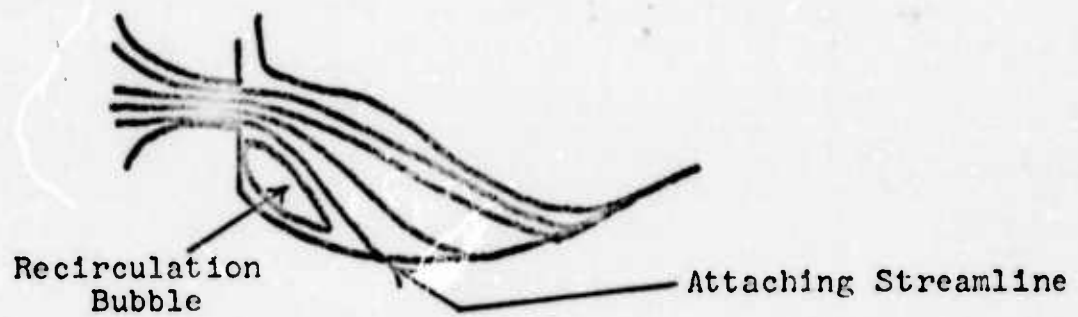
Figure 2. Flow Model for Concave Wall
