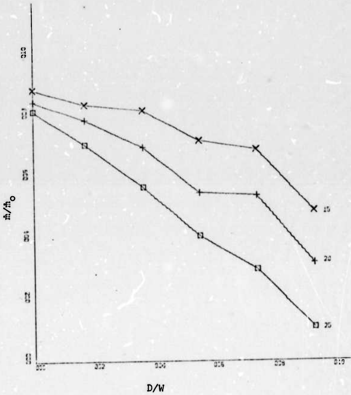
Figure 36. Flow Rate vs. Offset Distance for Convex Wall at Constant Deflection Angles, Jet Width = 2.62 inches, Re = 2.05 \times 10^5 , \alpha = 15, 20, 25 degrees.
