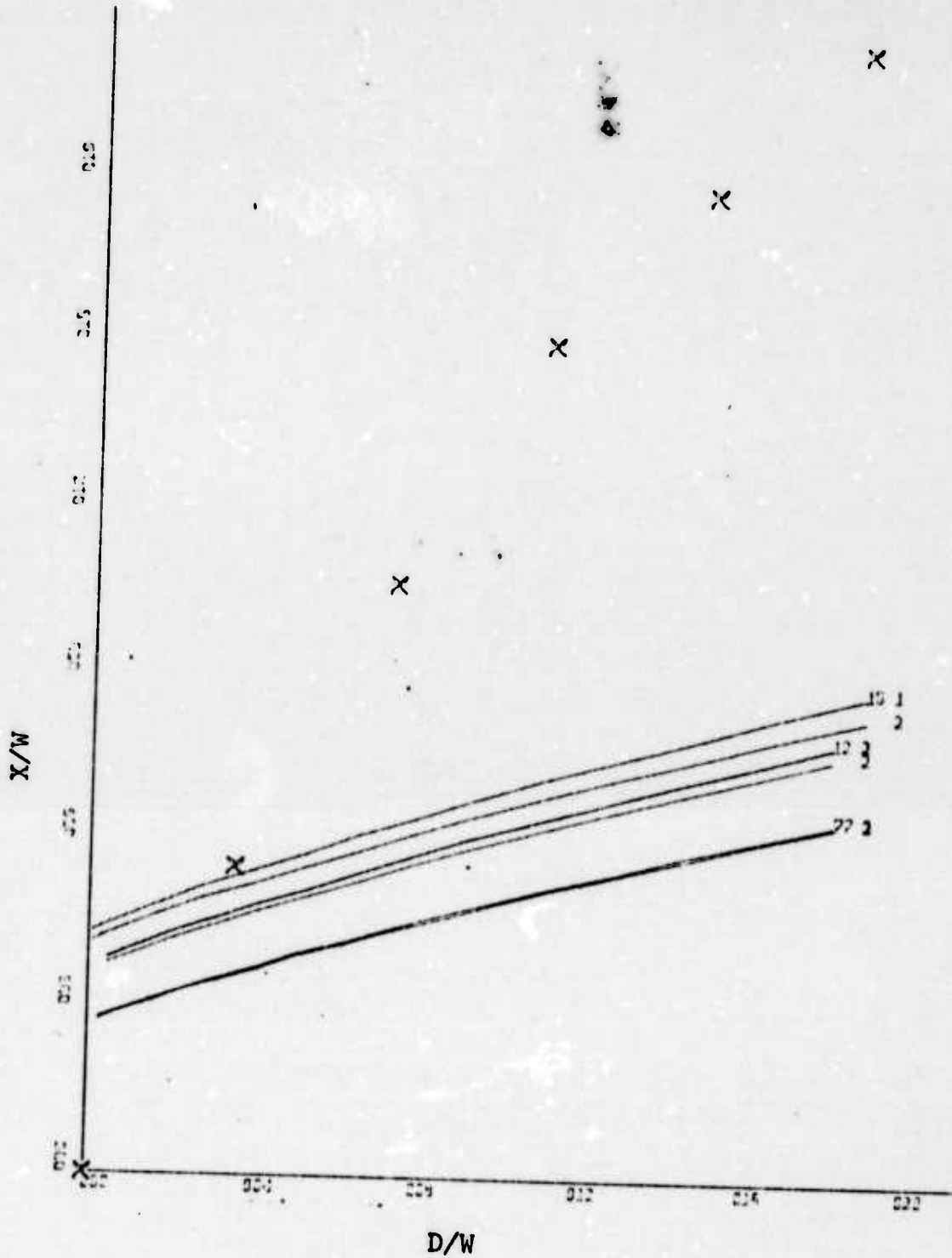
Figure 45. Attachment Distance vs. Offset Distance for a Concave Wall at 25 Degrees Incidence, Using Methods One(1) and Two(2) and Comparing With Experimental Data, Jet Width 1.31 Inches, Re = 1.475 \times 10^5 , \sigma = 7.7, 12, 15 .
