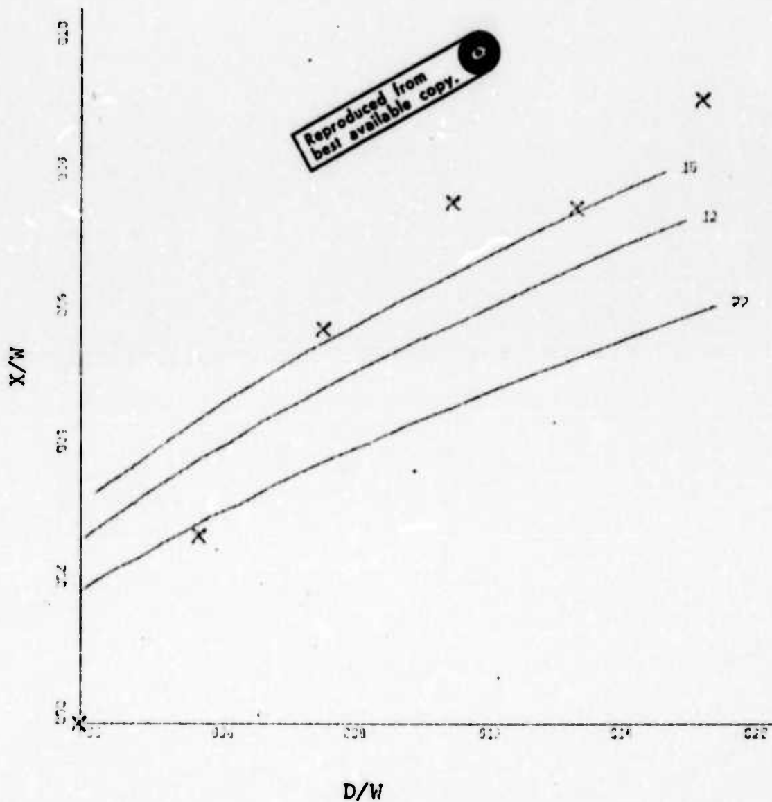
Figure 15. Attachment Distance vs. Offset Distance for a Planar Wall at 15 Degrees Incidence for Theoretical and Experimental Data, Jet Width 1.31 inches, Re = 147500 , \sigma = 7.7, 12, 15 .
