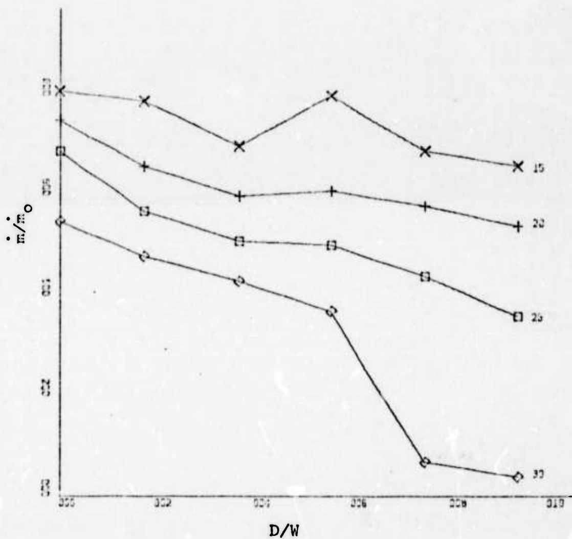
Figure 22. Flow Rate vs. Offset Distance for Planar Wall at Constant Deflection Angles, Jet Width of 2.62 inches, Re = 2.05 \times 10^5 , \alpha = 15, 20, 25, 30 Degrees
