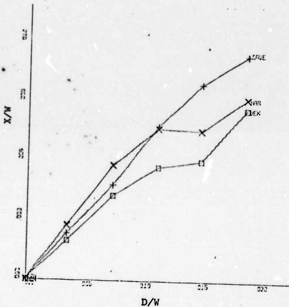
Figure 59. Attachment Distance vs. Offset Distance at 15 Degrees Wall Deflection for Planar, Concave, and Convex Walls, Jet Width 1.31 Inches, Re = 1.475 \times 10^5 .
