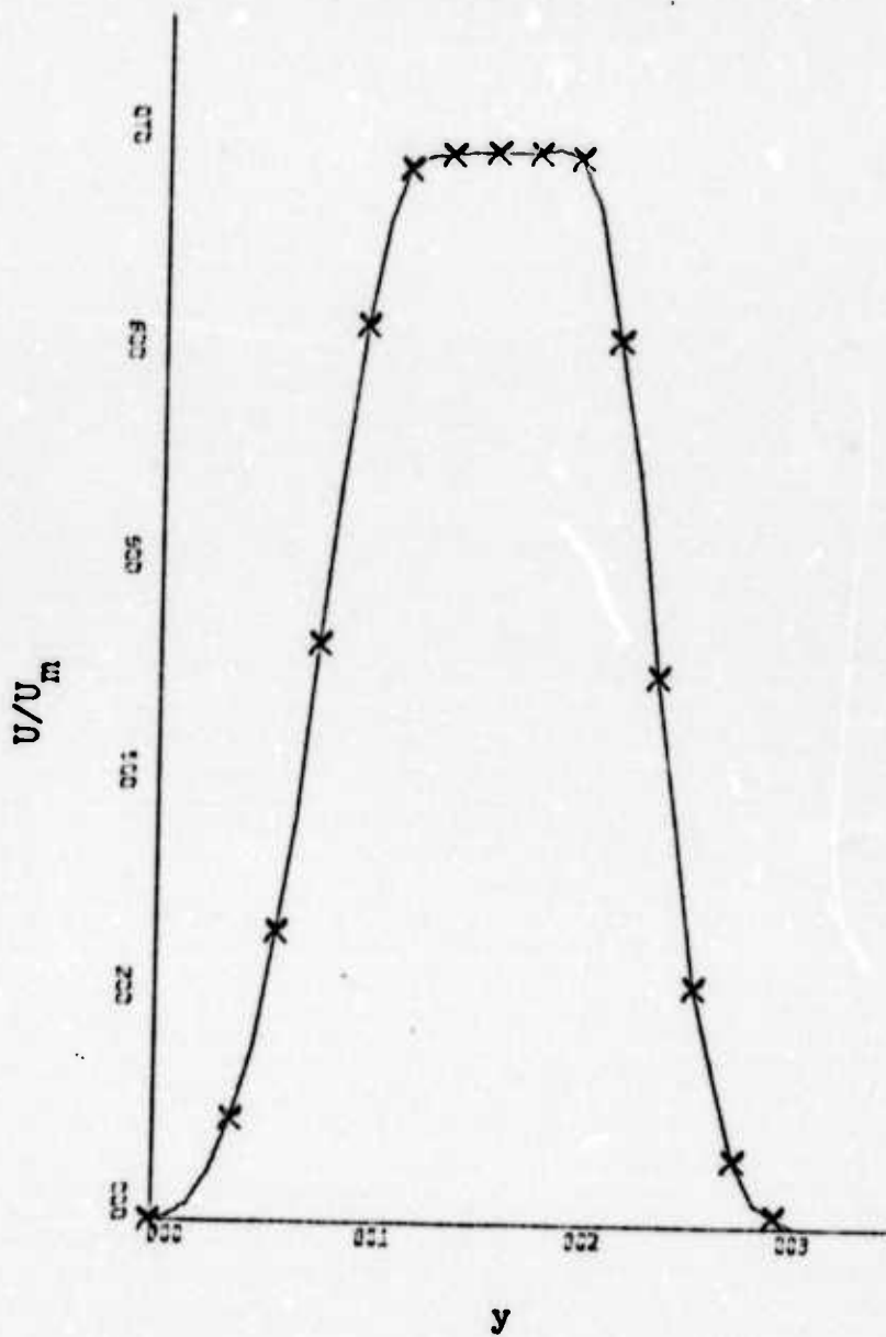
Figure 92. Velocity Profile at 5.24 Inches (4 Jet Widths) Downstream of Jet Exit for Jet Width of 1.31 Inches.
