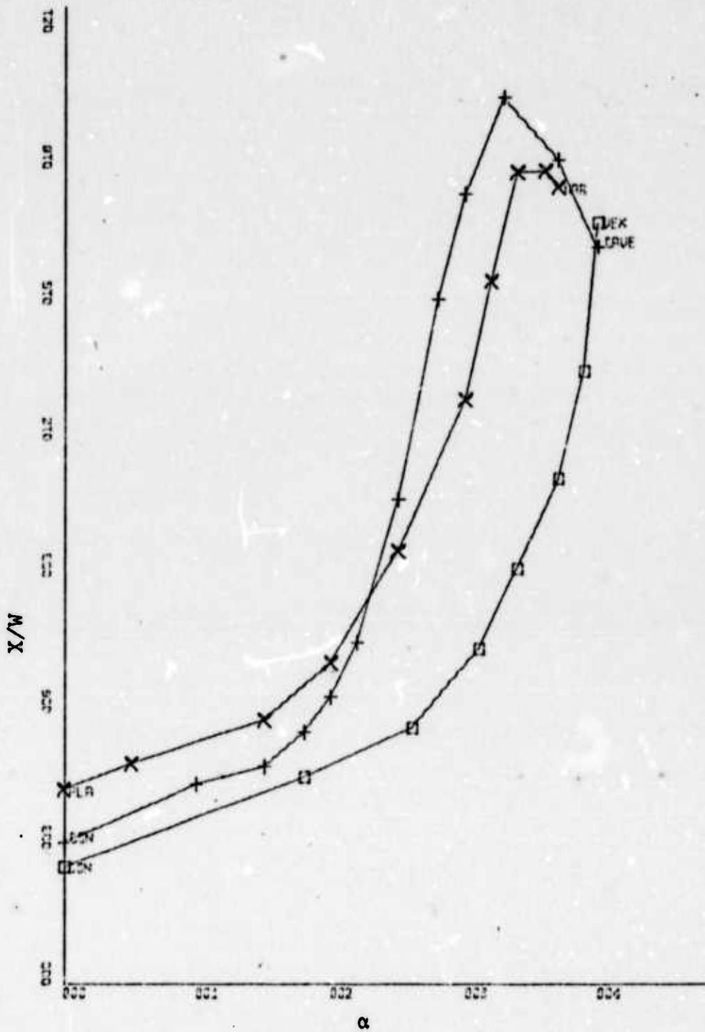
Figure 70. Attachment Distance vs. Deflection Angle for Jet Width of 1.31 Inches, Planar, Concave, and Convex Walls, Offset Distance ( D/W ) of 0.74, Re = 1.475 \times 10^5 .
