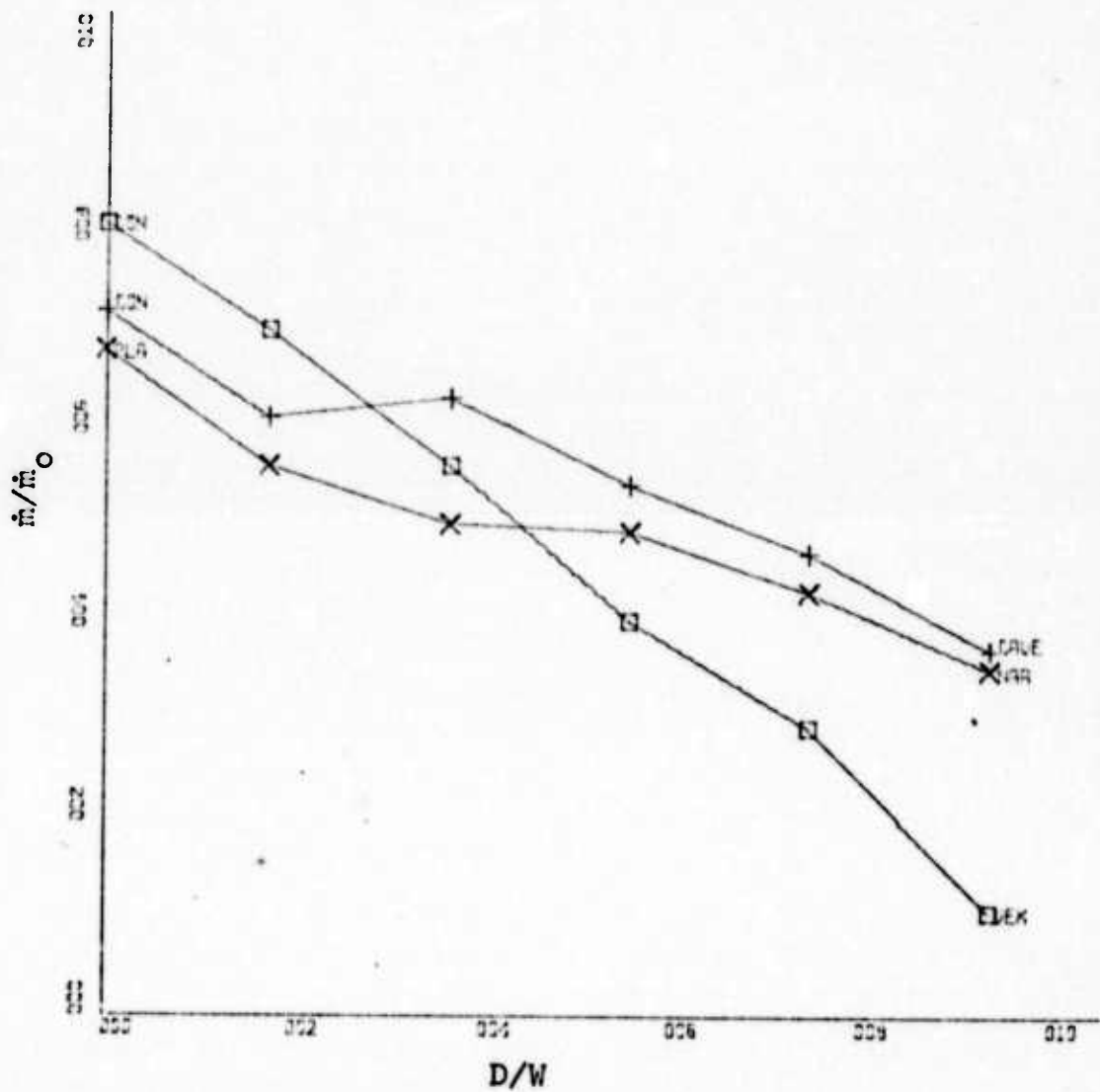
Figure 77. Flow Rate vs. Offset Distance for Planar, Concave, and Convex Walls, at 25 Degrees Deflection Angle, Jet Width of 2.62 Inches, Re = 2.05 \times 10^5 .
