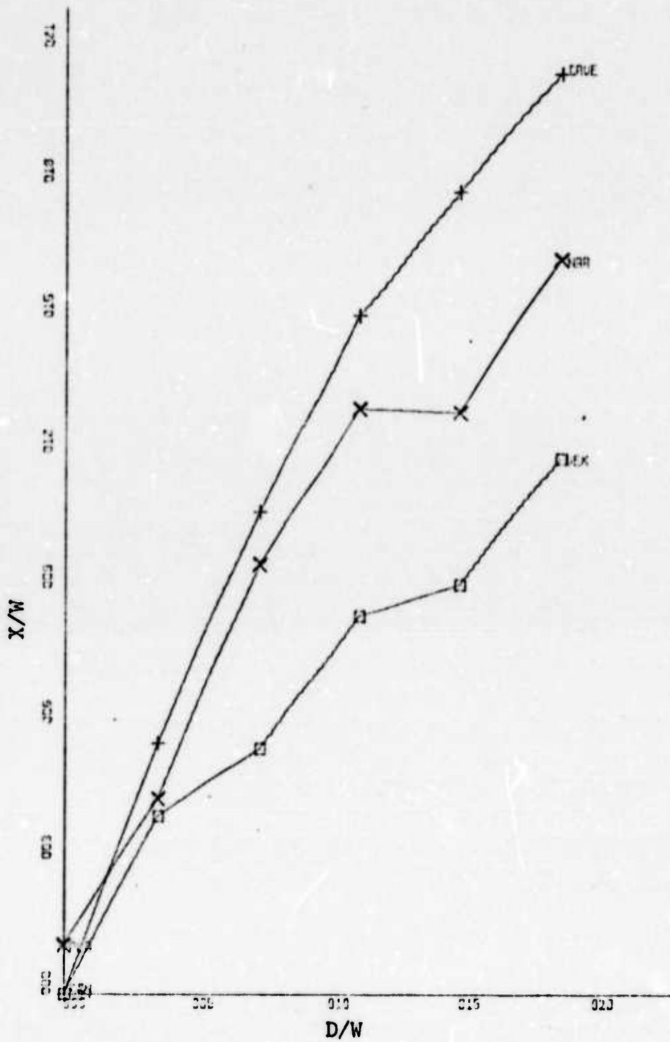
Figure 61. Attachment Distance vs. Offset Distance at 25 Degrees Wall Deflection for Planar, Concave, and Convex Walls, Jet Width of 1.31 Inches, Re = 1.475 \times 10^5 .
