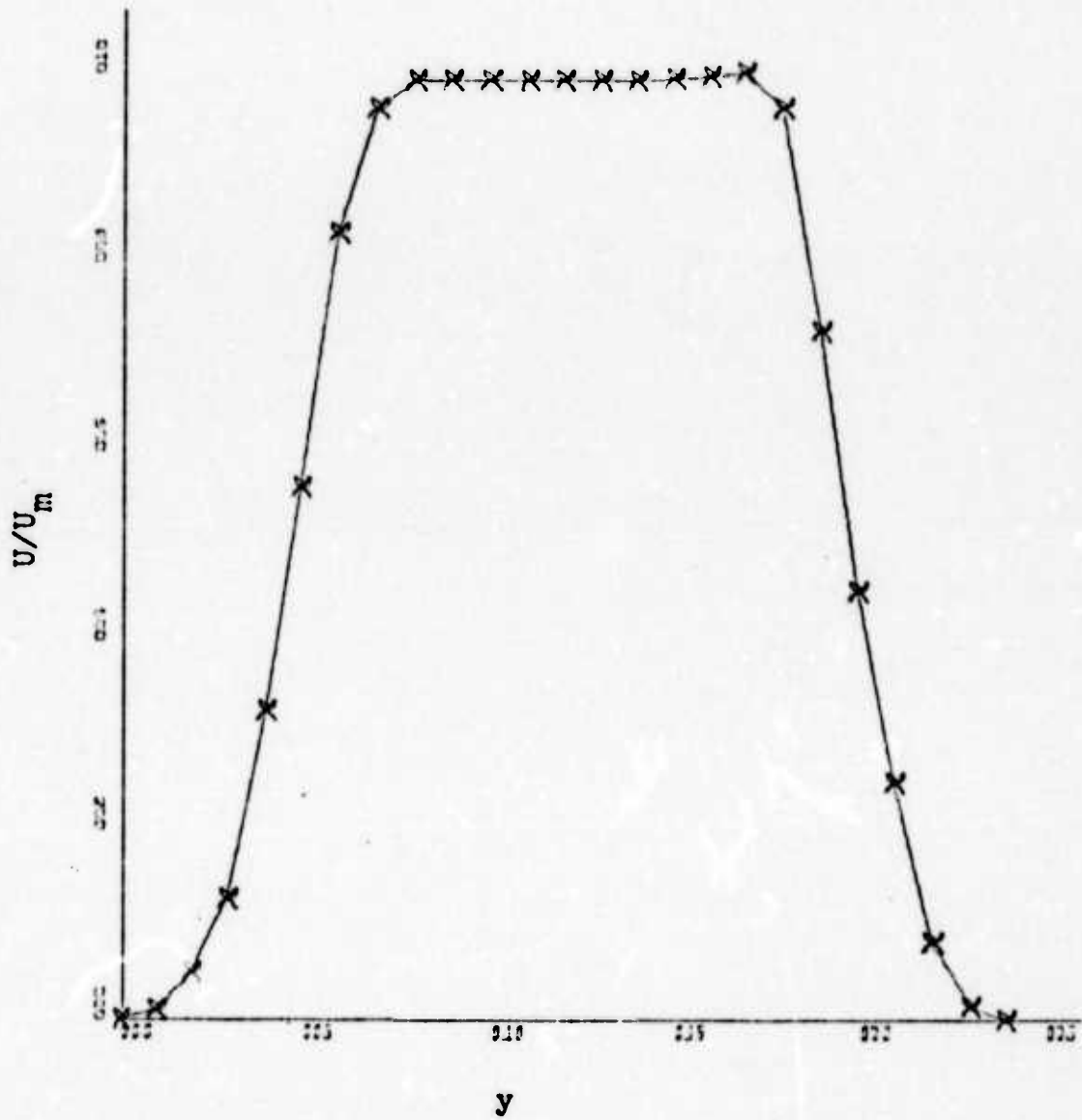
Figure 91. Velocity Profile at 2.62 Inches (2 Jet Widths) Downstream of Jet Exit for Jet Width of 1.31 Inches.
