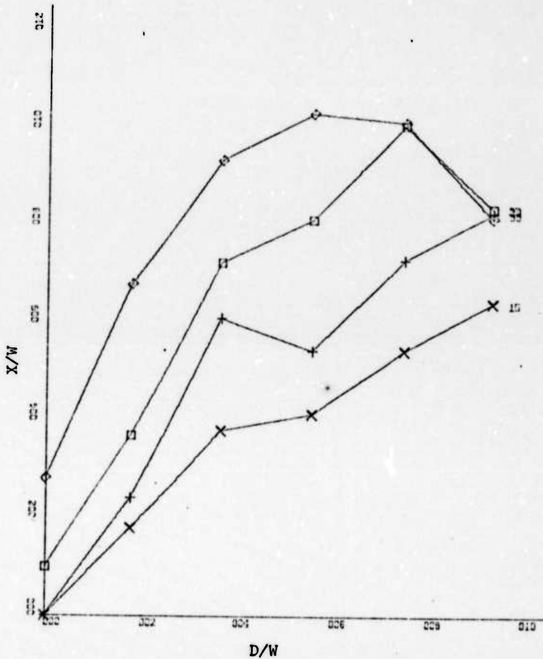
Figure 18. Attachment Distance vs. Offset Distance for Planar Wall, Re = 2.05 \times 10^5 , Constant Deflection Angles of 15, 20, 25, and 30 Degrees and Jet Width of 2.62 inches.
