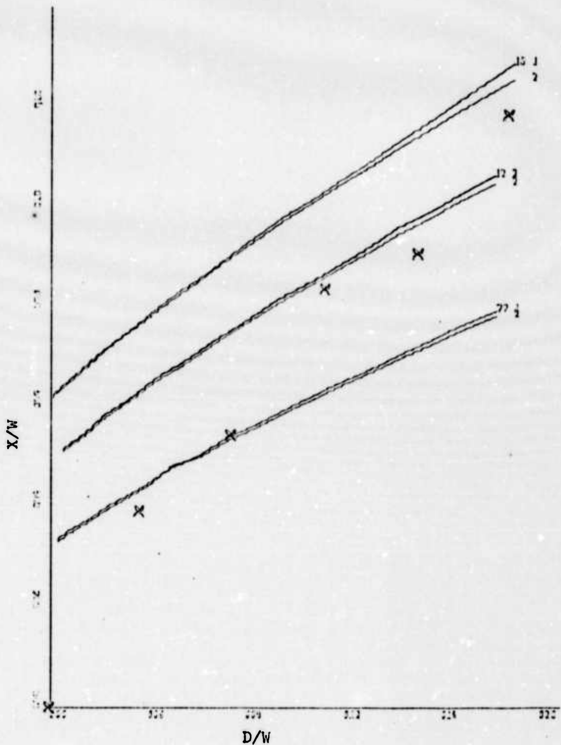
Figure 31. Attachment Distance vs. Offset Distance for a Convex Wall, at 25 Degrees Incidence using Methods One(1) and Two(2), and Comparing with Experimental data, Jet Width 1.31, Re = 1.475 \times 10^5 , \sigma = 7.7, 12, 15 .
