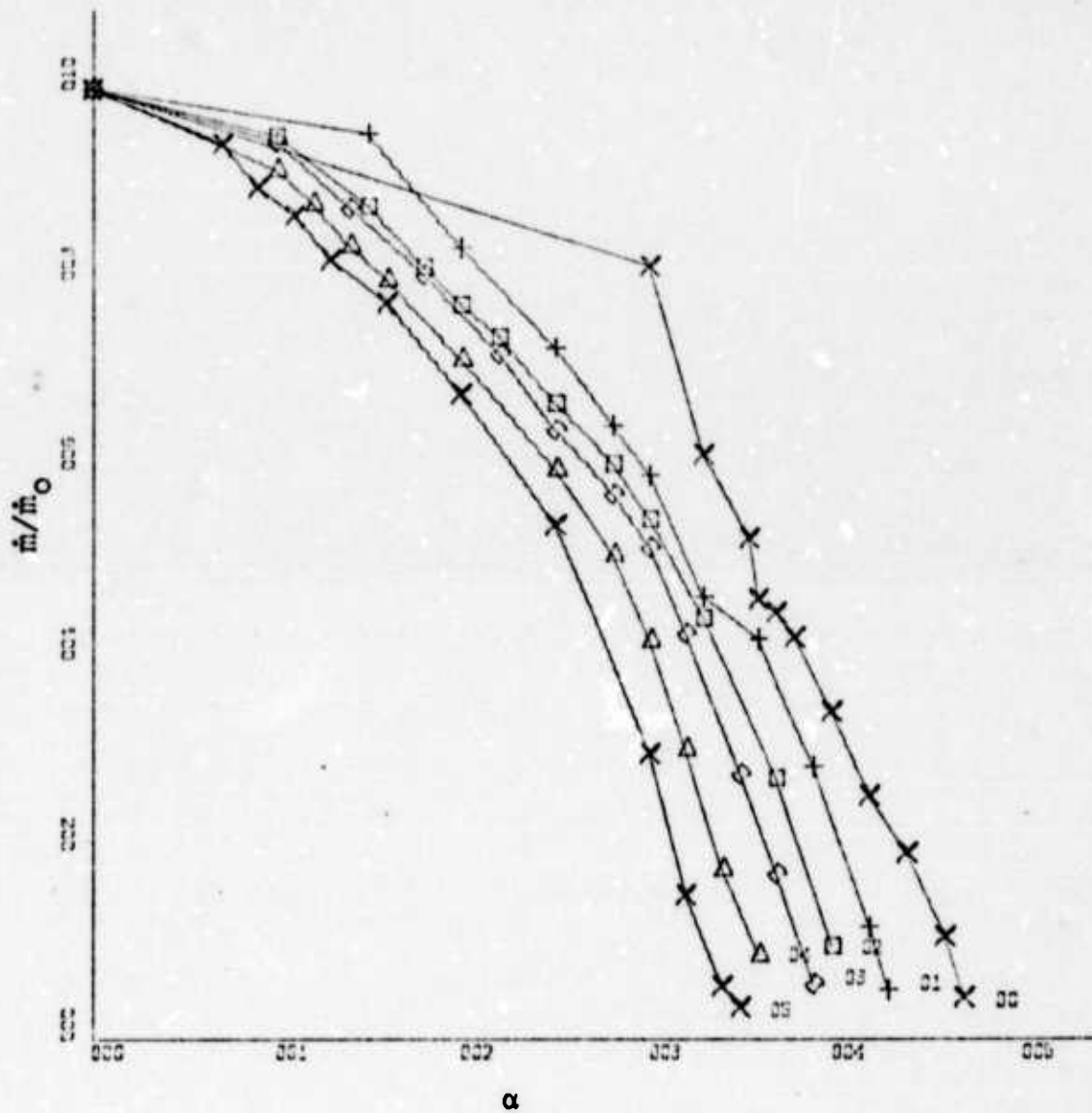
Figure 53. Flow Rate vs. Deflection Angle at Various Offset Distances for Concave Wall Re = 1.475 \times 10^3 , Jet Width of 1.31 Inches, D/W of 00, 01, 02, 03, 04, 05.
