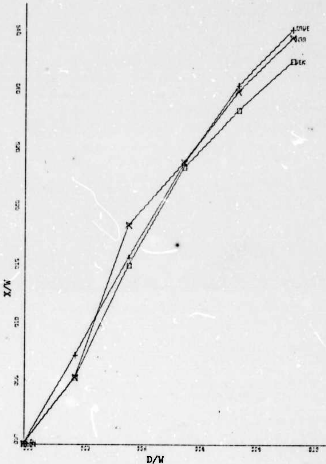
Figure 54. Attachment Distance vs. Offset Distance at 0 Degrees Deflection for Planar, Concave, and Convex Walls. Jet Width 2.62 Inches. Re = 2.05 \times 10^5 .
