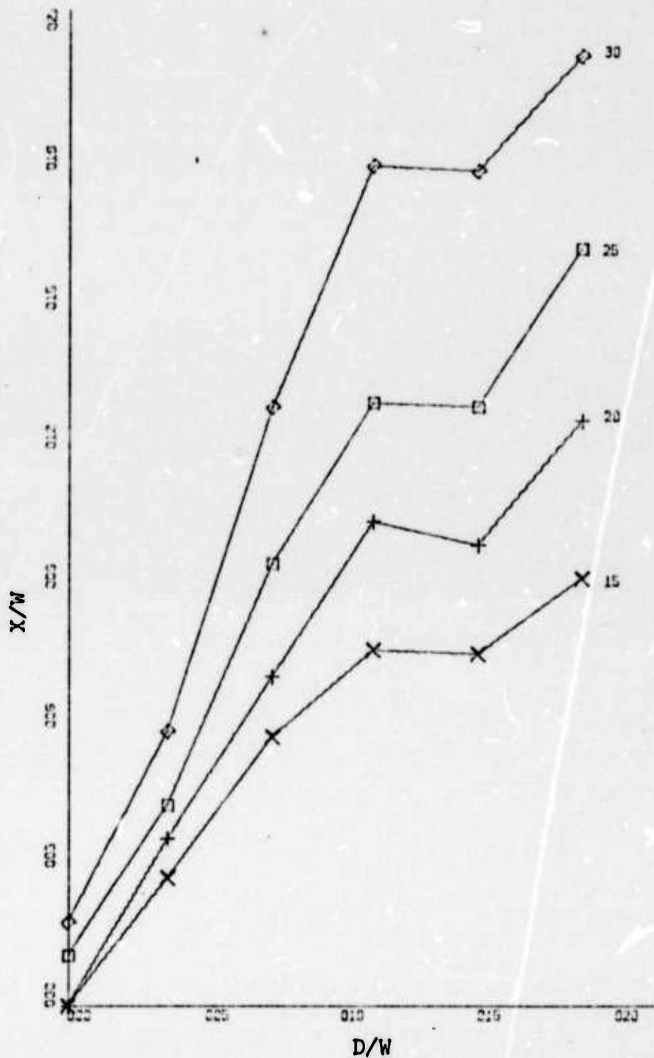
Figure 19. Attachment Distance vs. Offset Distance for Planar Wall, Re = 1.475 \times 10^5 Constant Deflection Angles of 15, 20, 25, 30 and Jet Width of 1.31 Inches.
