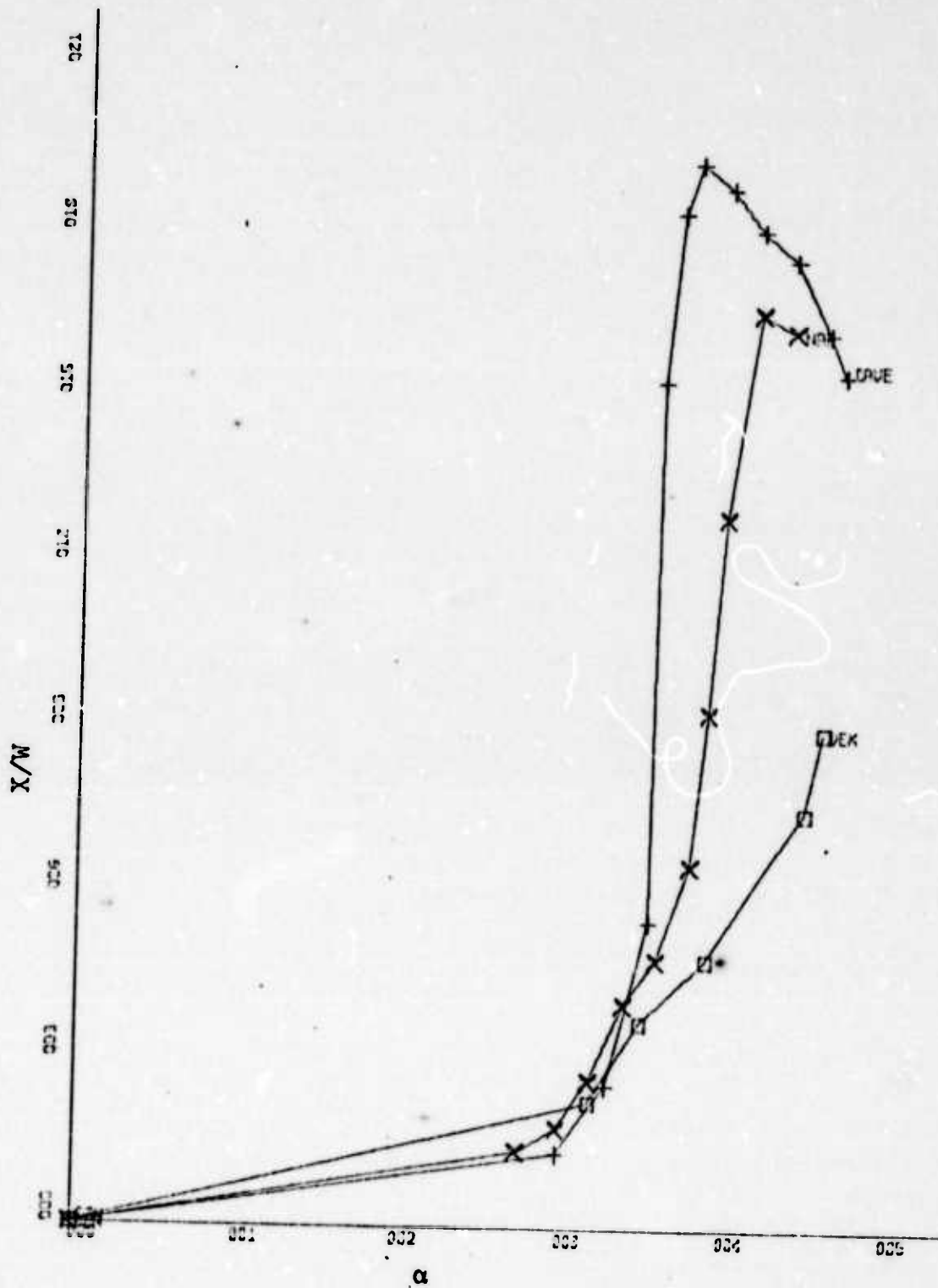
Figure 68. Attachment Distance vs. Deflection Angle for Jet Width of 1.31 Inches for Planar, Concave, and Convex Walls at Offset Distance ( D/W ) of 0.0, Re = 1.475 \times 10^5 .
