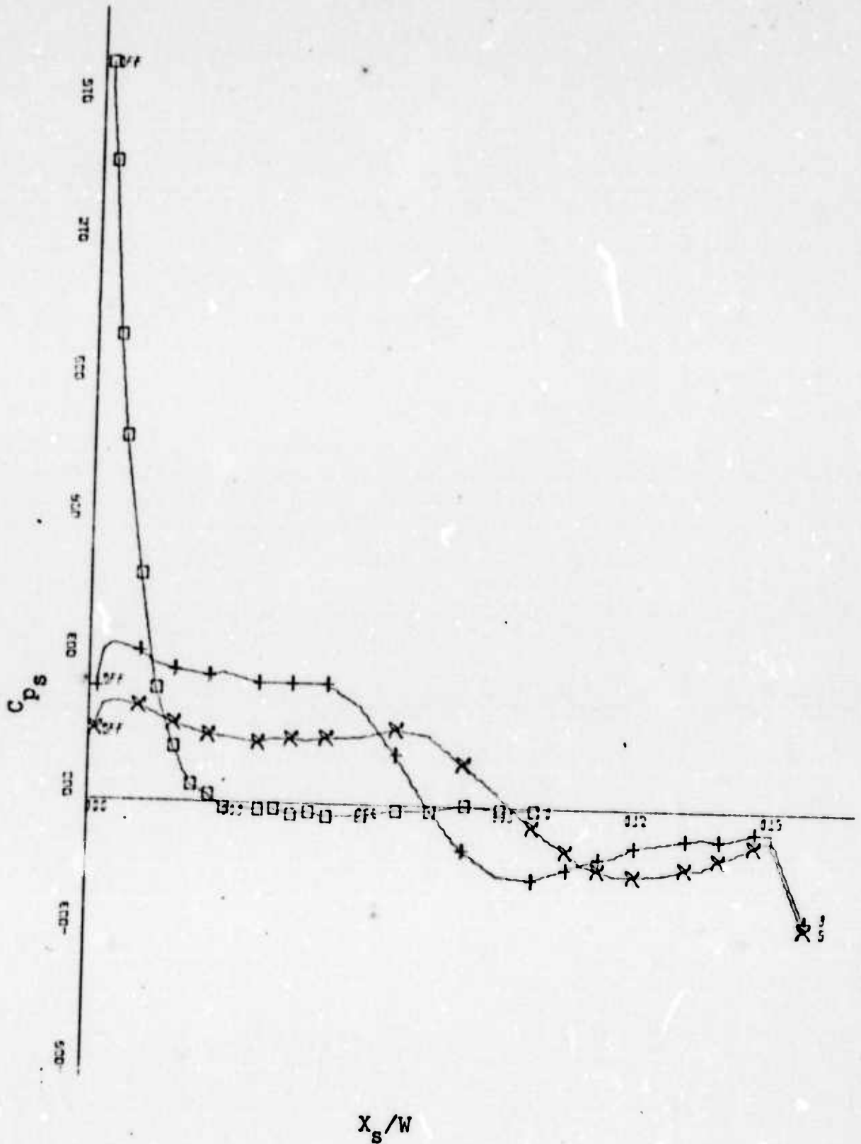
Figure 82. Surface Pressure Coefficient vs. Wall Position for Planar Wall at 15 Degrees Deflection Angle, for Various Offset Distances, Re = 2.05 \times 10^5 , Jet Width of 2.62 Inches.
