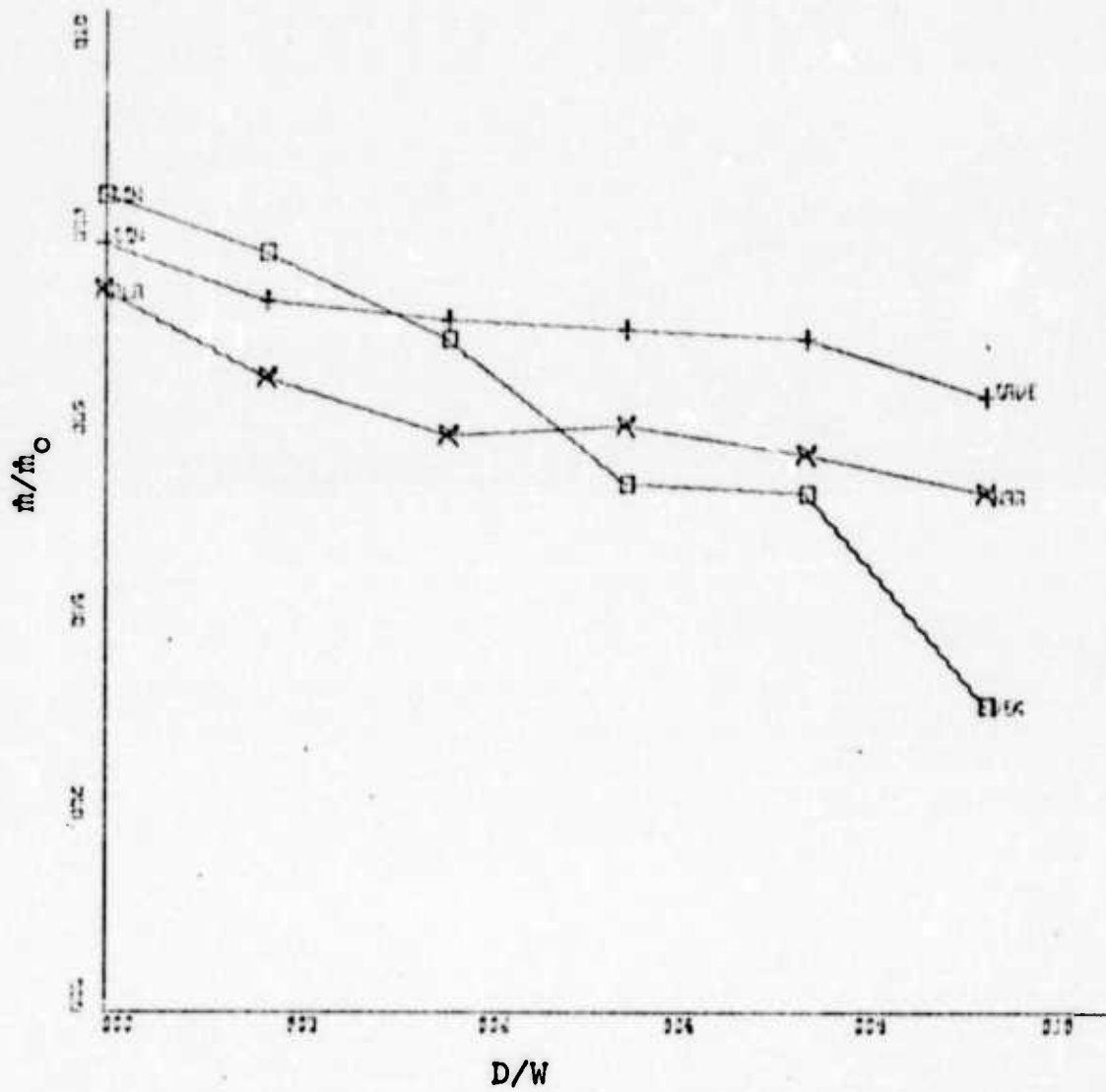
Figure 76. Flow Rate vs. Offset Distance for Planar, Concave, and Convex Walls, at 20 Degrees Deflection Angle, Jet Width of 2.62 Inches, Re = 2.05 \times 10^5 .
