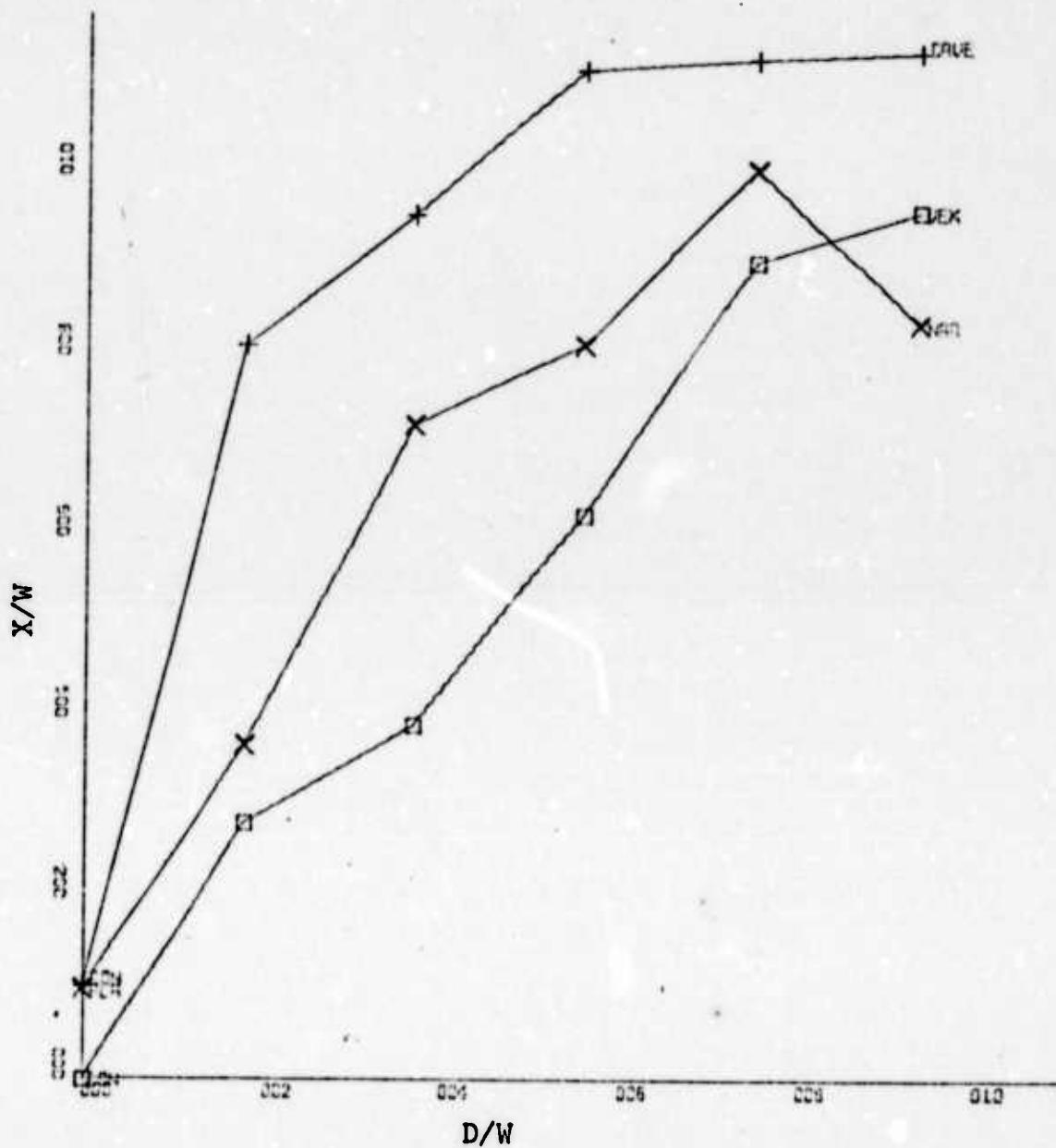
Figure 57. Attachment Distance vs. Offset at 25 Degrees Wall Deflection for Planar, Concave, and Convex Wall, Jet Width of 2.62 Inches, Re = 2.05 \times 10^5 .
