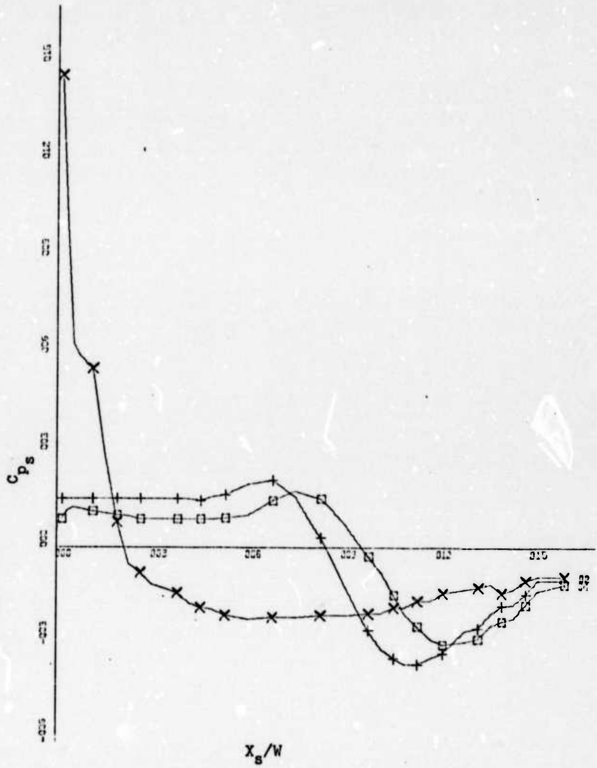
Figure 84. Surface Pressure Coefficient vs. Wall Position for Concave Wall at 25 Degrees Deflection Angle, for Various Offset Distances, Re = 2.05 \times 10^5 , Jet Width of 2.62 Inches.
