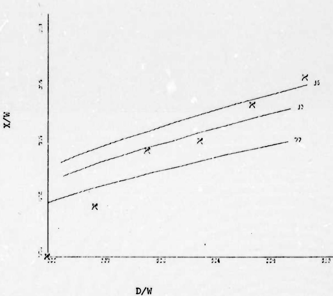
Figure 12. Attachment Distance vs. Offset Distance for Planar Wall at 15 Degrees Incidence for Theoretical and Experimental Data, Jet width 2.62 inches, Re = 2.05 \times 10^5 , \sigma = 7.7, 12, 15 .
