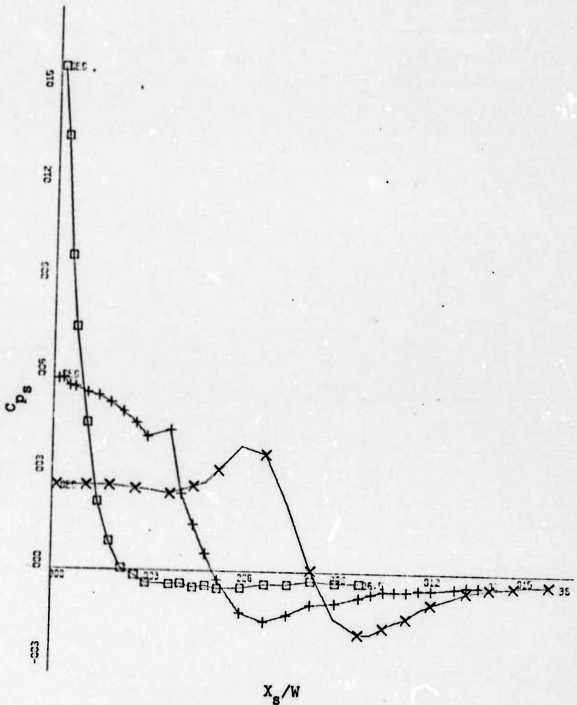
Figure 85. Surface Pressure Coefficient vs. Wall Position for Planar Wall at Various Deflection Angles and Offset Distance ( D/W ) of 0.0, Jet Width of 2.62 Inches, Re = 2.05 \times 10^5 , \alpha = 26.5, 32, 38 Degrees.
