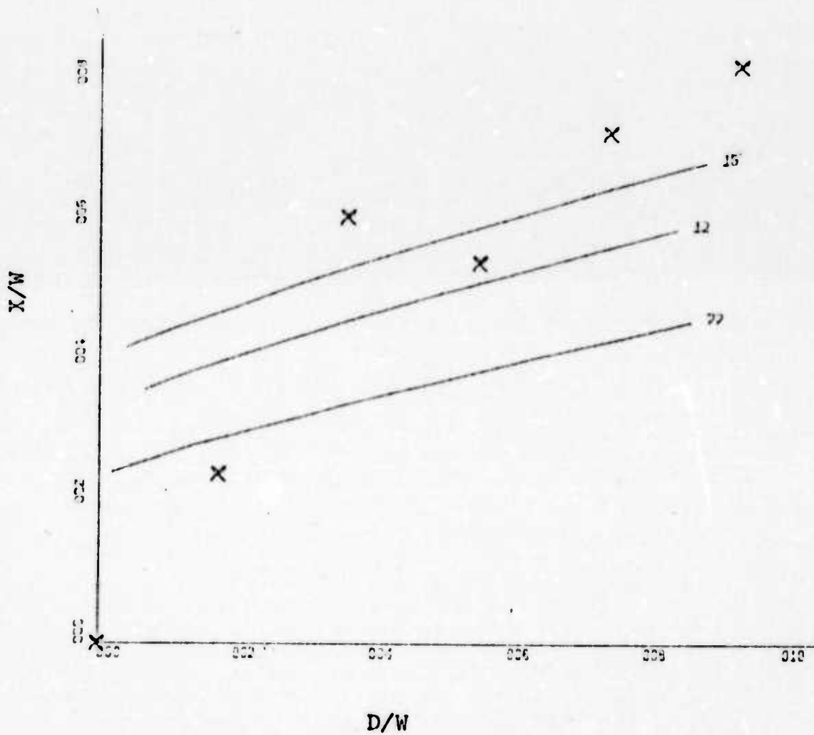
Figure 13. Attachment Distance vs. Offset Distance for Planar Wall at 20 Degrees Incidence for Theoretical and Experimental Data, Jet Width 2.62 inches, Re = 20.5 \times 10^5 , \sigma = 7.7, 12, 15 .
