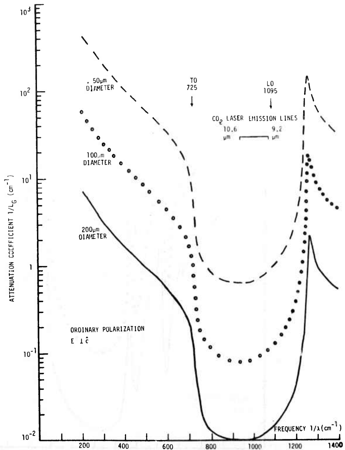
Figure 6. Frequency Dependence of the Attenuation Coefficient for the TE_{01} Mode of a BeO Capillary Waveguide
