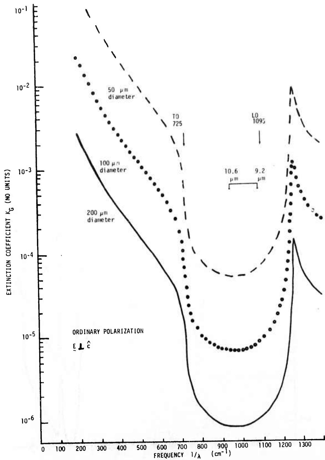
Figure 3. Frequency Dependence of the Extinction Coefficient for the TE_{01} Circular Mode of a BeO Capillary Waveguide
