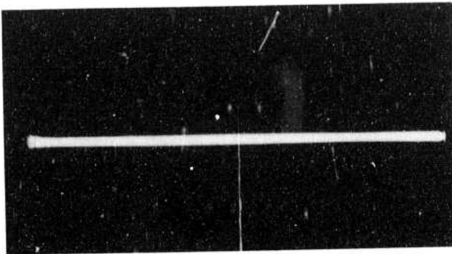
Figure 22. Continuous longitudinal \text{CO}_2:\text{N}_2:\text{He} discharge in planar structure, pressure 10-300 Torr 1:1:2, d=1\text{mm} longitudinal flow - discharge 15cm long, \sim 4\text{mm} wide
