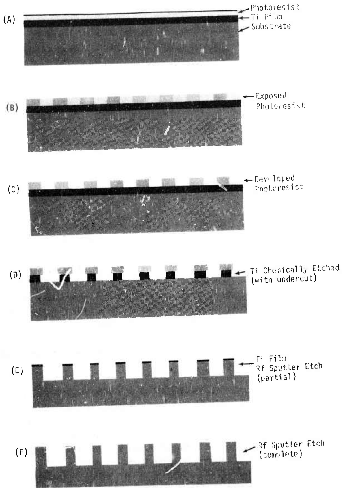
Figure 11. Processing Sequence for Deep Patterns (Diffraction Grating)
