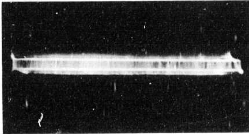
Figure 16. Plan view of \text{CO}_2:\text{He} plasma discharge using strip cathode and anode at bottom of channels - waveguide thickness 175 \mu , photographic exposure 1/2 sec (full scale)
