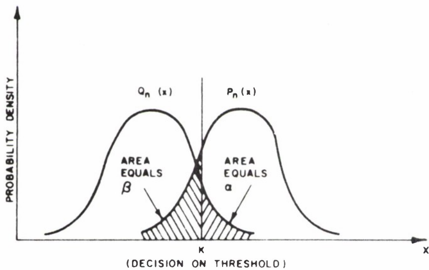
Figure 1-4. System Probability Density With Decision Regions
