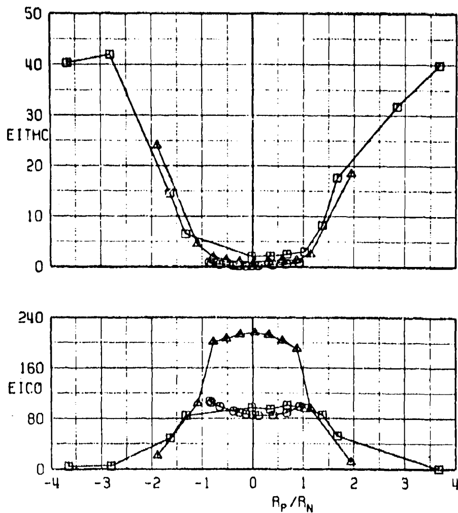
e. EITHC and EICO versus R_p/R_N Fig. 14 Continued
