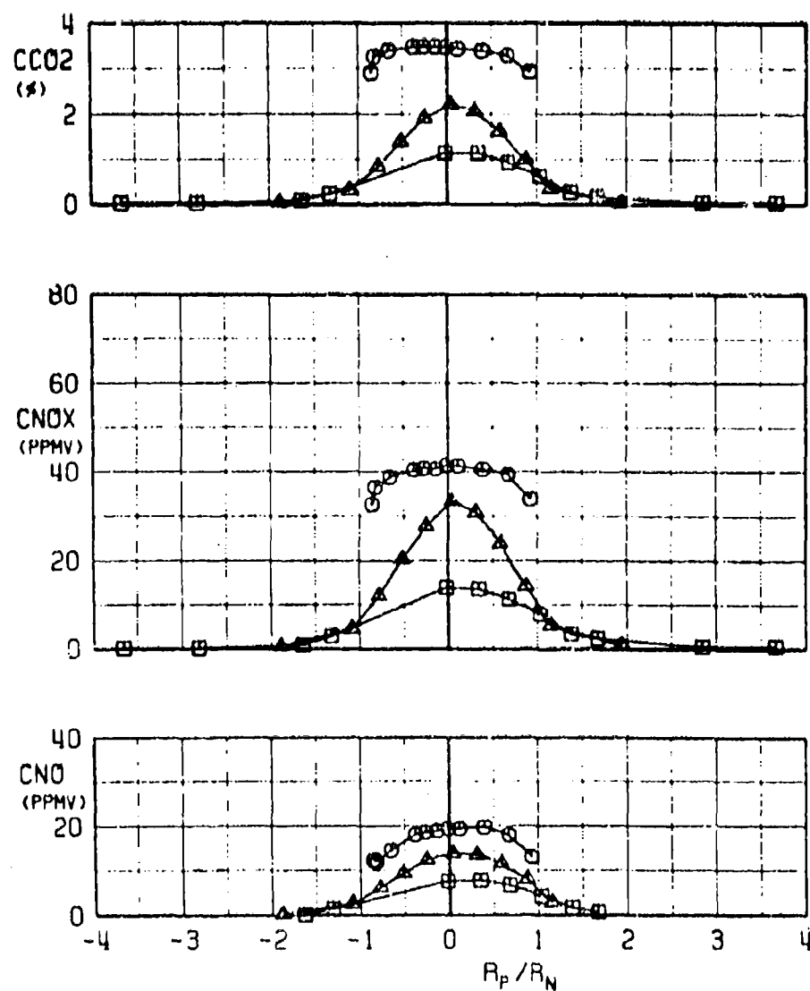
c. CCO 2 , CNO x , and CNO versus R_p/R_N Fig. 14 Continued
