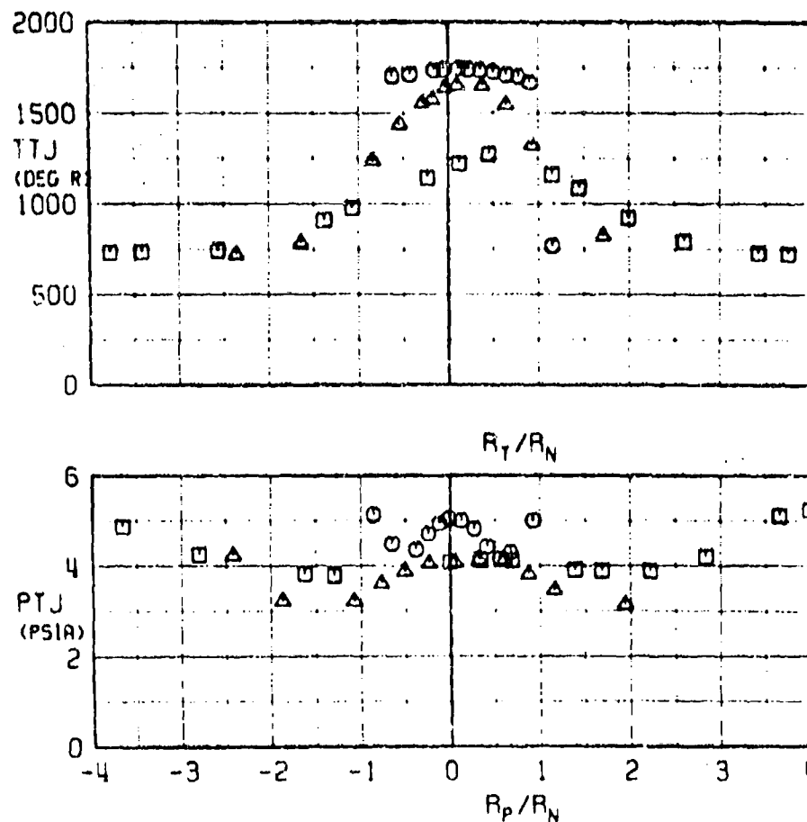
a. TTJ versus R_T/R_N , PTJ versus R_P/R_N Fig. 15 Variation of Emission Characteristics with Axial Probe Position (Mach 2.0/65,000 ft, MIL)
