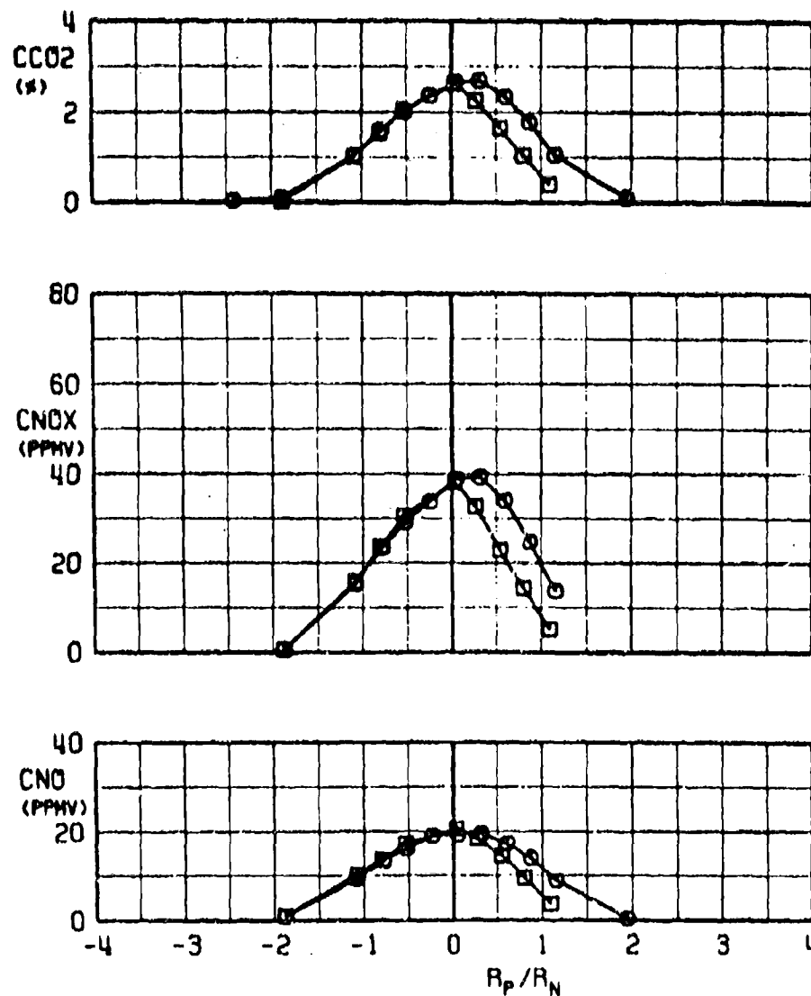
c. CO_2 , CNO_x , and CNO versus R_p/R_N Fig. 21 Continued
