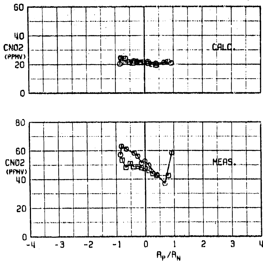
d. Calculated and Measured CNO_2 versus R_p/R_N Fig. 19 Concluded
