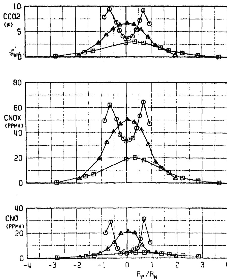
c. CCO_2 , CNO_x , and CNO versus R_P/R_N
