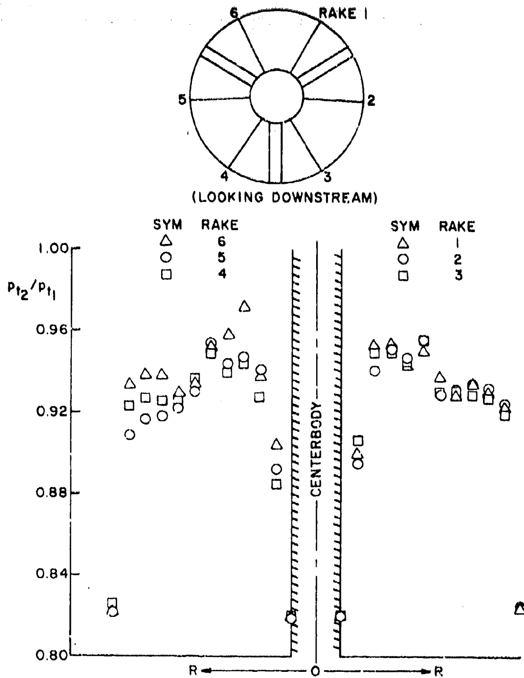
a. M_\infty = 1.6/55,000 ft Fig. 13 Typical Pressure Profiles at Compressor Inlet
