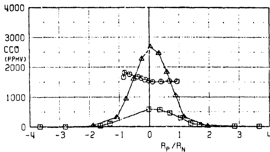
b. CTHC and CCO versus R_P/R_N Fig. 14 Continued
