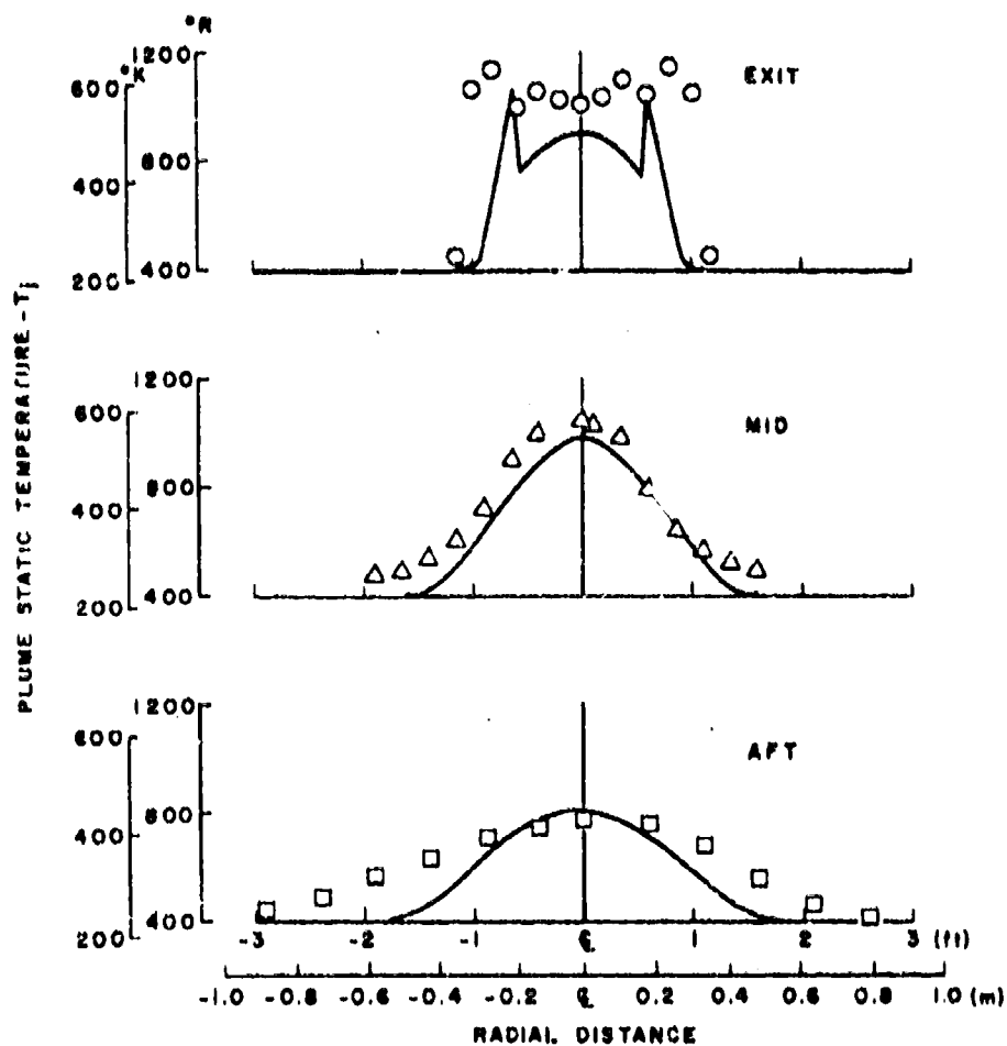
g. Plume Static Temperature Fig. 24 Continued
