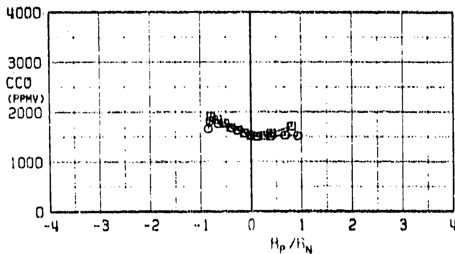
b. CTHC and CCO versus R_p/R_N Fig. 10 Continued
