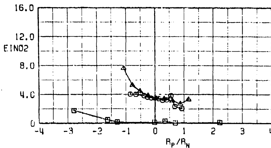
g. EINO 2 versus R_p/R_N Fig. 15 Concluded
