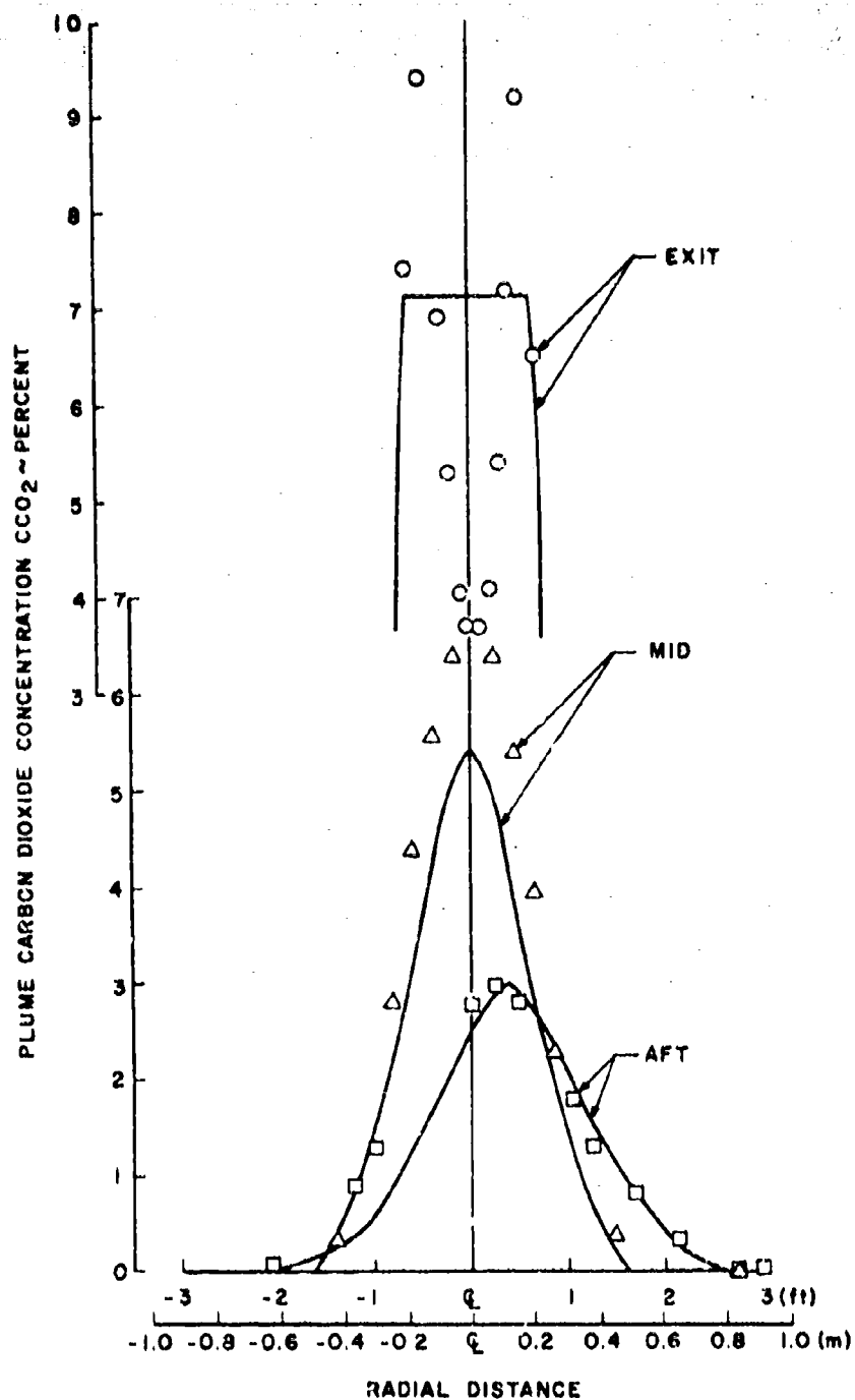
c. Plume Carbon Dioxide Concentration Fig. 27 Concluded
