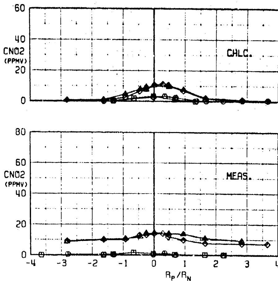
d. Calculated and Measured CNO 2 versus R_p/R_N Fig. 22 Concluded
