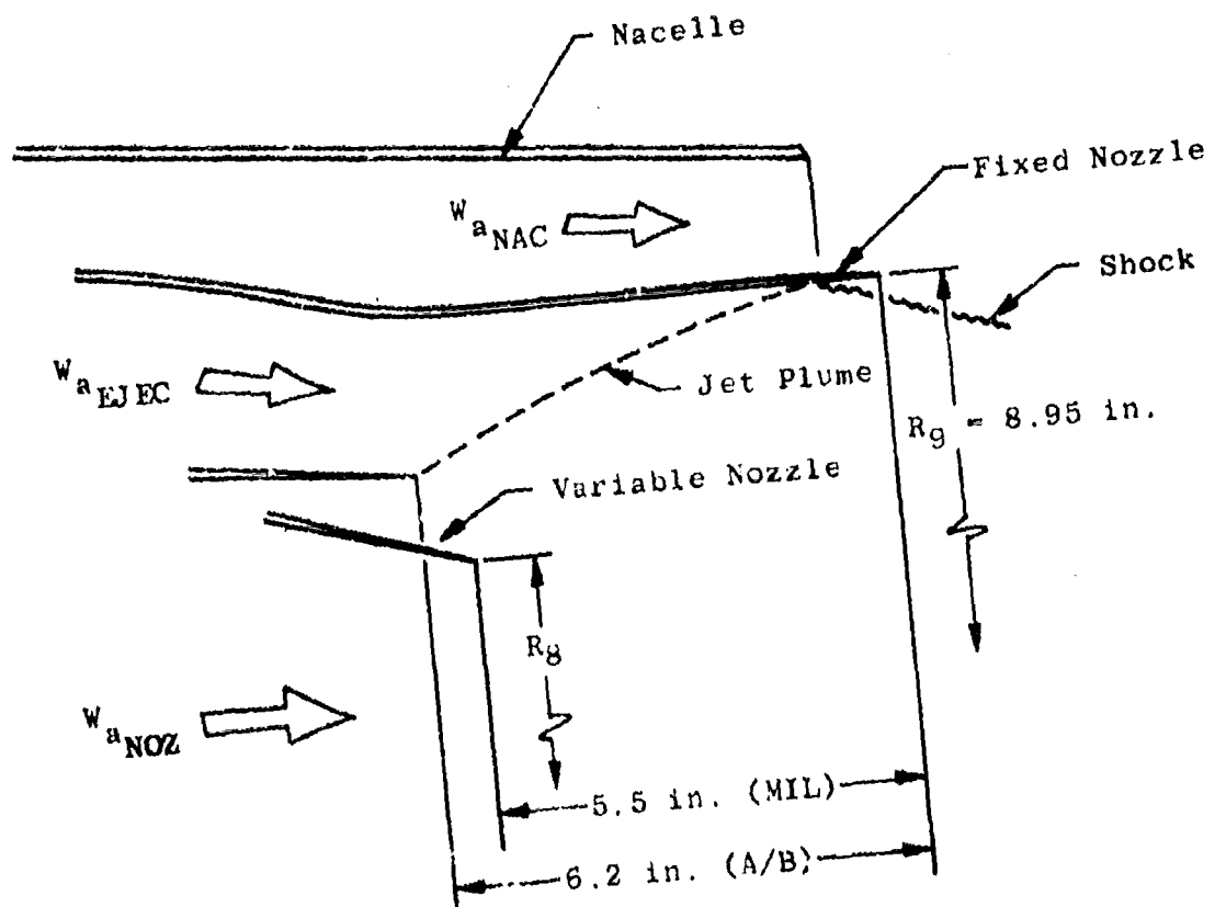
Fig. 4 J85-GE-5 Ejector Nozzle Shroud Schematic
