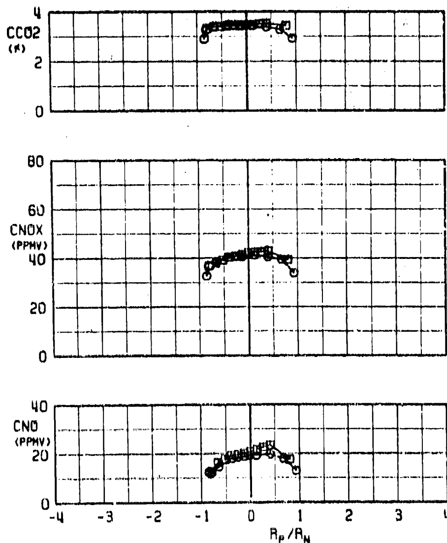
o. CCO_2 , CNO_x , and CNO versus R_p/R_N Fig. 10 Continued
