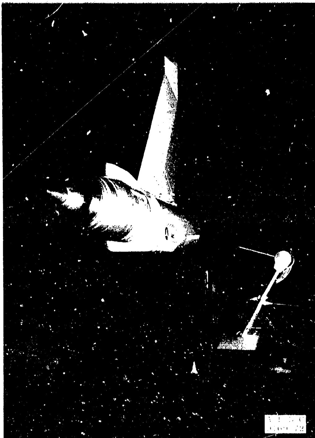
Fig. 2 Installation Photograph with Sample Probe at Position 2 (Mid Position)
