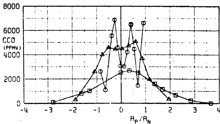
b. CTHC and CCO versus R_P/R_N Fig. 17 Continued
