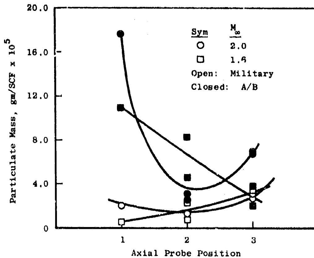
Fig. 30 Results of Gravimetric Filter Measurement of Particulate Emissions for Conditions Tested
