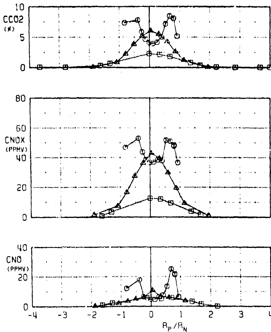
c. CCO_2 , CNO_x , and CNO versus R_p/R_N Fig. 16 Continued
