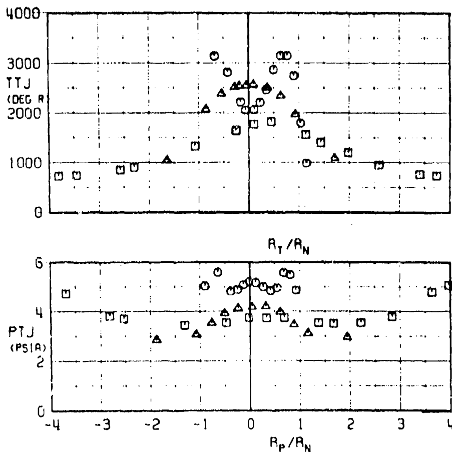
Fig. 17 Variation of Emission Characteristics with Axial Probe Position (Mach 2.0/65,000 ft, A/B)
