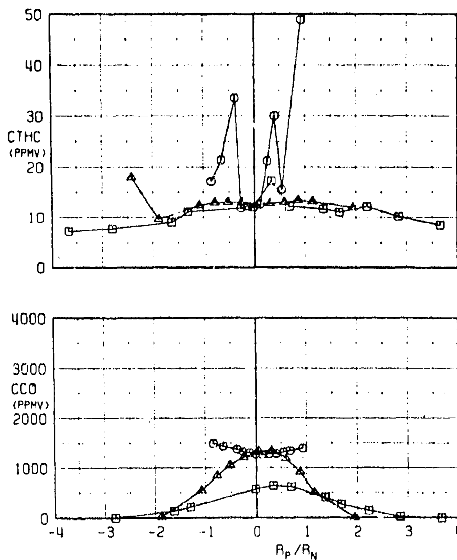
b. CTHC and CCO versus R_P/R_N Fig. 15 Continued
