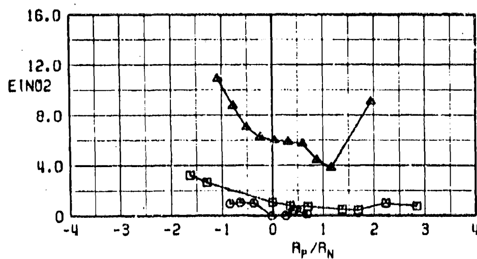
g. EINO 2 versus R_p/R_N Fig. 17 Concluded
