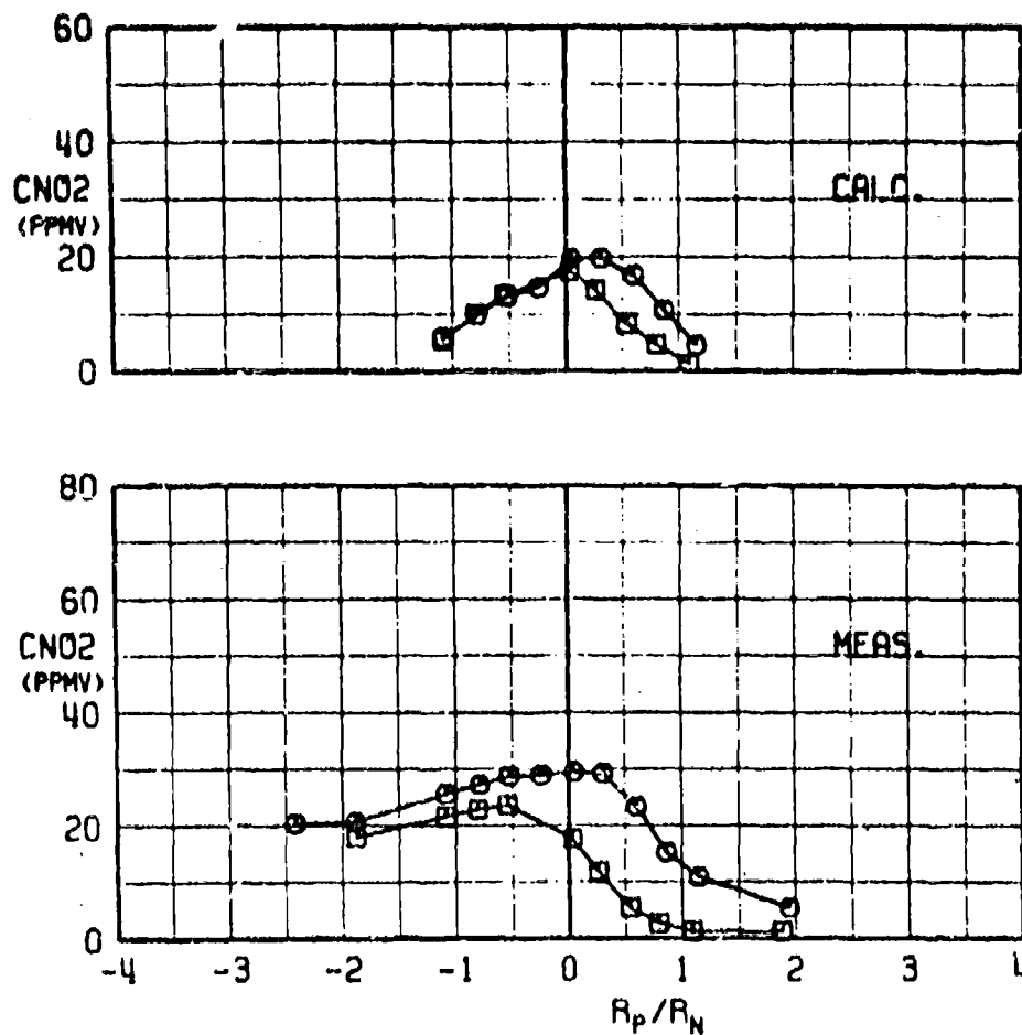
d. Calculated and Measured CNO 2 versus R_p/R_N Fig. 21 Concluded
