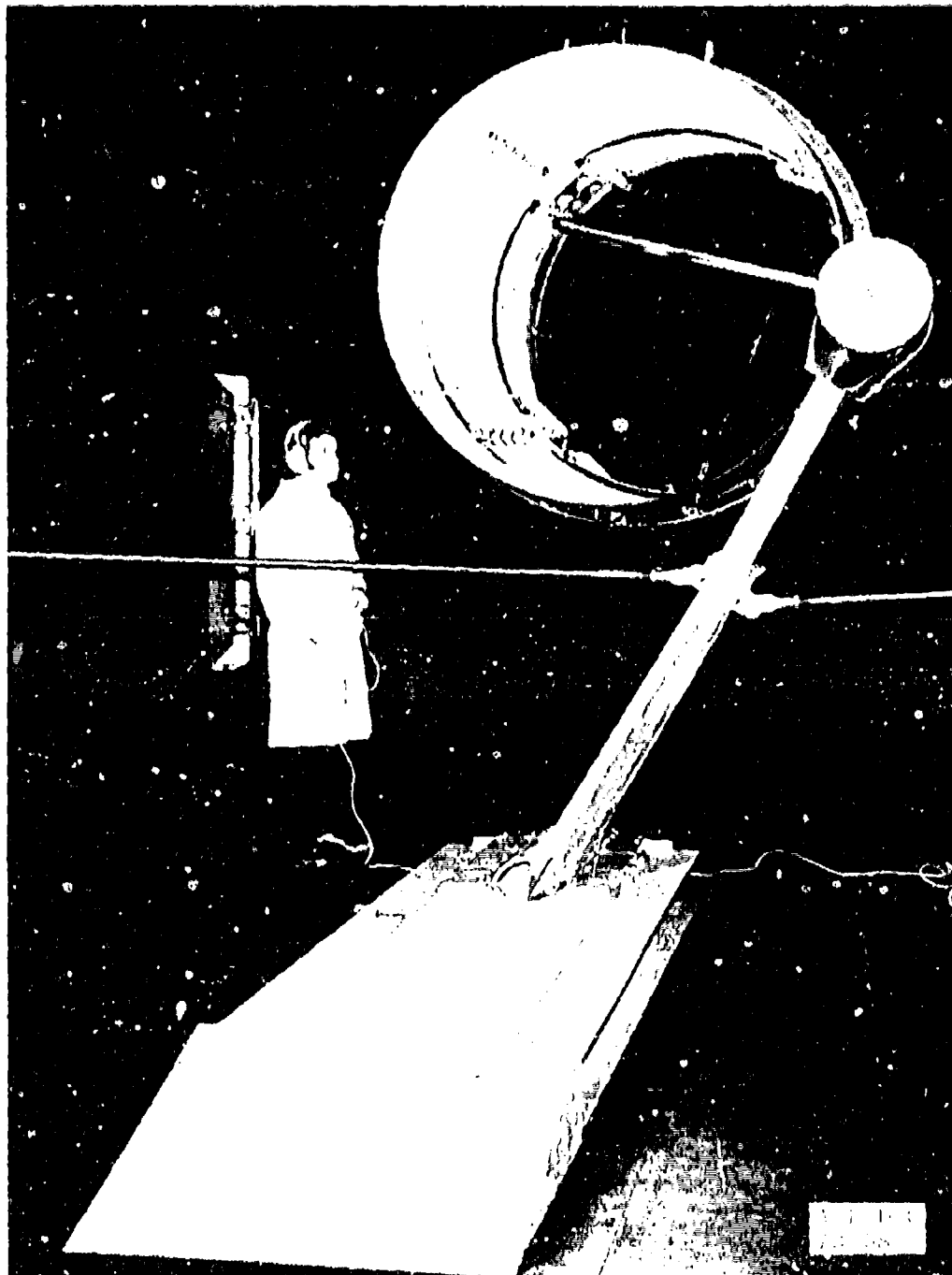
a. Axial Probe Position 3 (XP/DN = 19.9), Aft Station Fig. 6 Sample Probe Installation
