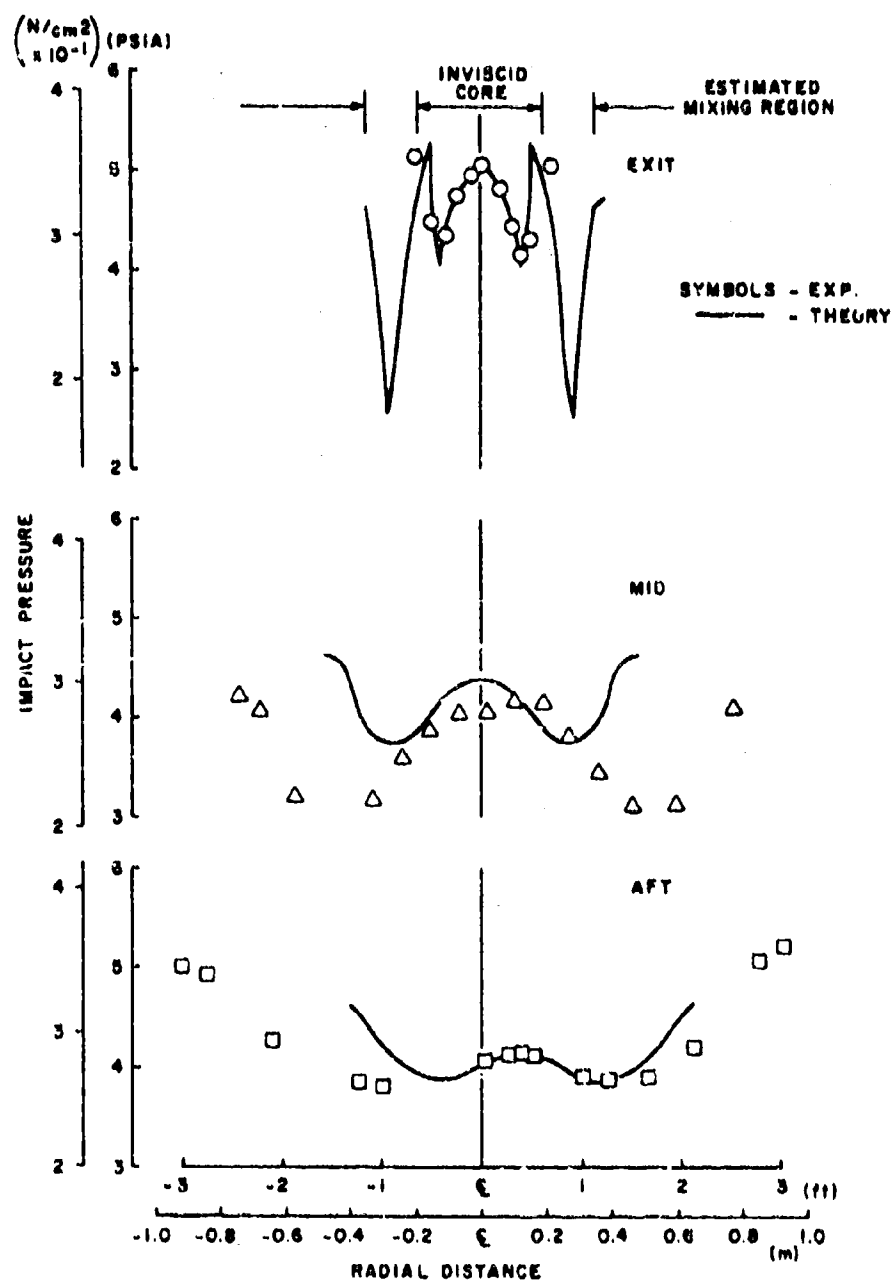
a. Plume Impact Pressure
