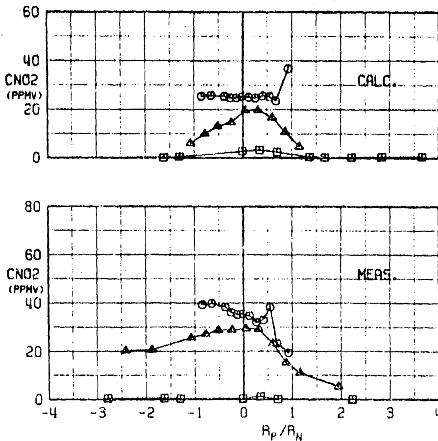
d. Calculated and Measured CNO 2 versus R_p/R_N Fig. 15 Continued
