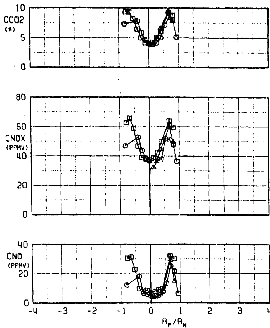
c. CCO_2 , CNO_x , and CNO versus R_P/R_N Fig. 20 Continued
