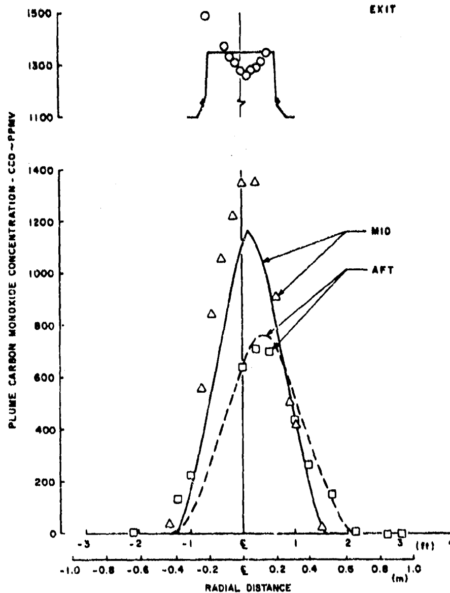
d. Plume Carbon Monoxide Concentration Fig. 24 Continued
