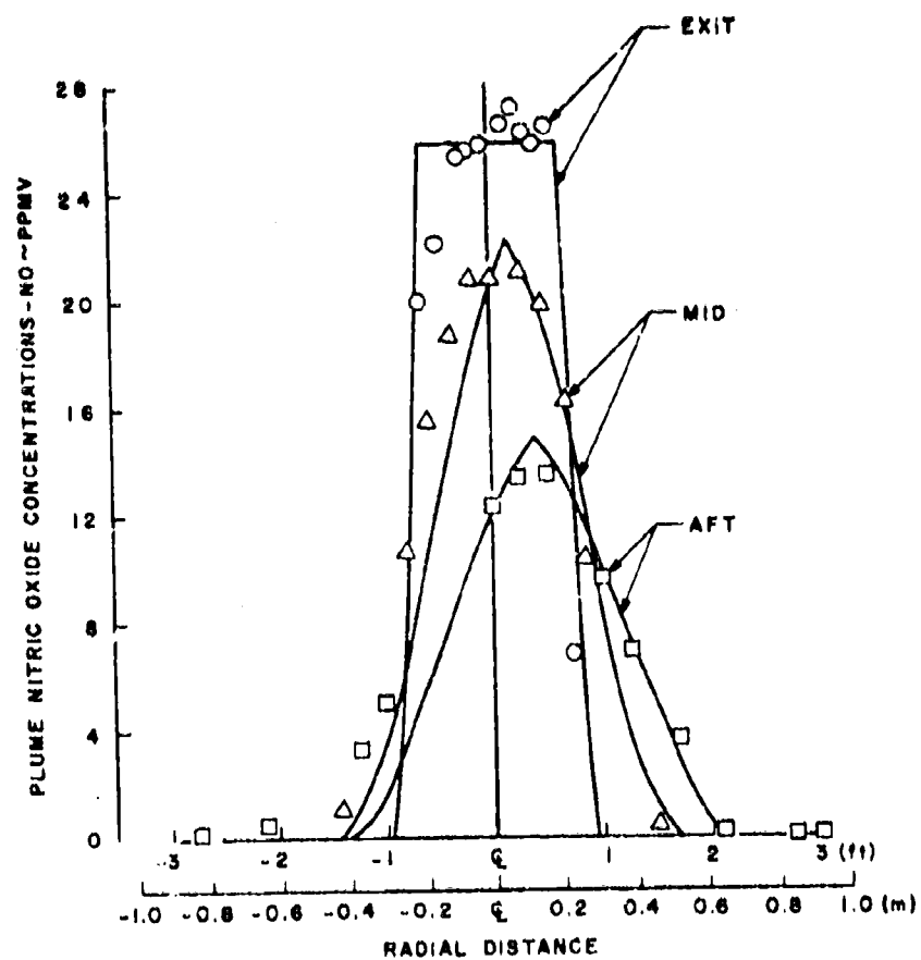
e. Plume Nitric Oxide Concentrations Fig. 24 Continued
