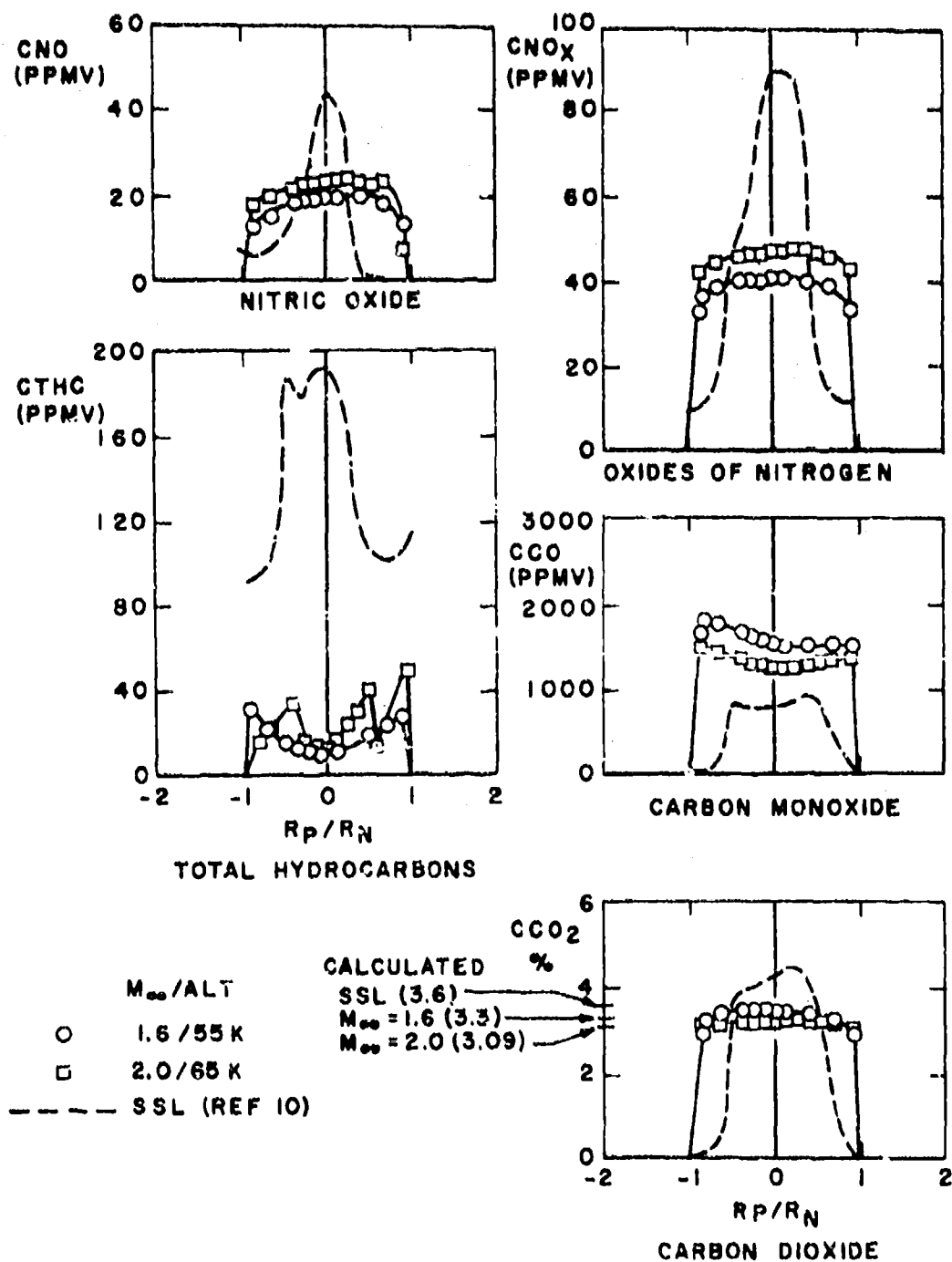
Fig. 23 Comparison of Exit Plane Profile for the Gaseous Emissions of the J85 Turbojet Engine
