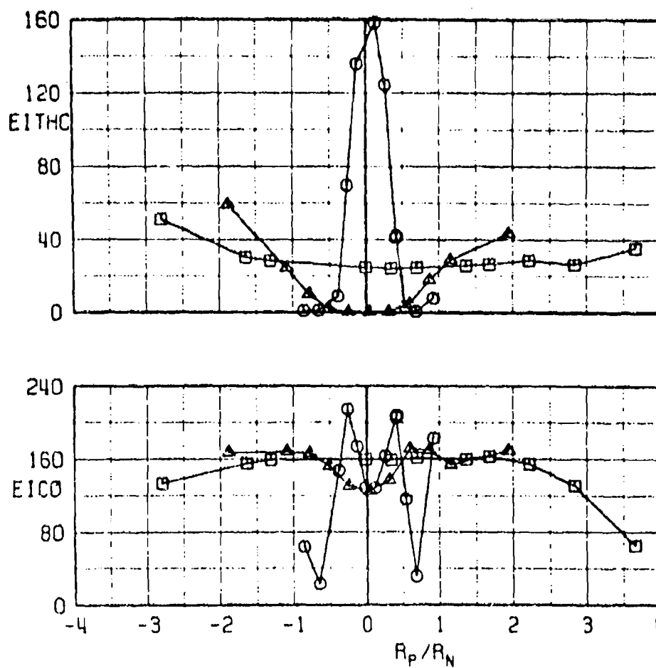
e. EITHC and EICO versus R_P/R_N Fig. 17 Continued
