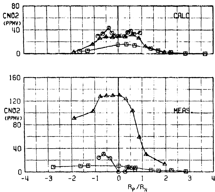
d. Calculated and Measured CNO 2 versus R_p/R_N Fig. 17 Continued
