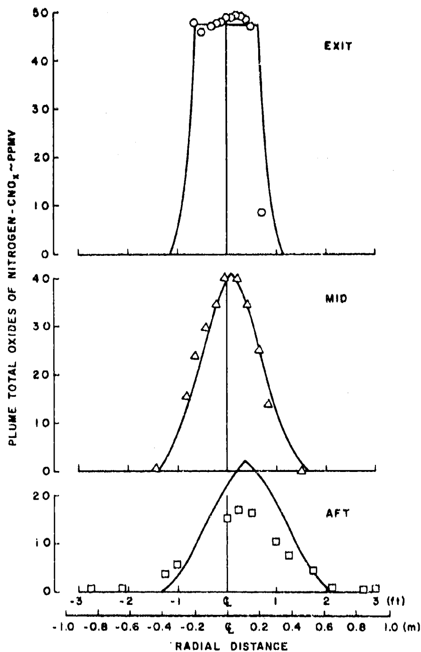
f. Plume Total Oxides of Nitrogen Concentration Fig. 24 Continued
