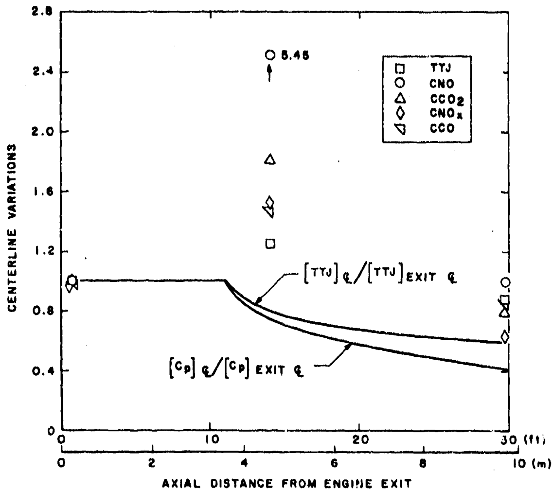
Fig. 28 Centerline Decay Characteristics of the Emission Concentrations and Total Temperature in the Exhaust Plume at Mach 2.0/65,000 ft, Afterburning Power
