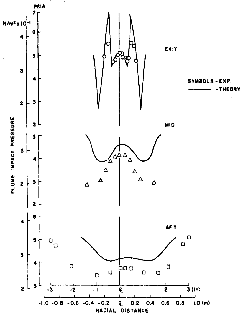
a. Plume Impact Pressure
