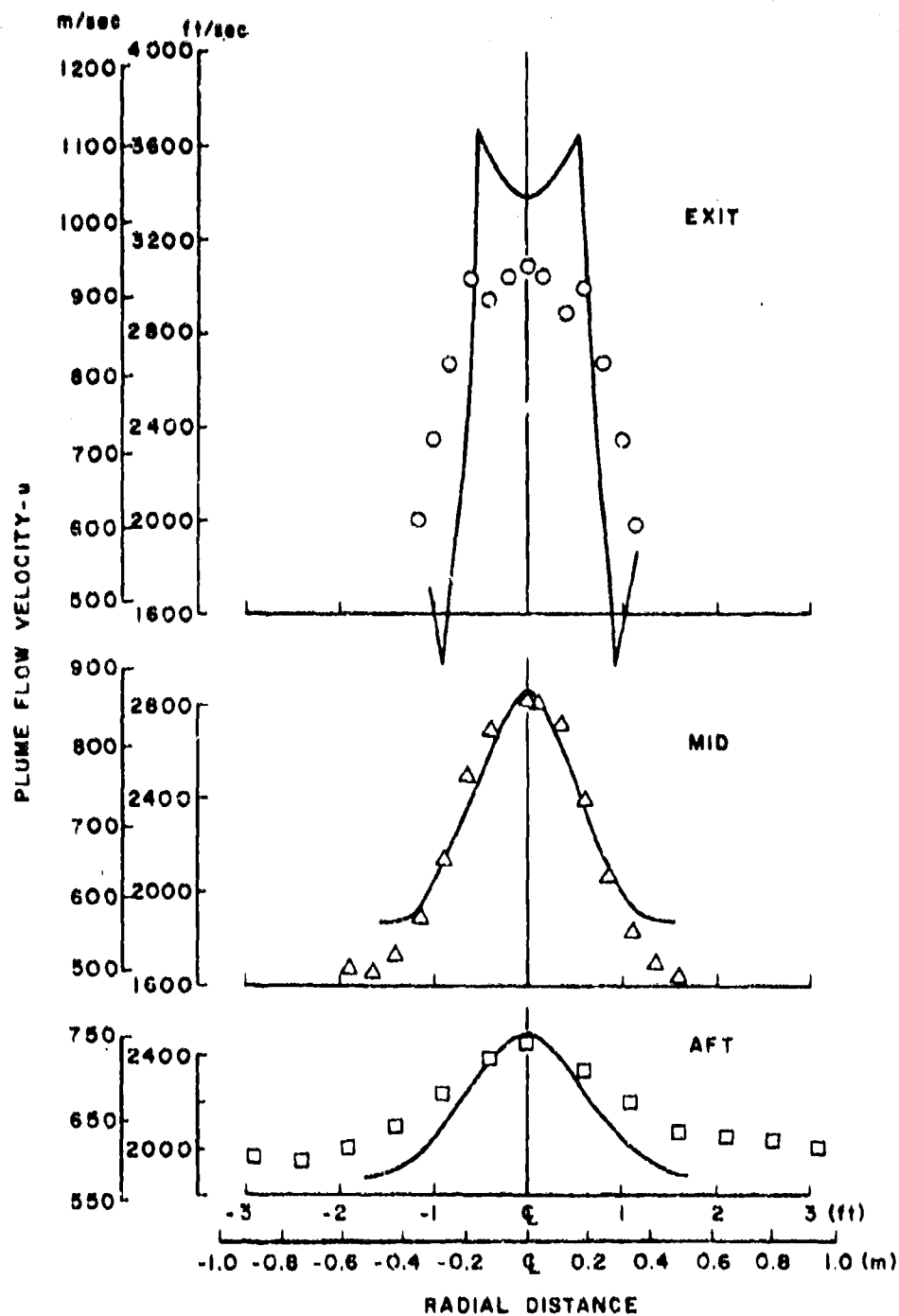
h. Plume Flow Velocity Fig. 24 Concluded
