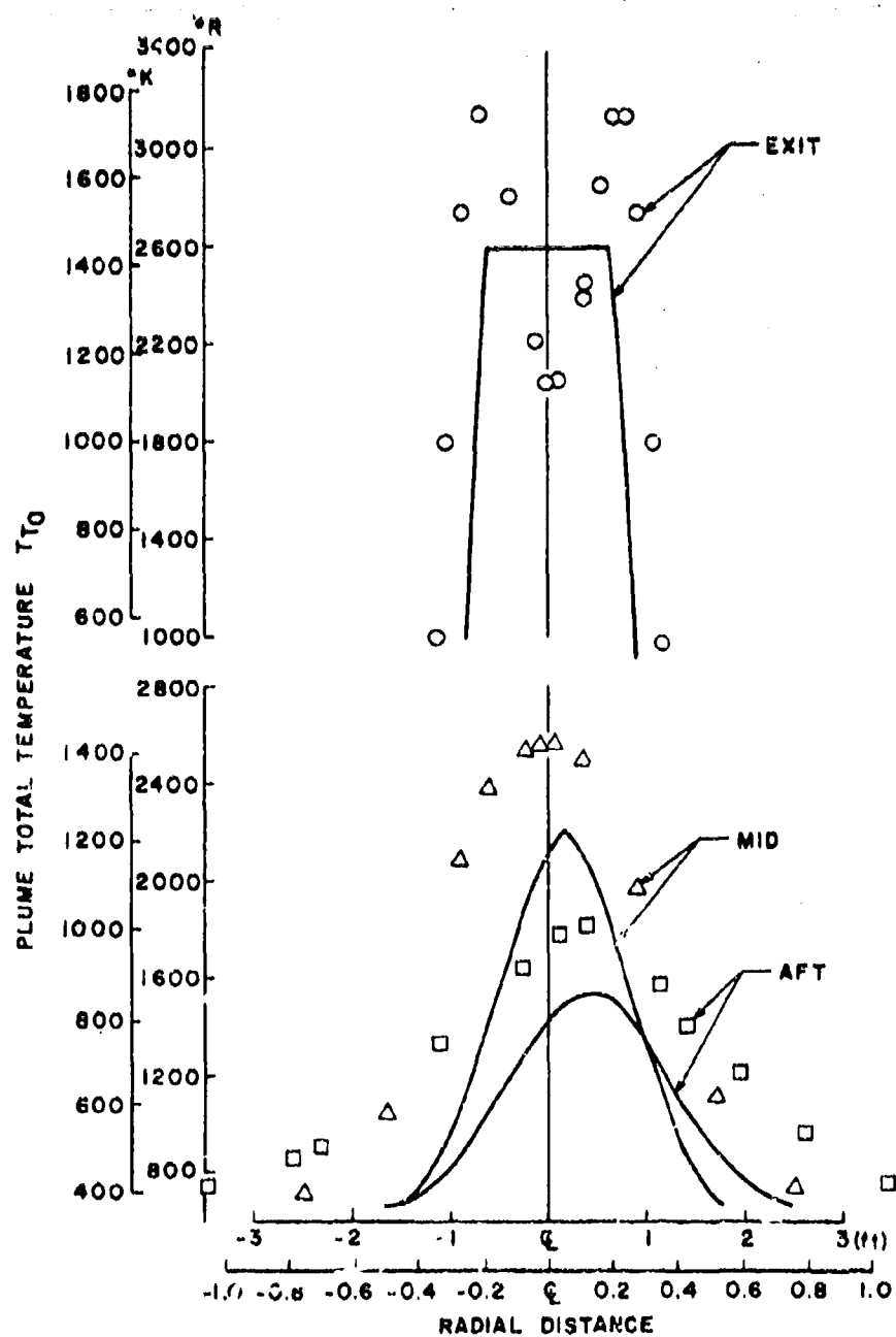
b. Plume Total Temperature Fig. 27 Continued
