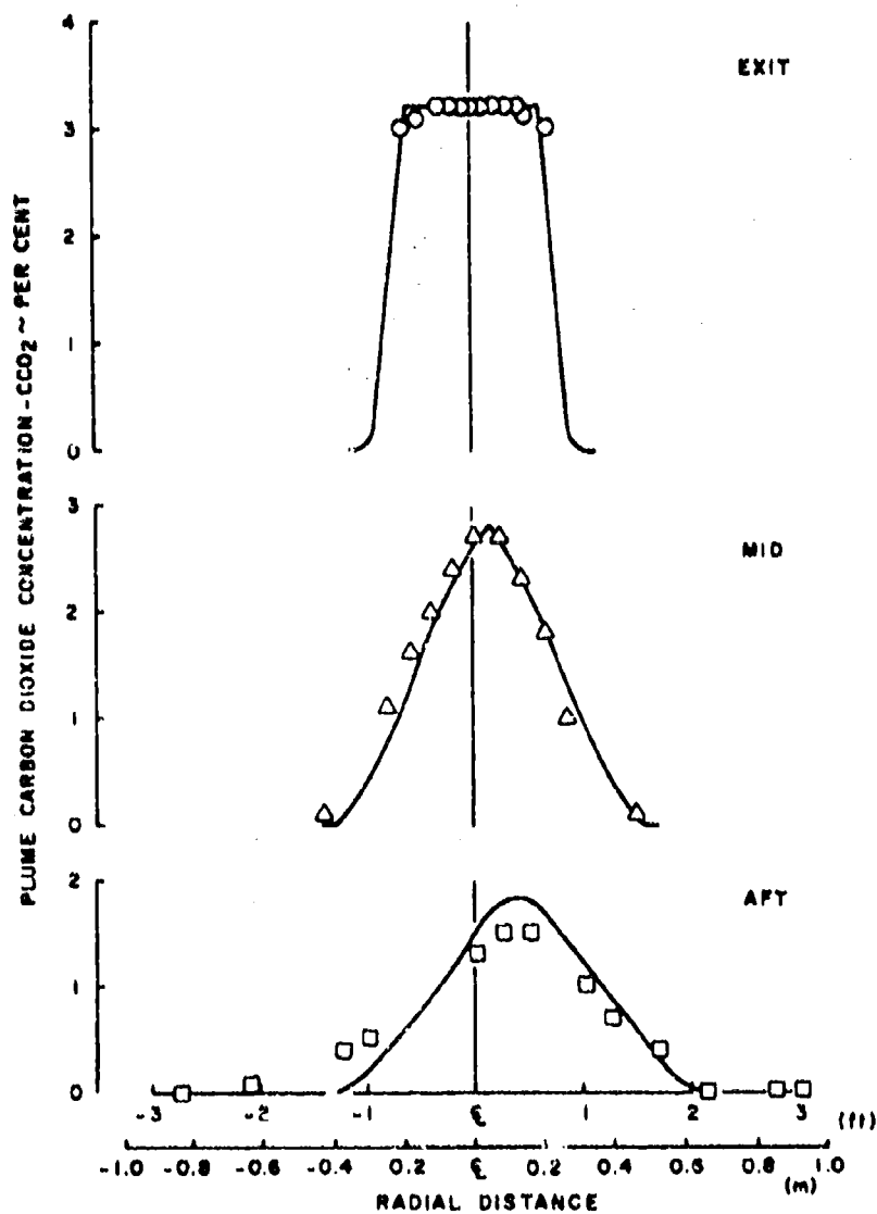
c. Plume Carbon Dioxide Concentration Fig. 24 Continued
