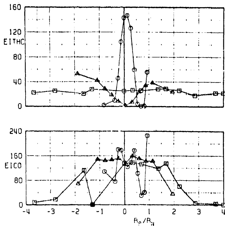
e. EITHC and EICO versus R_p/R_N Fig. 16 Continued
