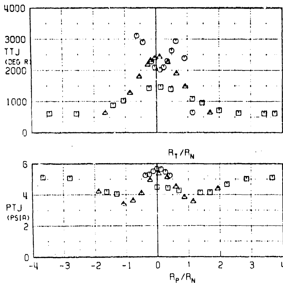
a. TTJ versus R_T/R_N and PTJ versus R_P/R_N Fig. 16 Variation of Emission Characteristics with Axial Probe Position (Mach 1.6/55,000 ft, A/B)
