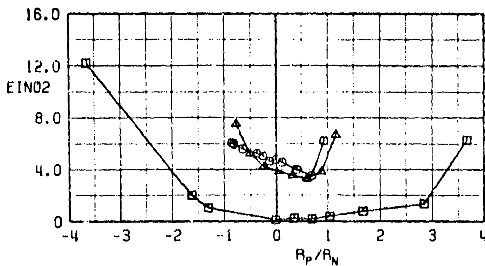
g. EINO_2 versus R_p/R_N Fig. 14 Concluded
