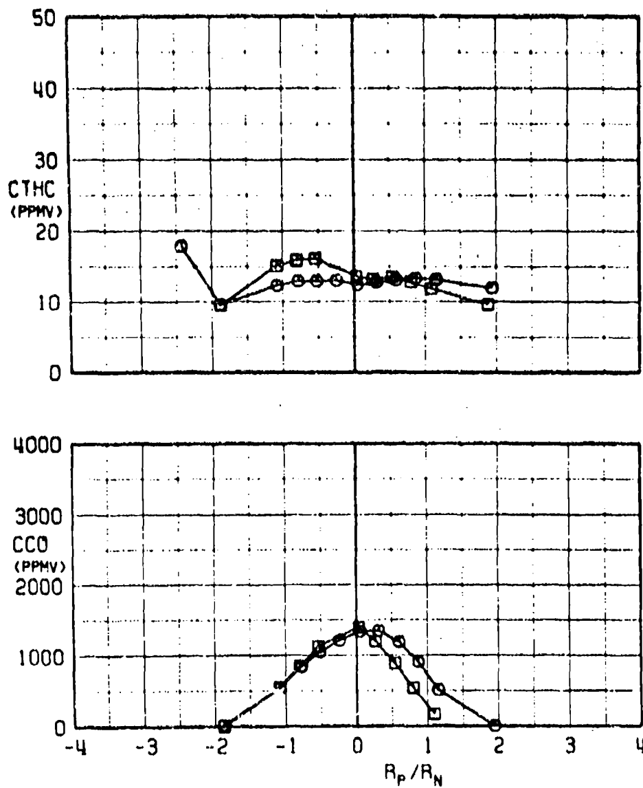
b. CTHC and CCO versus R_P/R_N Fig. 21 Continued
