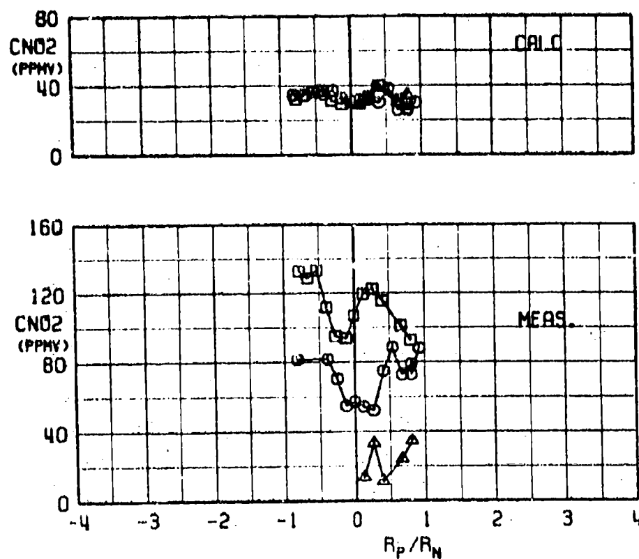
d. Calculated and Measured CNO_2 versus R_p/R_N Fig. 20 Concluded
