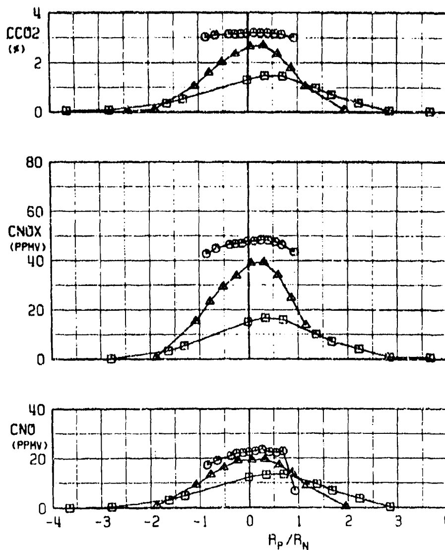
c. CCO_2 , CNO_x , and CNO versus R_P/R_N Fig. 15 Continued
