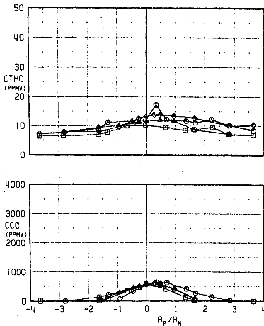
b. CTHC and CCO versus R_p/R_N Fig. 22 Continued
