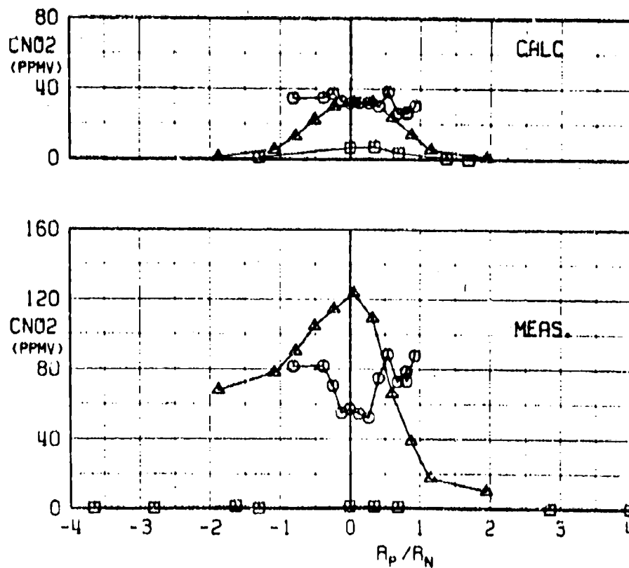
d. Calculated and Measured CNO_2 versus R_p/R_N Fig. 16 Continued
