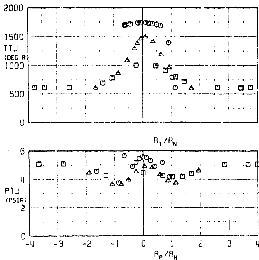
a. TTJ versus R_T/R_N , PTJ versus R_P/R_N Fig. 14 Variation of Emission Characteristics with Axial Probe Position (Mach 1.6/55,000 ft, MIL)
