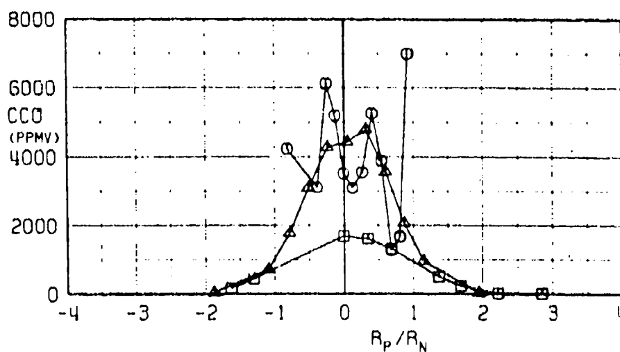
b. CTHC and CCO versus R_p/R_N Fig. 16 Continued
