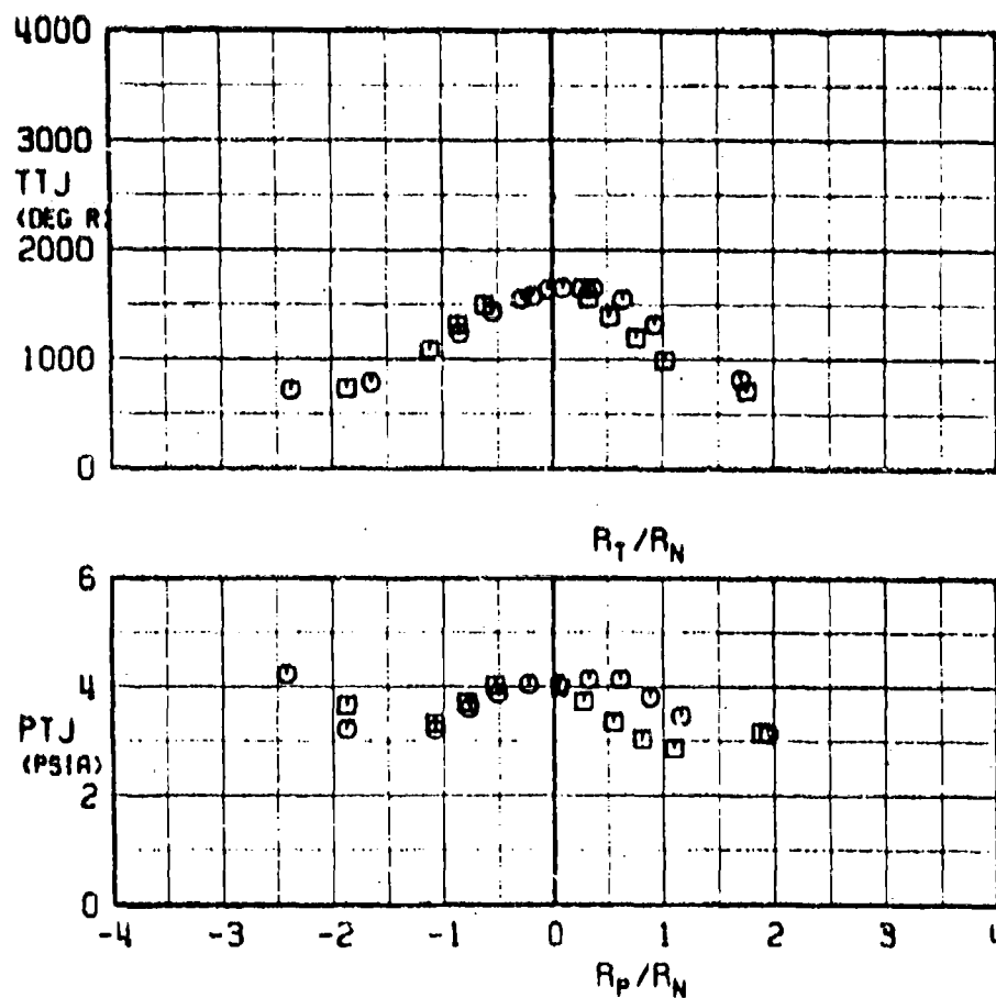
a. TTJ versus R_T/R_N and PTJ versus R_P/R_N Fig. 21 Comparison of Exhaust Emission Concentrations at Horizontal and Vertical Plume Axis (Mach 2.0/65,000 ft, MIL, Mid Station)
