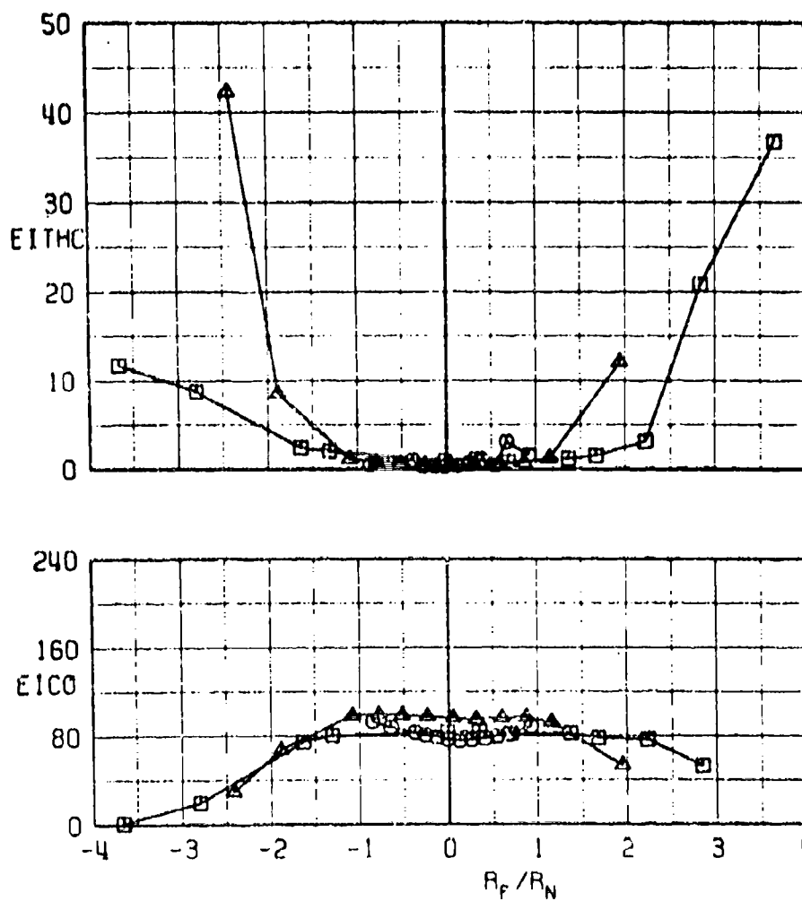
e. EITHC and EICO versus R_F/R_N Fig. 15 Continued
