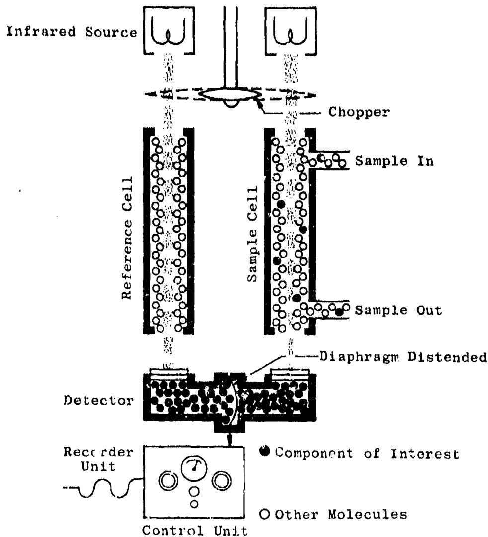
b. Typical NDIR Detector ( \text{CO} , \text{CO}_2 ) Fig. 11 Continued
