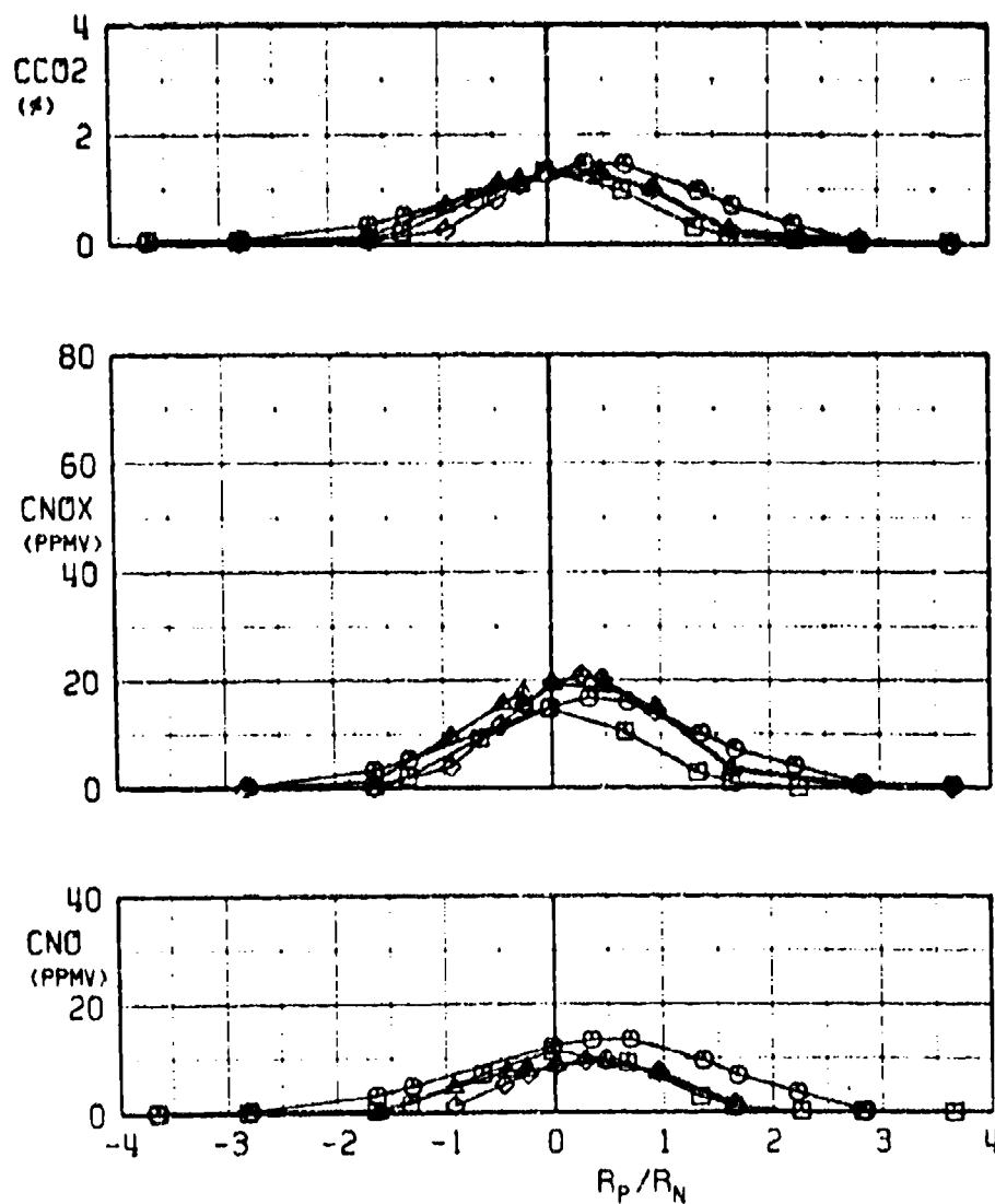
c. CCO_2 , CNO_x , and CNO versus R_p/R_N Fig. 22 Continued
