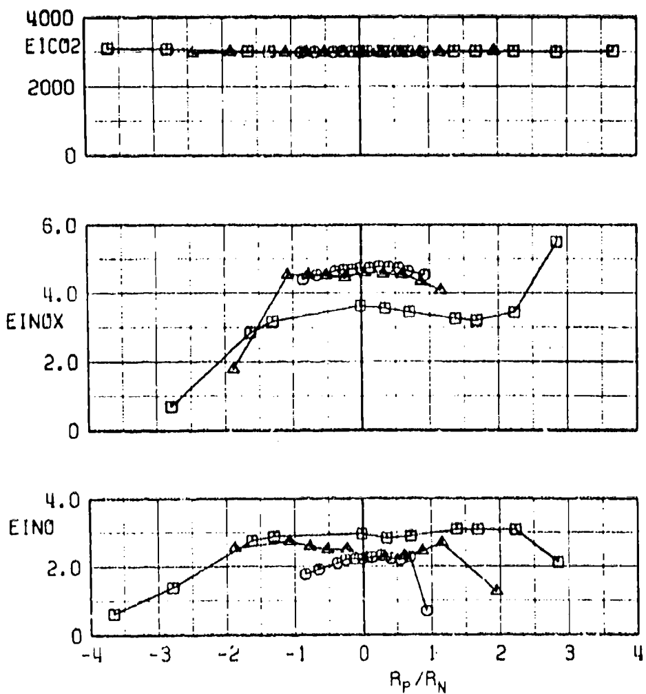
f. EICO 2 , EINO x and EINO versus R_p/R_N Fig. 15 Continued
