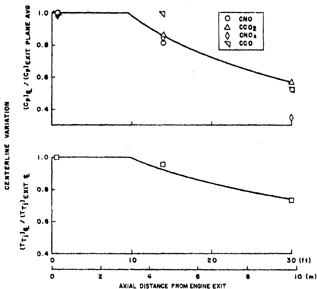
Fig. 26 Centerline Decay Characteristics of the Emission Concentrations and Total Temperature in the Exhaust Plume at Mach 2.0/65,000 ft, Military Power
