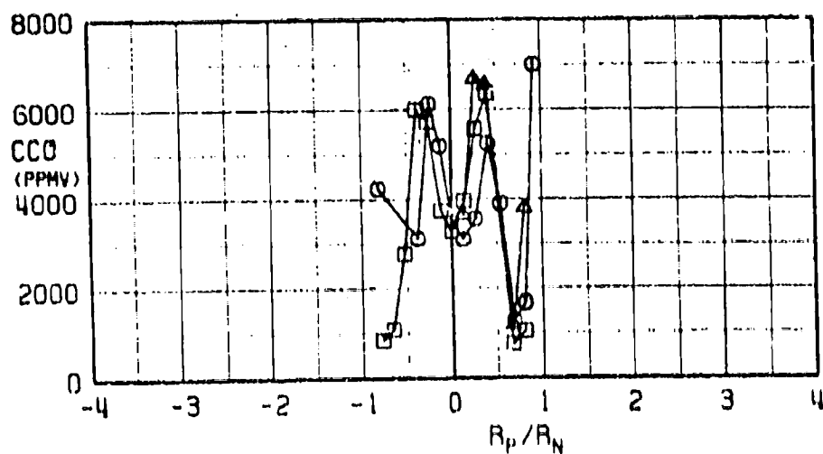
b. CTHC and CCO versus R_P/R_N Fig. 20 Continued
