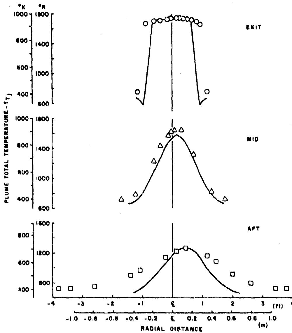
b. Plume Total Temperature Fig. 24 Continued
