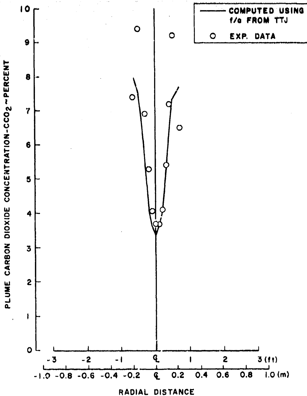
Fig. 29 Comparison of Theoretical and Experimental Carbon Dioxide Concentrations at the Exit Plane for Mach 2.0/65,000 ft, Afterburning Power
