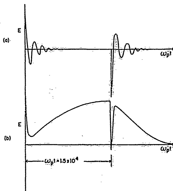
Figure 18. Response to a 10^{-6} sec Square Pulse for (a) v_c = 0 , \omega_p = 1.5 \times 10^{10} and (b) v_c = \omega_p = 1.5 \times 10^{10}
