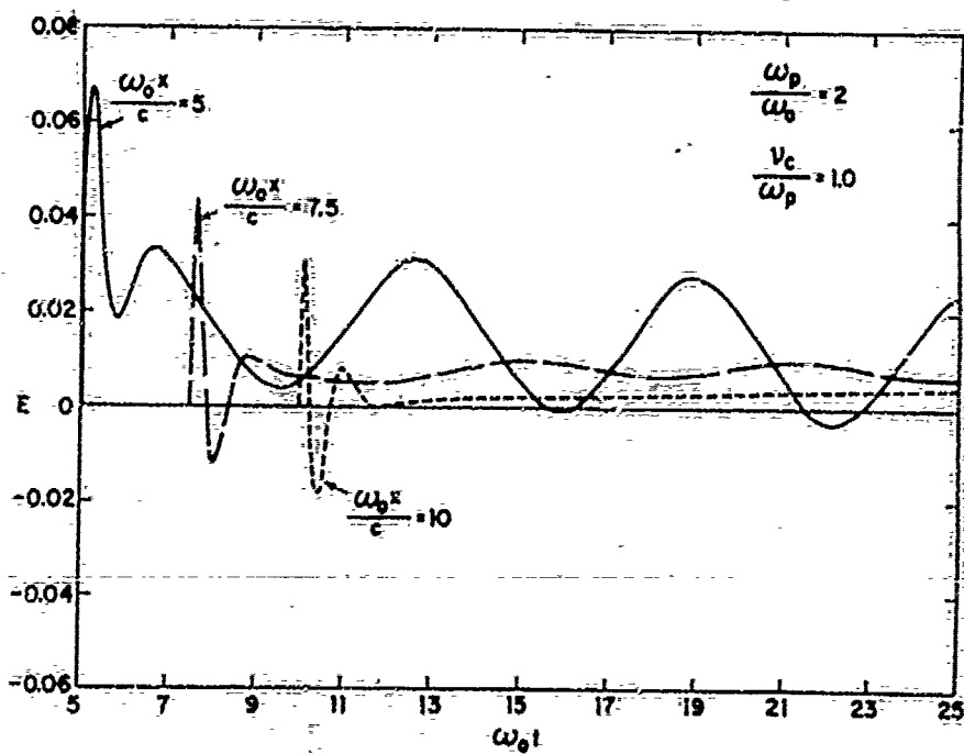
Figure 9. Transient Response to Step-Carrier Sine Wave for v_c/\omega_p = 1.0 and \omega_p/\omega_0 = 2
