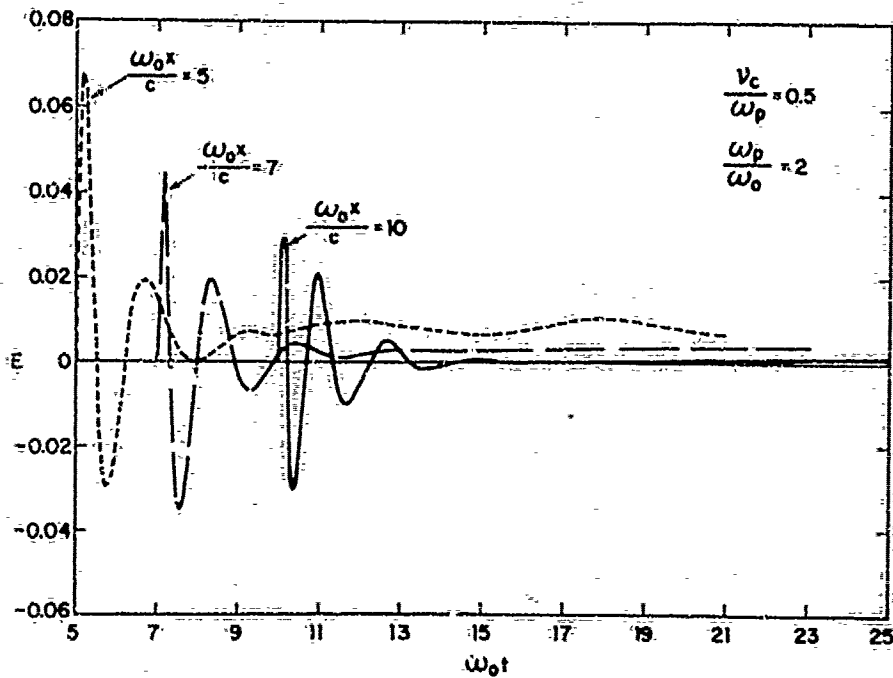
Figure 8. Transient Response to Step-Carrier Sine Wave for v_c/\omega_p = 0.5 and \omega_p/\omega_0 = 2
