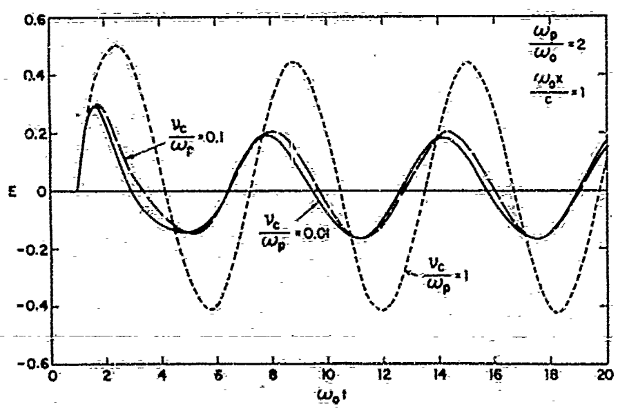
Figure 5. Transient Response to Step-Carrier Sine Wave for \omega_0 x/c = 1 and \omega_p/\omega_0 = 2
