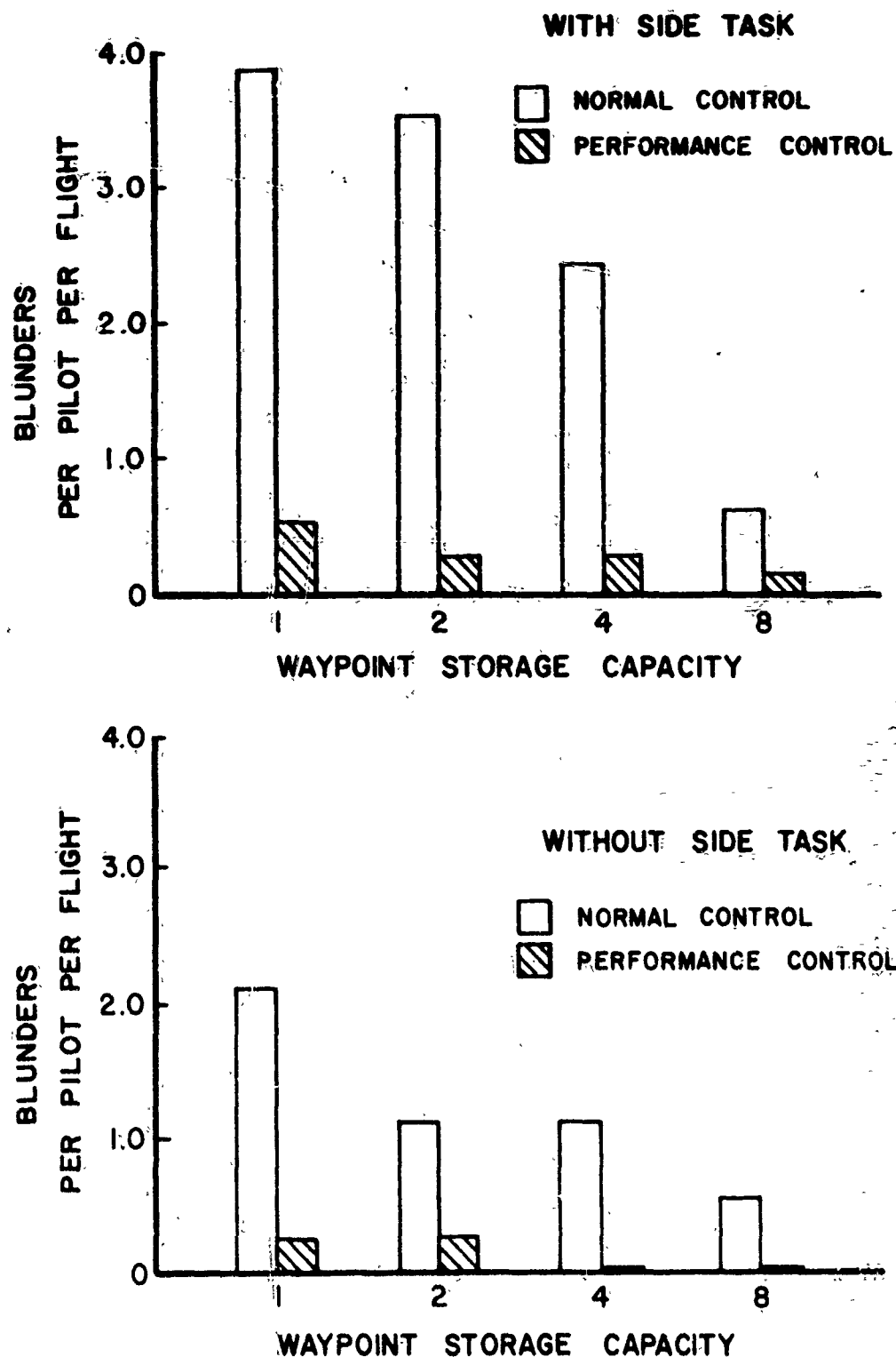
Figure 26. Area navigation procedural blunders as a function of computer waypoint storage capacity for normal control and flight performance control, with and without side-task loading.
