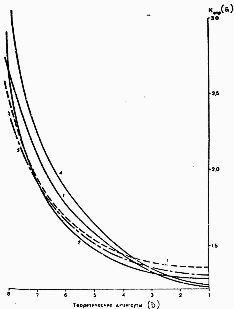
Figure 2. Values of k_{отр} = \frac{(l_{отр})_{max}^{1/4}}{l_1^{1/4}} for icebreakers with stern screws: 1) "Moskva"; 2) "Sibir"; 3) "Krasin"; 4) "Sibiryakov"; and 5) "Yermak". a) k_{отр} ; b) theoretical frames.
