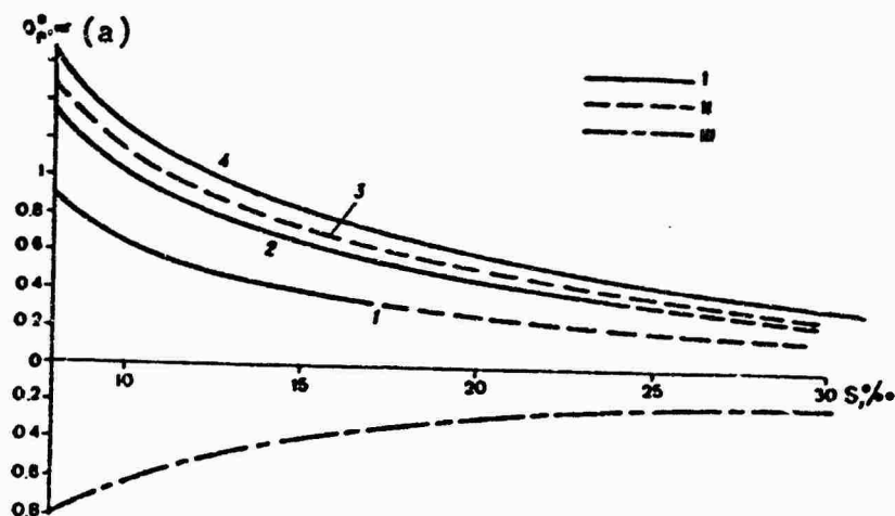
Figure 1. Dependence of \sigma_v upon the salinity of the water with an ice thickness of 10 millimeters (1), 15 millimeters (2), 20--22 millimeters (3) and 25--30 millimeters (4). I) according to experimental data; II) according to extrapolation data; III) presumed curve (in spraying of the surface of the ice with a NaCl solution, ice thickness 25--30 millimeters). a) \sigma_v , kilograms.
