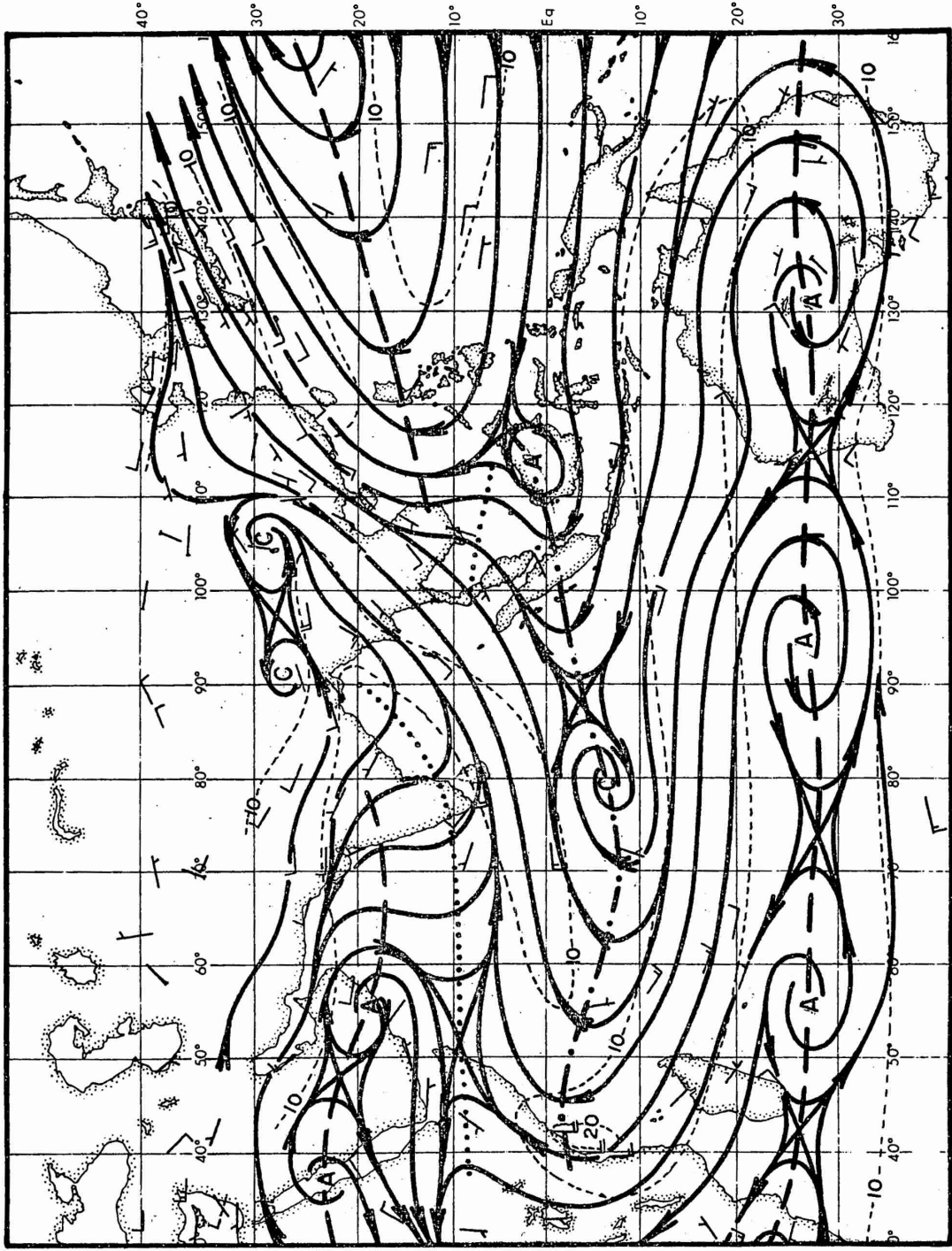
MAY, 850 mb
