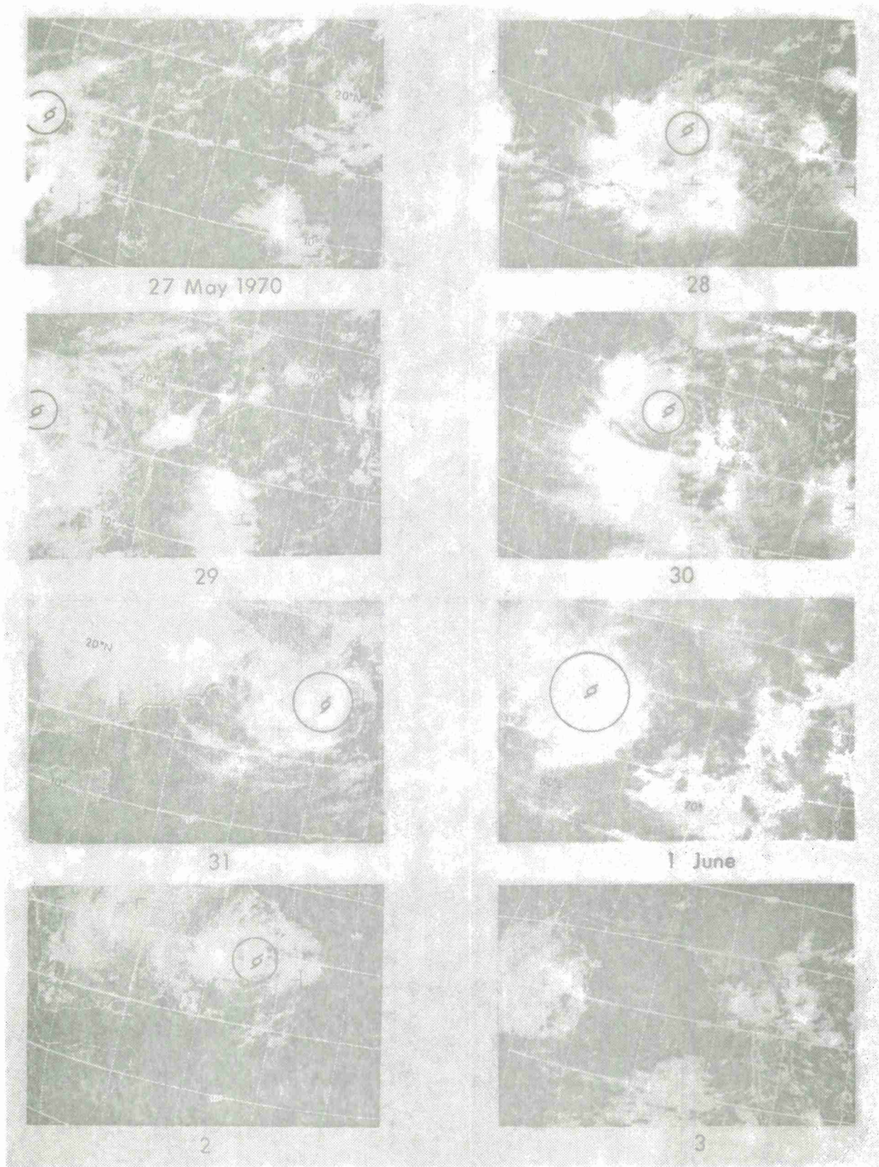
Figure 2. Satellite views of a moderate cyclonic storm in the Arabian Sea (May 1970)
