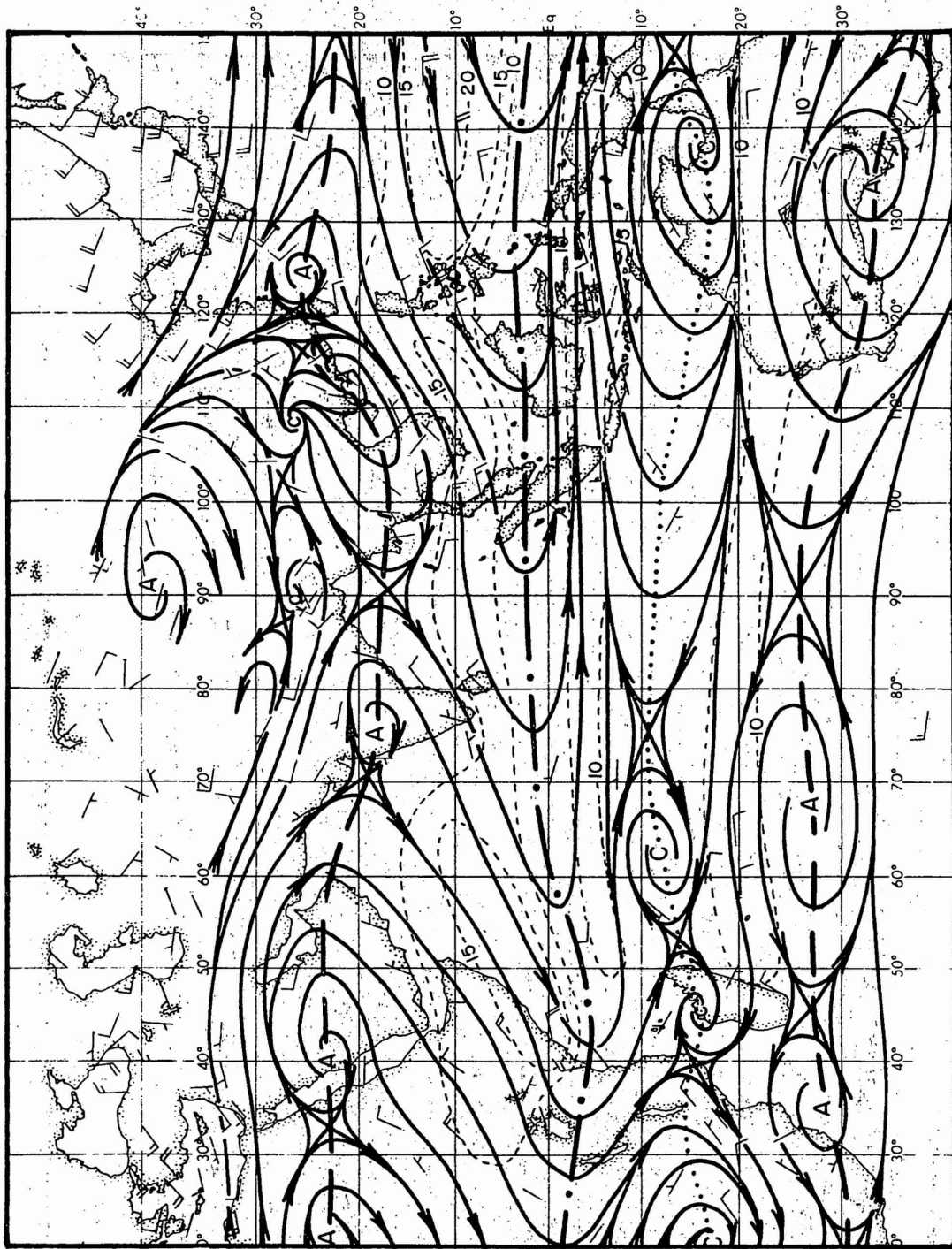
JANUARY, 850 mb
