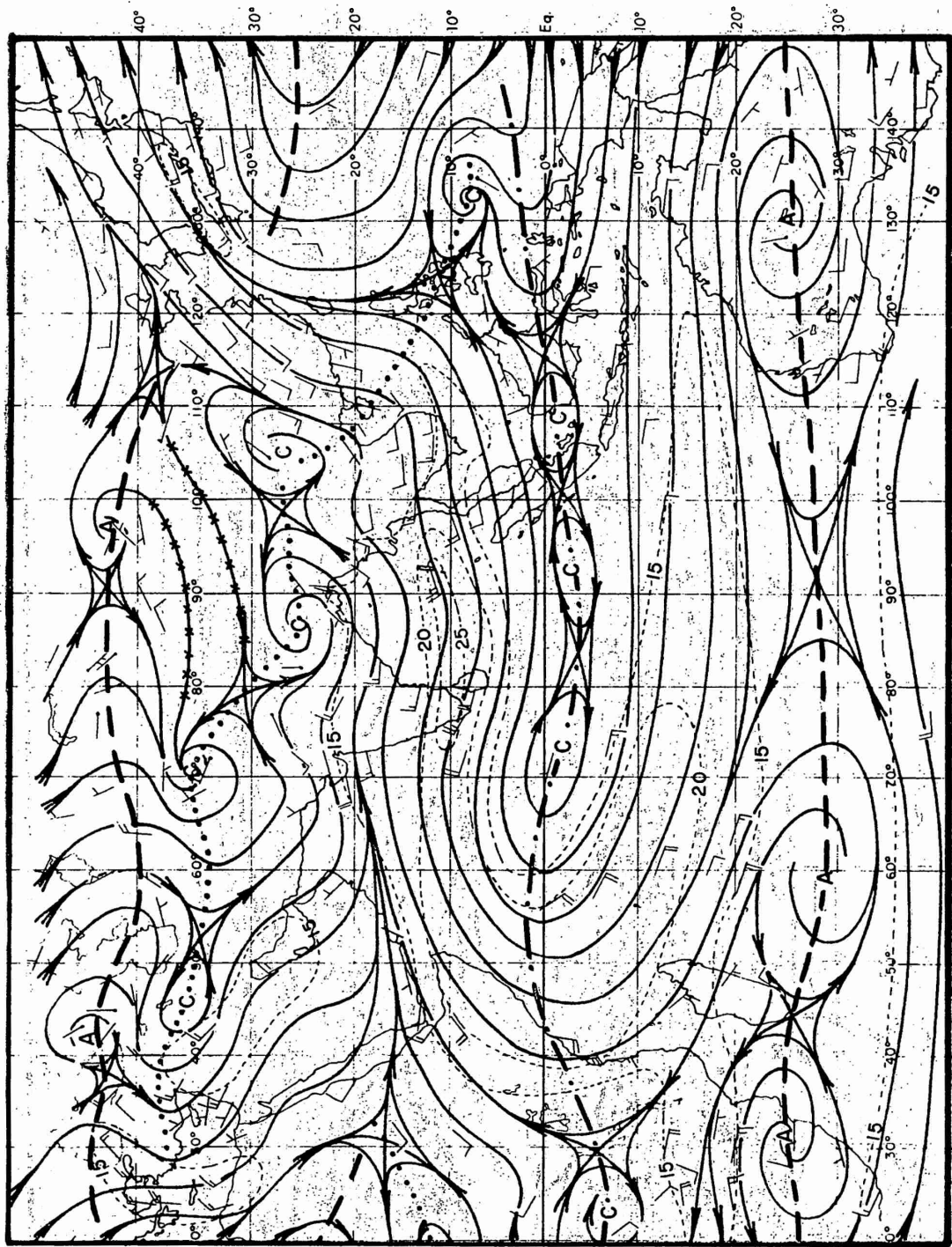
JULY, 850 mb Figure 31
