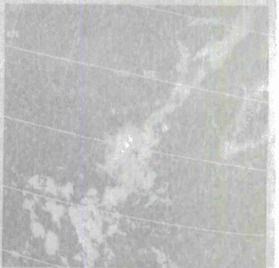
Figure 24. Satellite views of a tropical storm in the southwestern Arabian Sea (November 1967).
