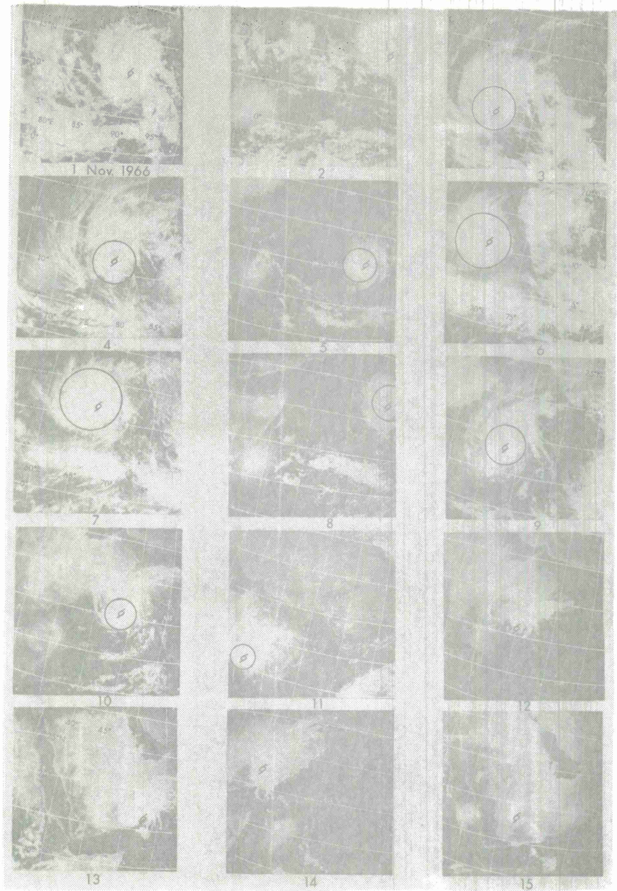
Figure 1. Satellite views of a moderate cyclonic storm in the Bay of Bengal and Arabian Sea (November 1966)
