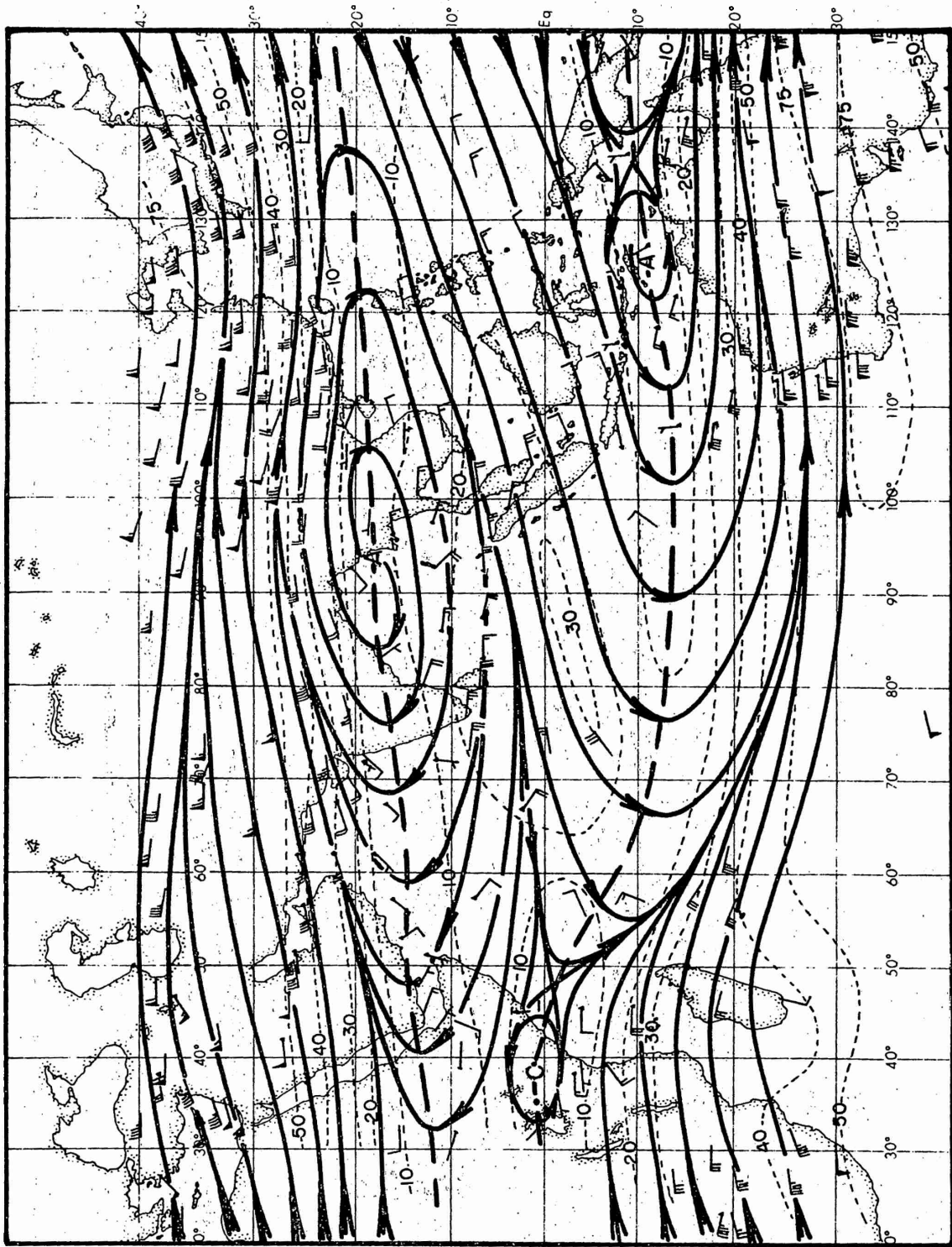
OCTOBER, 200 mb
