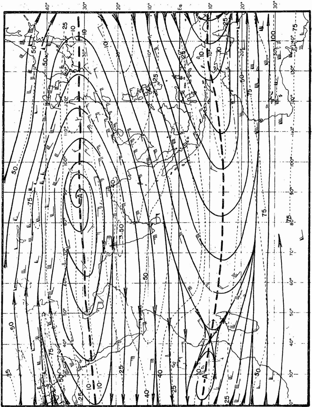
JULY, 200 mb
