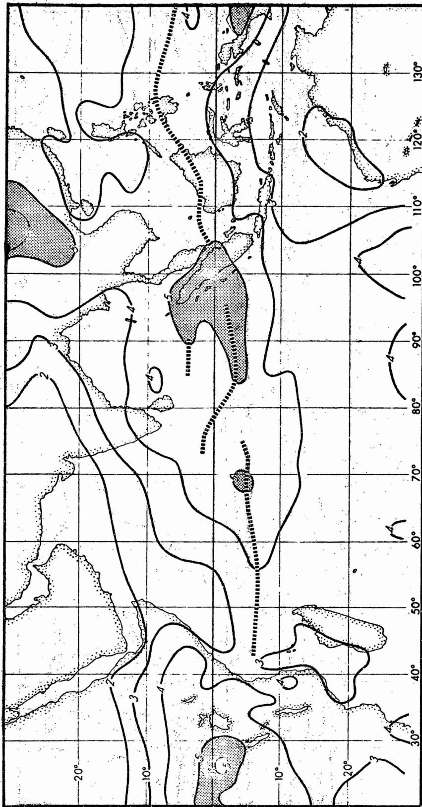
Figure 39. Mean cloudiness (in octas) over the Indian Ocean (October)
