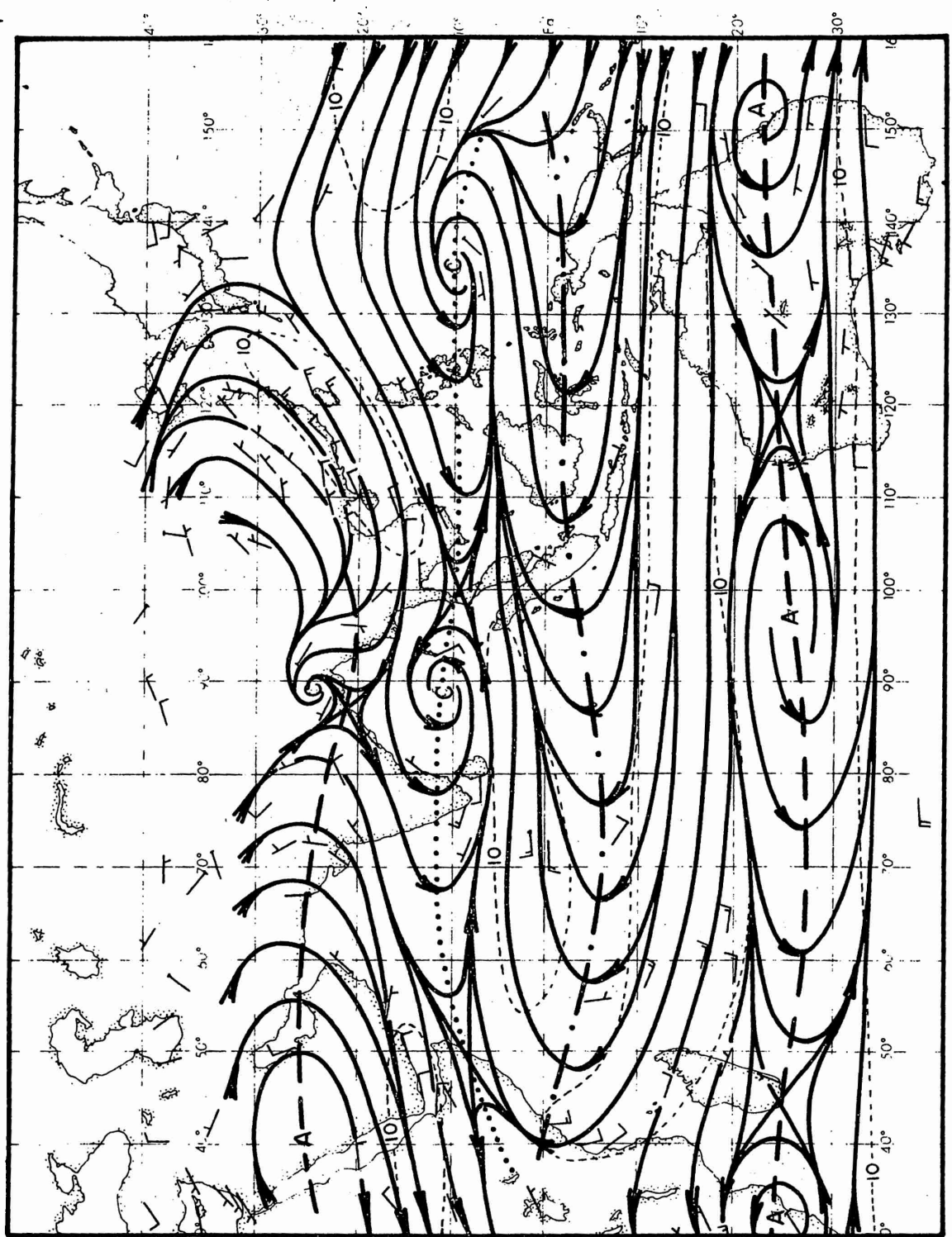
OCTOBER, 850 mb Figure 26
