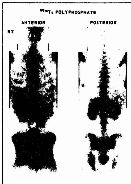
Figure 3. Anterior and posterior views in a normal technetium-99m polyphosphate bone scan
