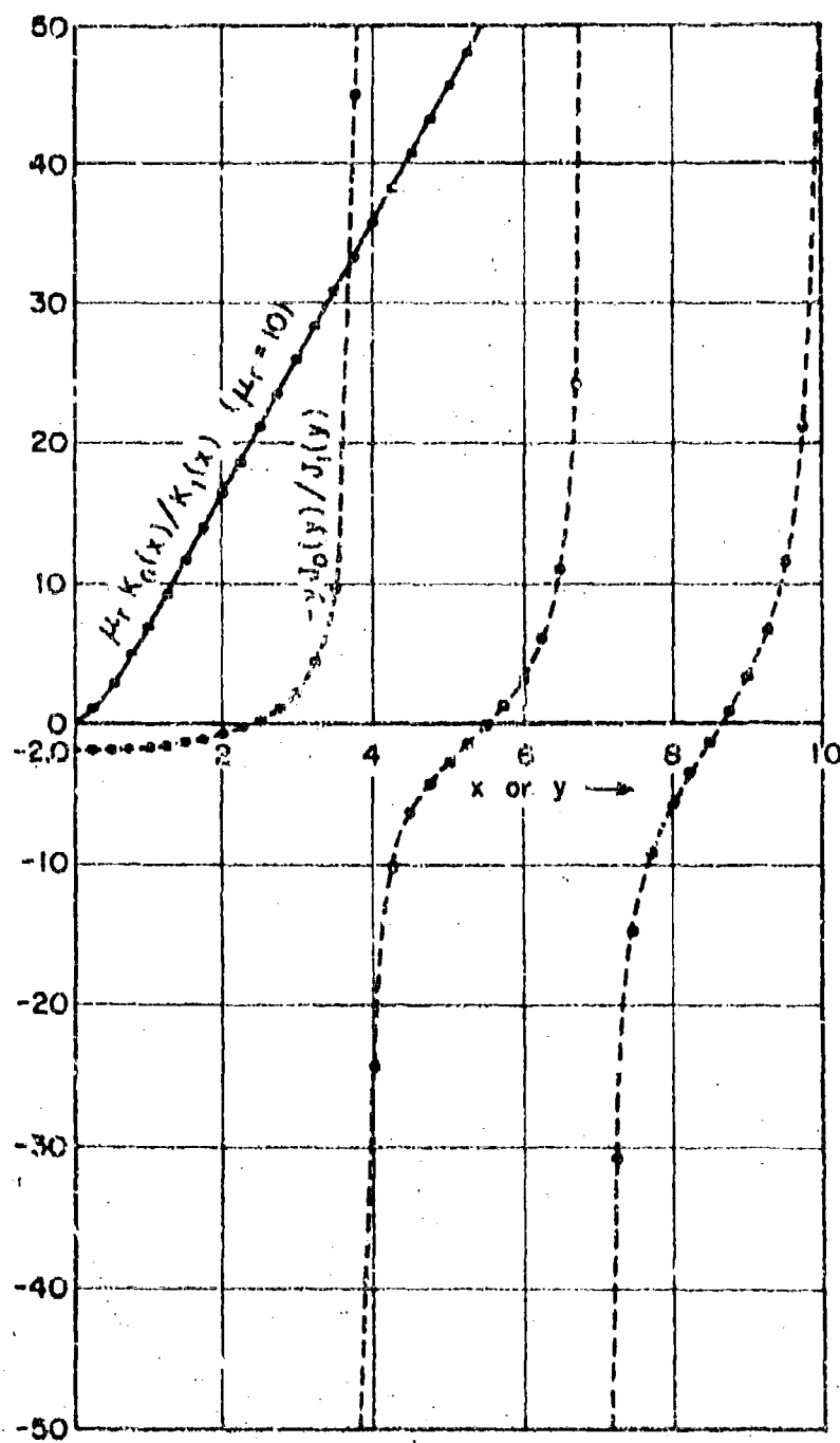
FIG. 5 GRAPHICAL SOLUTION FOR TRANSCENDENTAL EQN (26)
