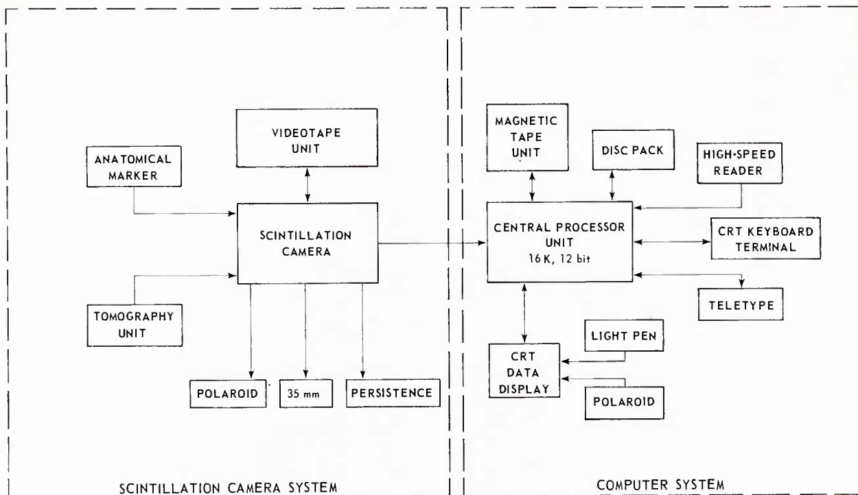
Figure 1. Systems assembly of the scintillation camera and computer
