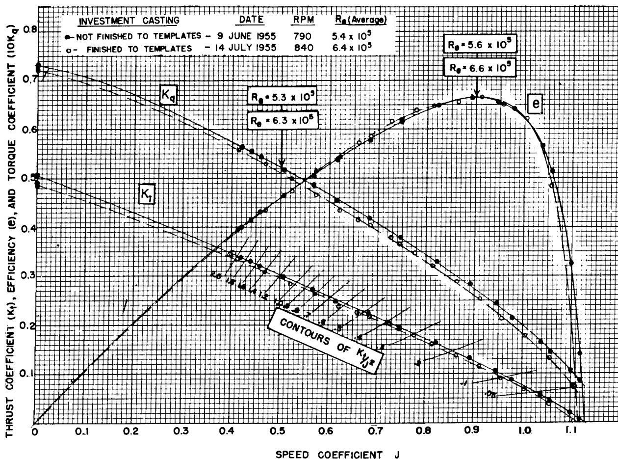
Figure 2 - Open-Water Characteristics of Propeller 3448
