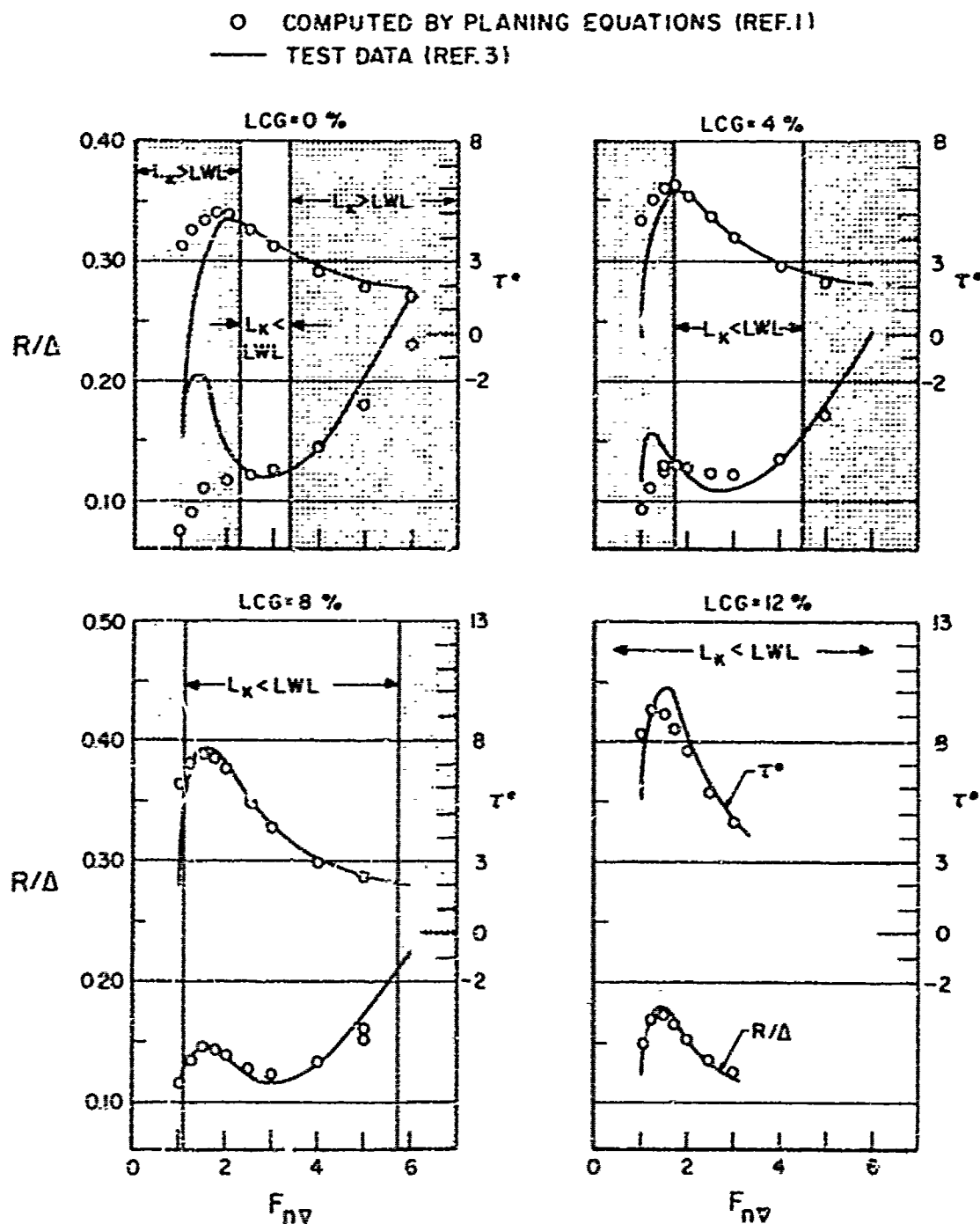
FIG. 2. RESISTANCE AND TRIM VS F_v SERIES 62, L/B=7.0 , \lambda p/\nabla^{2/3}=7.0 , \Delta=100,000 LBS
