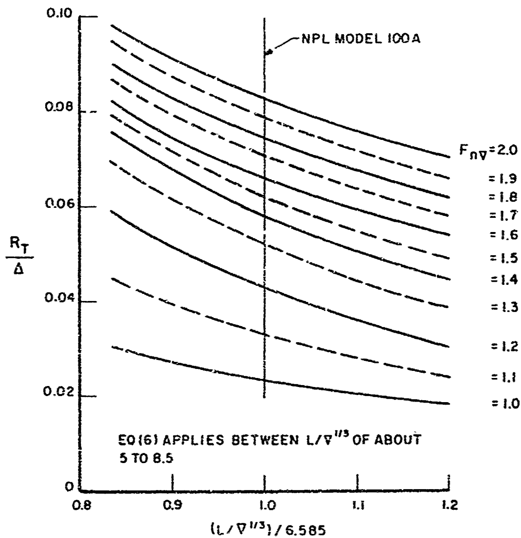
FIG.24a. INFLUENCE OF VARIATIONS OF L/V^{1/3} ON R_T/\Delta , FROM EQ (6) FOR A PARTICULAR HULL FORM
