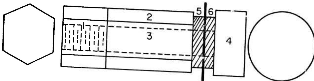
Fig. 5-9 The P-7 resonator
