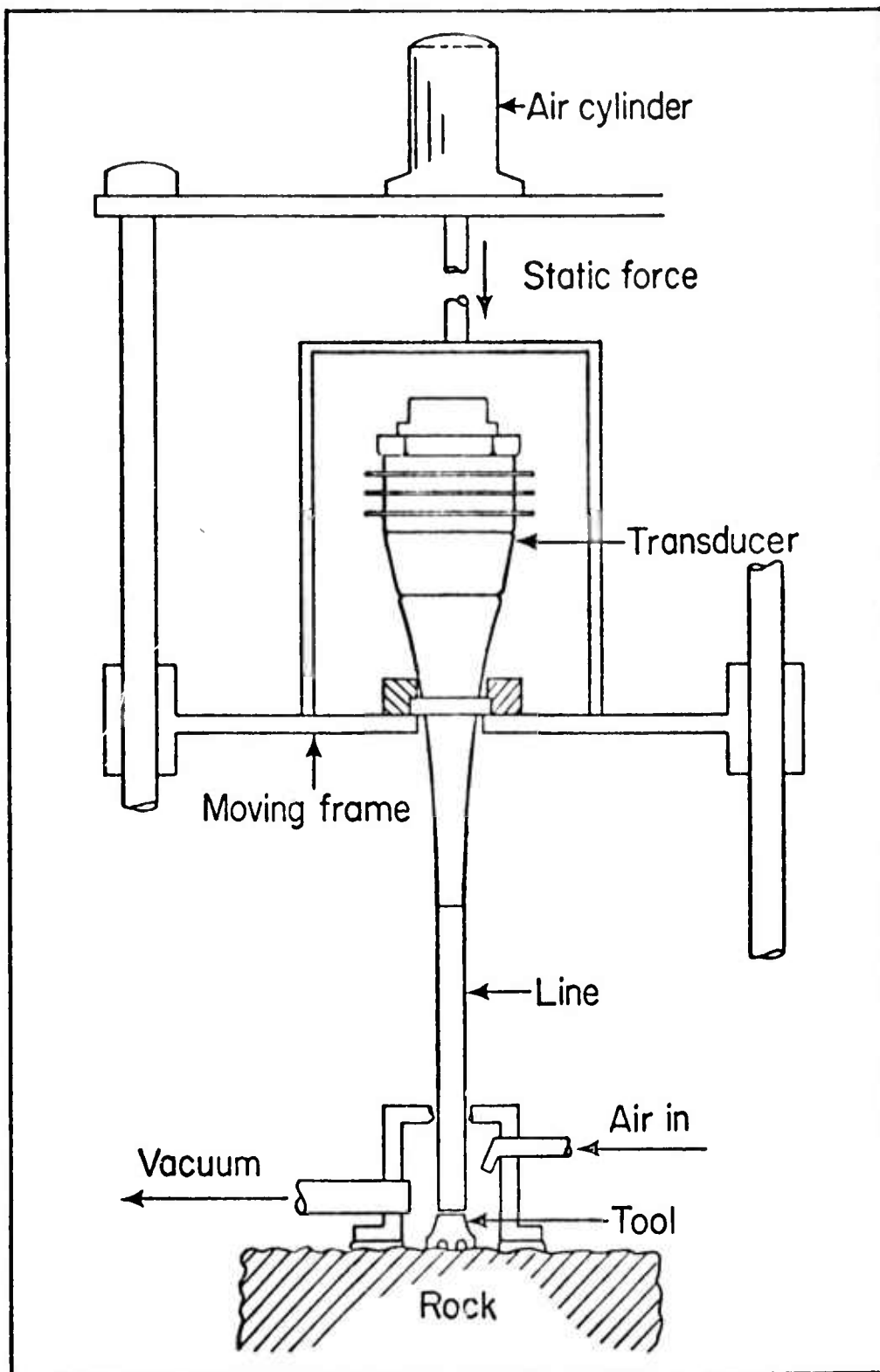
Fig. 3-1 Drilling apparatus
