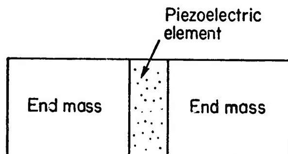
Fig. 4-7 Cylindrical sandwich type resonator
