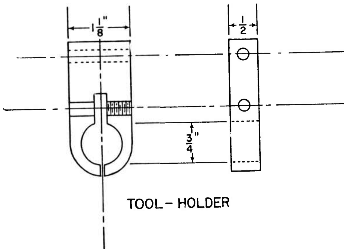
Fig. 1-21 Two-piece impact tool
