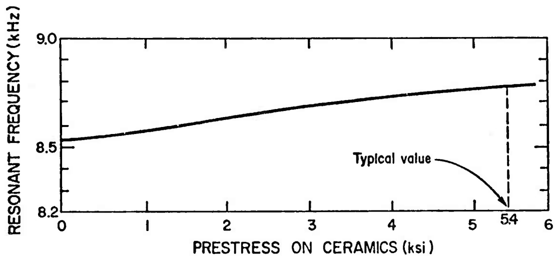
Fig. 5-17 The prestress effect on the resonant frequency of a simple resonator
