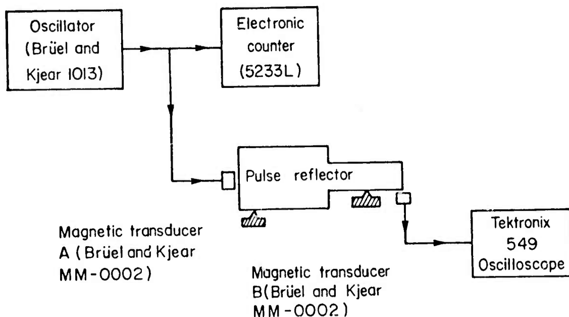
Fig. 6-5 Schematic diagram of apparatus
