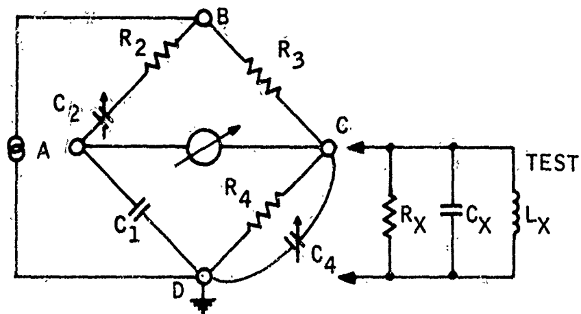
Figure 2-2. Schering Bridge Circuit
