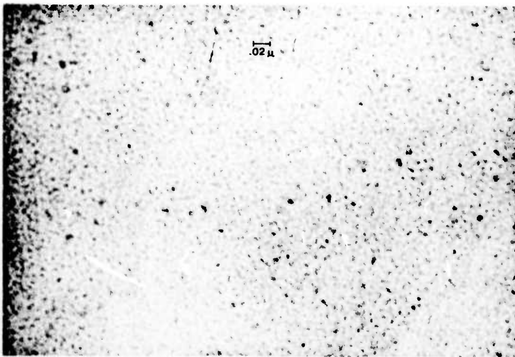
(a) TEM photograph of \text{Ge}_{20}\text{Se}_{40}\text{Te}_{40} annealed at 145^\circ\text{C} for 30 minutes. Crystallite particle size is \sim 68\text{\AA} .
