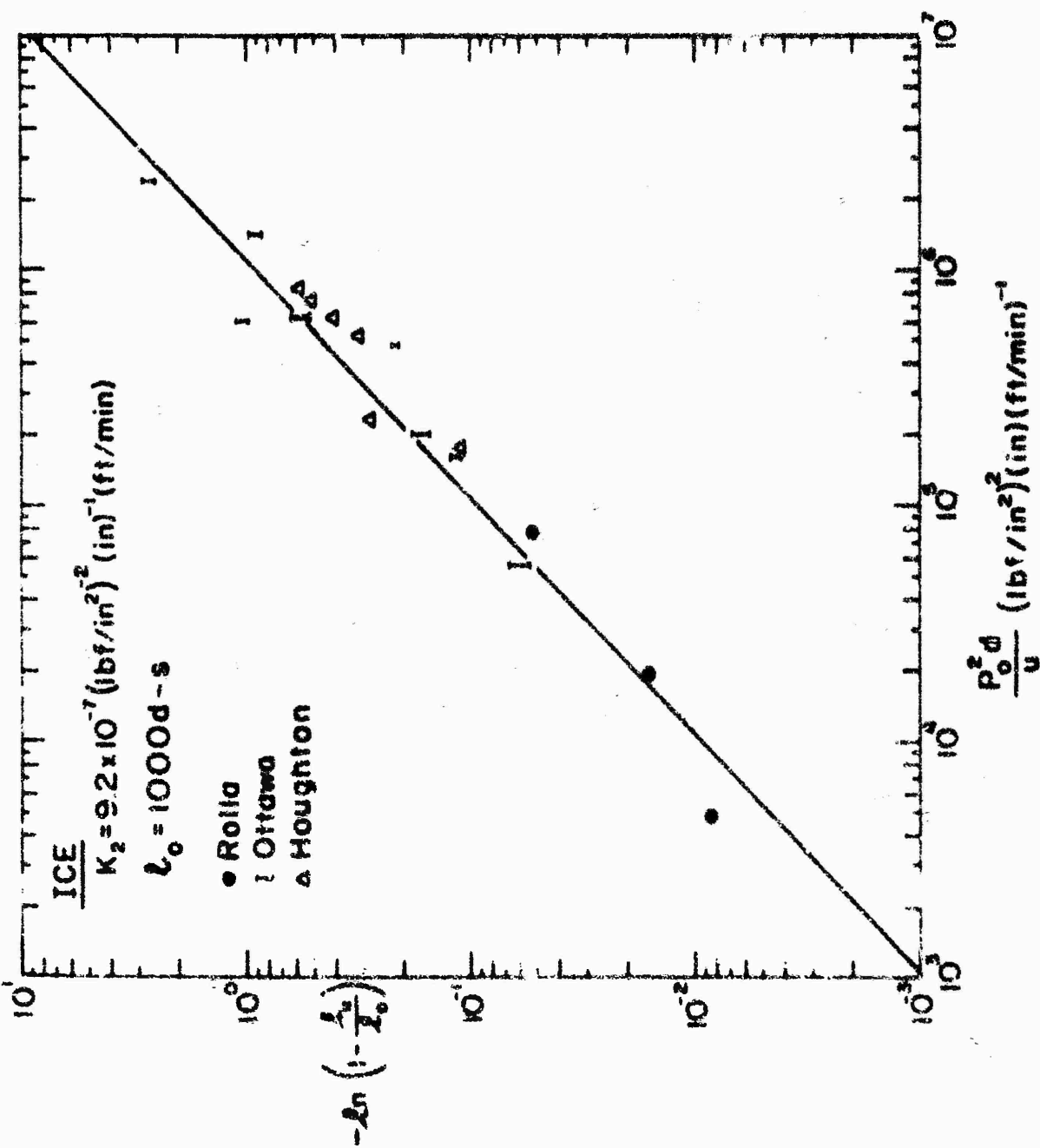
Figure 8. Logarithmic plot of -\ln (1-L/L_0) against P_o^2 d/u for three different assumptions on f_o .
