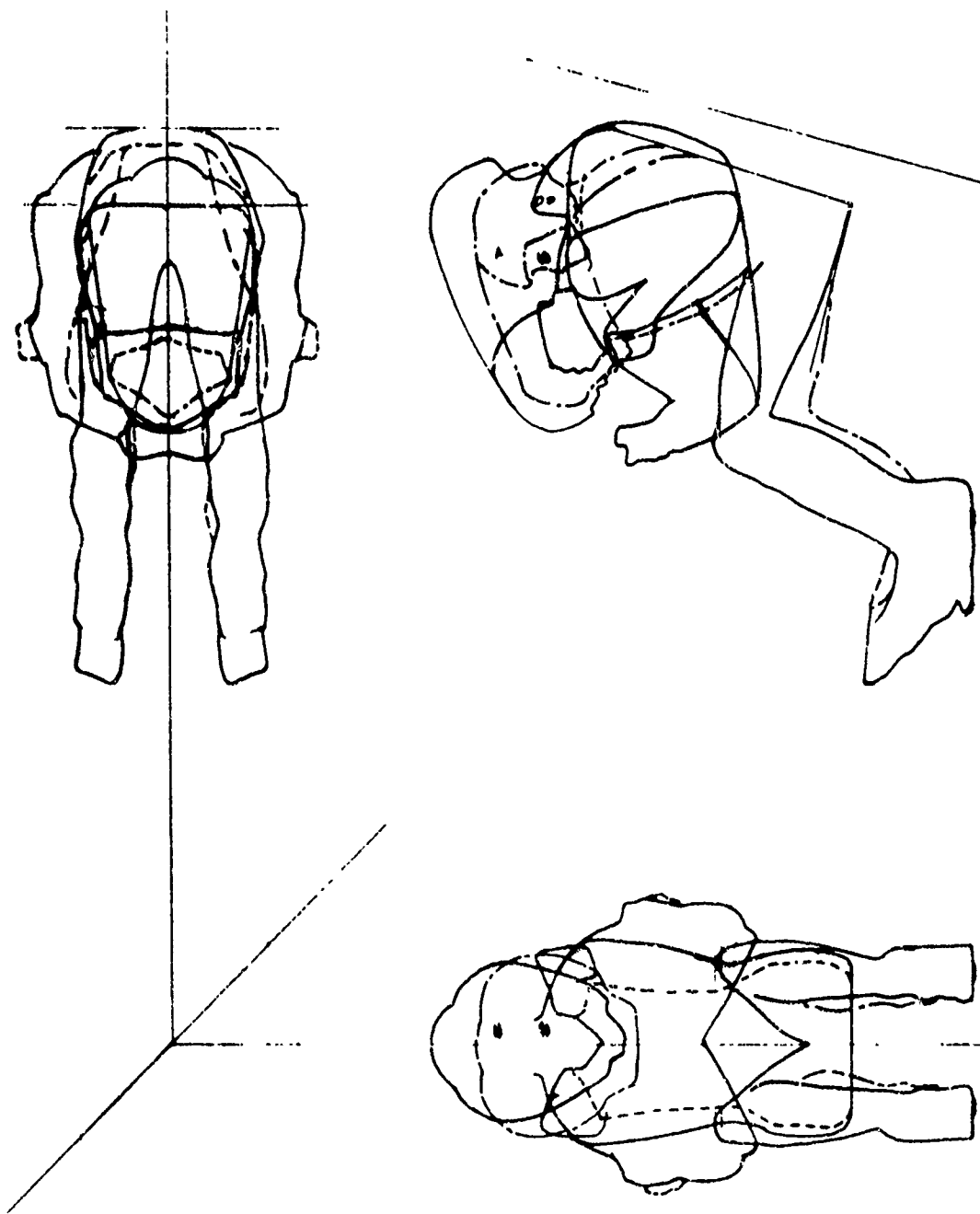
COPLOT MOTION ENVELOPE AH-1G
