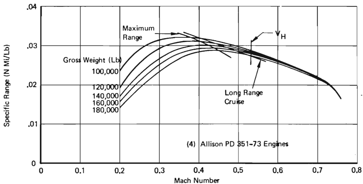
Figure 39: Fuel Mileage at Sea Level – Standard Day
