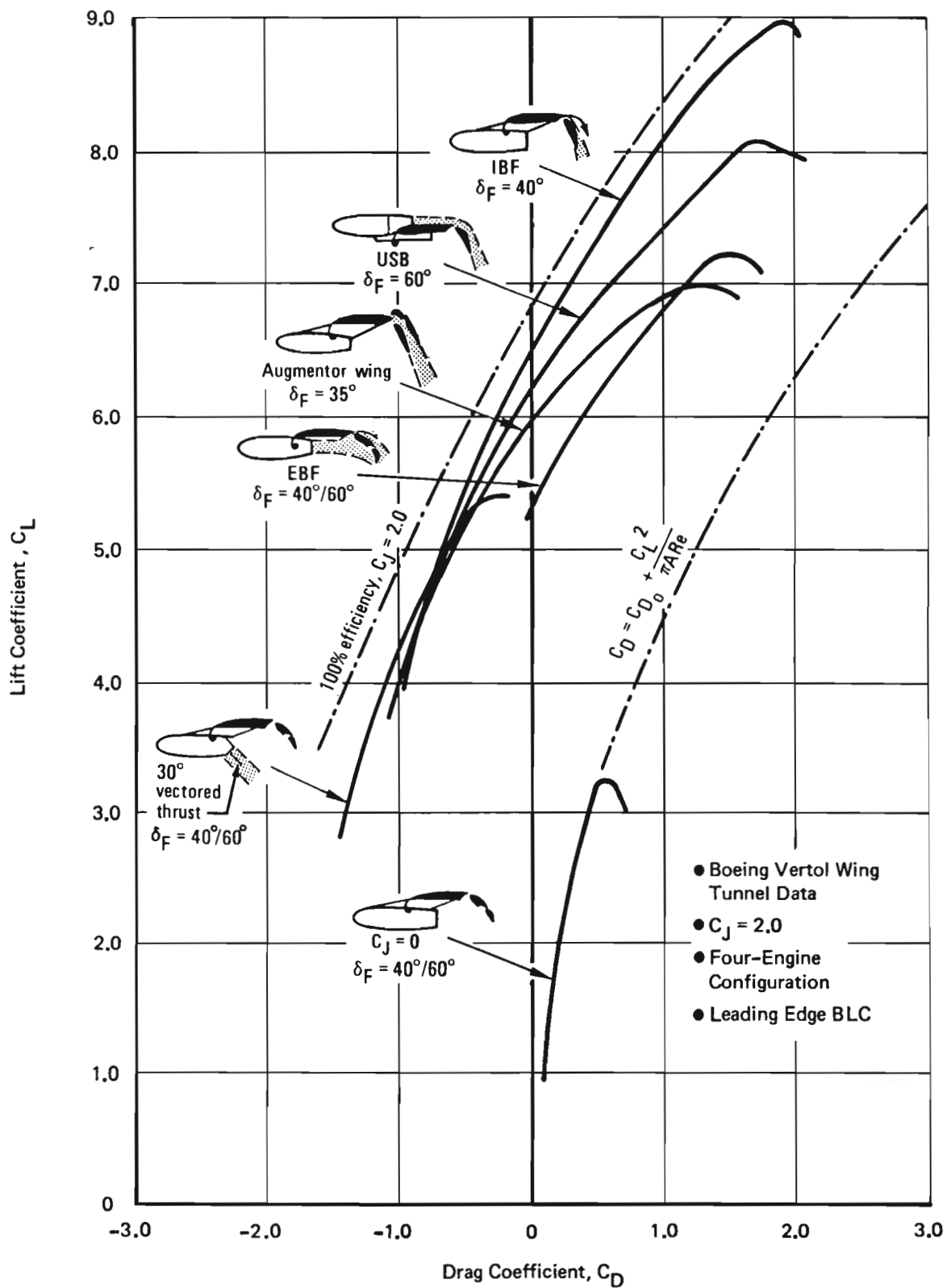
Figure 84: Drag Polars for Various Powered-Lift Concepts
