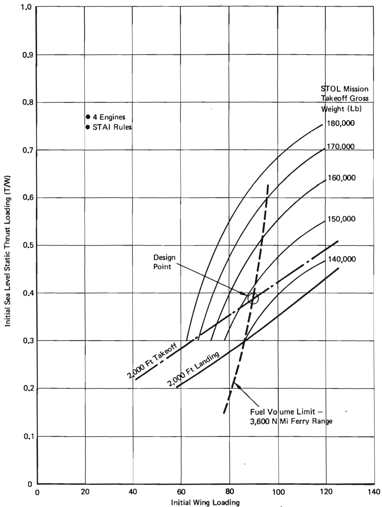
Figure 85: Parametric Design – USB Airplane
