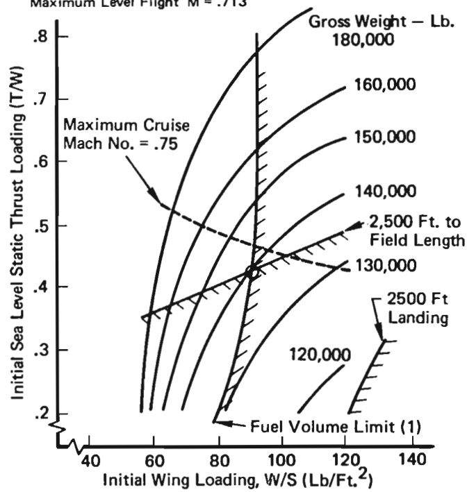
Figure 93: 2,500 FT. FIELD LENGTH TRADE
