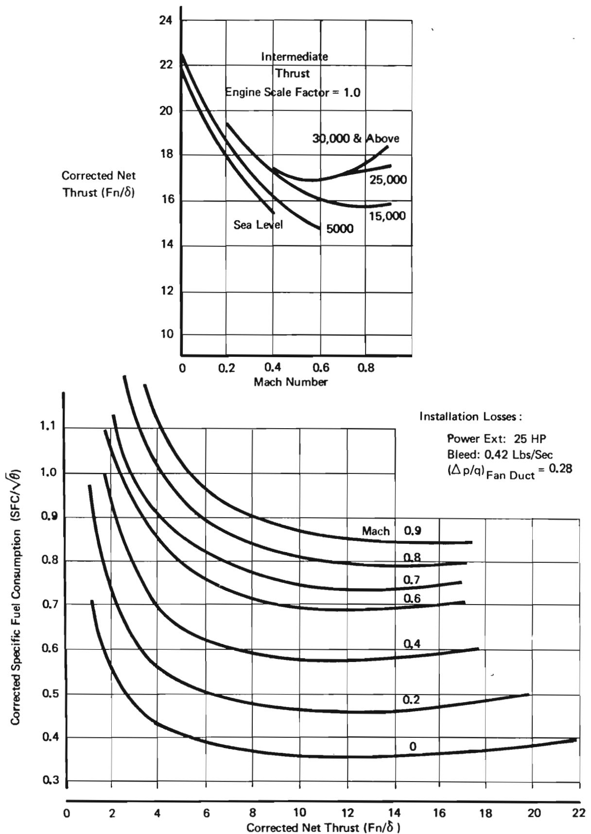
Figure 24 : Allison PD 351-73 Installed Performance
