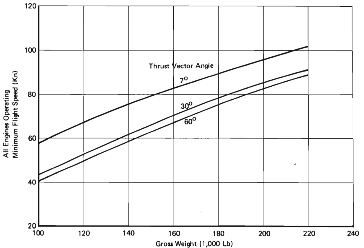
Figure 36: Minimum Flight Speeds – 2,500 Feet/93°F
