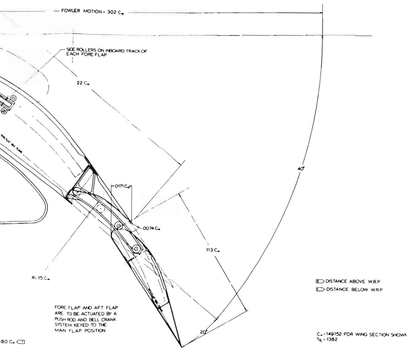
Figure 104: Trailing Edge Flap Mechanization
