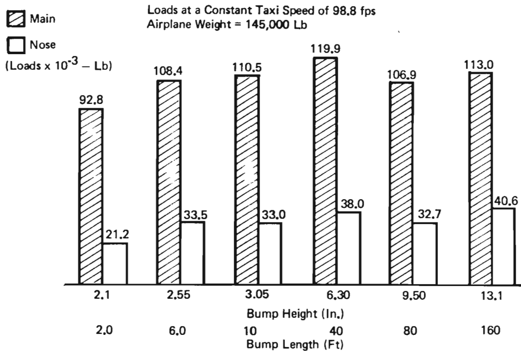
Figure 74: Taxi Loads – Varying Bump – Constant Speed
