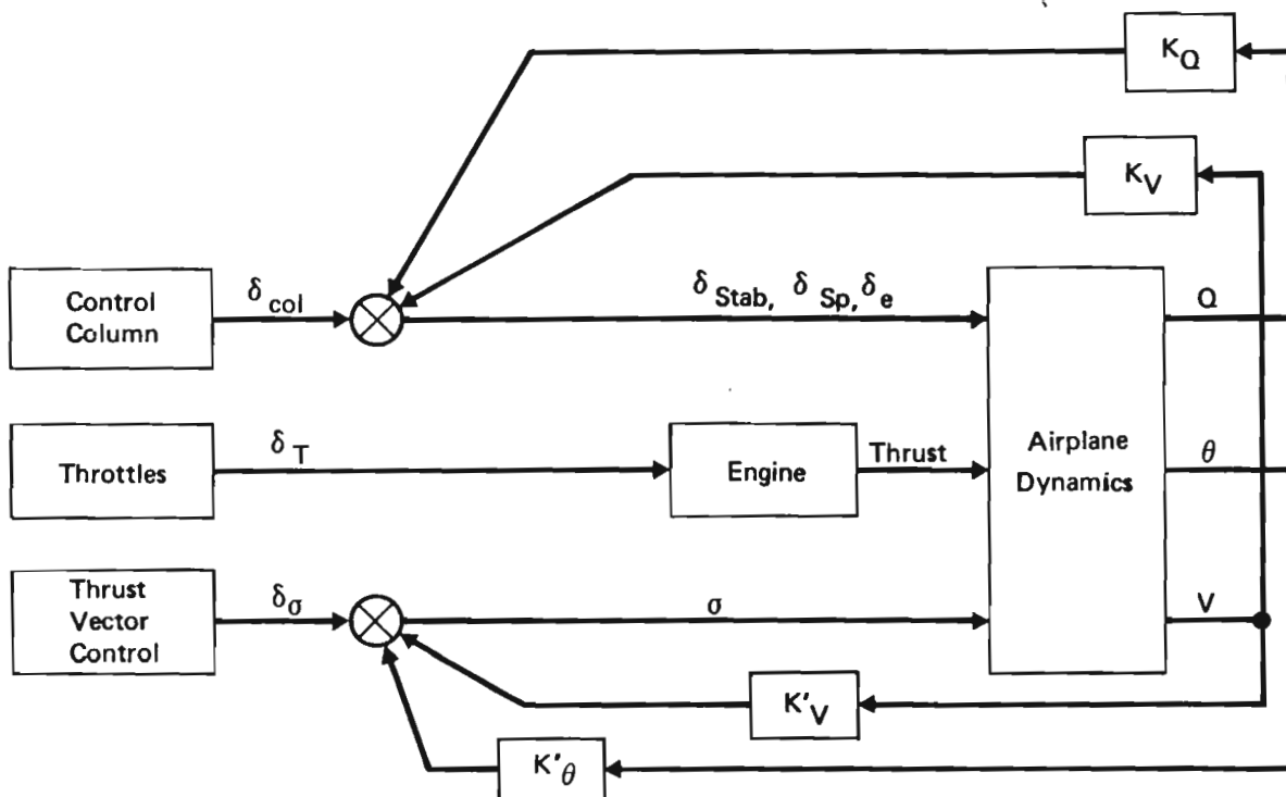
Figure 50: Longitudinal Control Augmentation System
