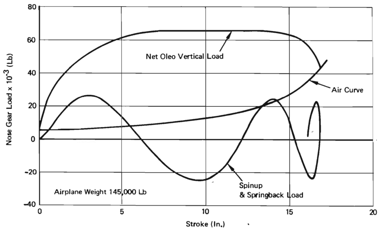
Figure 71: Nose Gear Landing Impact – 15 FPS
