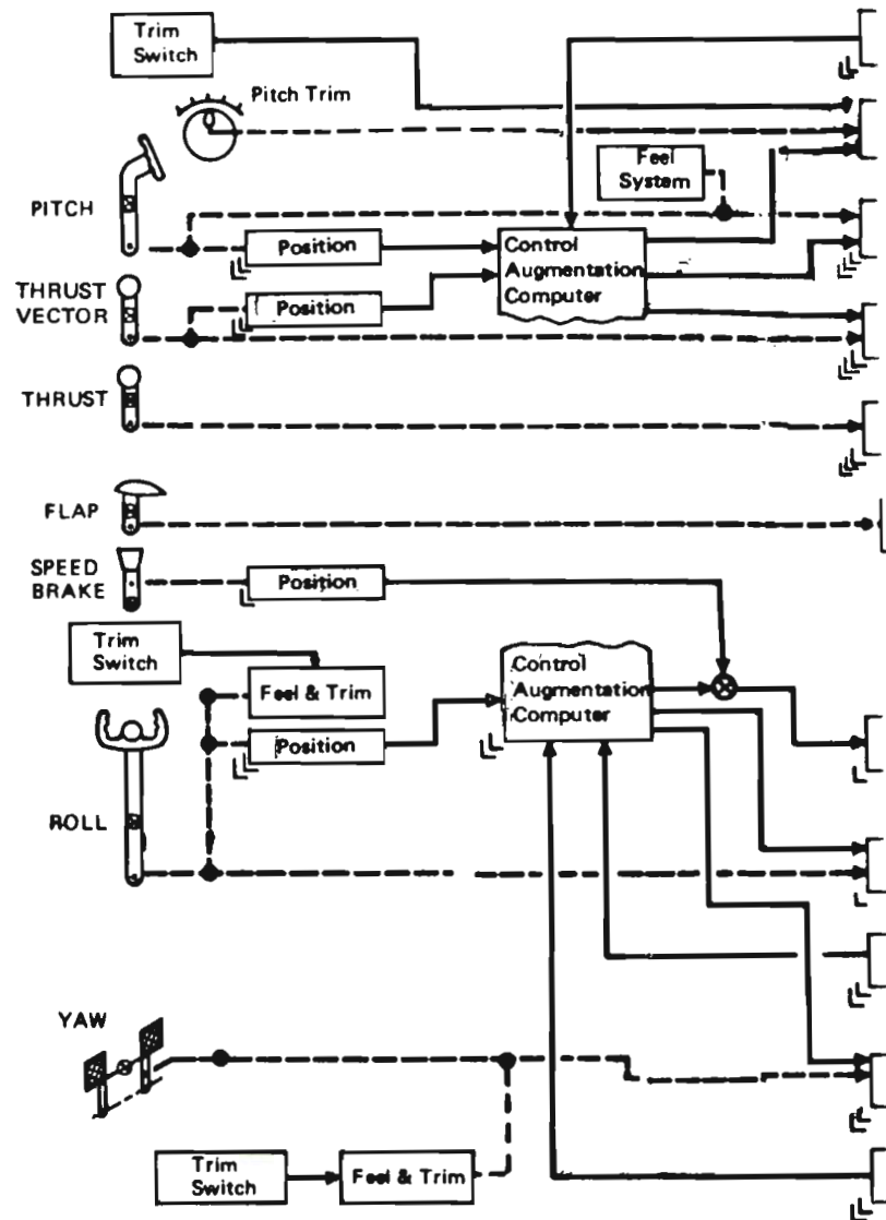
FLIGHT CONTROL SYSTEM
