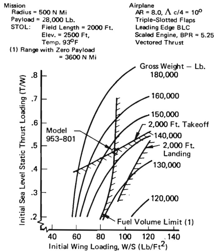
Figure 89: PARAMETRIC DESIGN CHART BASELINE AIRPLANE
