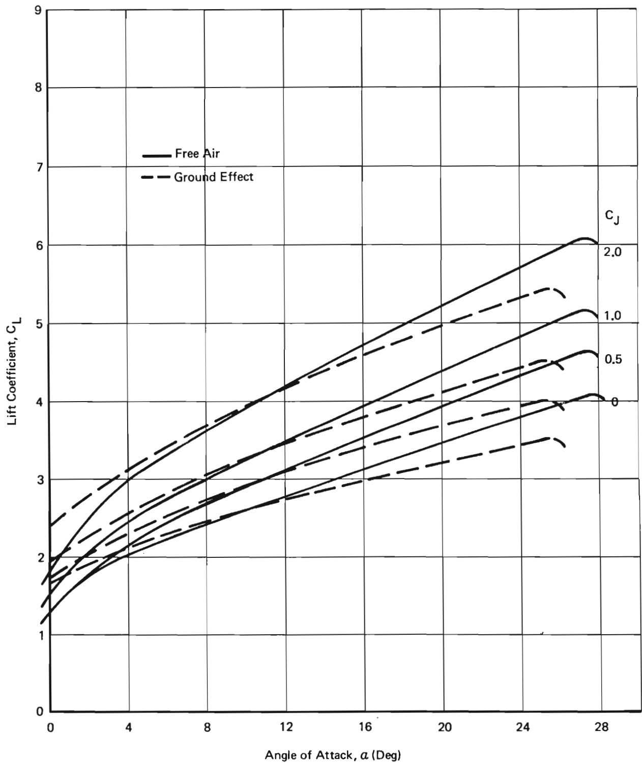
Figure 14: Trimmed Lift – All Engines Operating, Thrust Vector = 30^\circ
