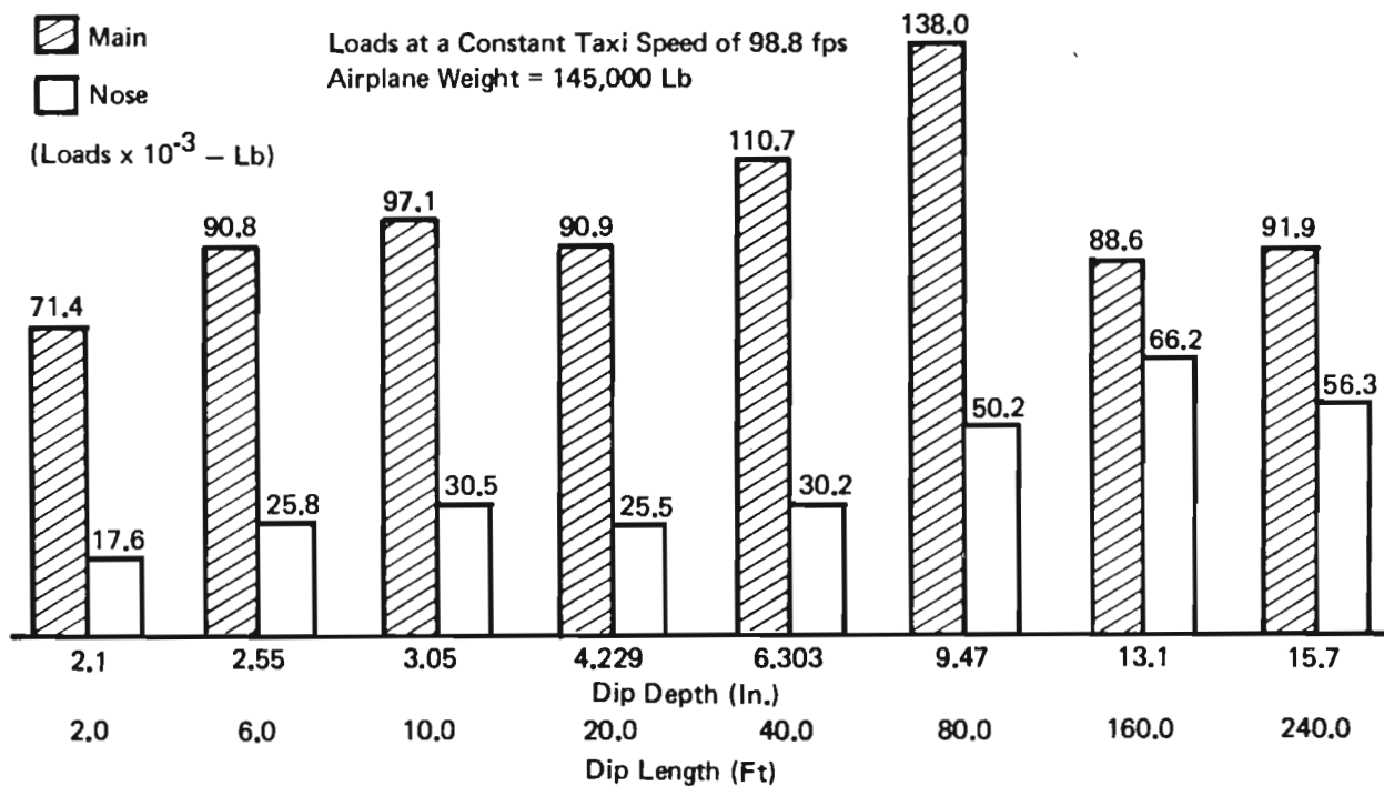
Figure 72: Taxi Loads – Varying Dip Constant Speed
