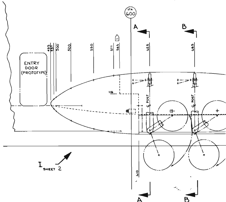
L SIDE VIEW
