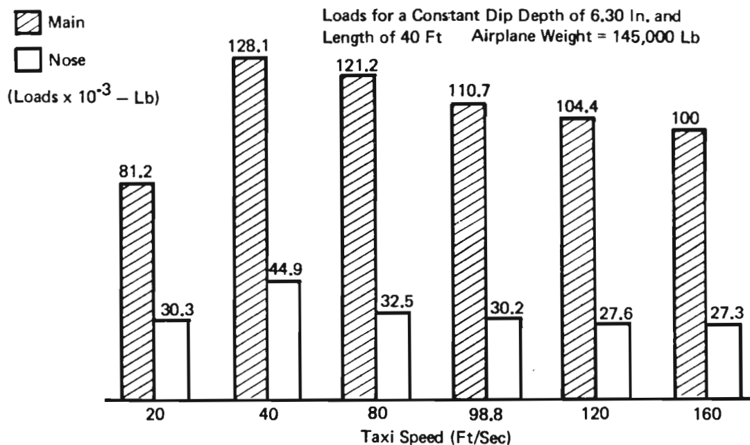
Figure 73: Taxi Loads – Speed Variation Constant Dip
