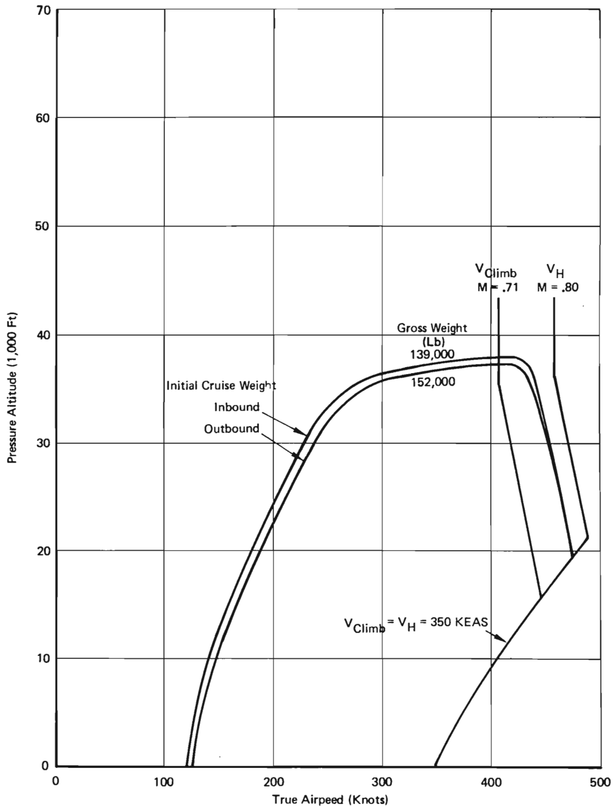
Figure 7: Speed – Altitude Envelope
