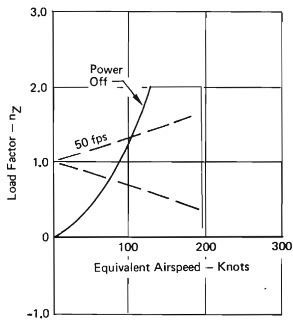
Figure 58: V-n Diagrams - Flaps Down
