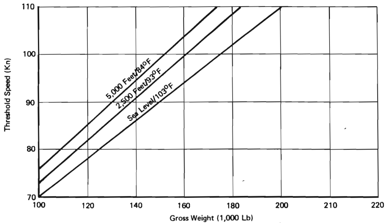
Figure 31: Normal Liftoff & Threshold Speeds – Hot Atmosphere
