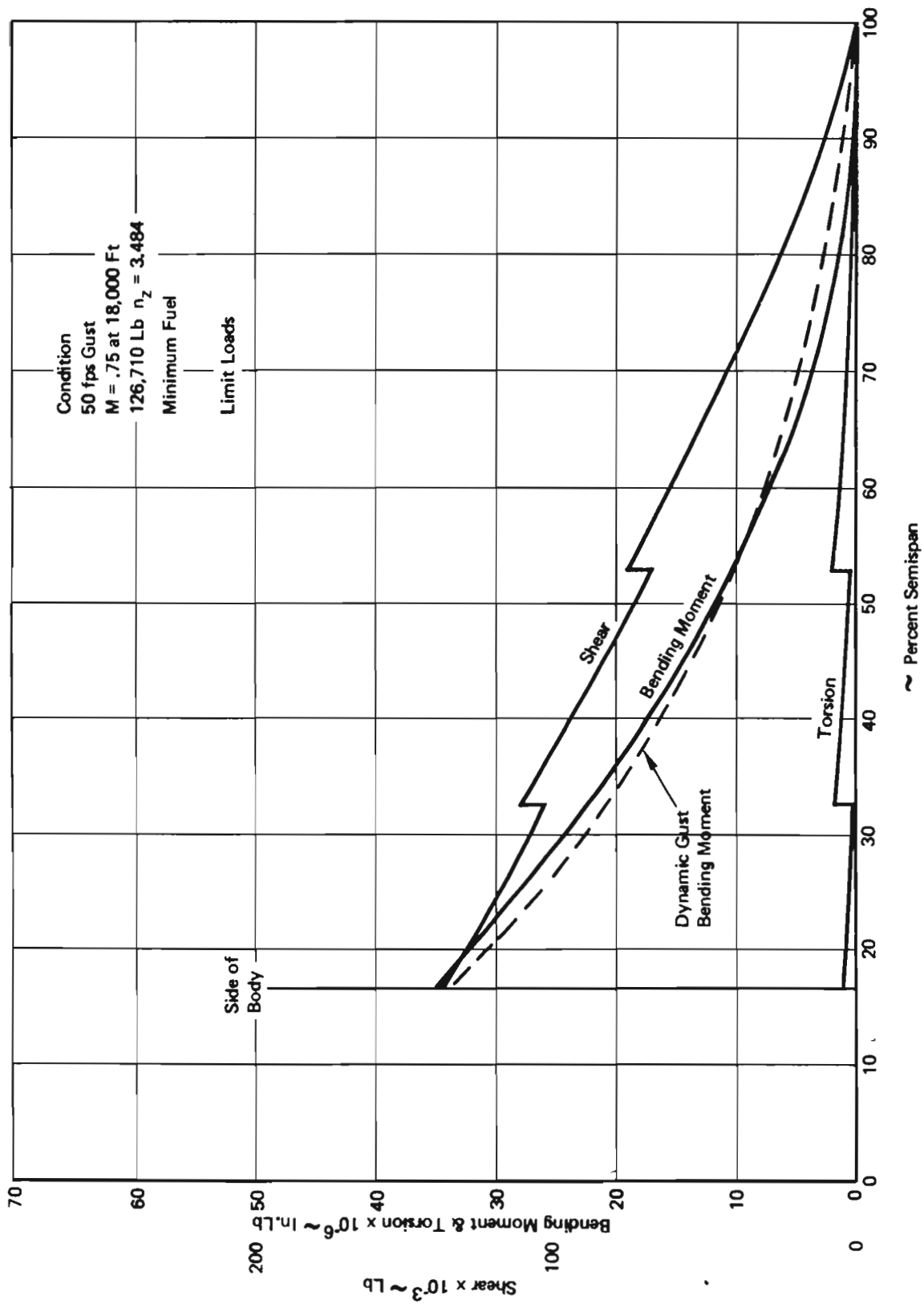
Figure 64: Wing Loads Maximum Bending
