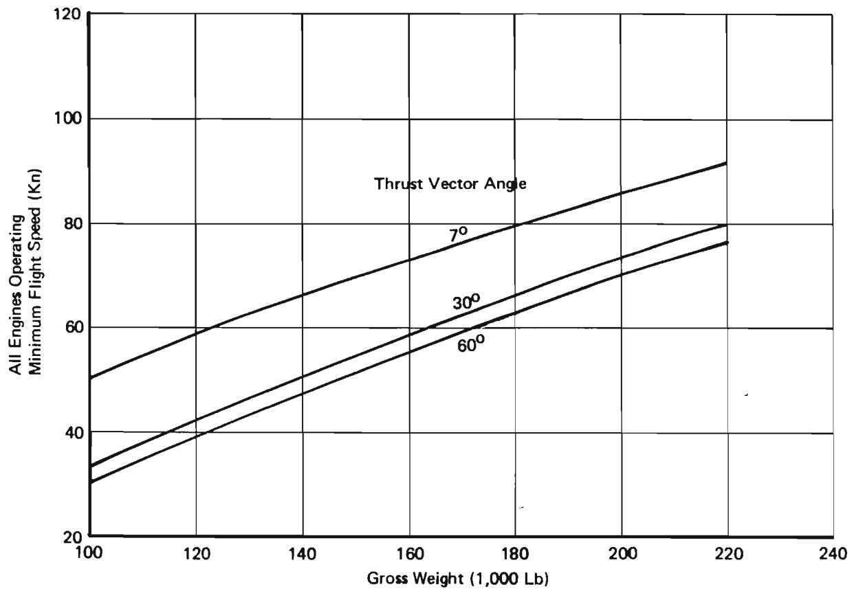
Figure 35: Minimum Flight Speeds – Sea Level Standard
