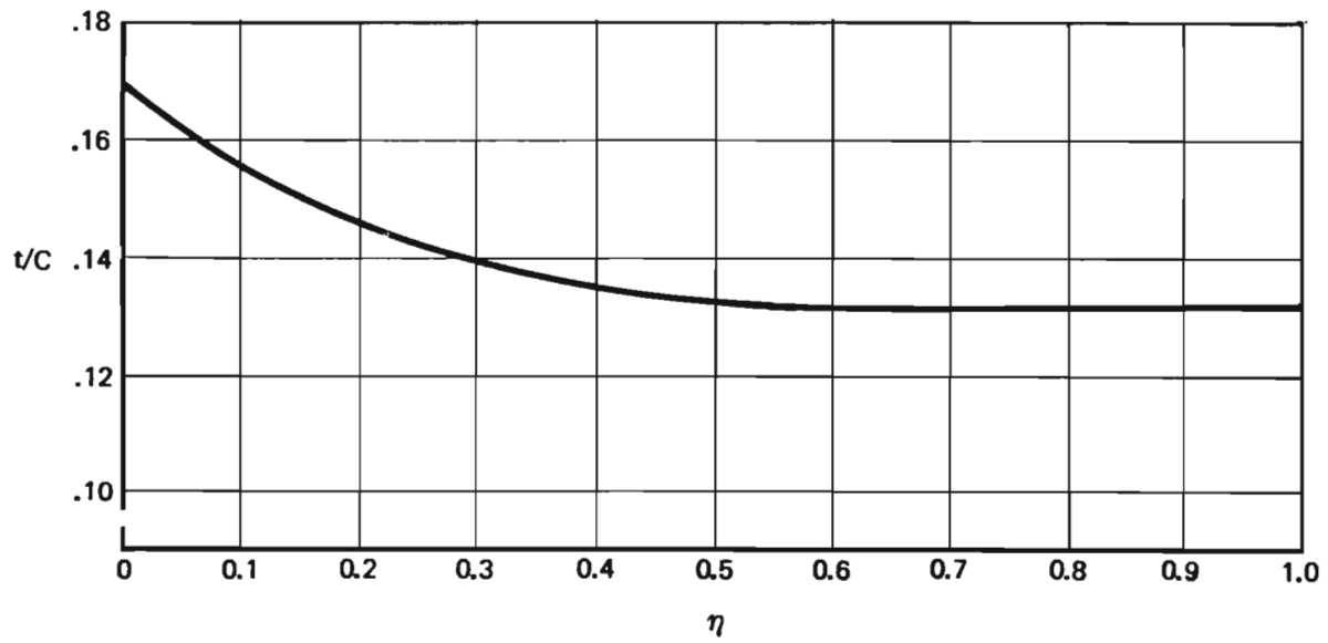
Figure 97: Wing Thickness Distribution
