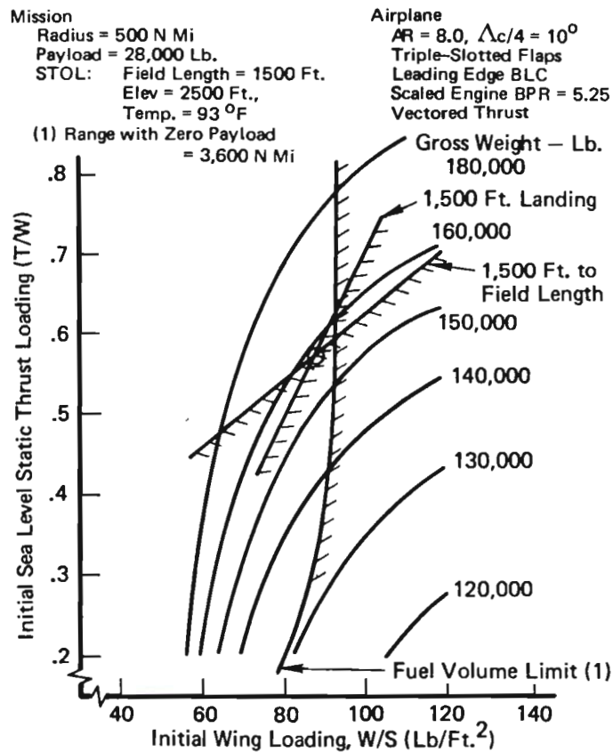
Figure 92: 1500 FT FIELD LENGTH TRADE
