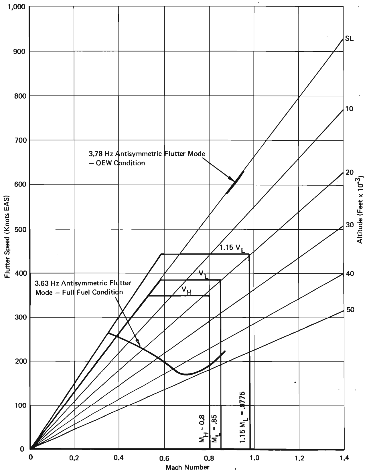
Figure 77: Comparison of Flutter Boundary to Structural Placard — Strength Design
