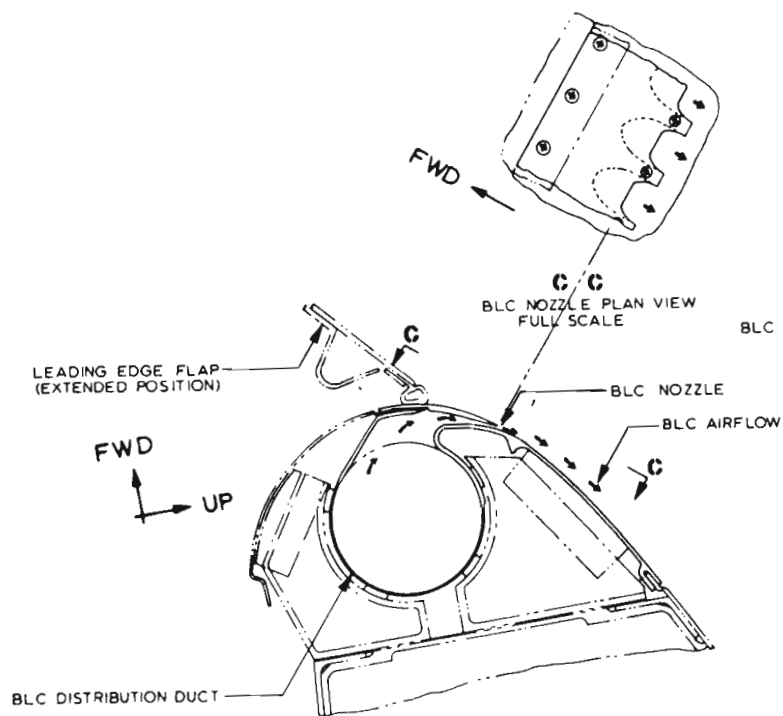
13 13 TYPICAL LEADING EDGE INSTL FULL SCALE
