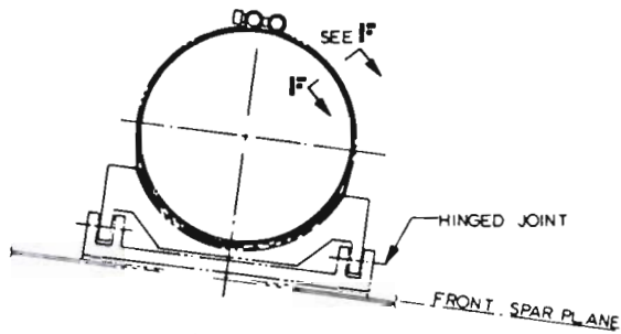
TYPICAL INTERMEDIATE DUCT SUPPORT 1/2 SCALE
