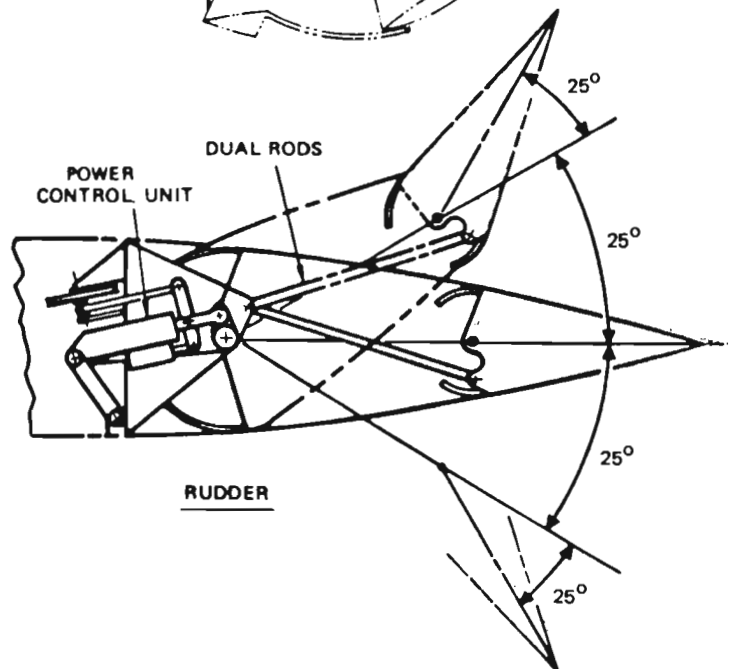
Figure 46: Primary Flight Control System
