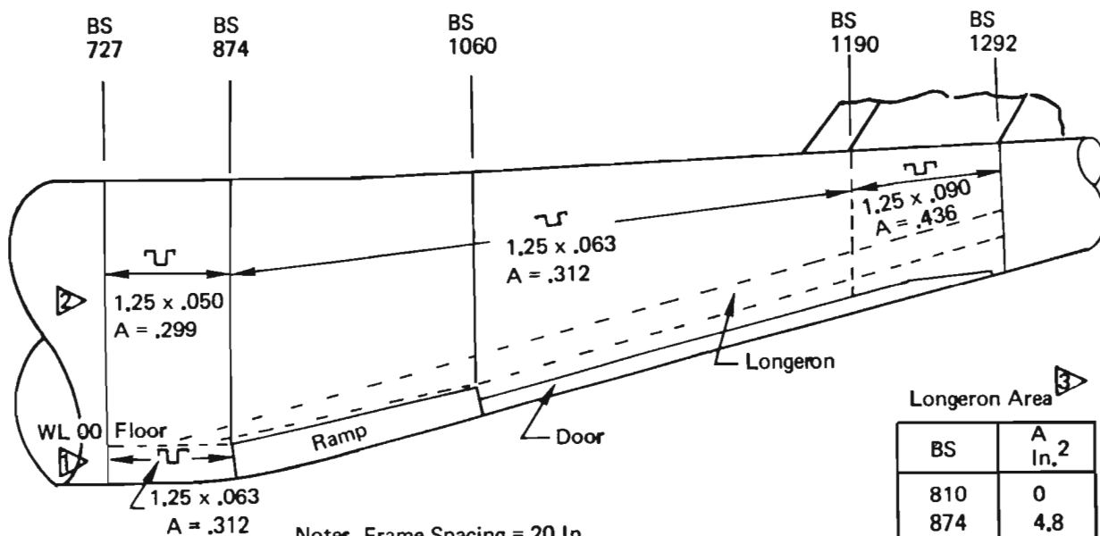
Figure 61 : Aft Body Skin Structural Requirements
