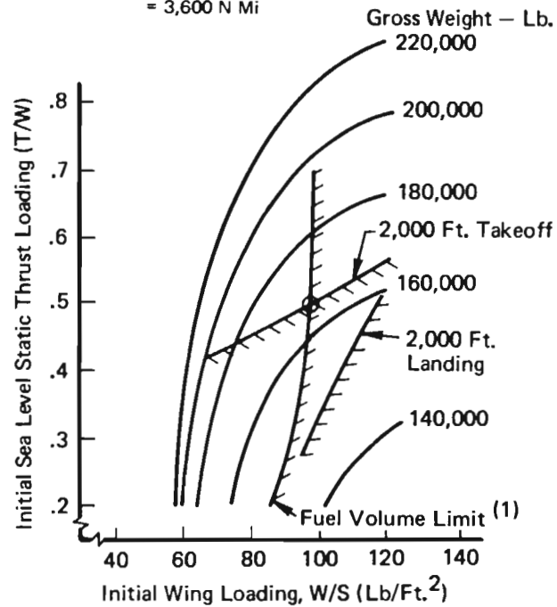
Figure 91: 750 N MI MISSION RADIUS TRADE
