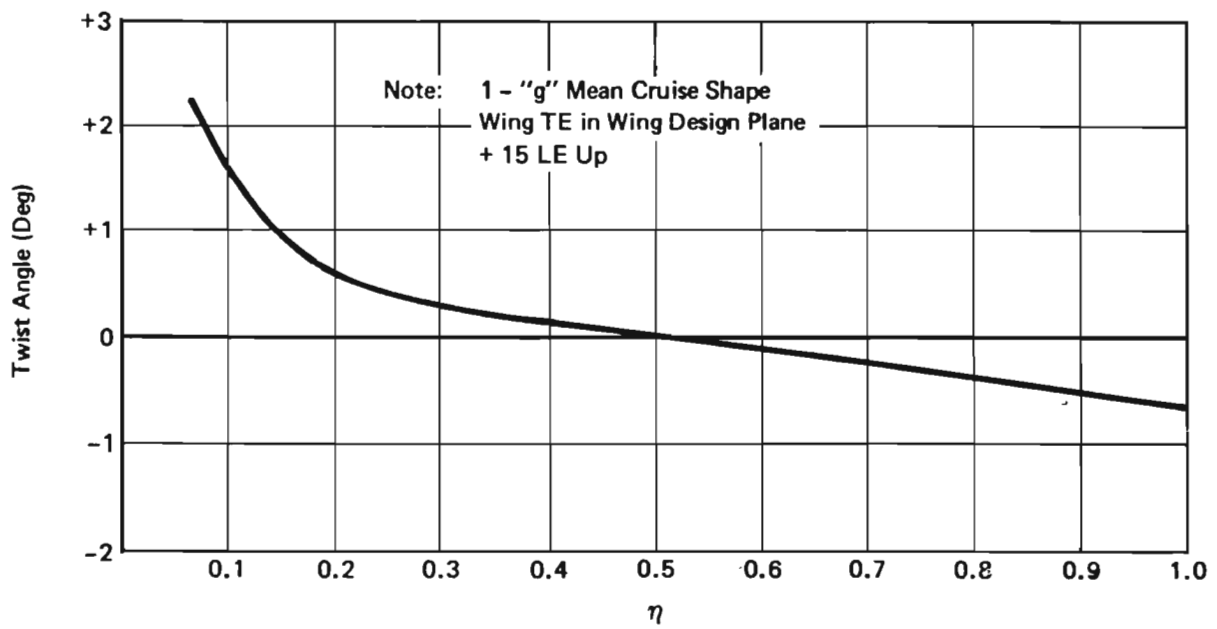
Figure 98: Wing Twist
