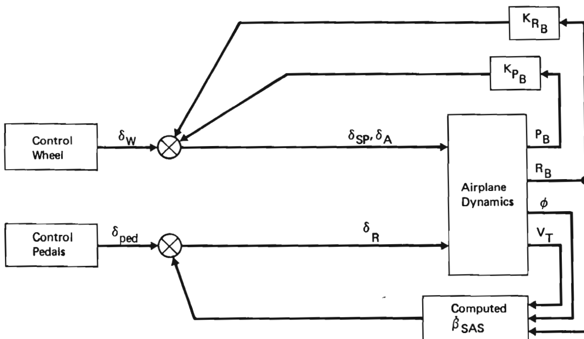
Figure 51: Lateral/Directional Control Augmentation System
