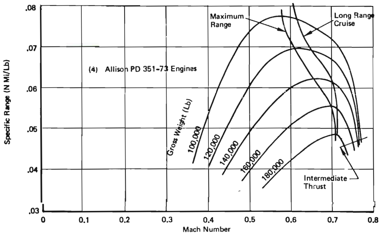
Figure 42: Fuel Mileage at 35,000 Feet – Standard Day
