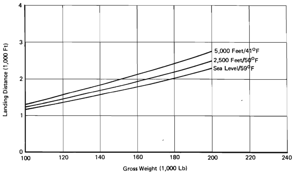
Figure 32: Normal Takeoff & Landing – Standard Atmosphere
