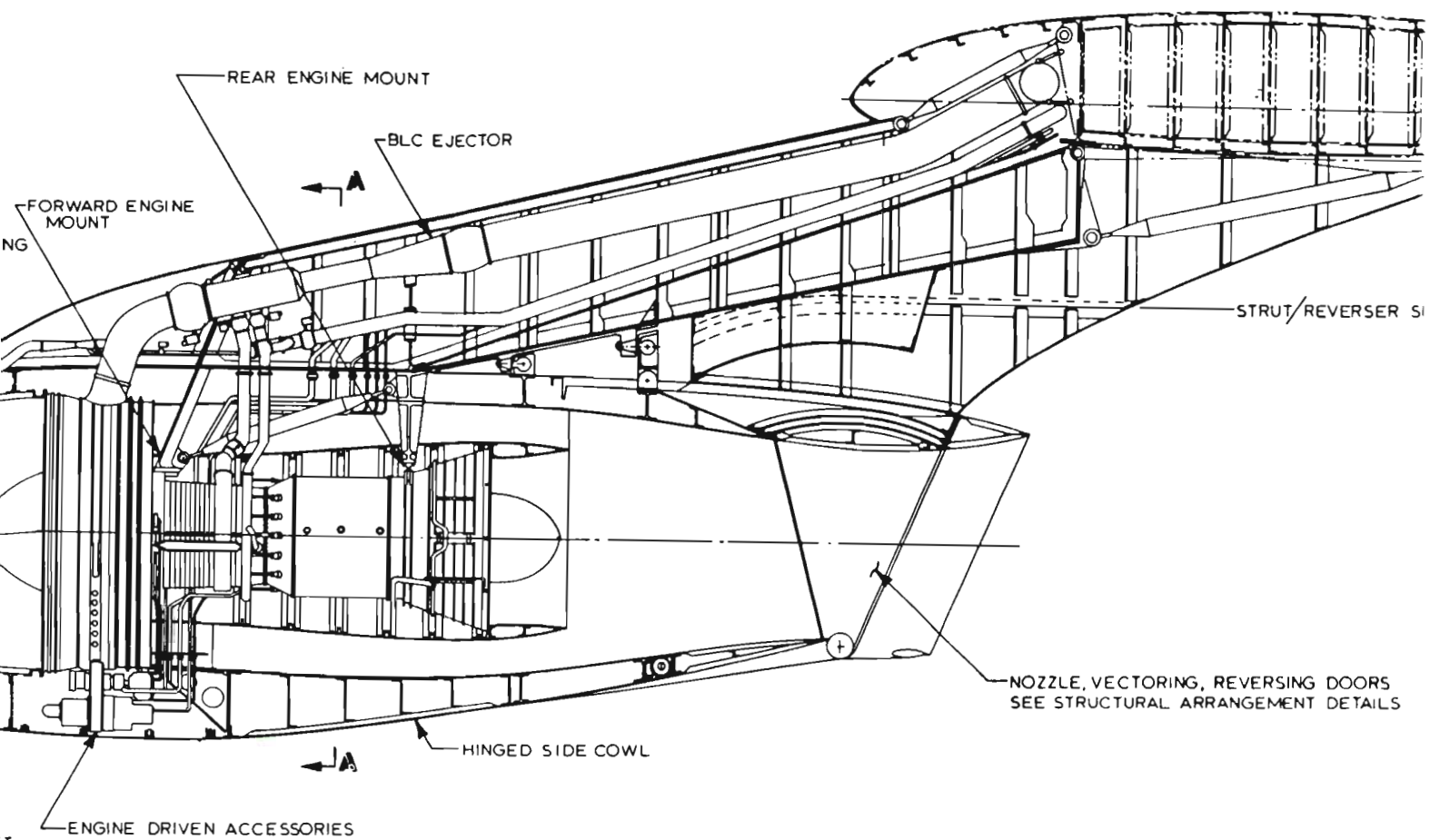
VIEW LOOKING AT ENGINE (NEAR SIDE COWLING REMOVED)
