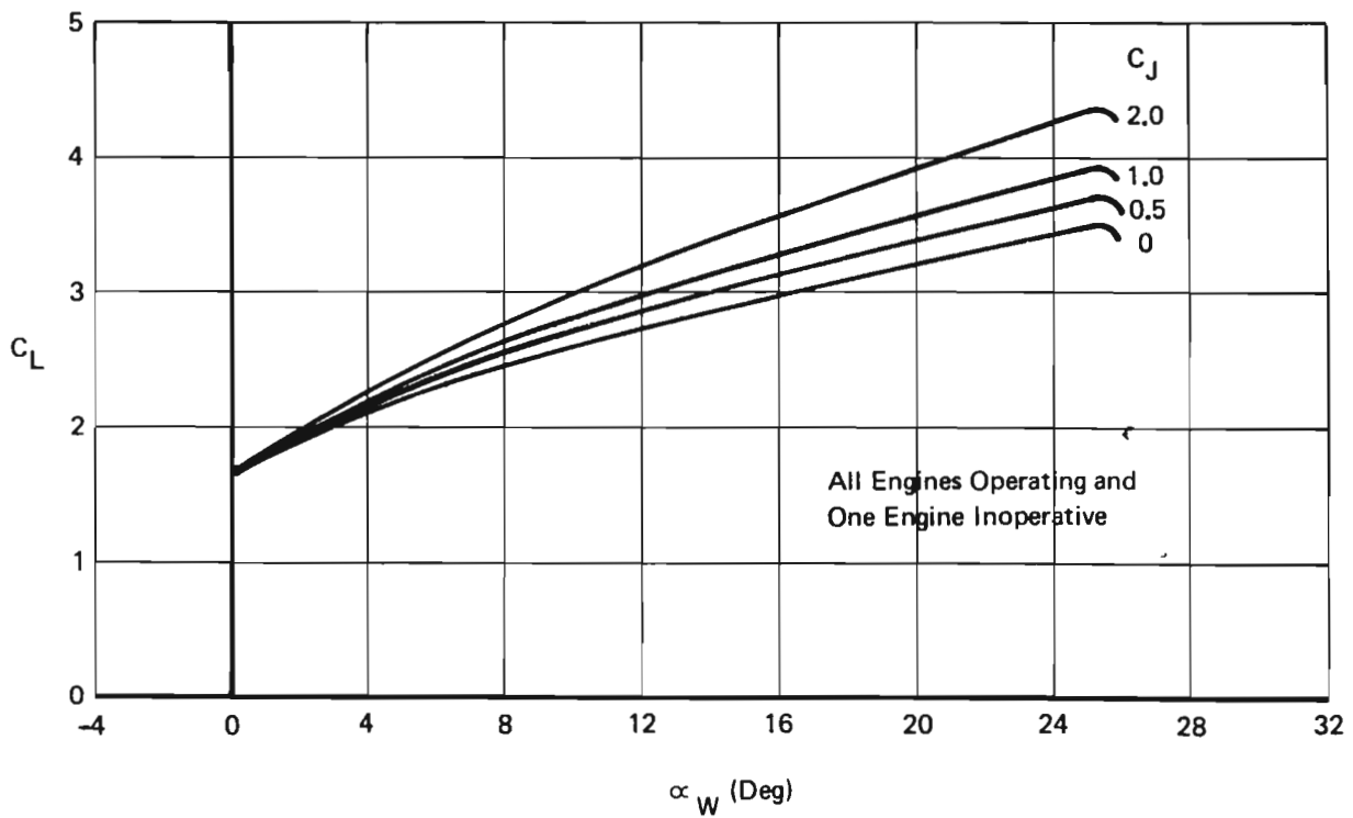
Figure 12: Trimmed Lift – Ground Effect, Thrust Vector = 0^\circ
