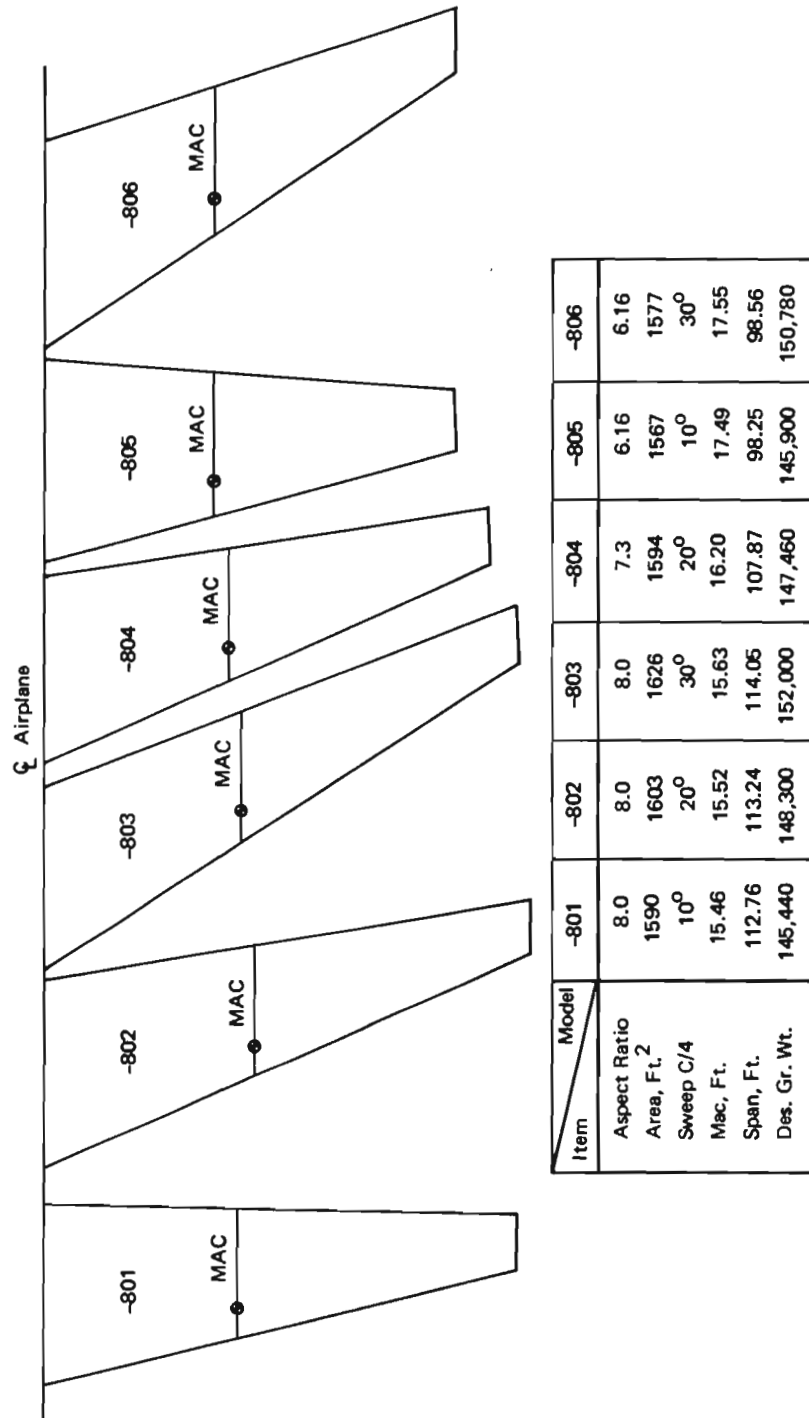
Figure 87: WING PLANFORM PARAMETRIC STUDY CONFIGURATIONS
