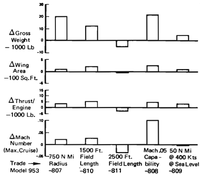
Figure 90: INCREMENTAL EFFECTS OF TRADES ON BASELINE PARAMETERS
