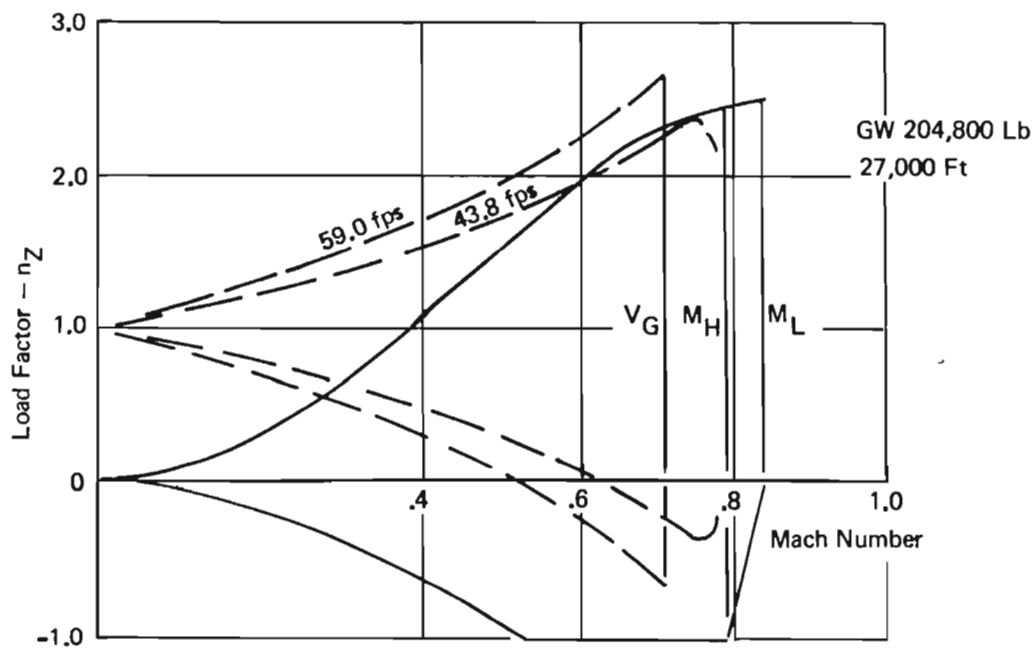
Figure 56: V-n Diagrams - Basic Flight Design Weight - C_{Transport}
