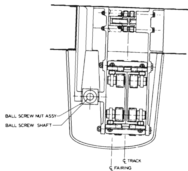
SECTION A-A (FLAP UP)
