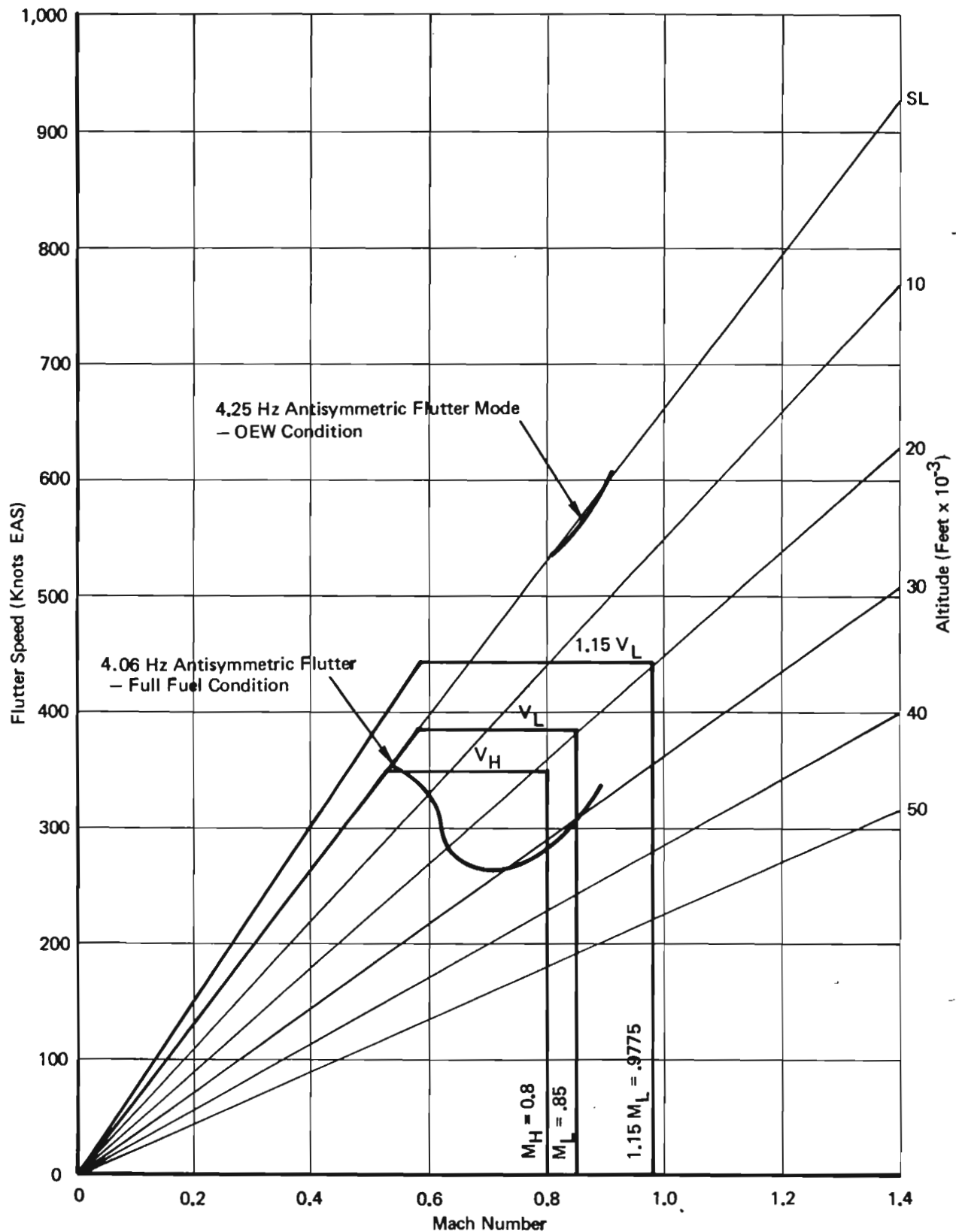
Figure 78: Comparison of Flutter Boundary to Structural Placard – Uniformly Stiffened Wing
