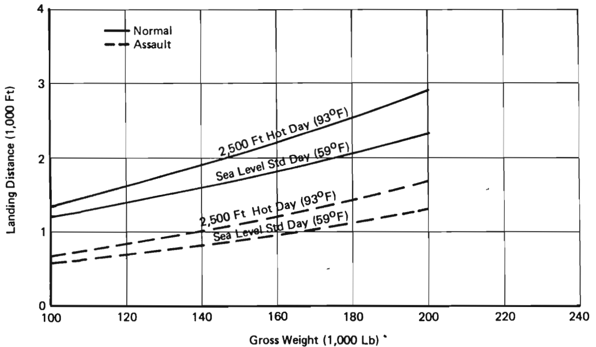
Figure 6 : Takeoff and Landing Distance Summary
