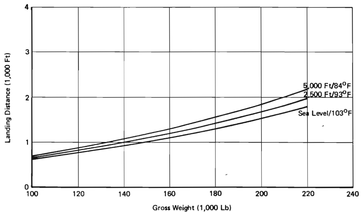
Figure 33: Assault Takeoff and Landing – Hot Atmosphere
