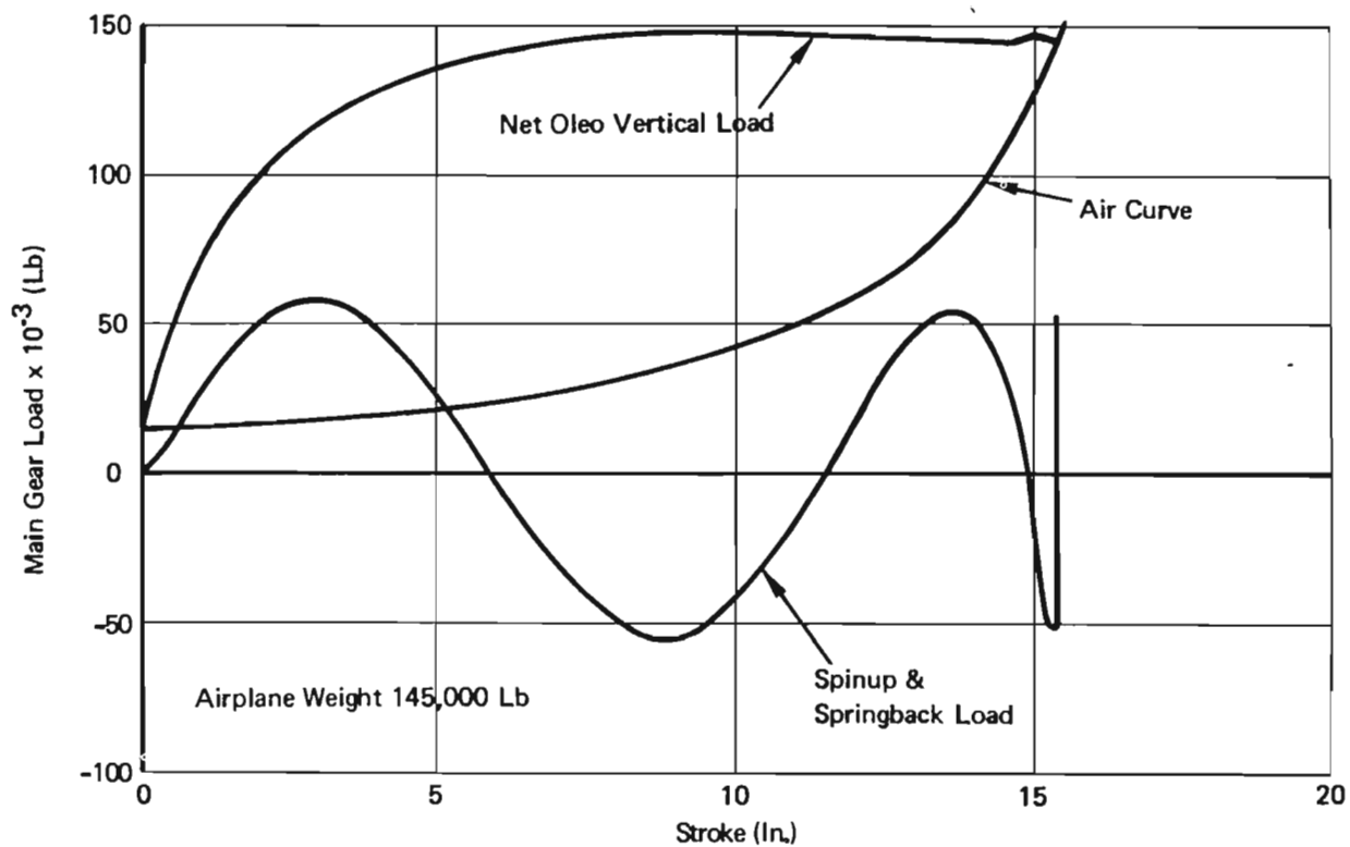
Figure 70: Main Gear Landing Impact – 15 FPS
