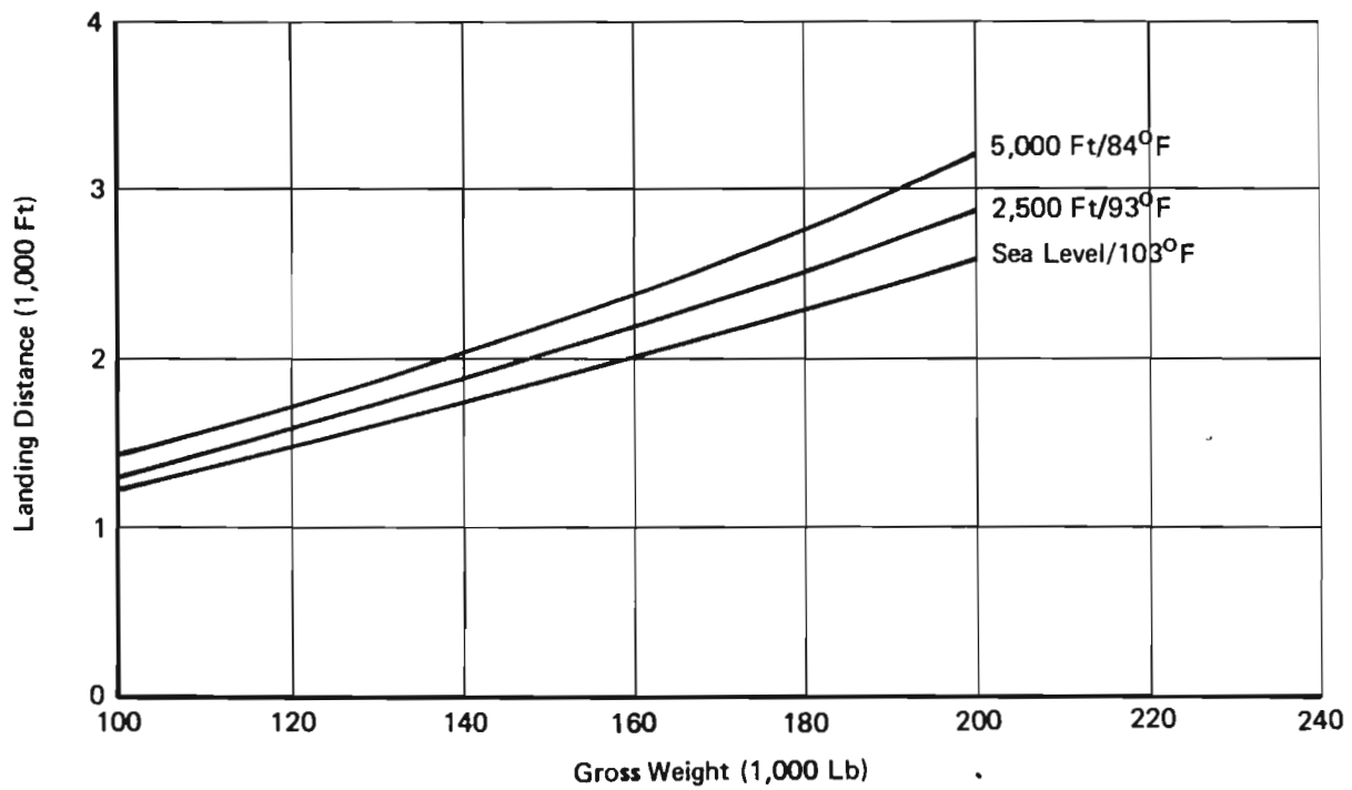
Figure 29: Normal Takeoff & Landing – Hot Atmosphere
