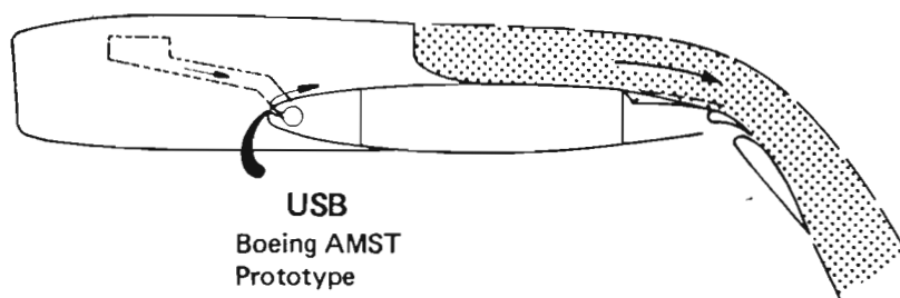
Figure 83: Powered Lift STOL Concepts
