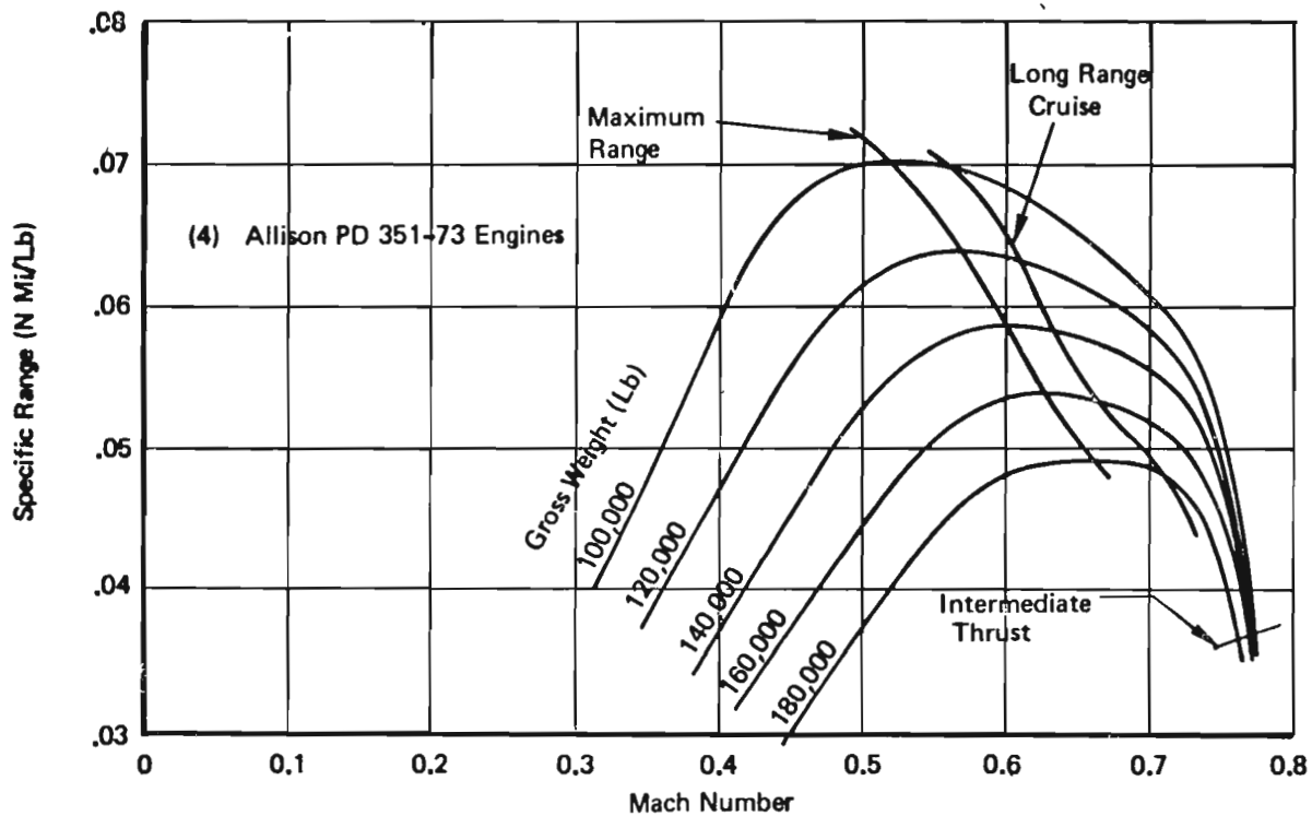
Figure 41: Fuel Mileage at 30,000 Feet – Standard Day
