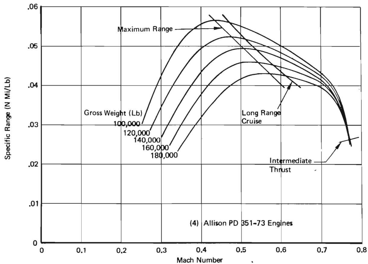
Figure 40: Fuel Mileage at 20,000 Feet – Standard Day
