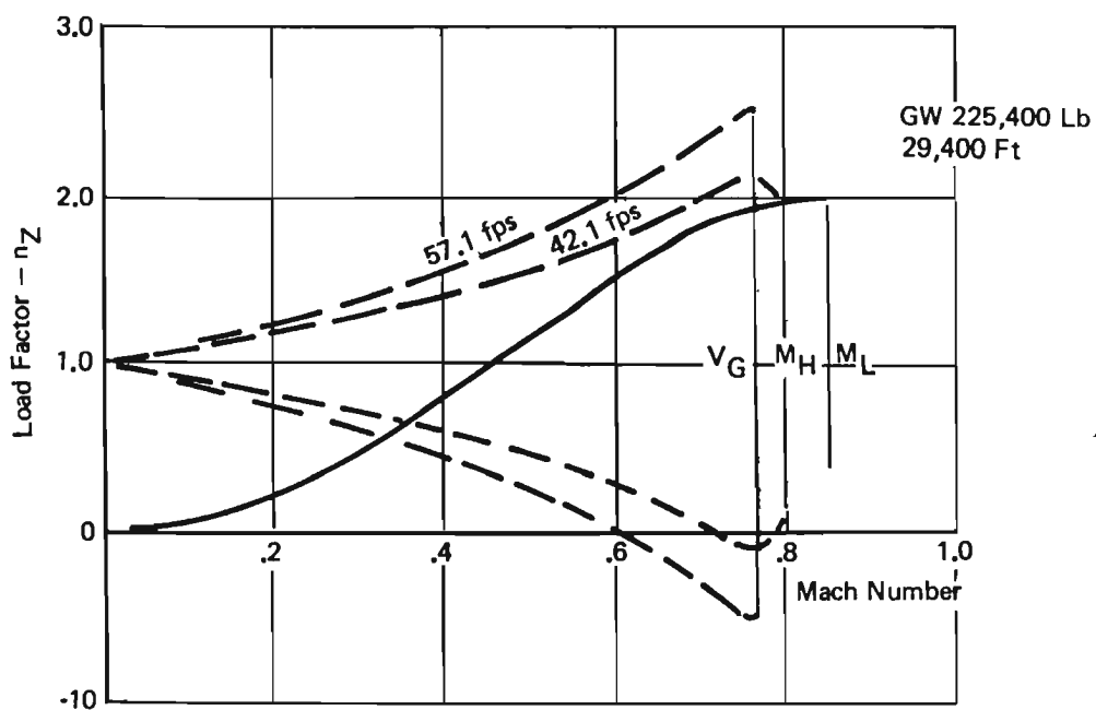
Figure 55: V-n Diagrams — Maximum Gross Weight
