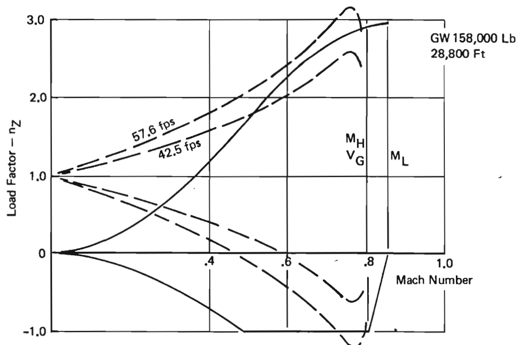
Figure 57: V-n Diagrams - Basic Flight Design Weight - C_{Assault}
