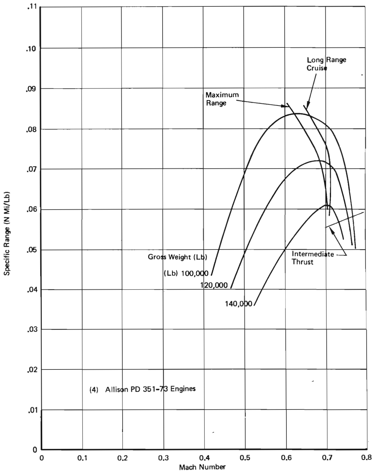
Figure 43: Fuel Mileage at 40,000 Feet – Standard Day
