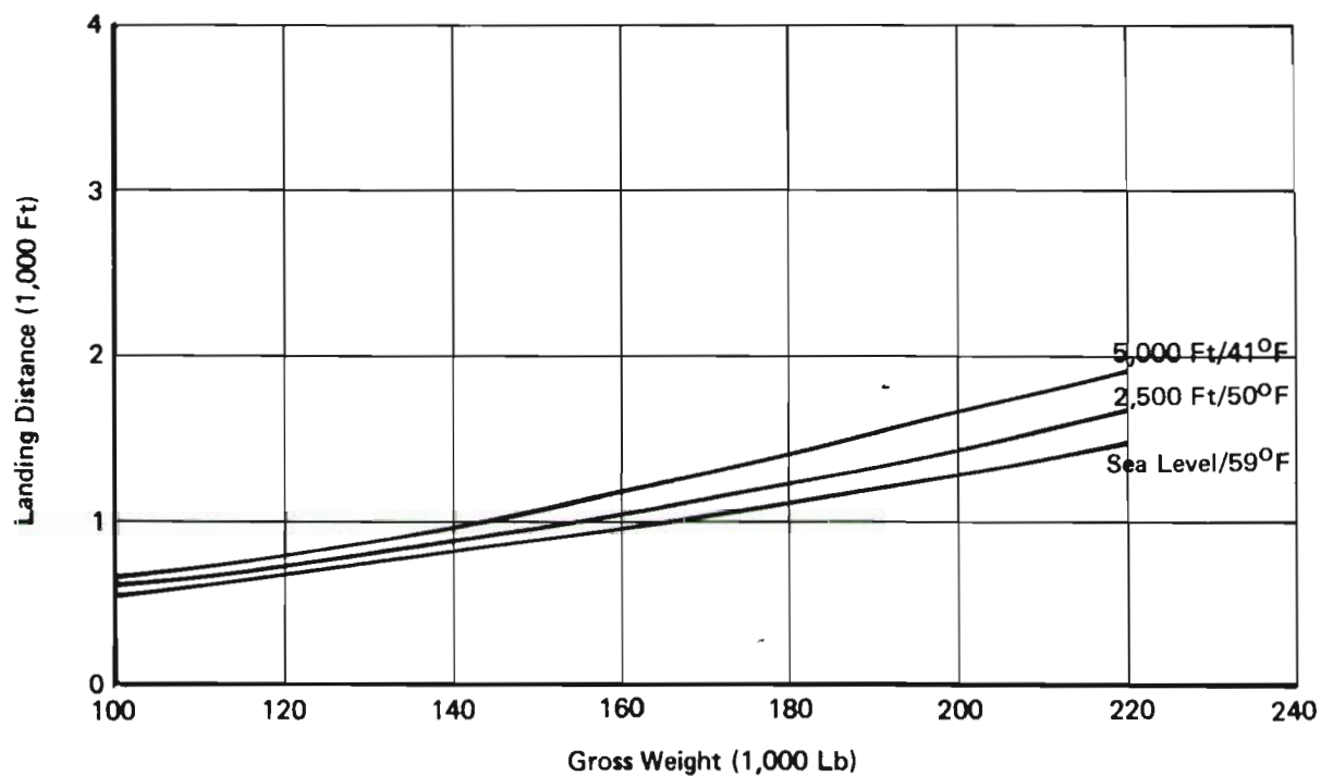
Figure 34: Assault Takeoff and Landing – Standard Atmosphere
