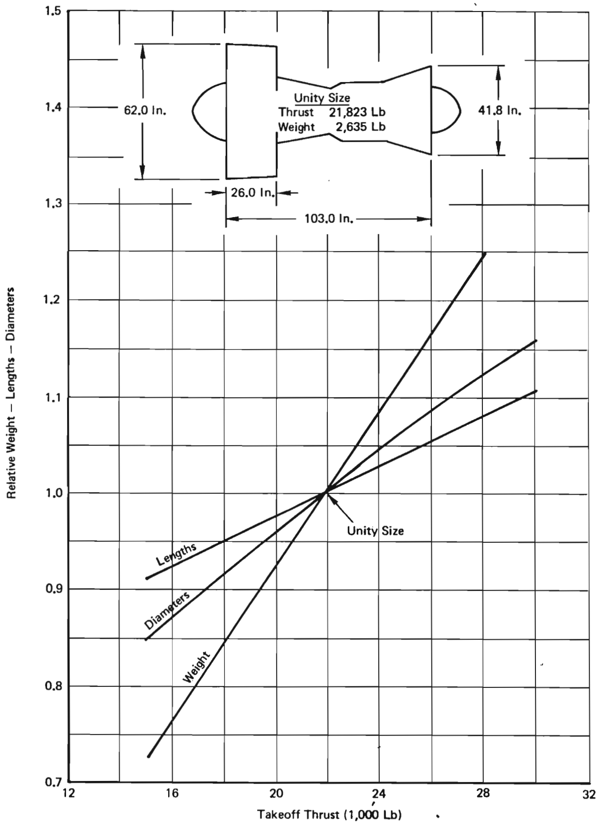
Figure 20: Engine Sizing Chart
