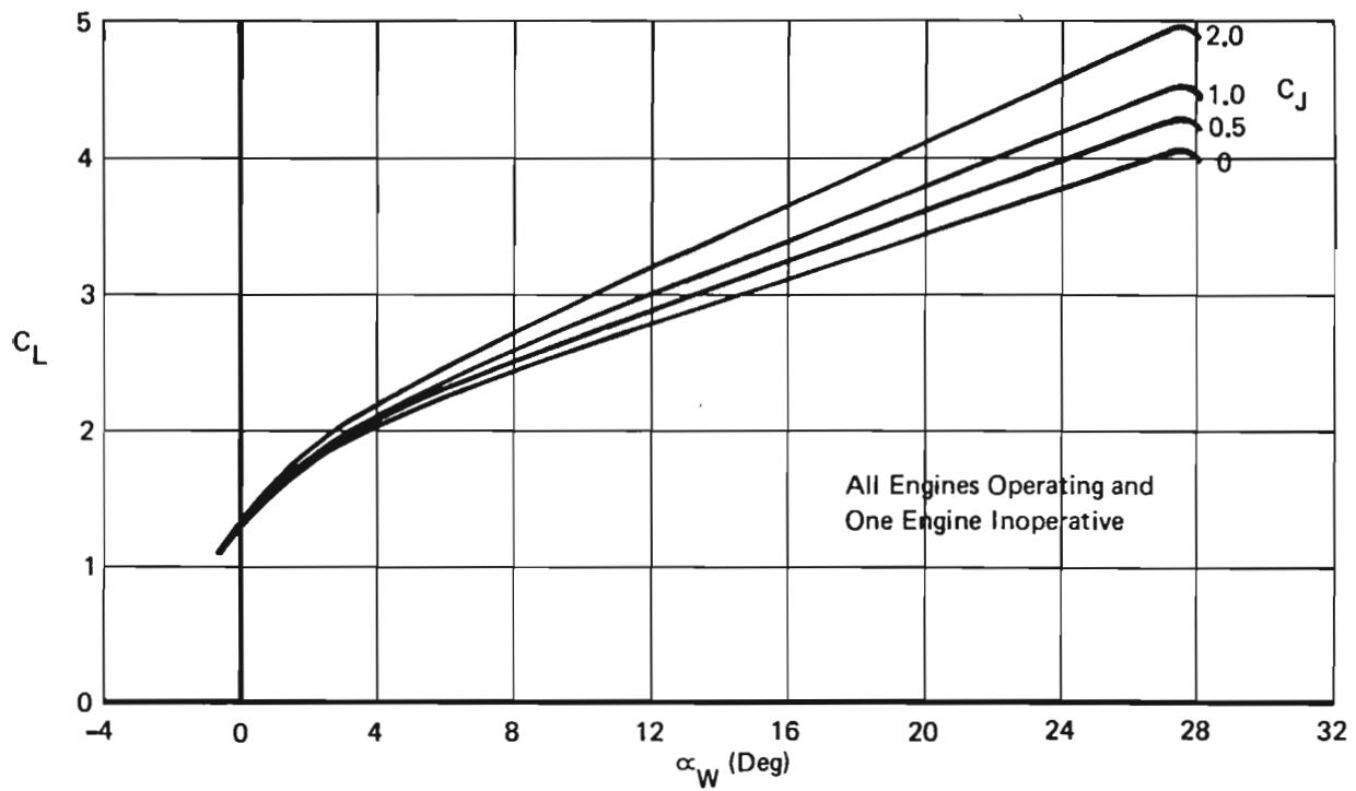
Figure 11: Trimmed Lift – Free Air, Thrust Vector = 0^\circ
