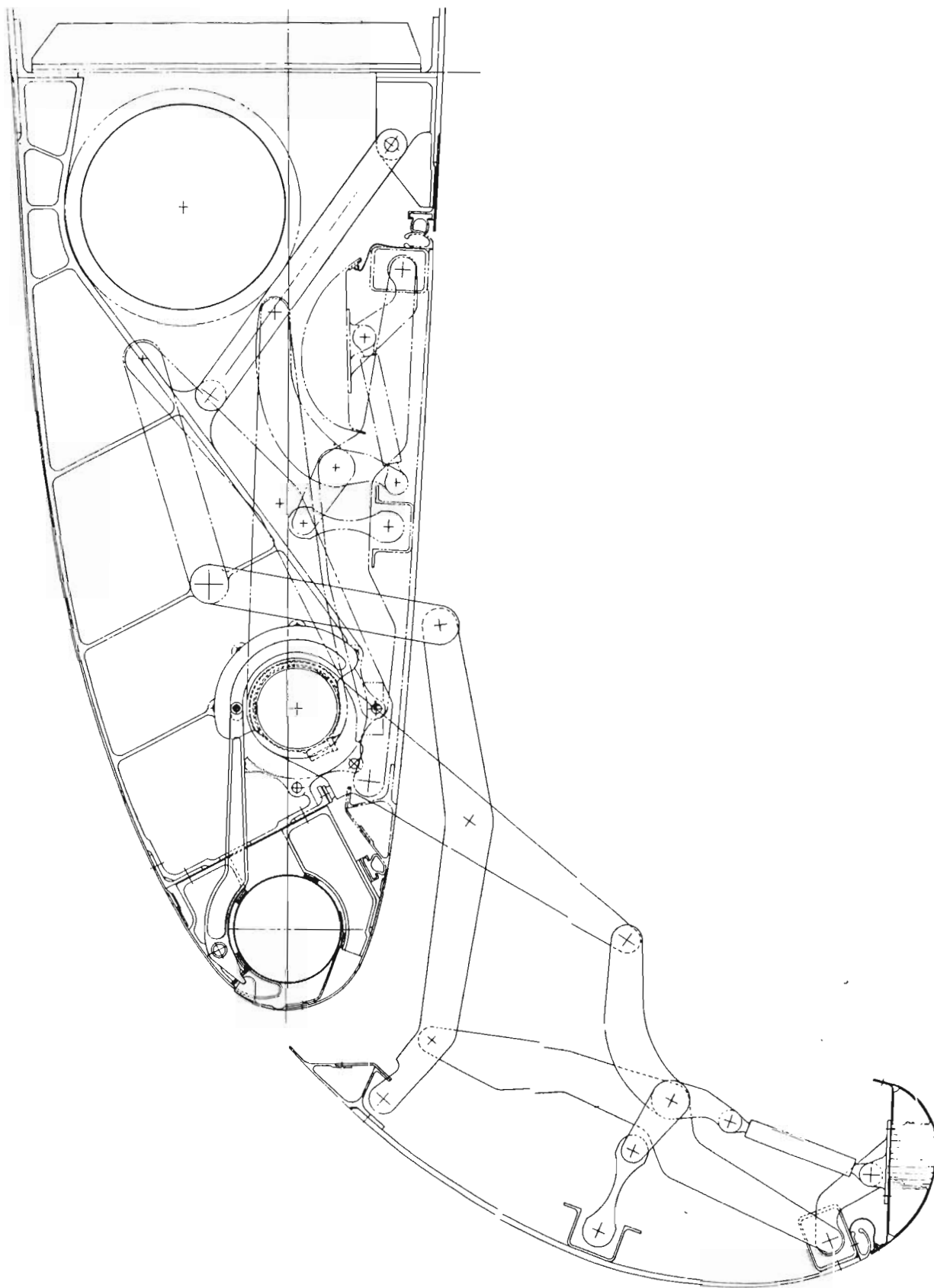
Figure 103: Leading Edge Flap Mechanization
