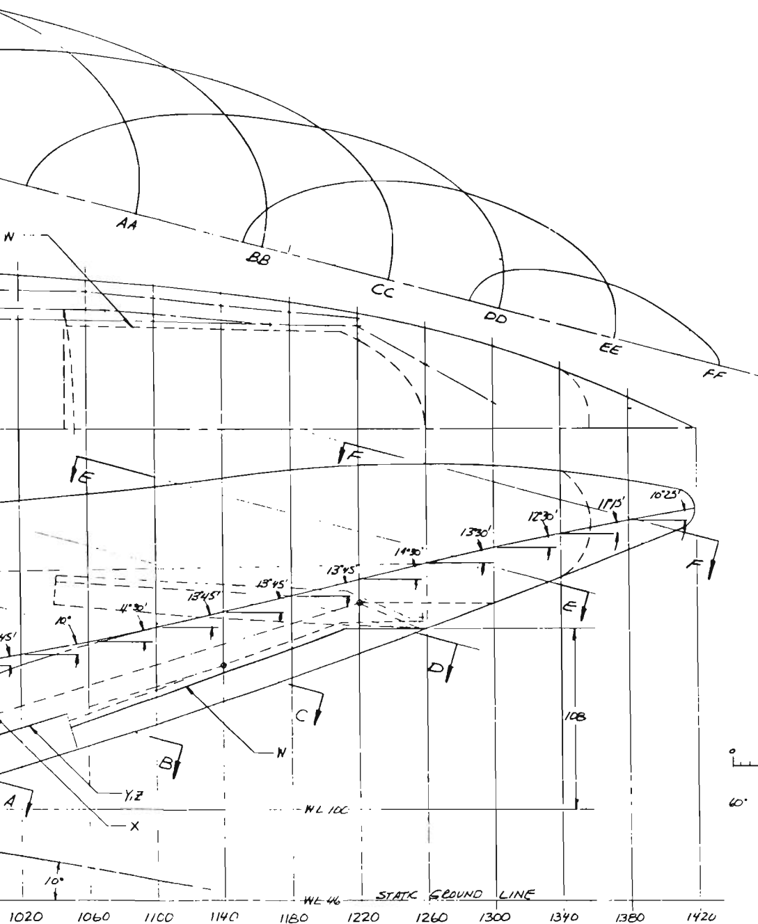
Figure 106: Aft Body Loft
