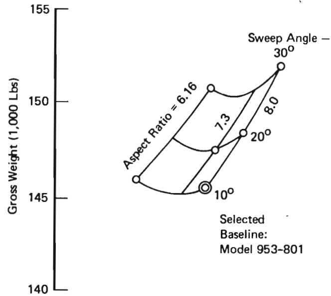
Figure 88: PLANFORM STUDY – RESULTS
