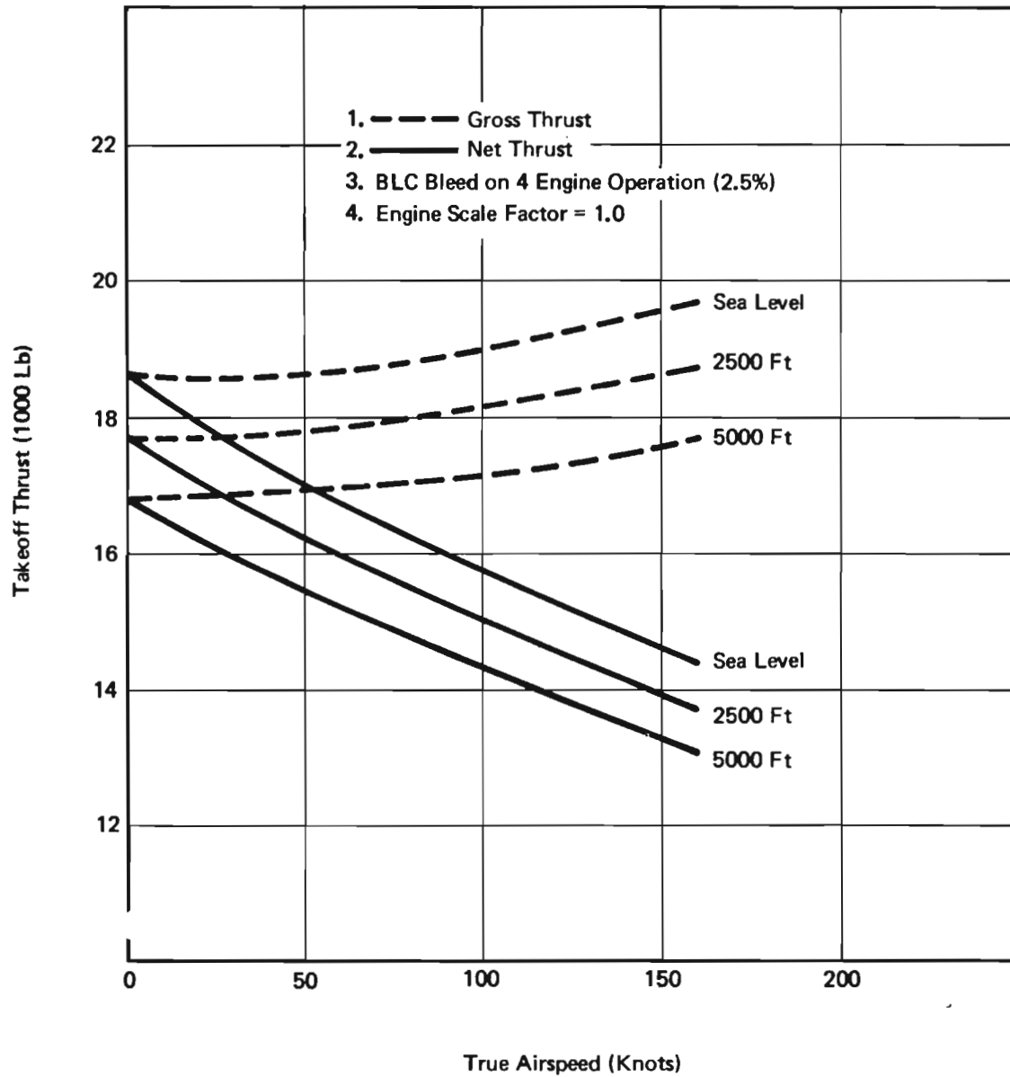
Figure 22: PD 351-73 Takeoff Thrust – Hot Day
