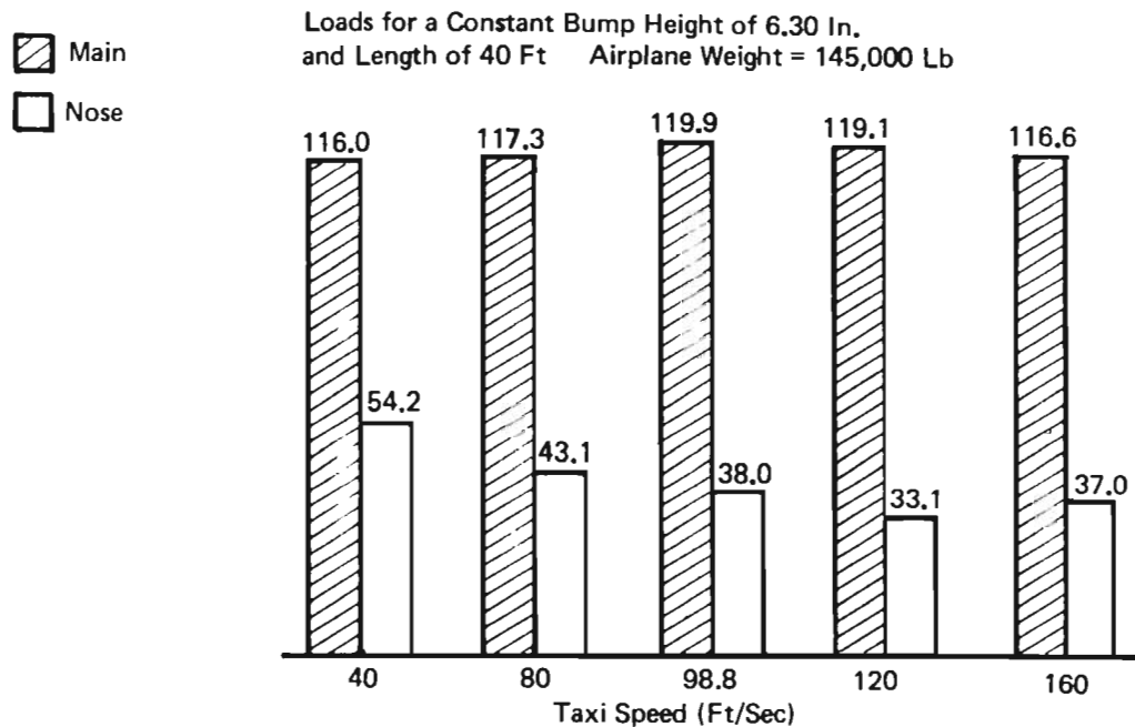
Figure 75: Taxi Loads – Speed Variation – Constant Bump
