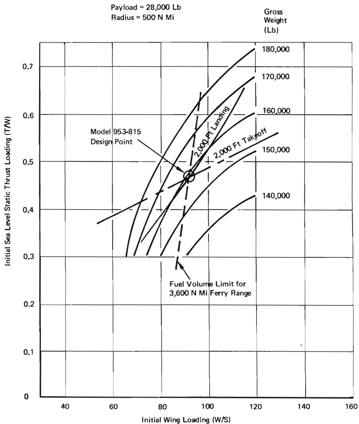
Figure 8: Parametric Design – Model 953-815
