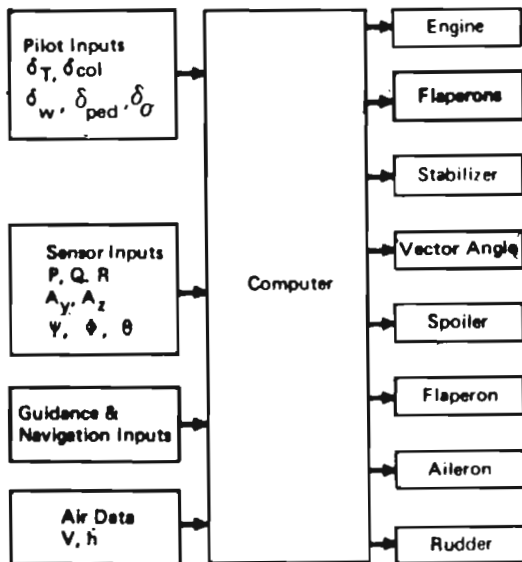
AUTOMATIC FLIGHT CONTROL SYSTEM (AFCS)
