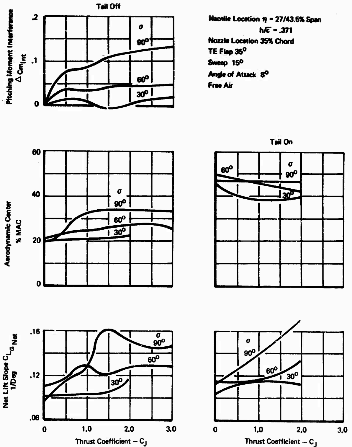
Figure 97: Effect of Thrust on Longitudinal Stability \Lambda = 30^\circ
