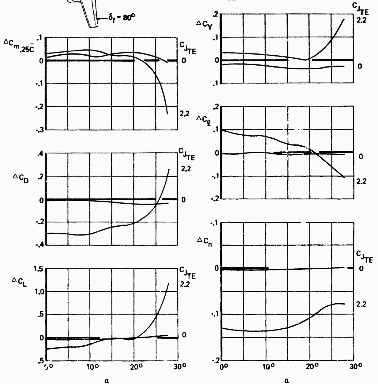
Figure 146: Jet Flap Aileron
