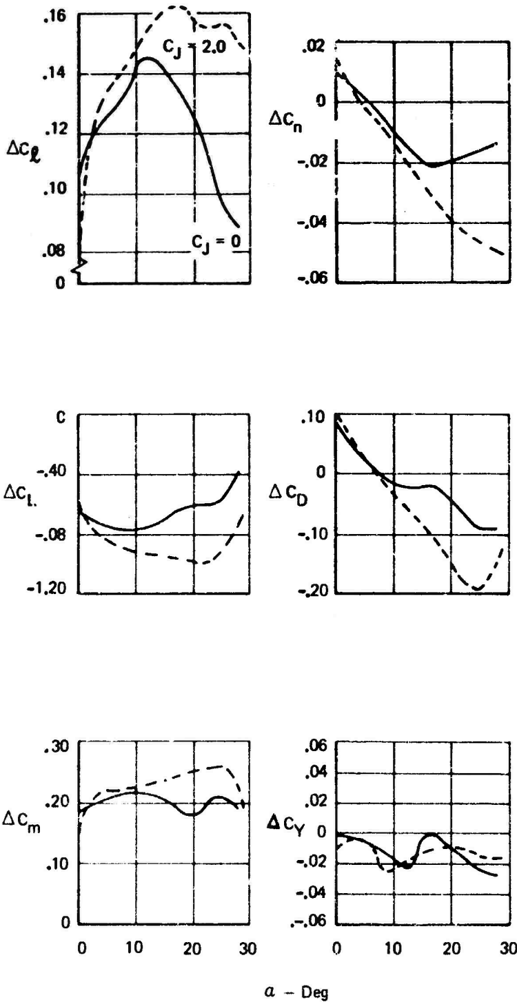
Figure 135: Spoiler Effectiveness
