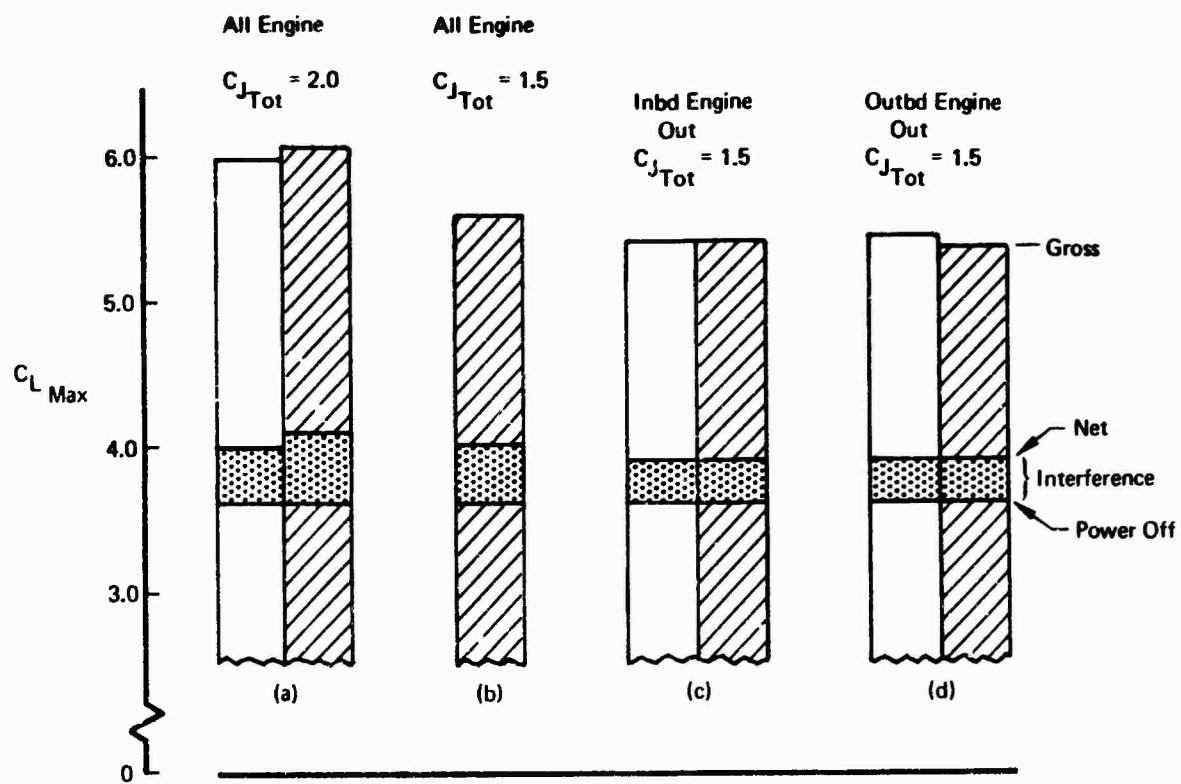
Figure 87: Effect of an Engine Failure on C_{L Max}
