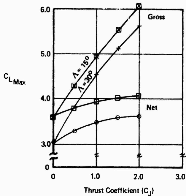
Figure 90: Comparison of C_{LMax} for 15^\circ and 30^\circ Wing Sweep
