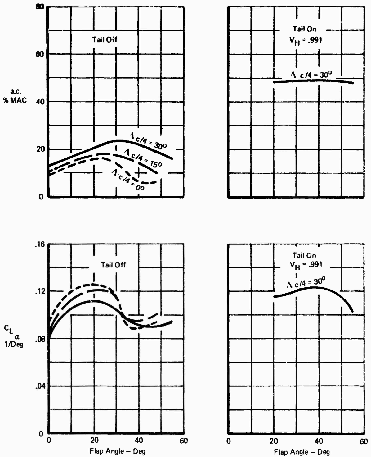
Figure 20: Lift Curve Slope and Aerodynamic Center – Effect of Trailing Edge Flap Angle
