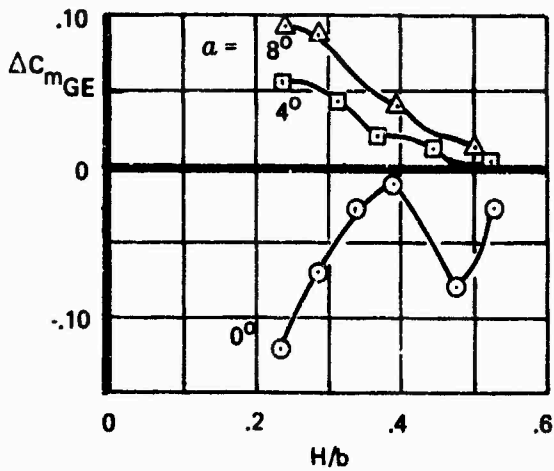
Figure 74: Effect of Ground Height on Longitudinal Characteristics
