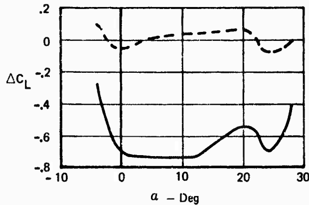
Figure 136: Lateral Control – Combined Aileron and Spoiler
