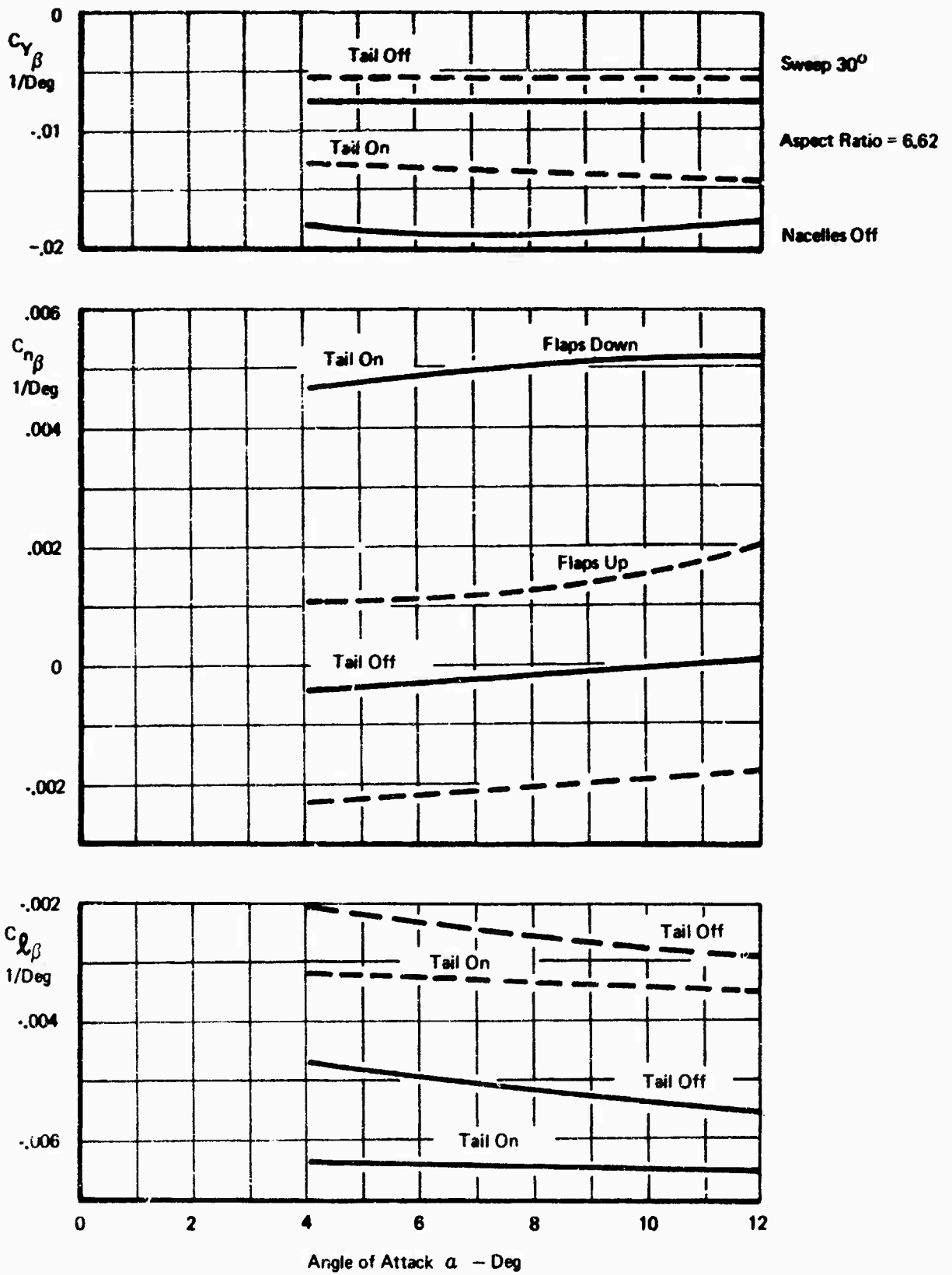
Figure 31: Effect of Tail - \beta Stability Derivatives
