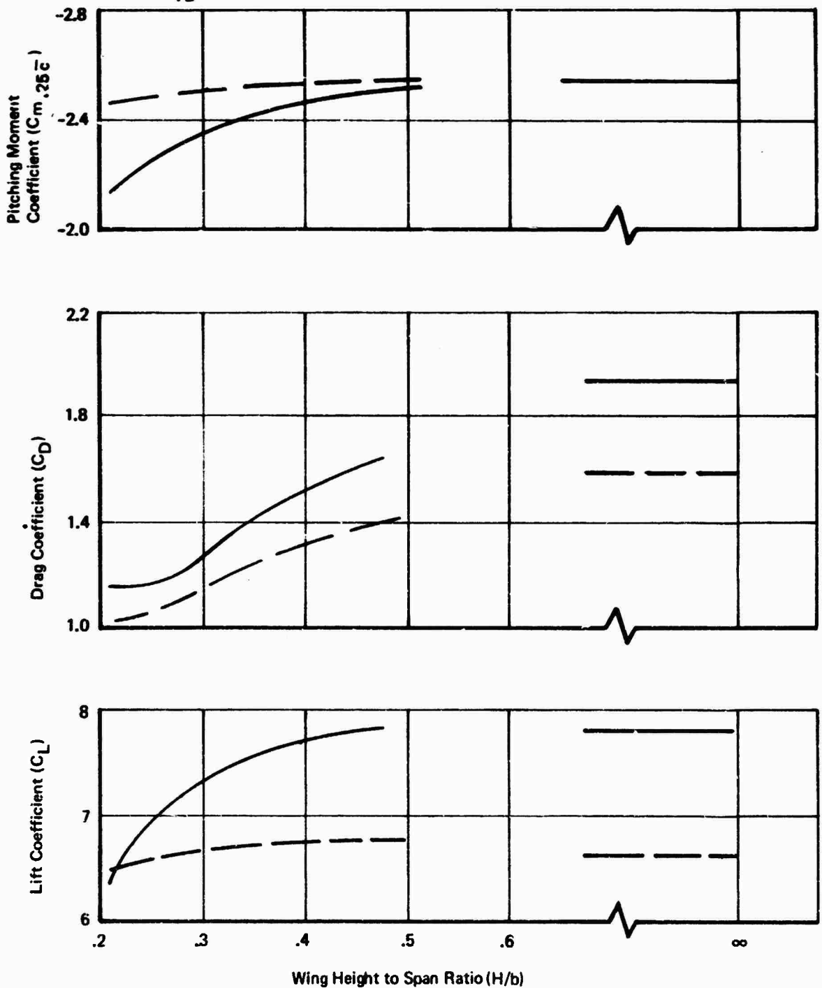
Figure 152: Ground Effect on Jet Flap Characteristics
