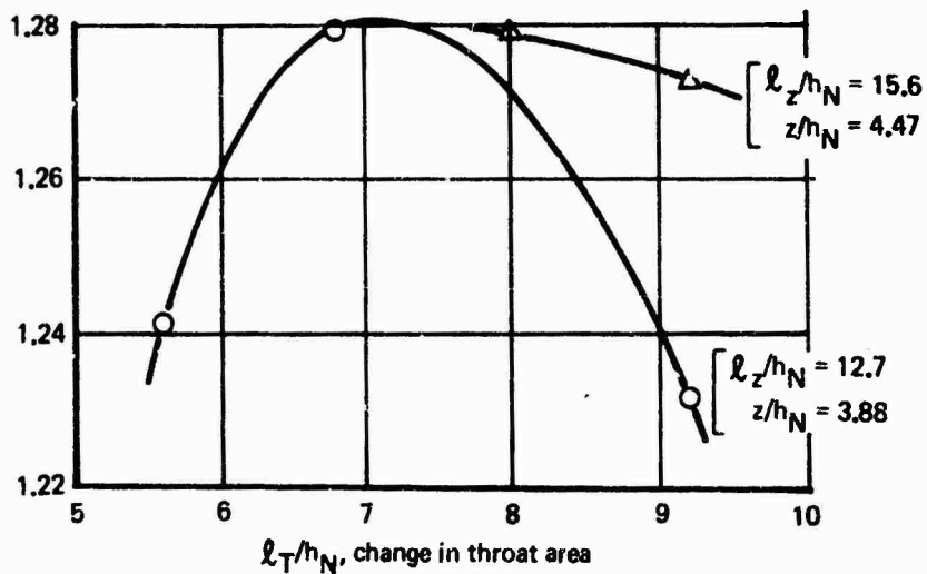
Figure 158: Effect of Augmentor flap Geometry on Static Thrust Augmentation Ratio
