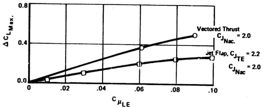
Figure 143: Leading Edge Boundary Layer Control Effectiveness
