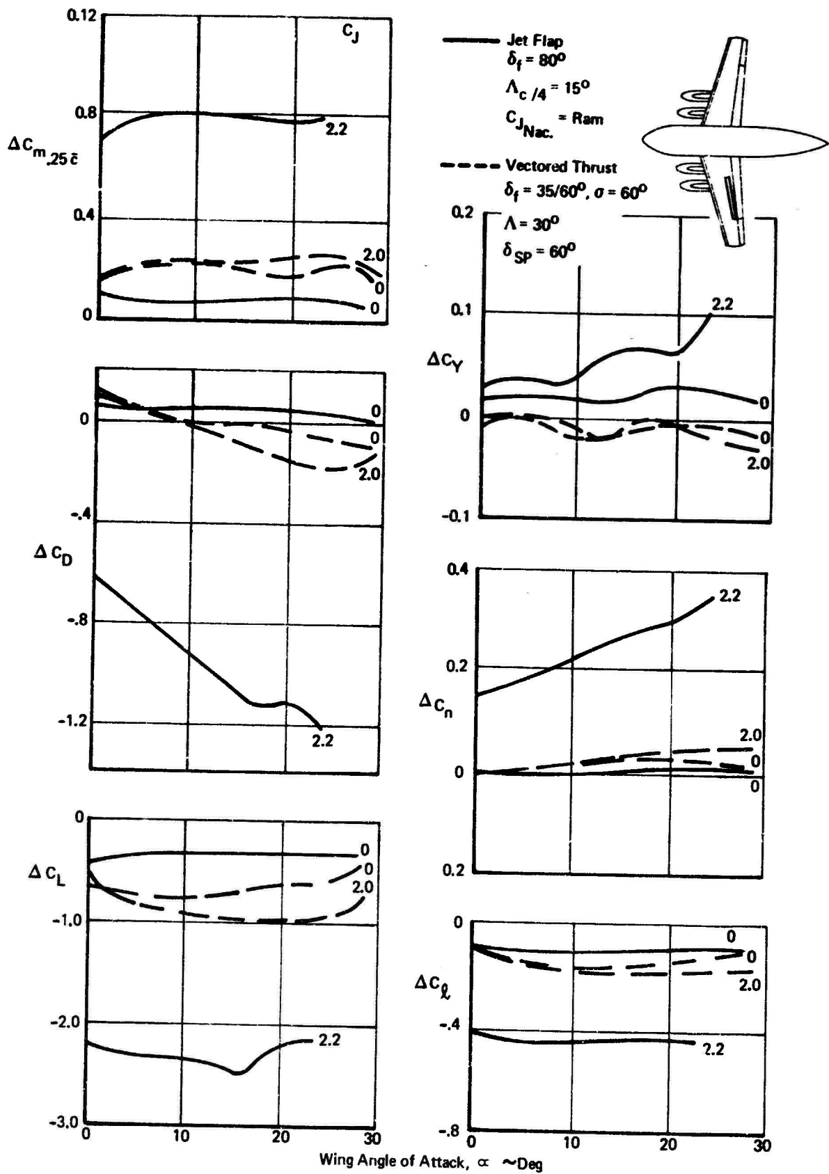
Figure 145: Spoiler Effects — Jet Flap and Vektored Thrust
