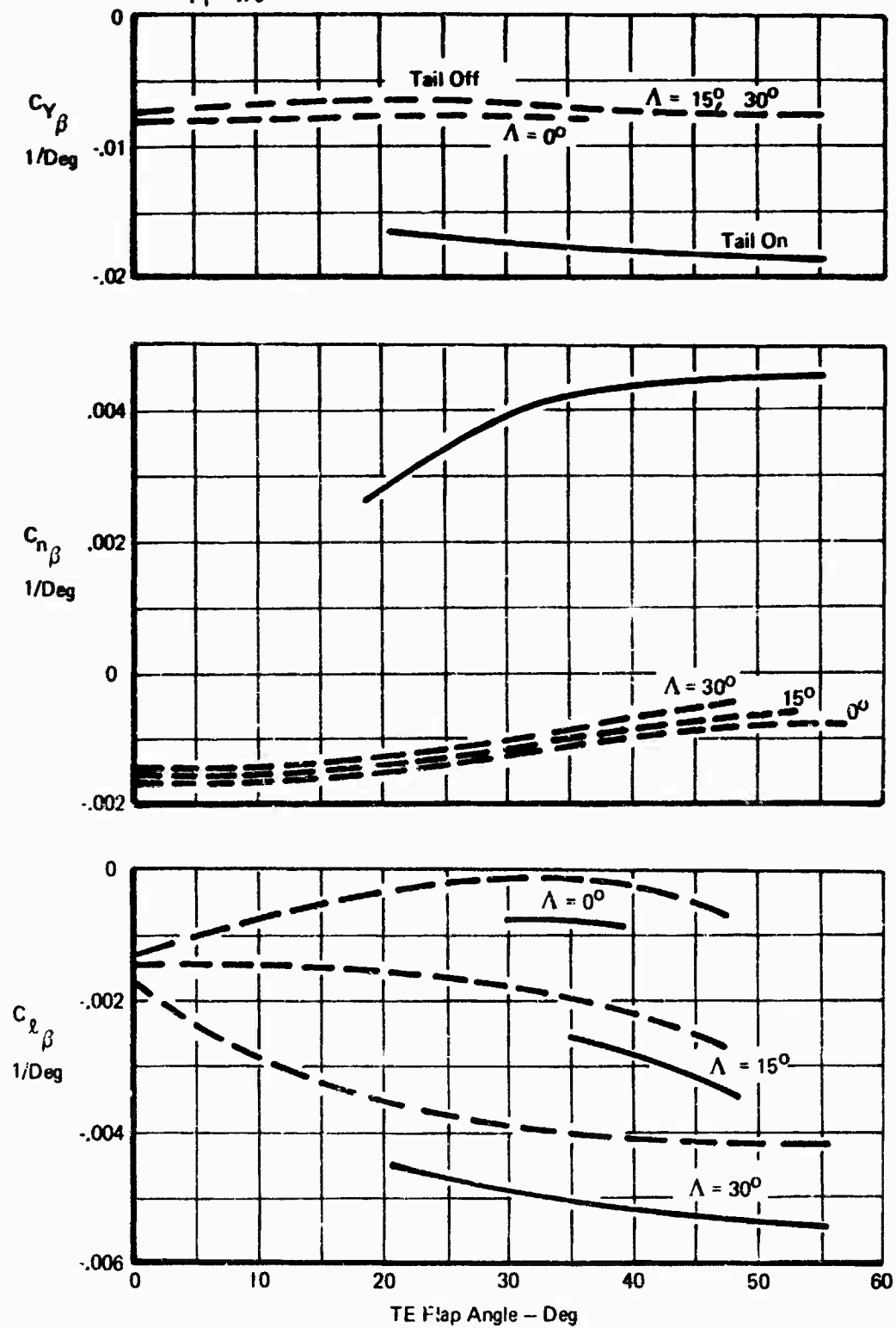
Figure 27: Effect of T.E. Flap Angle on \beta Stability Derivatives
