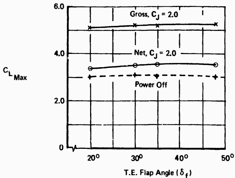
Figure 88: Effect of Flap Angle On C_{L Max}
