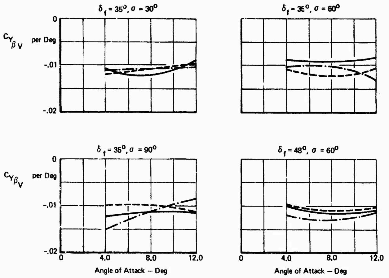
Figure 126: Effect of Angle of Attack on Tail Input to Side Force Derivative
