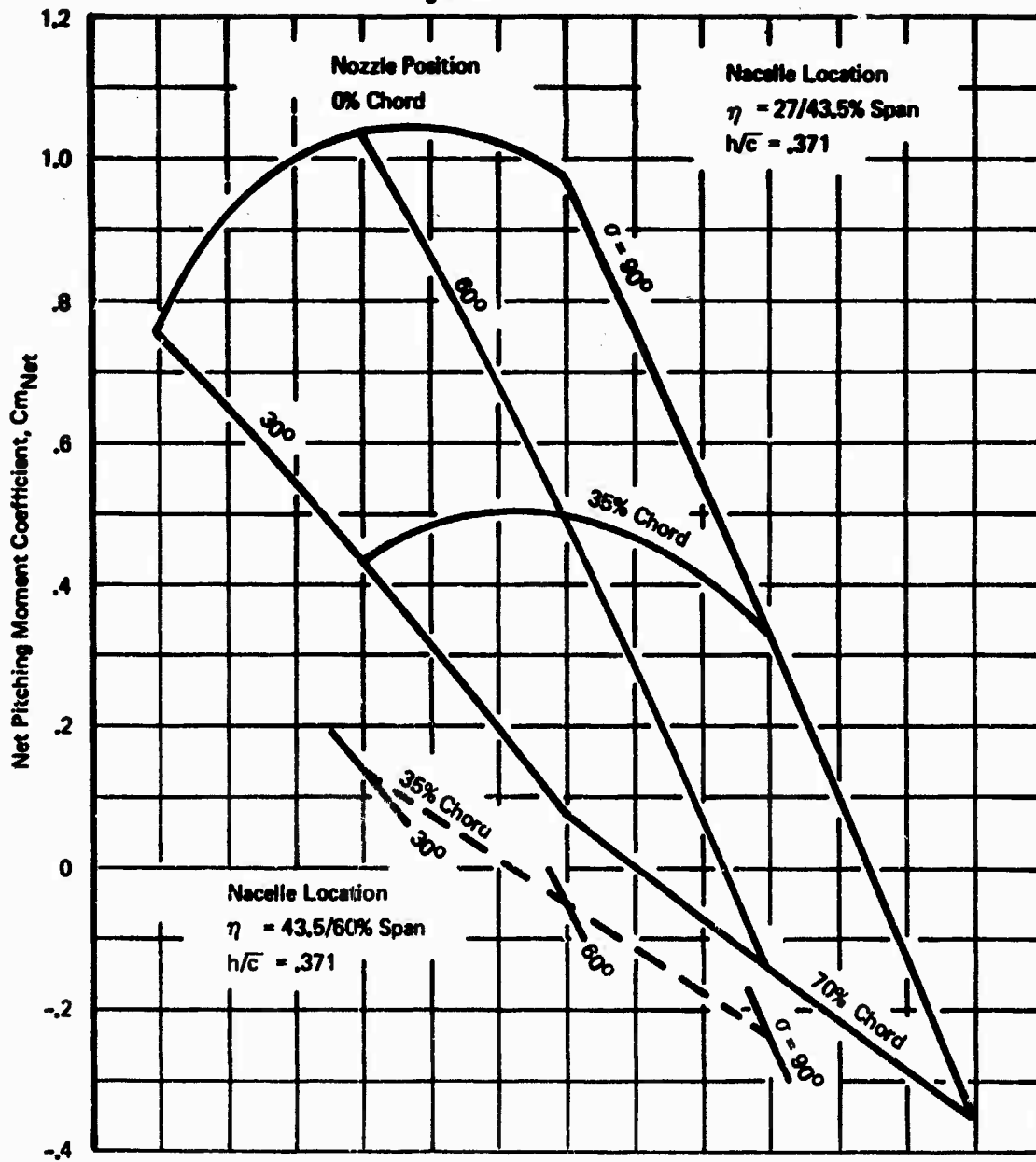
Figure 95: Direct Pitching Moment Due to Vected Thrust
