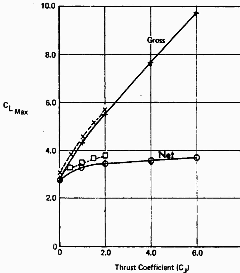
Figure 93: Effect of Reynolds Number on C_{L Max}
