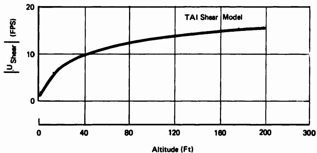
Figure 7: Change in Flightpath Due to Windshear
