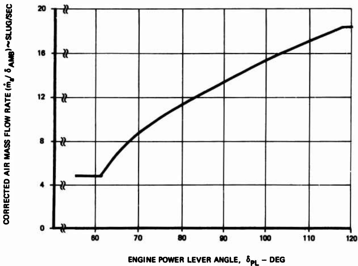
Figure 109: Corrected Air Mass Flow Rate
