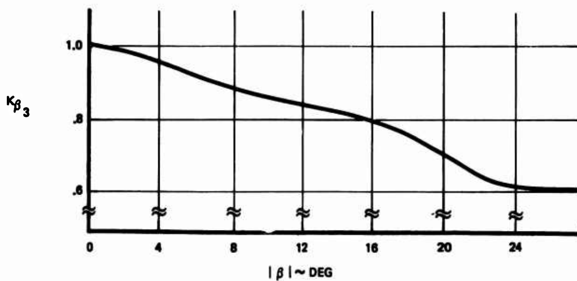
Figure 98: Yawing Moment Due to Directional Control
