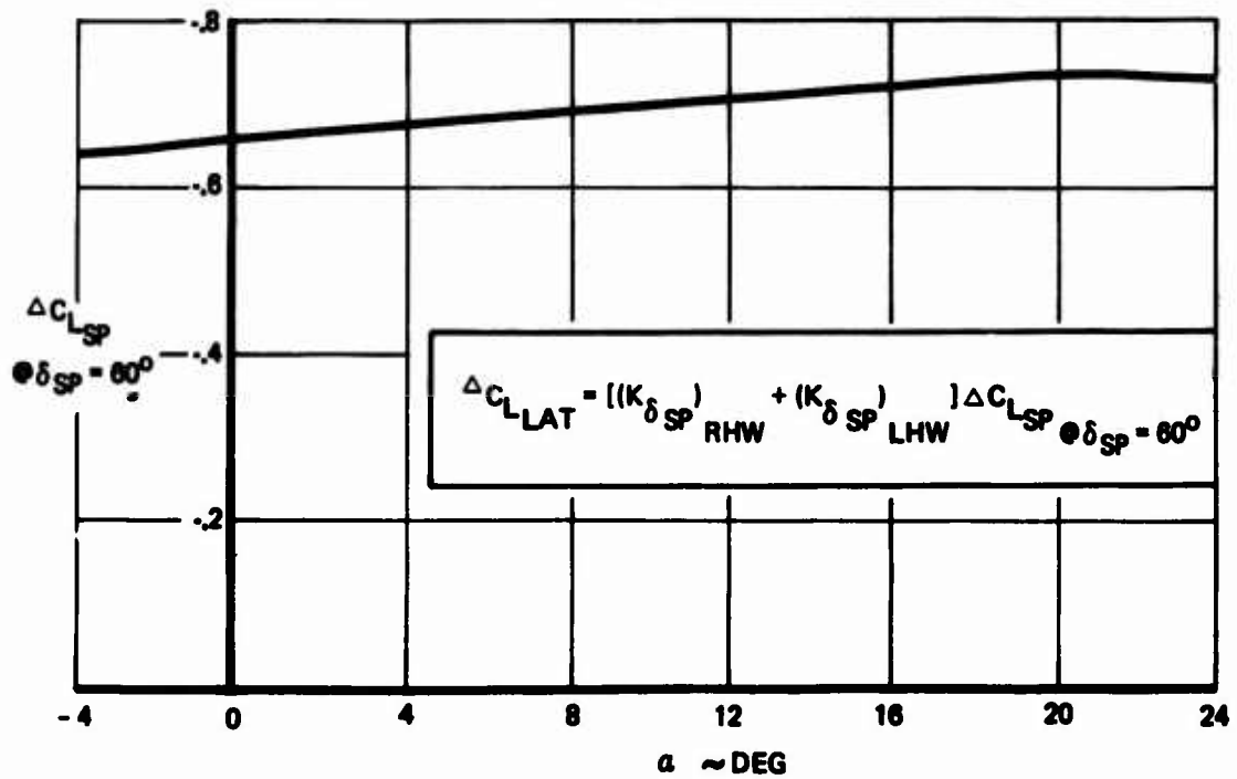
Figure 81: Lift Coefficient Effect of Lateral Control
