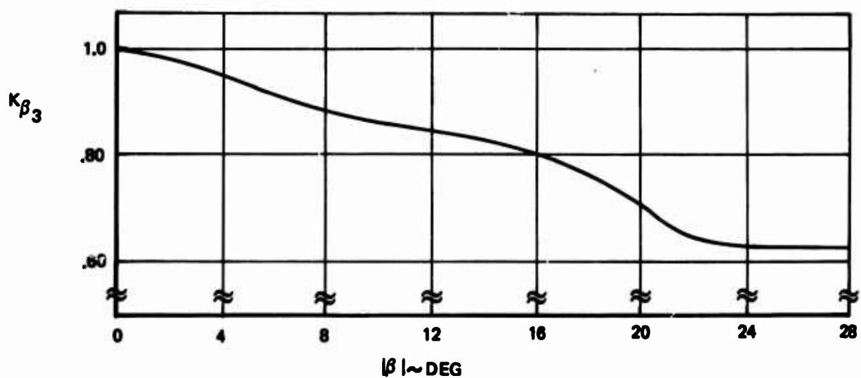
Figure 62: Yawing Moment Coefficient Effect of Rudder Deflection
