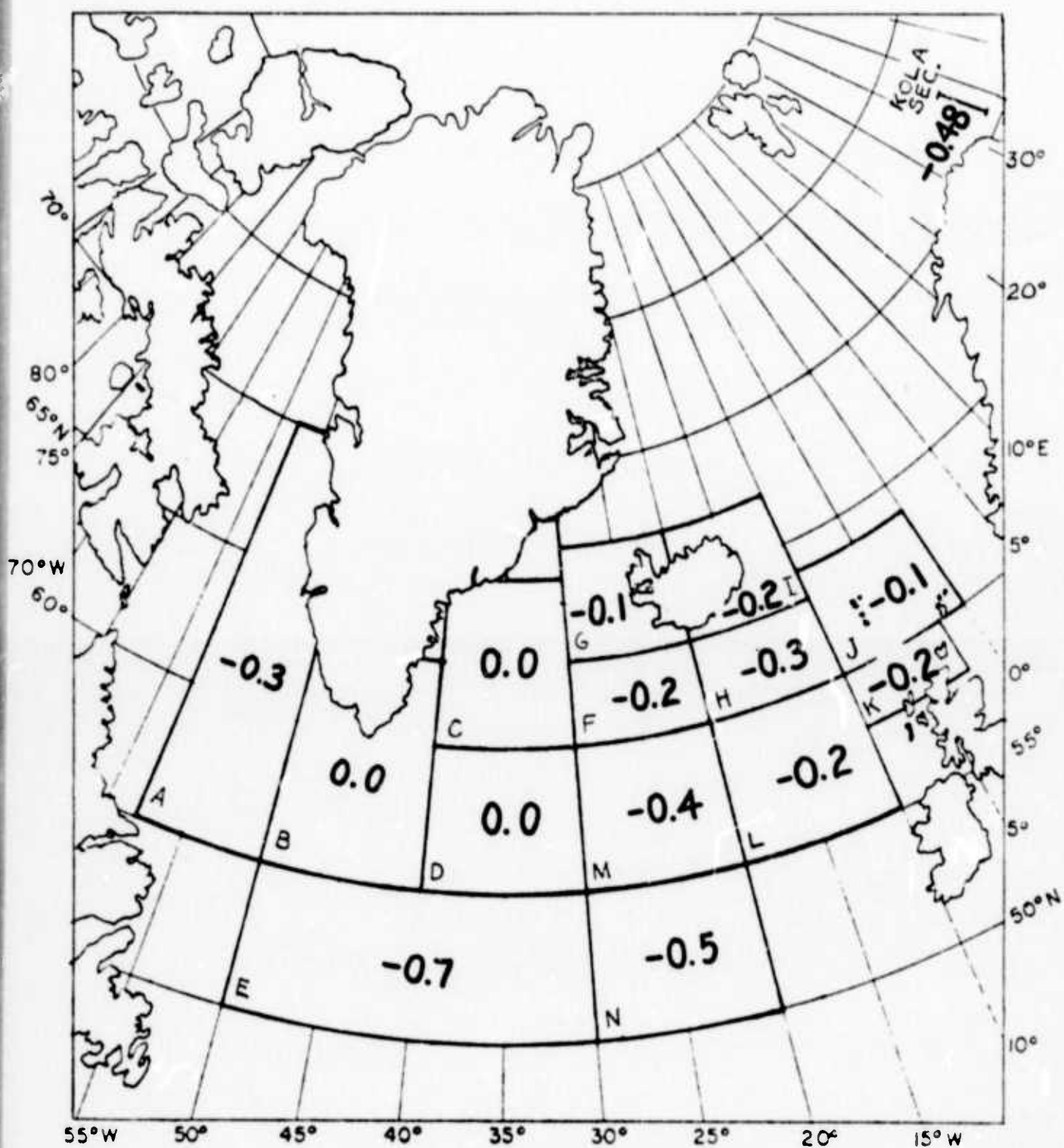
Figure 6. Differences (1961-1970 minus 1951-1960) April-September Sea Surface Temperature Areas A-N and Annual 0-200 m Sea Temperature Kola Section ( ^{\circ}\text{C} ).
