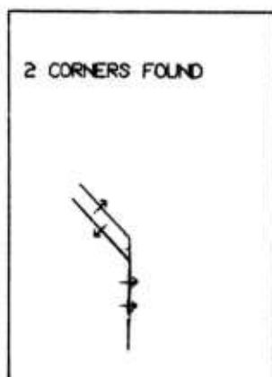
Fig. 13. Digitized picture of two blocks and the matching corners that the program found for the four model corners.
