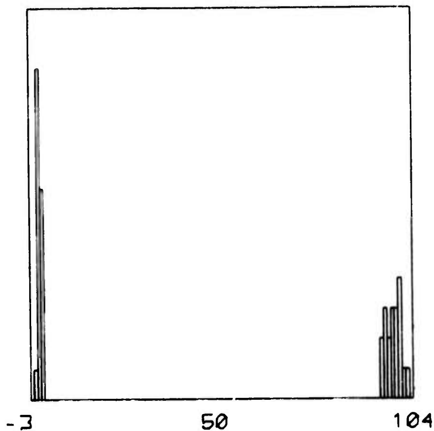
Fig. 2. Histogram of number of edge points versus their residual. (a) All edge points. (b) Edge points in a small \alpha -C region.
