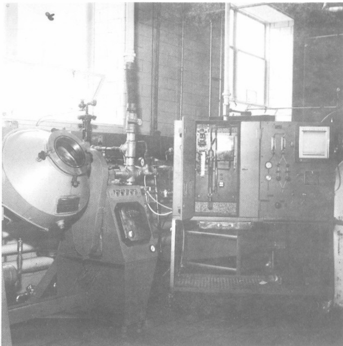
4A.4.1 Vacuum tumble-dryer used for treating fresh or partially-dried lots with mixtures of \text{SO}_2 in air, and the apparatus for metering and analyzing for \text{SO}_2 .
