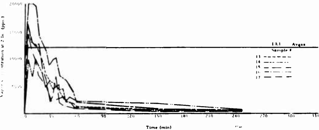
FIGURE III-15. TEST NO. 15—FOUR GALLONS OF AVGAS IN A SPILL TEST
