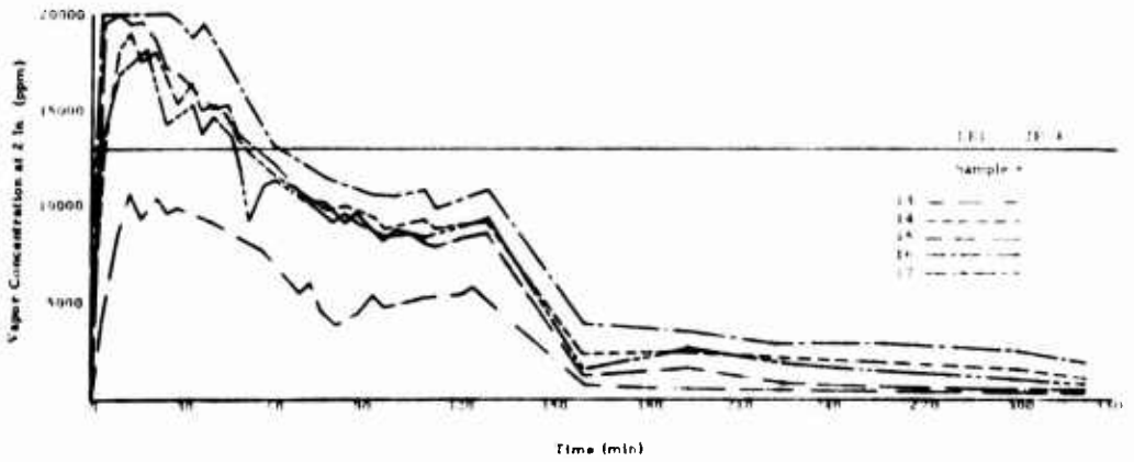
FIGURE III-22. TEST NO. 22 FOUR GALLONS OF JP-4 IN A SPILL TEST
