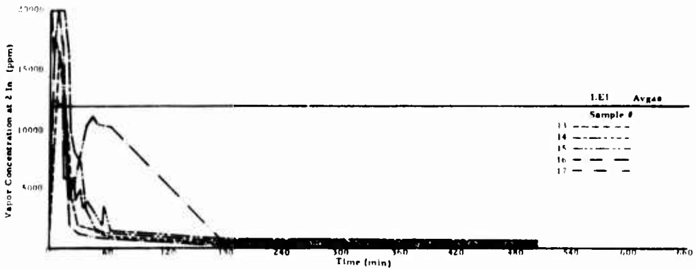
FIGURE III-12. TEST NO. 12—FOUR GALLONS OF AVGAS IN A SPILL TEST
