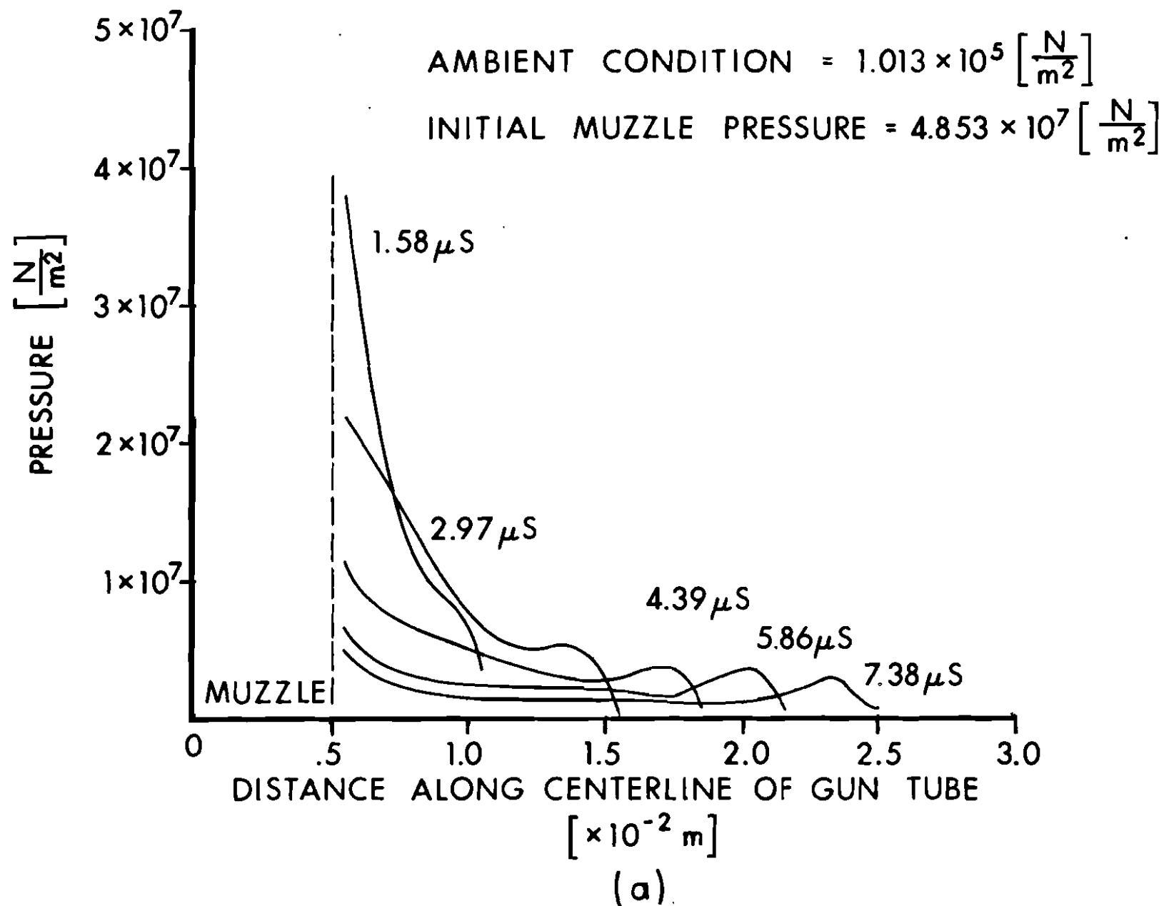
Figure 5. Pressure Versus Distance along the Axis of the Gun Tube.
