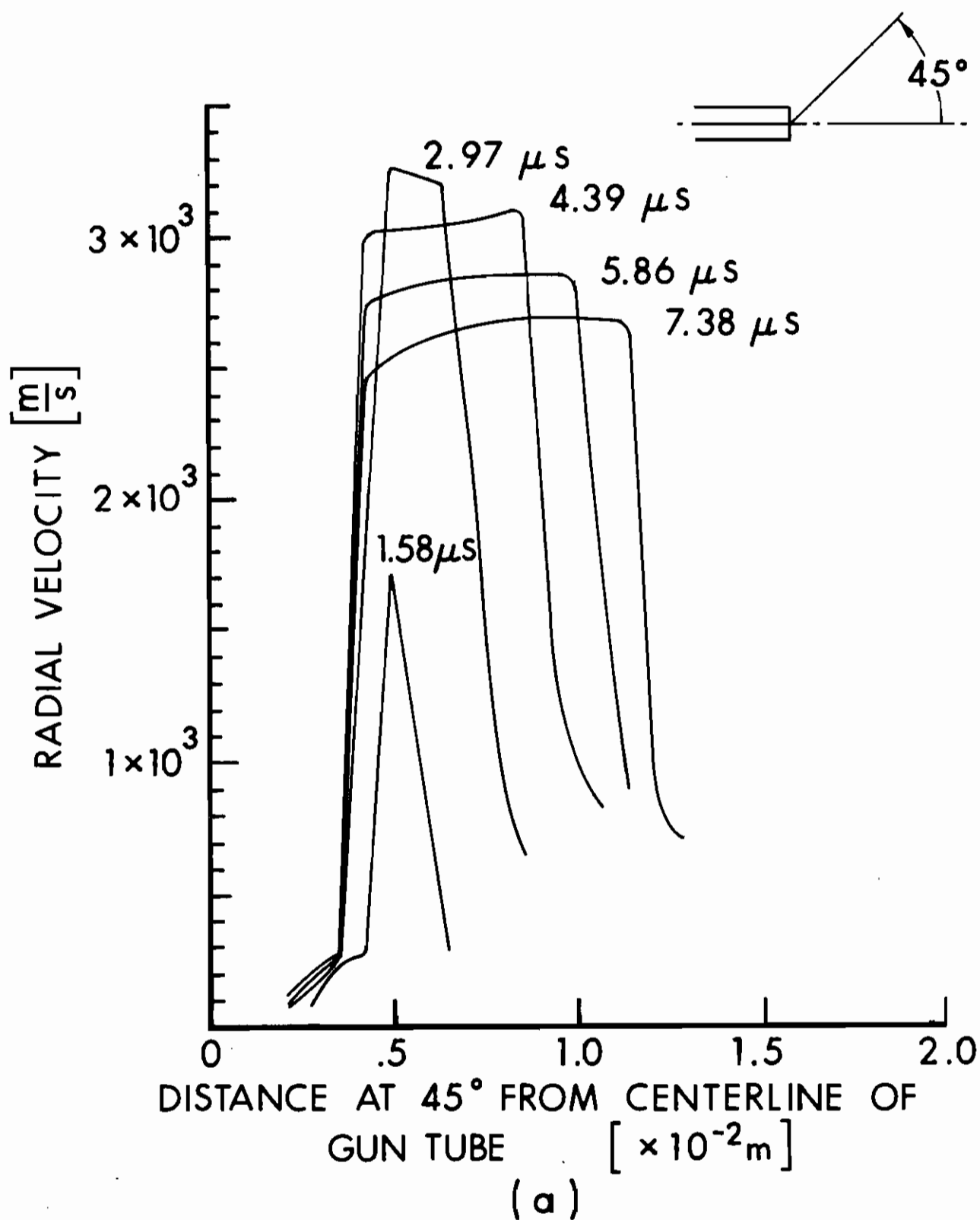
Figure 10. Radial Velocity Versus Distance at 45^\circ from Axis of the Gun.
