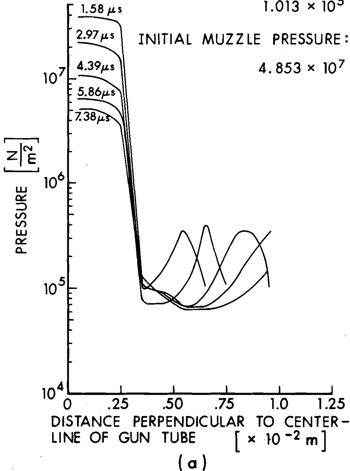
Figure 6. Pressure Versus Distance at 90° from the Axis of the Gun Tube Measured from the Muzzle.
