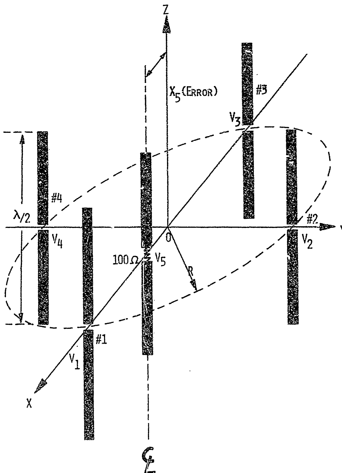
Figure 1 : A Four-Element Circular Array, Progressively Phased. A Fifth Element is Placed Near Array Center, Where the Null is.
