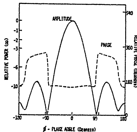
FIGURE 4. RADIATION AND PHASE PATTERNS OF THE ARRAY WHEN ALL PHASE SHIFTERS ARE EXCITED PER TABLE II.
