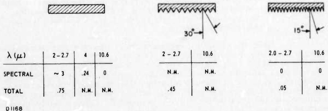
Fig. 9 Results of Spectral and Total Reflectivity Measurements of Three Different Surfaces
