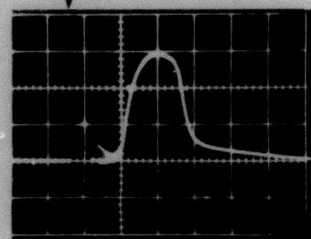
Fig. 22a The Temporal Behavior of 2P Transitions
