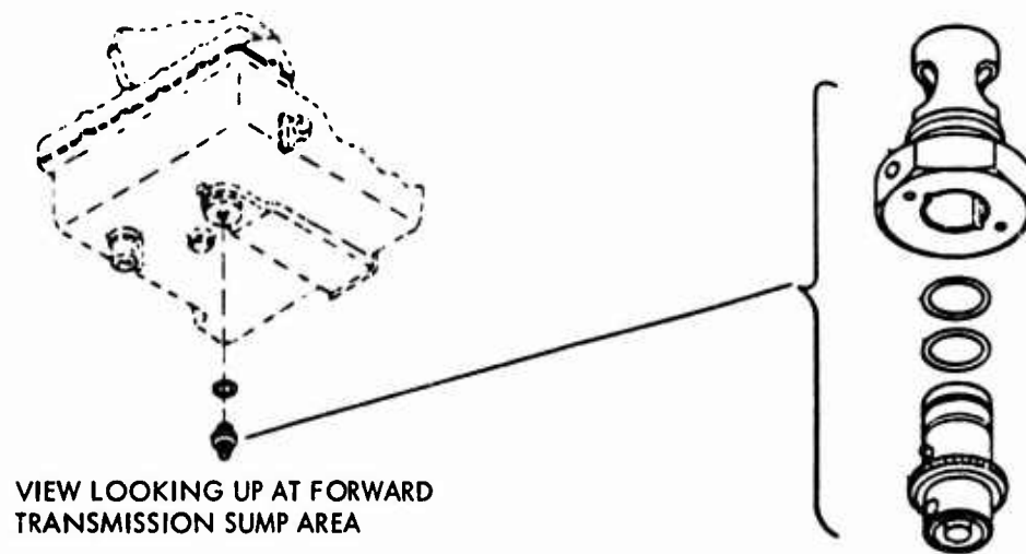
Figure 26. Bayonet-Type Chip Detector, Transmission Installation.
