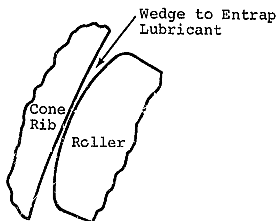
Figure 73. Roller-End/Cone Rib (Flange) Contact.
