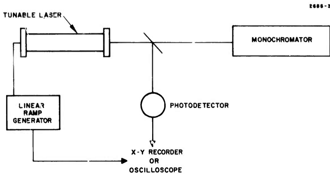
Fig. 5. Experimental arrangement for tuning range measurements.
