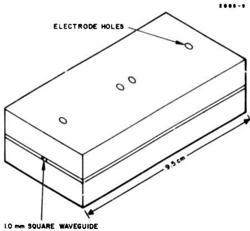
Fig. 16. Square bore, BeO waveguide laser.
