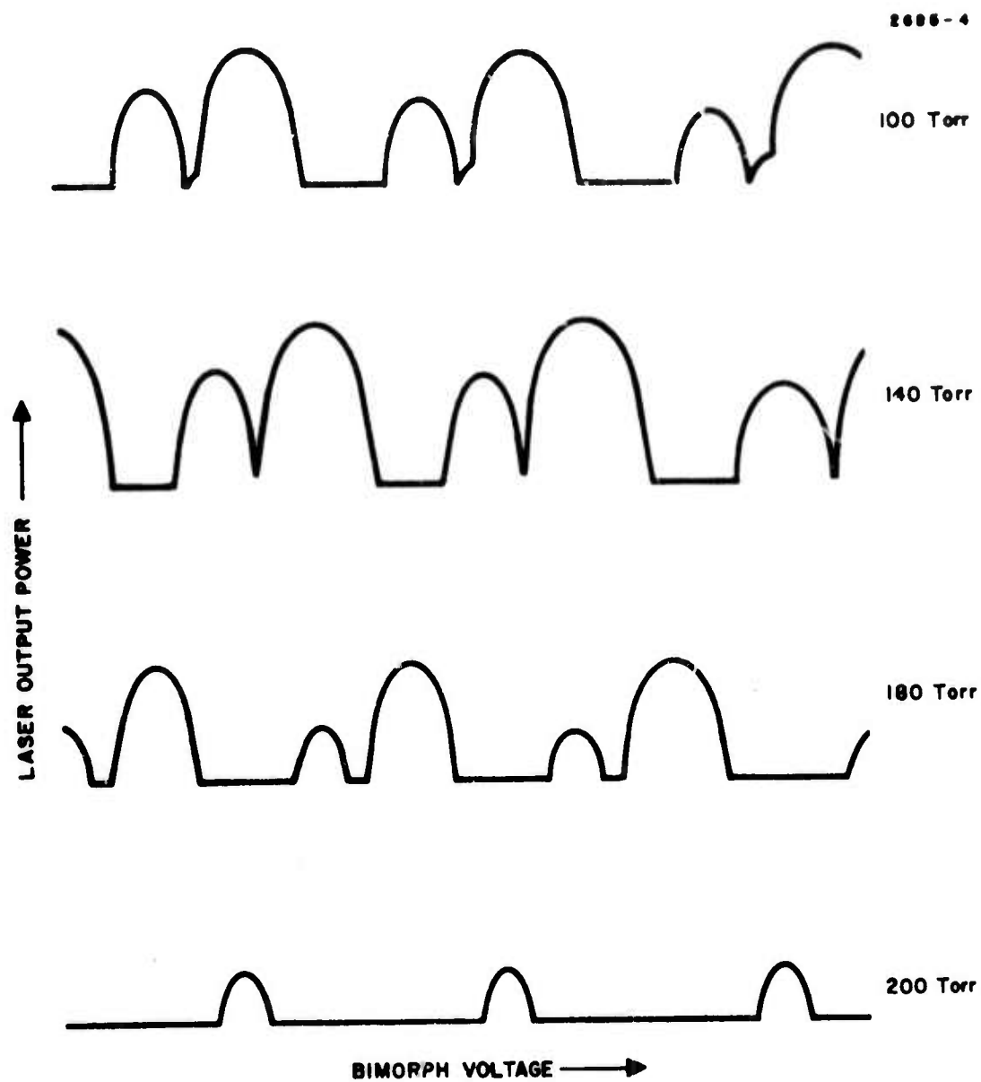
Fig. 7. Tuning characteristic of tube A-18 for various total gas pressures.
