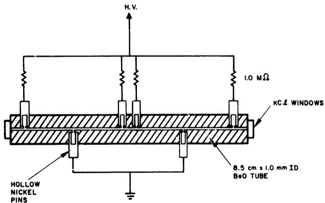
Fig. 1. Test section for multiple electrode geometry.
