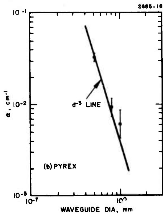
Fig. 15. Measured waveguide losses for precision bore.
