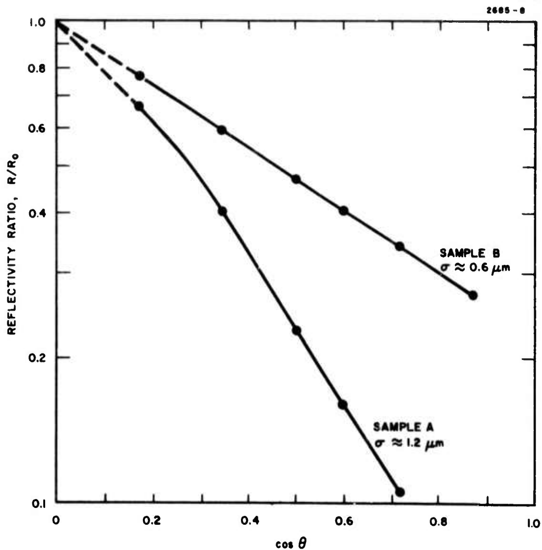
Fig. 13. Reflectivity ratio R/R_0 versus \cos \theta .
