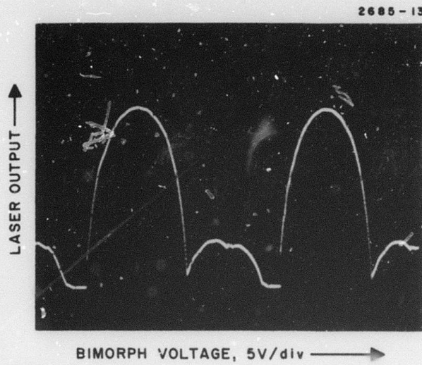
Fig. 6. Laser output power versus bimorph tuning for tube A-18.
