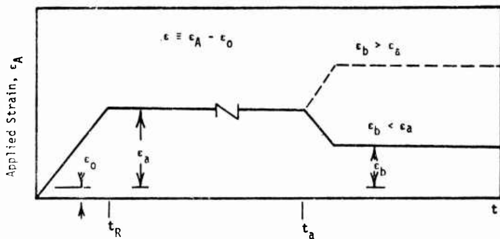
APPLIED STRAIN HISTORY FOR TWO-STEP RELAXATION TEST
